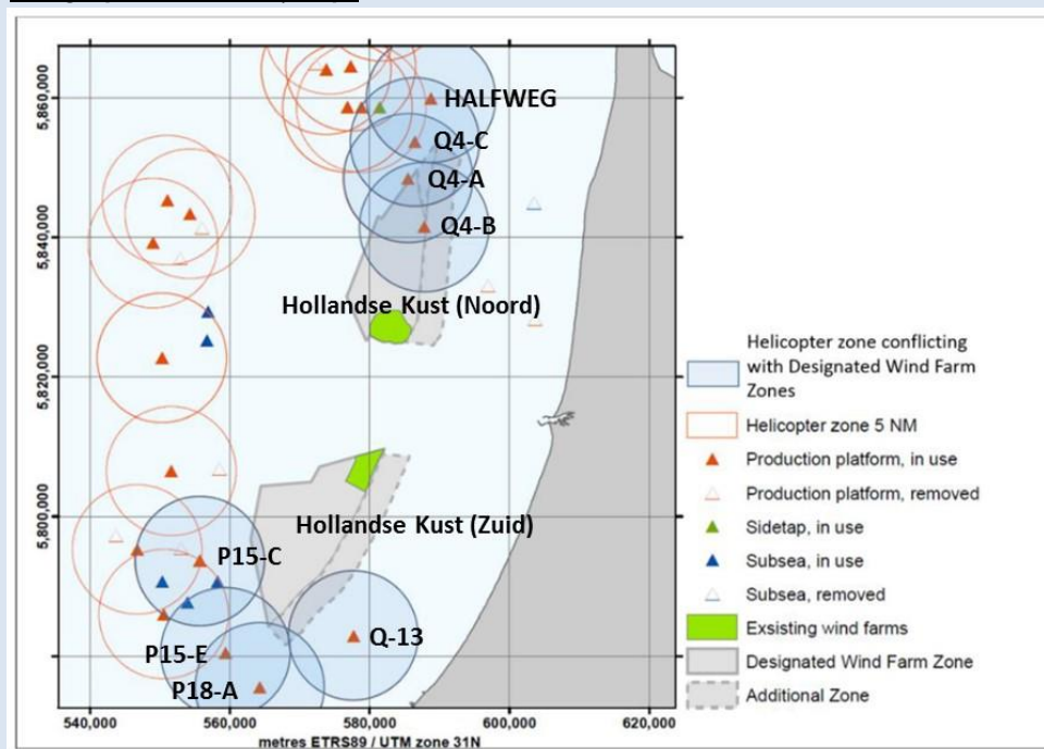
Oil & gas platforms in study scope
