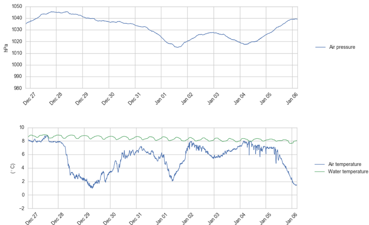
Figure 4.1 Time series plots of air pressure (upper panel), air and water temperature (lower panel), 26 Dec - 6 Jan 2017.
