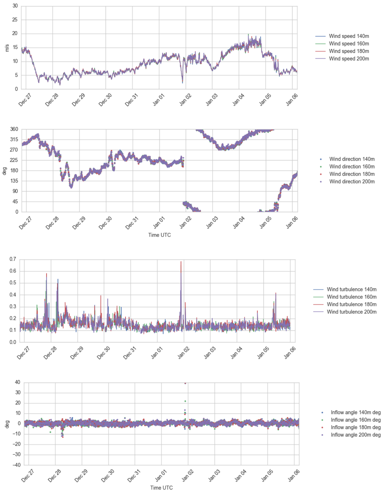
Figure 4.12 Plots of wind profile data, 140 – 200 m a.s.l., 26 Dec - 6 Jan 2017.
