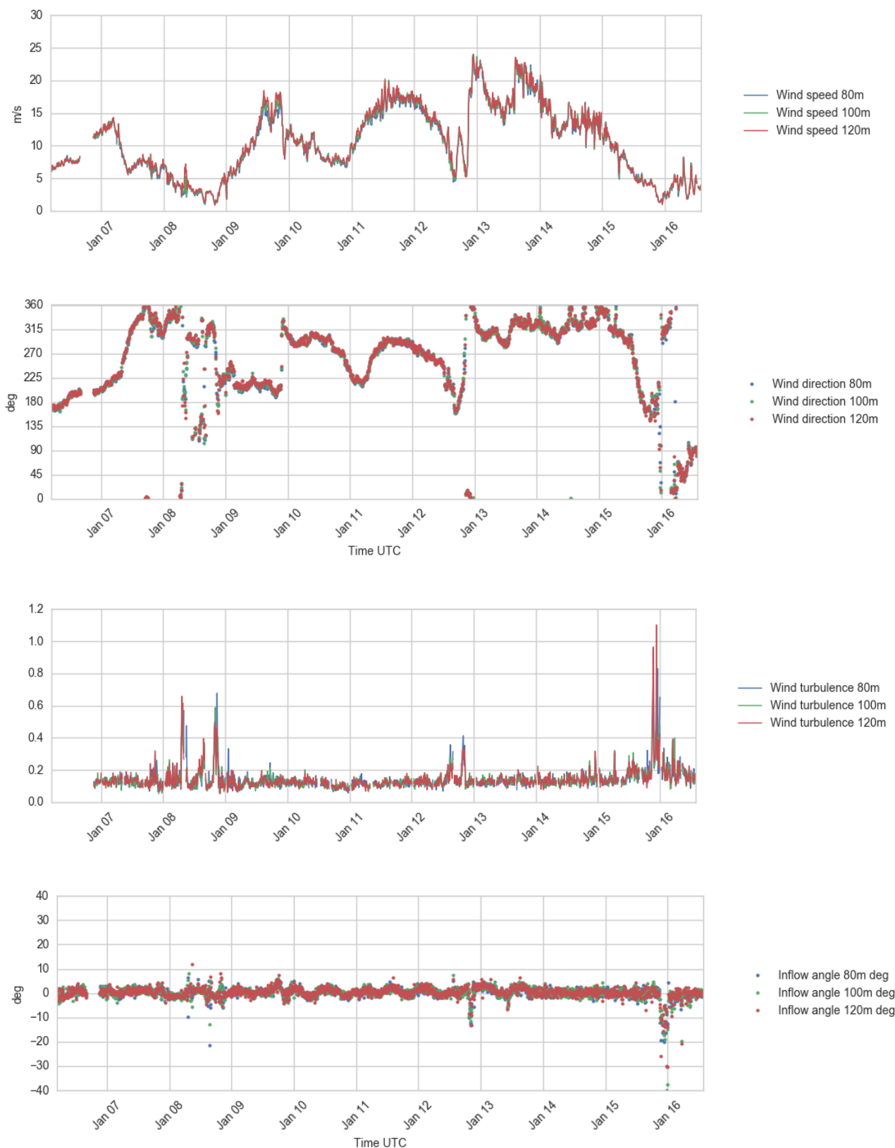
Figure 4.14 Plots of wind profile data, 80 – 120 m a.s.l., 6 - 16 Jan 2017.
