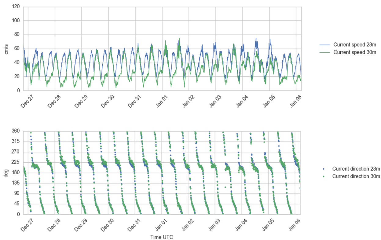
Figure 4.22 Time series plots of current speed (upper) and direction (lower panel), 28 - 30 m depth, 26 Dec - 6 Jan 2017.
