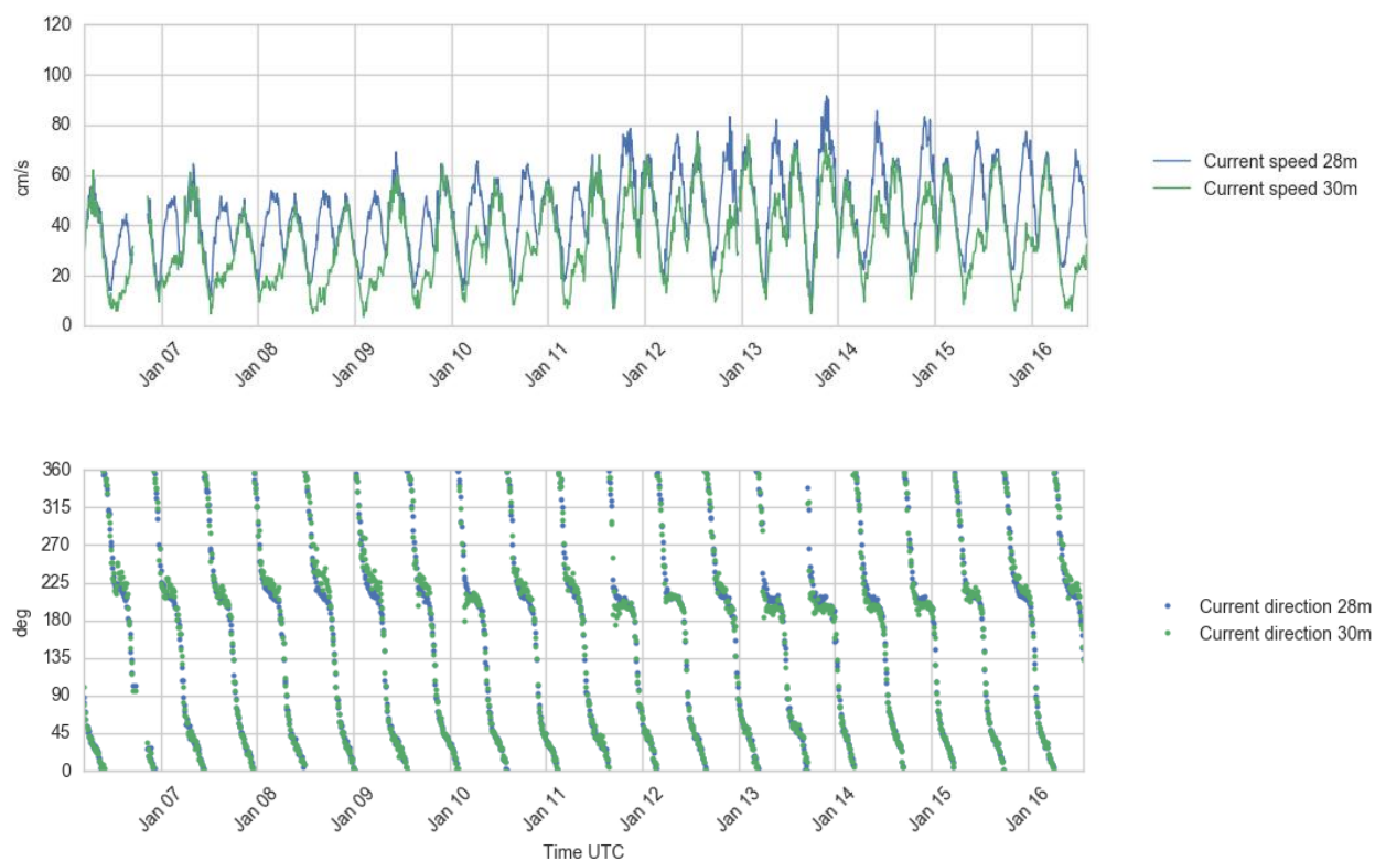
Figure 4.26 Time series plots of current speed (upper) and direction (lower panel), 28 – 30 m depth, 6 - 16 Jan 2017.
