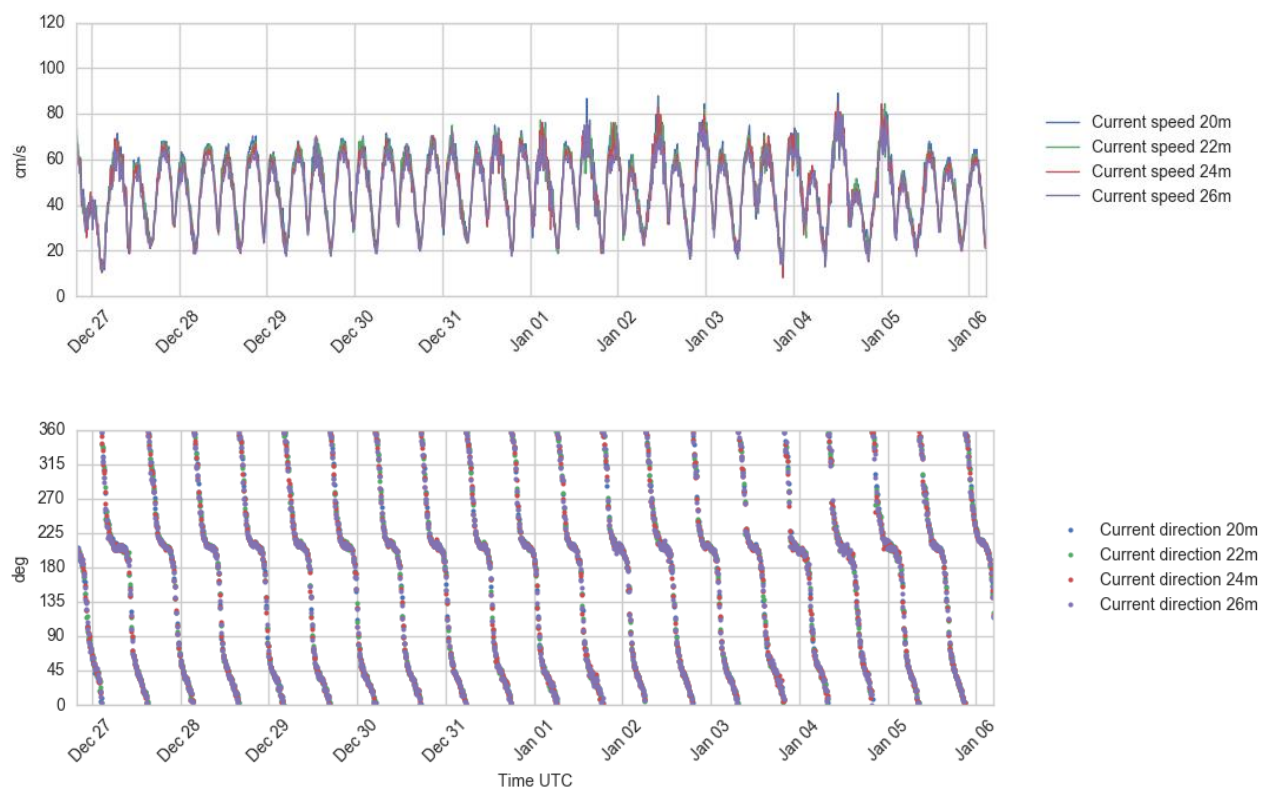
Figure 4.21 Time series plots of current speed (upper) and direction (lower panel), 20 - 26 m depth, 26 Dec - 6 Jan 2017.
