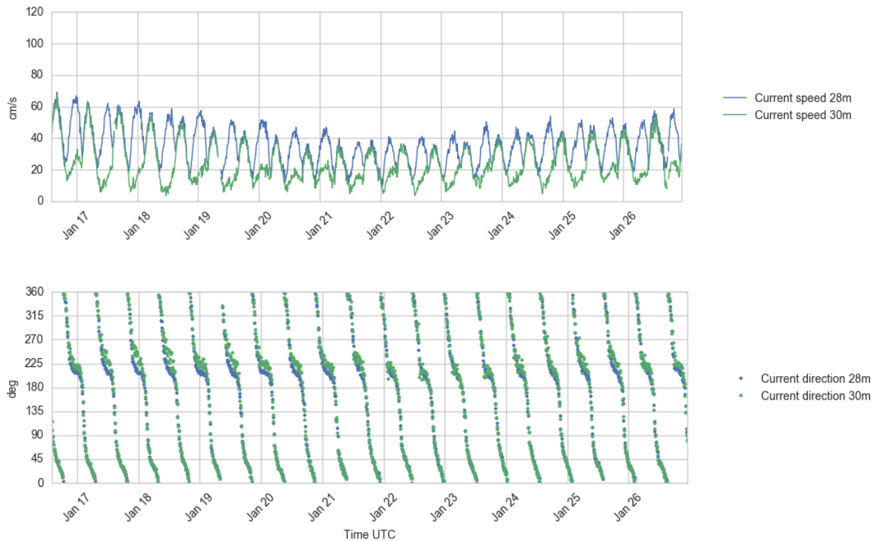
Figure 4.30 Time series plots of current speed (upper) and direction (lower panel), 28 - 30 m depth, 16 - 26 Jan 2017.
