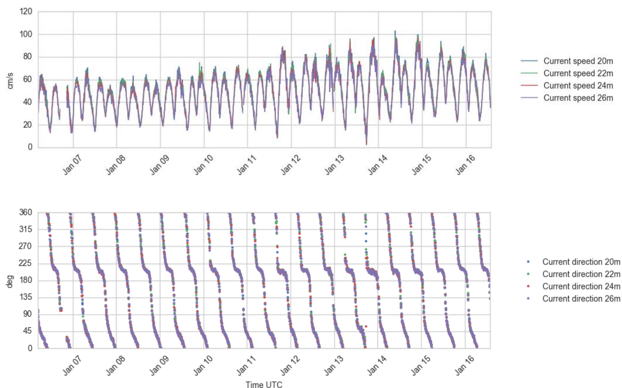
Figure 4.25 Time series plots of current speed (upper) and direction (lower panel), 20 – 26 m depth, 6 - 16 Jan 2017.
