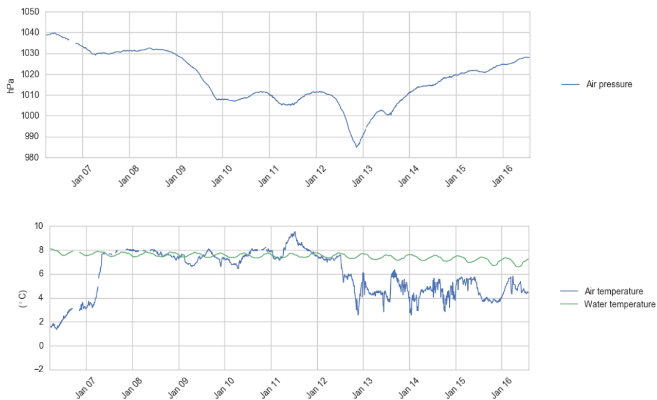
Figure 4.2 Time series plots of air pressure (upper panel), air and water temperature (lower panel), 6 - 16 Jan 2017.
