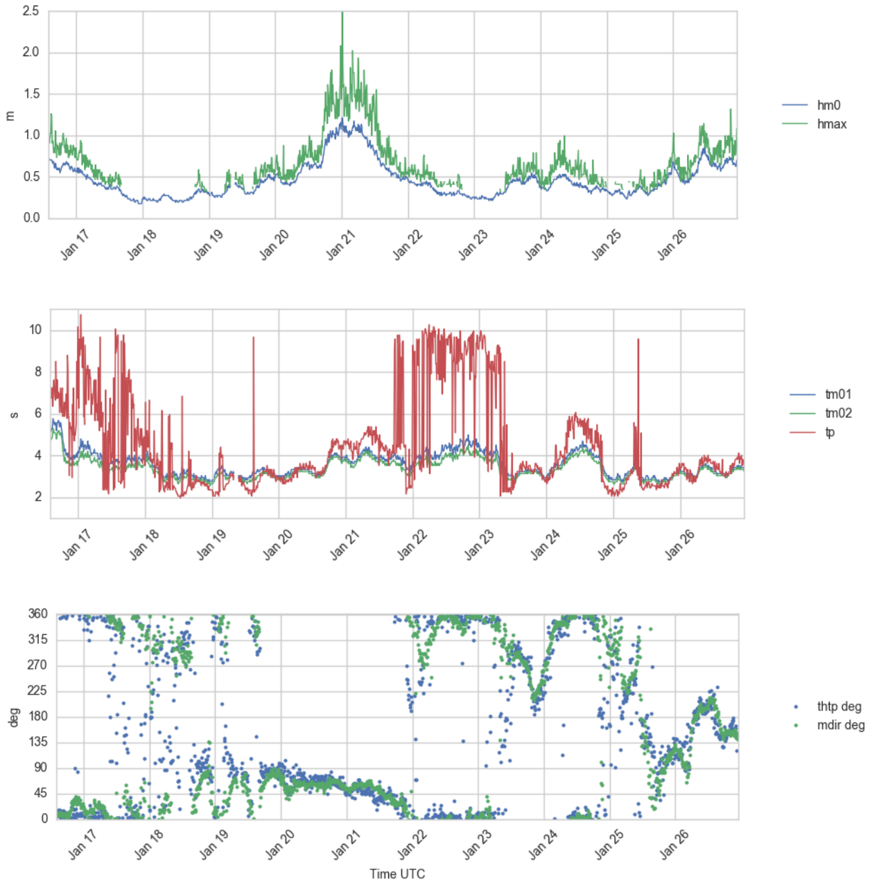
Figure 4.6 Time series plots of wave height (Hm0 and Hmax) (upper panel), wave period (Tm01, Tm02 and Tp) (second panel), and wave direction (ThTp and Mdir) (lower panel), 16 - 26 Jan 2017.
