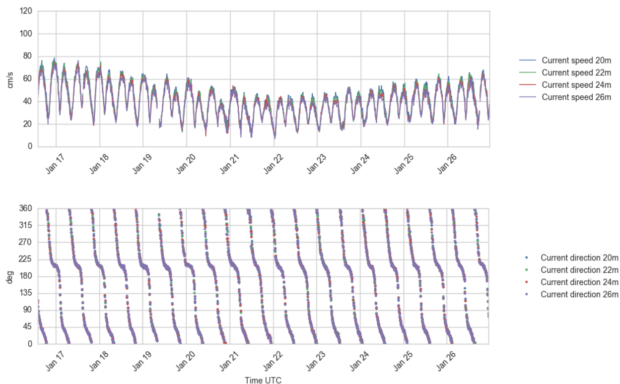
Figure 4.29 Time series plots of current speed (upper) and direction (lower panel), 20 - 26 m depth, 16 - 26 Jan 2017.
