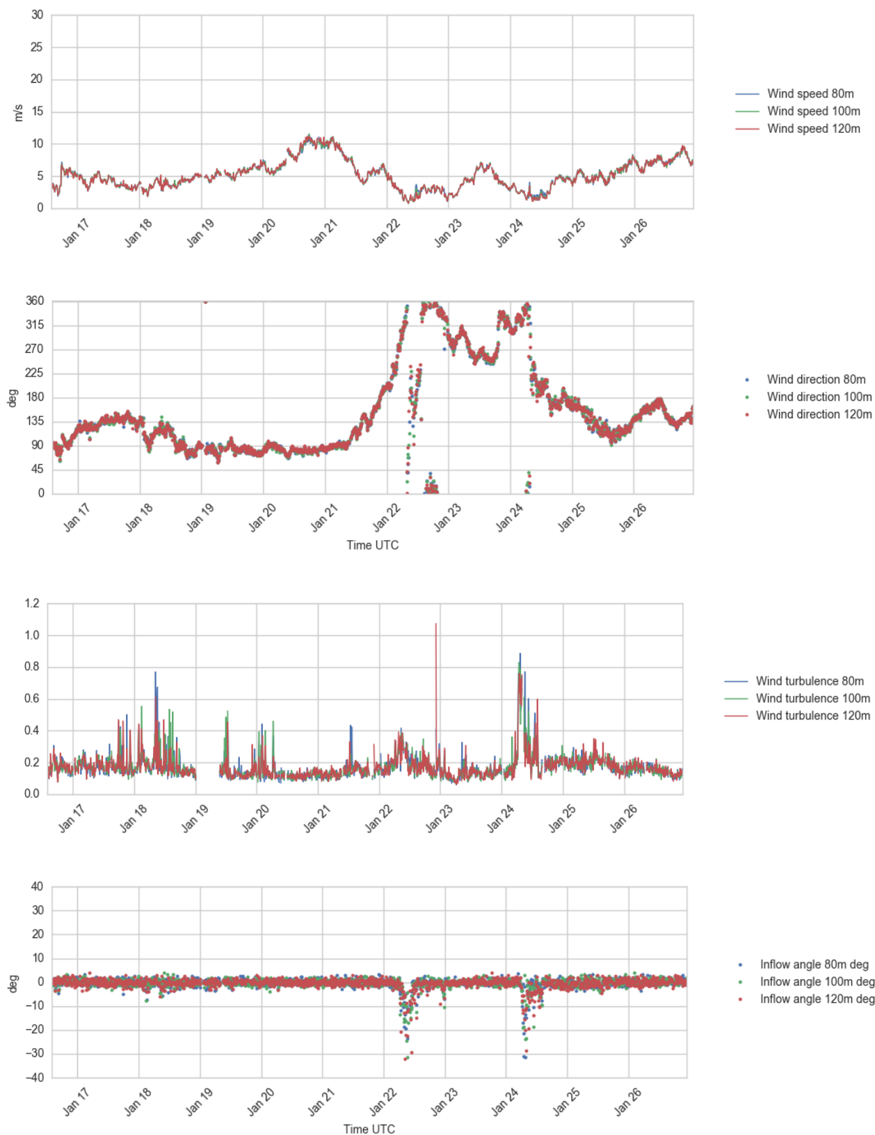
Figure 4.17 Plots of wind profile data, 80 – 120 m a.s.l., 16 - 26 Jan 2017.
