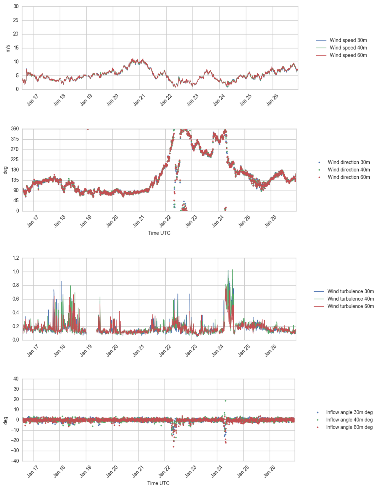
Figure 4.16 Plots of wind profile data, 30 – 60 m a.s.l., 16 - 26 Jan 2017.
