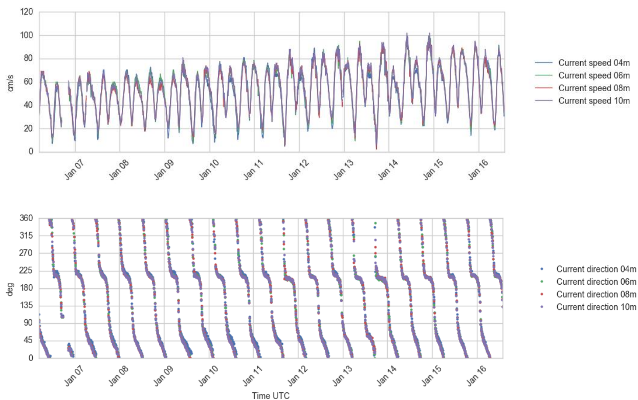
Figure 4.23 Time series plots of current speed (upper) and direction (lower panel), 4 - 10 m depth, 6 - 16 Jan 2017.
