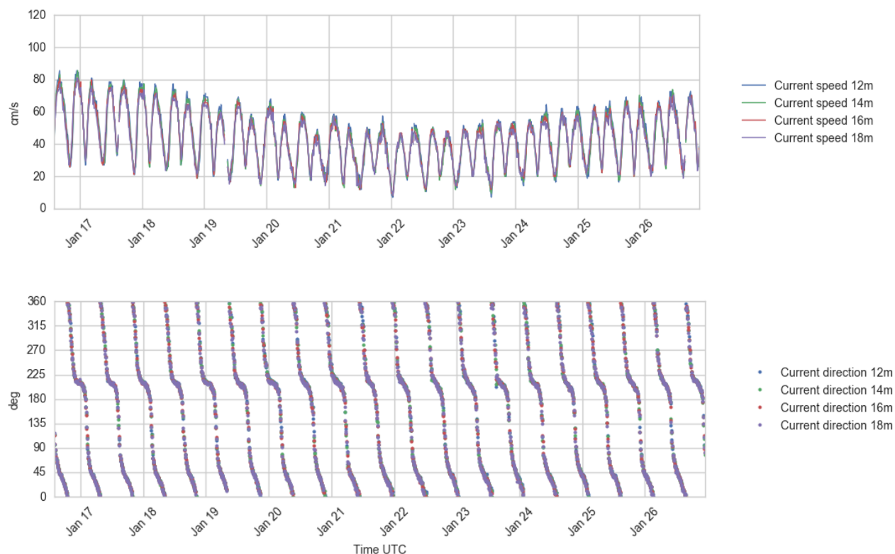
Figure 4.28 Time series plots of current speed (upper) and direction (lower panel), 12 - 18 m depth, 16 - 26 Jan 2017.
