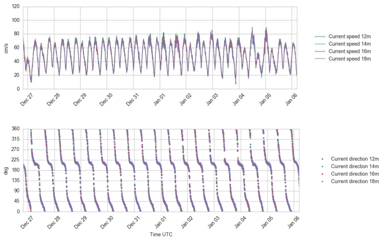
Figure 4.20 Time series plots of current speed (upper) and direction (lower panel), 12 - 18 m depth, 26 Dec - 6 Jan 2017.
