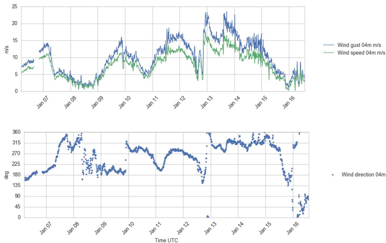
Figure 4.8 Plots of wind speed and gust (upper), and wind direction (lower) at 4 m a.s.l., 6 - 16 Jan 2017.
