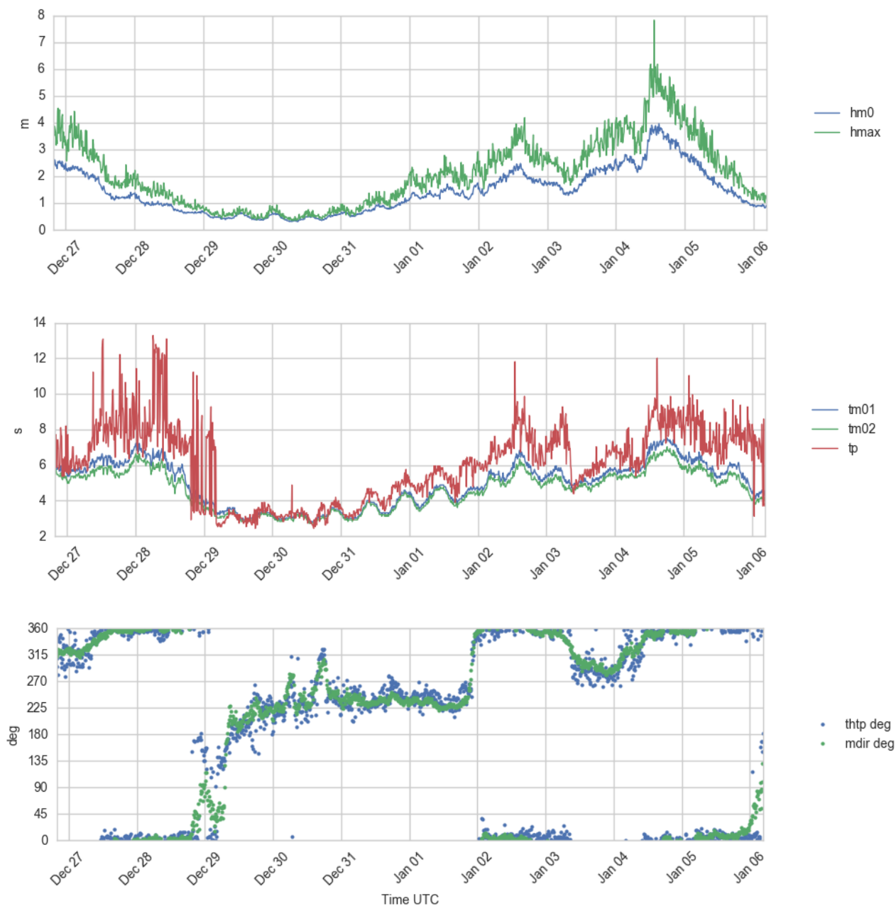
Figure 4.4 Time series plots of wave height ( Hm0 and Hmax ) (upper panel), wave period ( Tm01 , Tm02 and Tp ) (second panel), and wave direction ( ThTp and Mdir ) (lower panel), 26 Dec - 6 Jan 2017.
