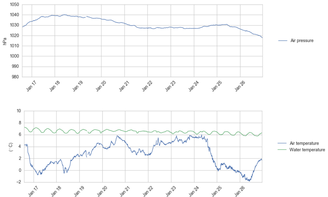
Figure 4.3 Time series plots of air pressure (upper panel), air and water temperature (lower panel), 16 - 26 Jan 2017.
