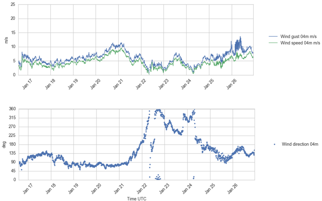
Figure 4.9 Plots of wind speed and gust (upper), and wind direction (lower) at 4 m a.s.l., 16 - 26 Jan 2017.
