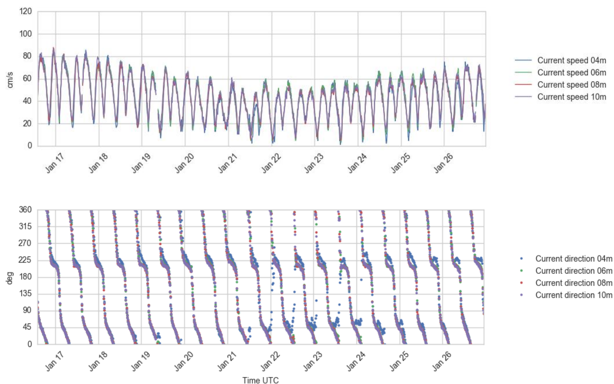
Figure 4.27 Time series plots of current speed (upper) and direction (lower panel), 4 - 10 m depth, 16 - 26 Jan 2017.
