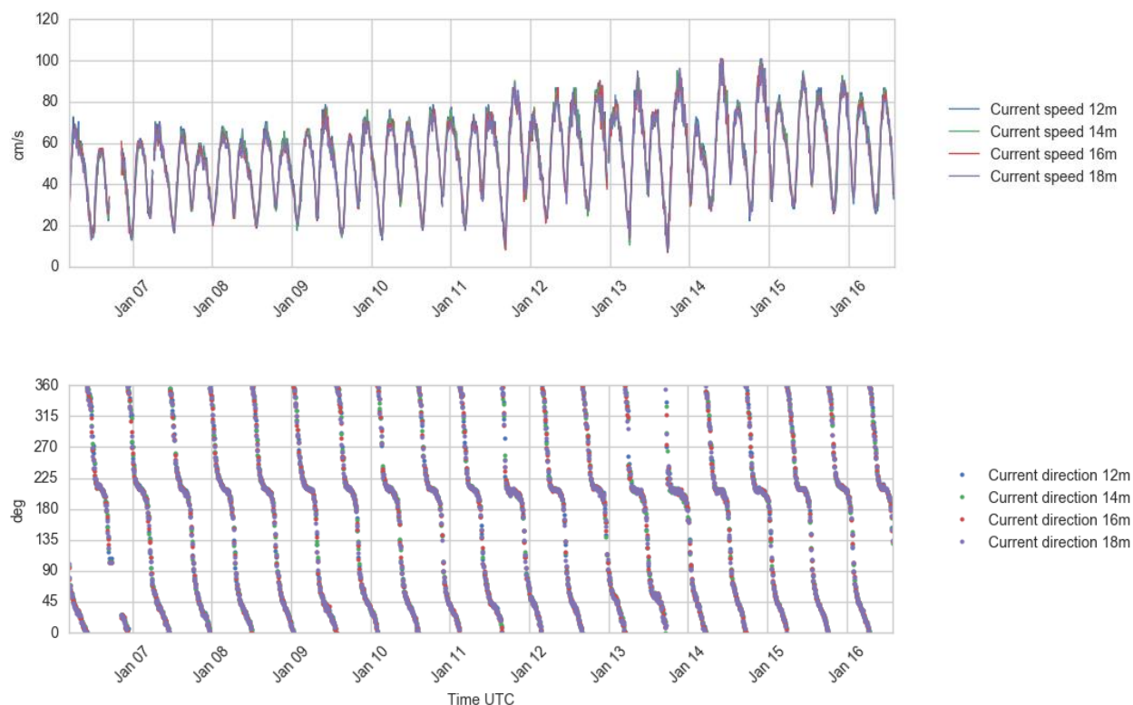
Figure 4.24 Time series plots of current speed (upper) and direction (lower panel), 12 -18 m depth, 6 - 16 Jan 2017.
