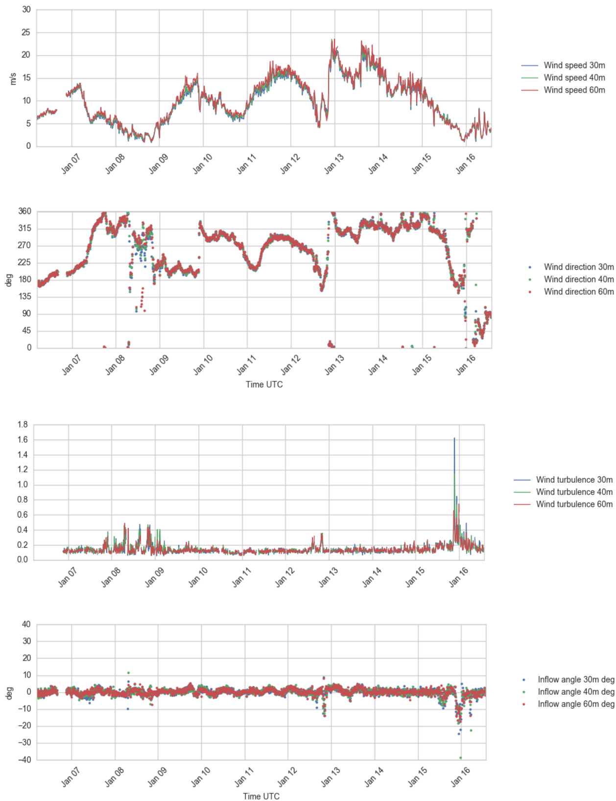
Figure 4.13 Plots of wind profile data, 30 – 60 m a.s.l., 6 - 16 Jan 2017.
