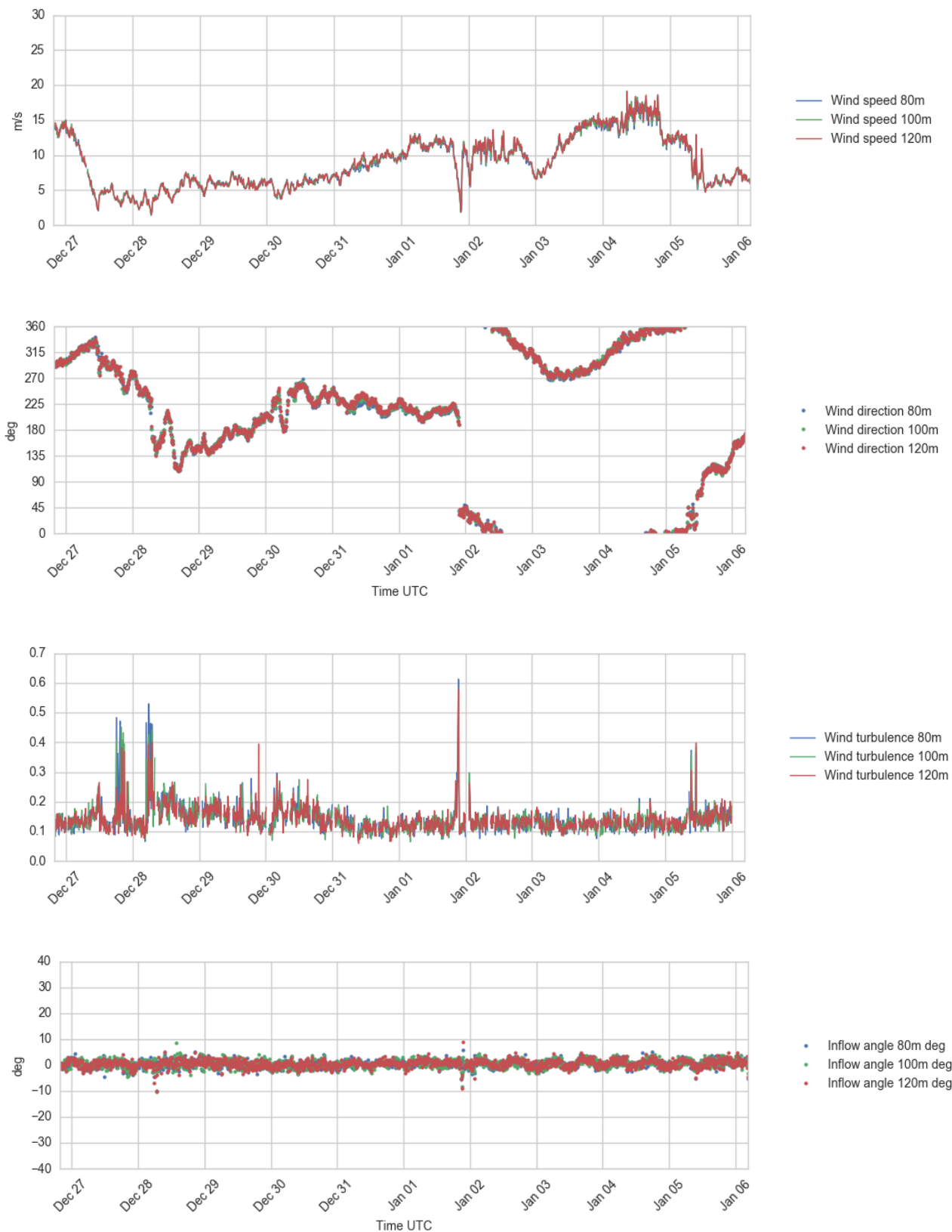
Figure 4.11 Plots of wind profile data, 80 – 120 m a.s.l., 26 Dec - 6 Jan 2017.
