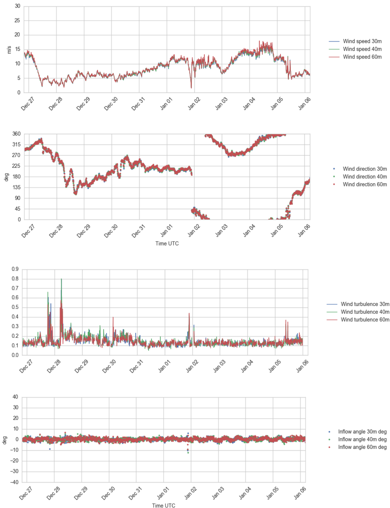
Figure 4.10 Plots of wind profile data, 30 – 60 m a.s.l., 26 Dec - 6 Jan 2017.
