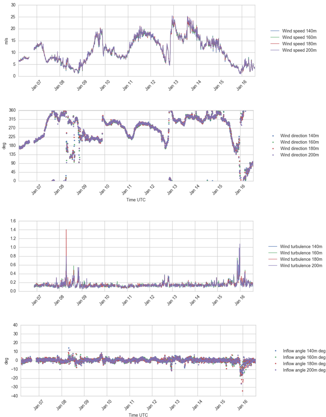
Figure 4.15 Plots of wind profile data, 140 – 200 m a.s.l., 6 - 16 Jan 2017.
