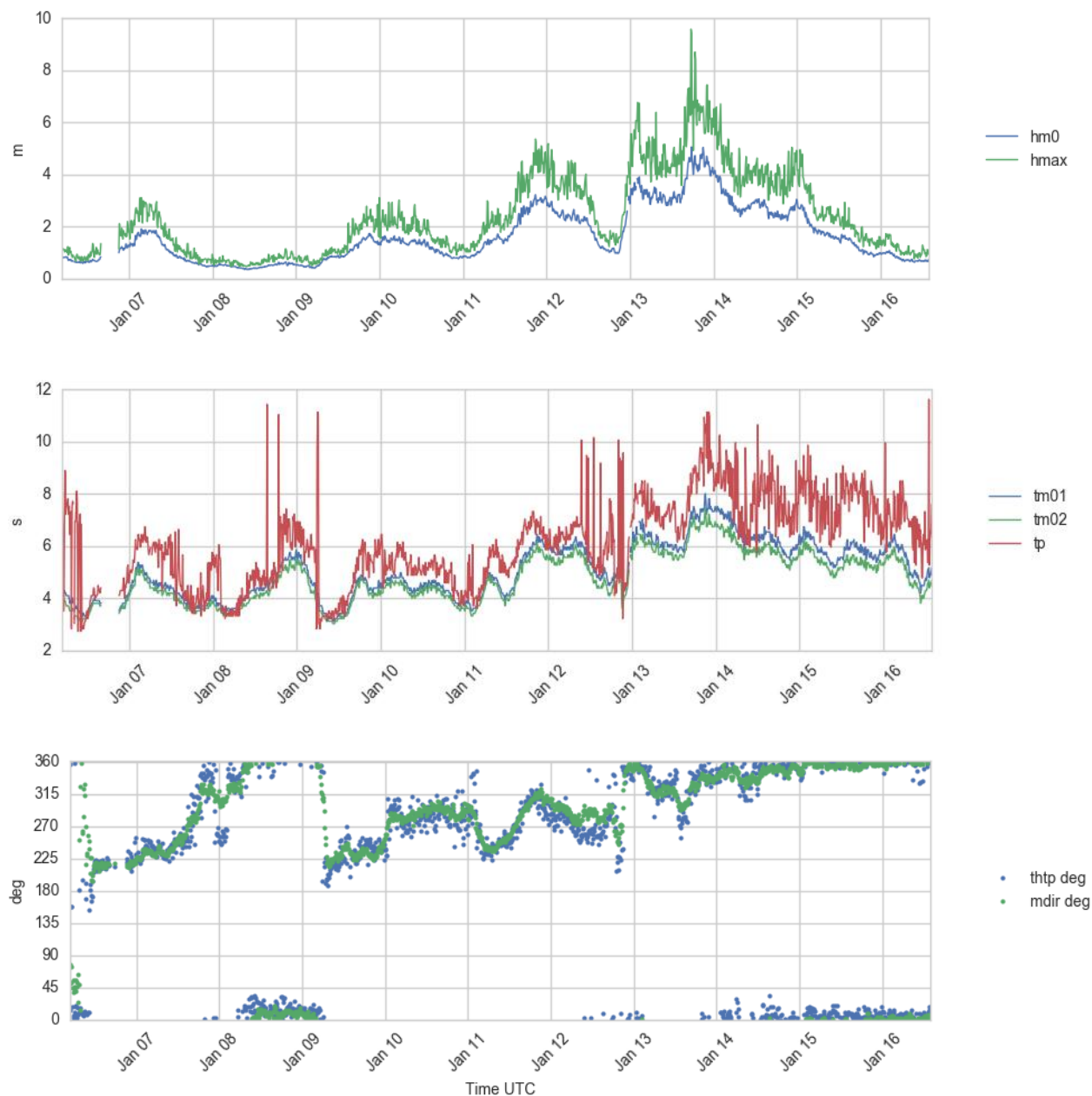
Figure 4.5 Time series plots of wave height (Hm0 and Hmax) (upper panel), wave period (Tm01, Tm02 and Tp) (second panel), and wave direction (ThTp and Mdir) (lower panel), 6 - 16 Jan 2017.
