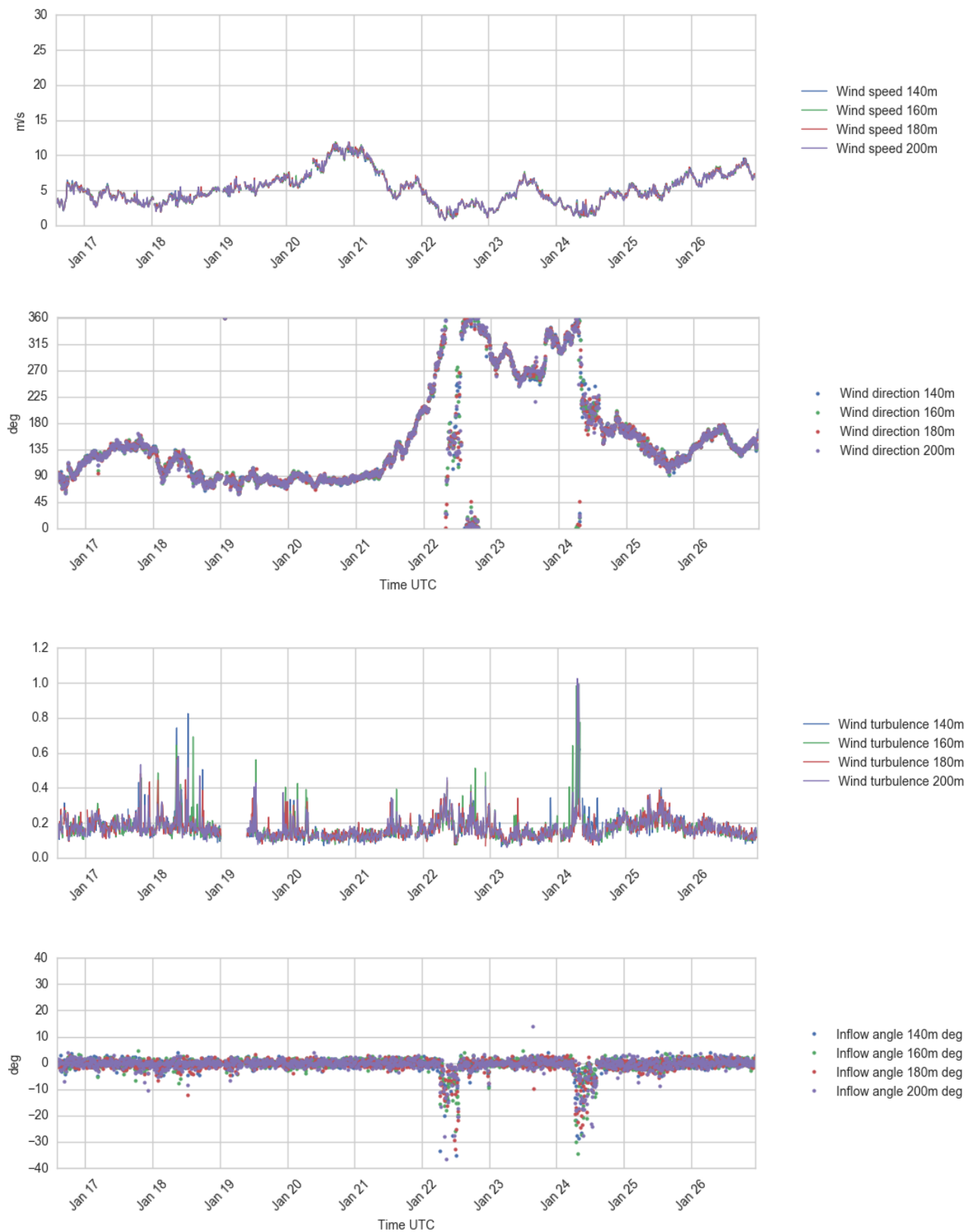
Figure 4.18 Plots of wind profile data, 140 – 200 m a.s.l., 16 - 26 Jan 2017.
