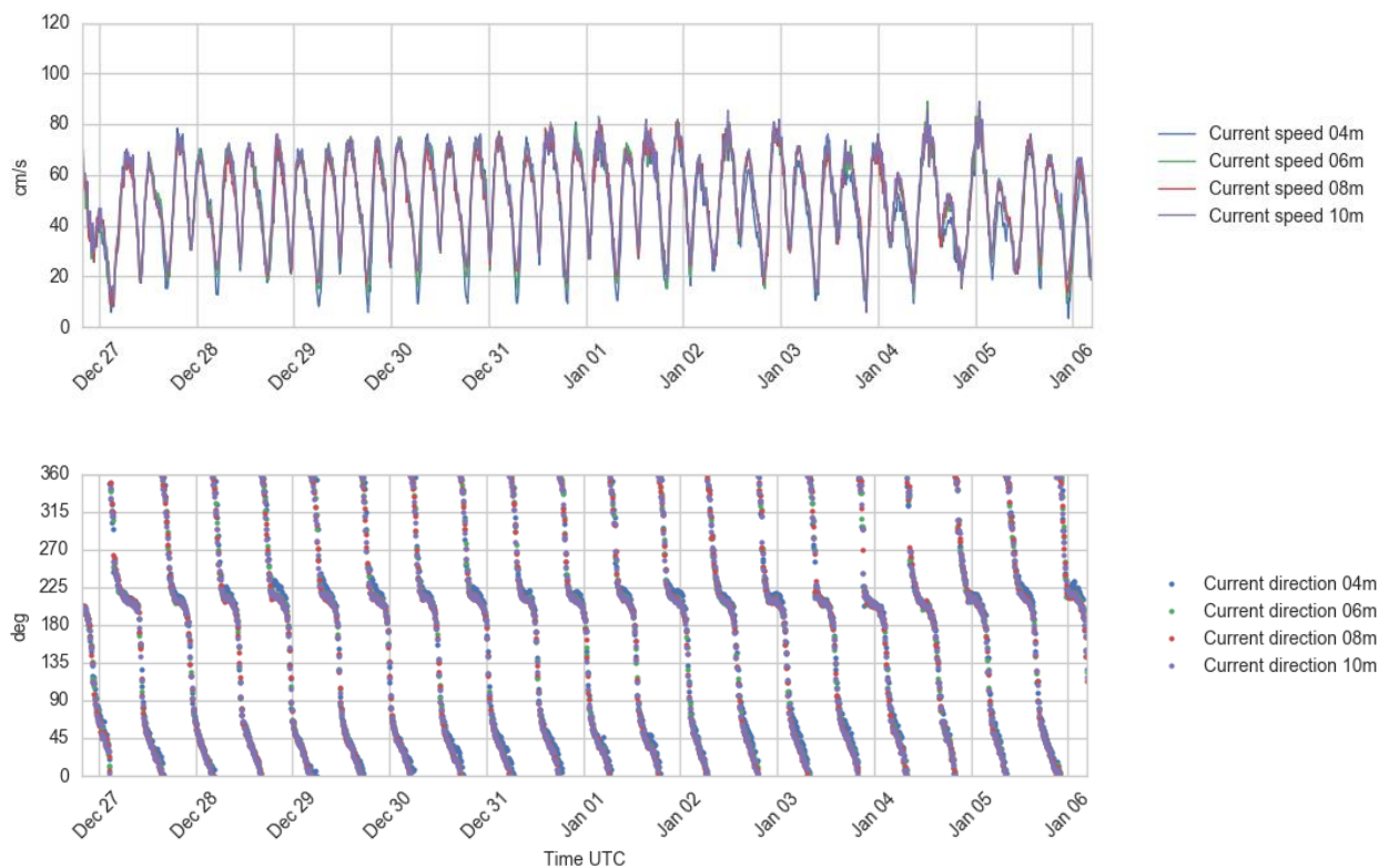
Figure 4.19 Time series plots of current speed (upper) and direction (lower panel), 4 - 10 m depth, 26 Dec - 6 Jan 2017.
