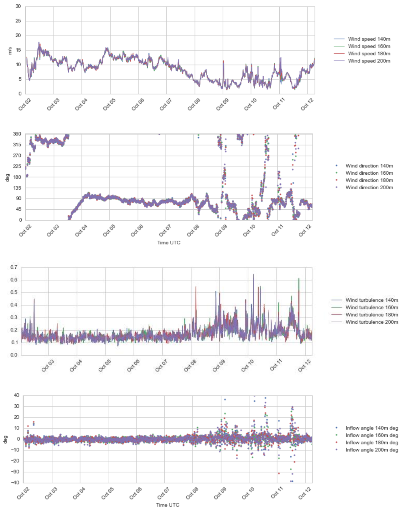
Figure 4.15 Plots of wind profile data, 140 – 200 m a.s.l., 2 - 12 Oct 2016.
