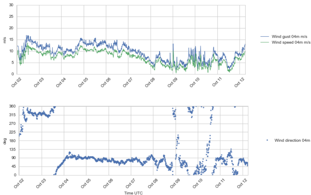
Figure 4.8 Plots of wind speed and gust (upper), and wind direction (lower) at 4 m a.s.l., 2 - 12 Oct 2016.
