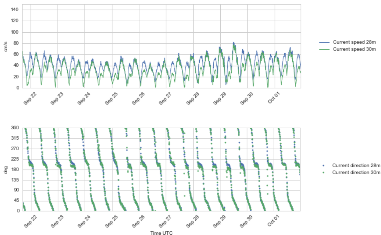
Figure 4.22 Time series plots of current speed (upper) and direction (lower panel), 28 - 30 m depth, 21 Sept - 1 Oct 2016.
