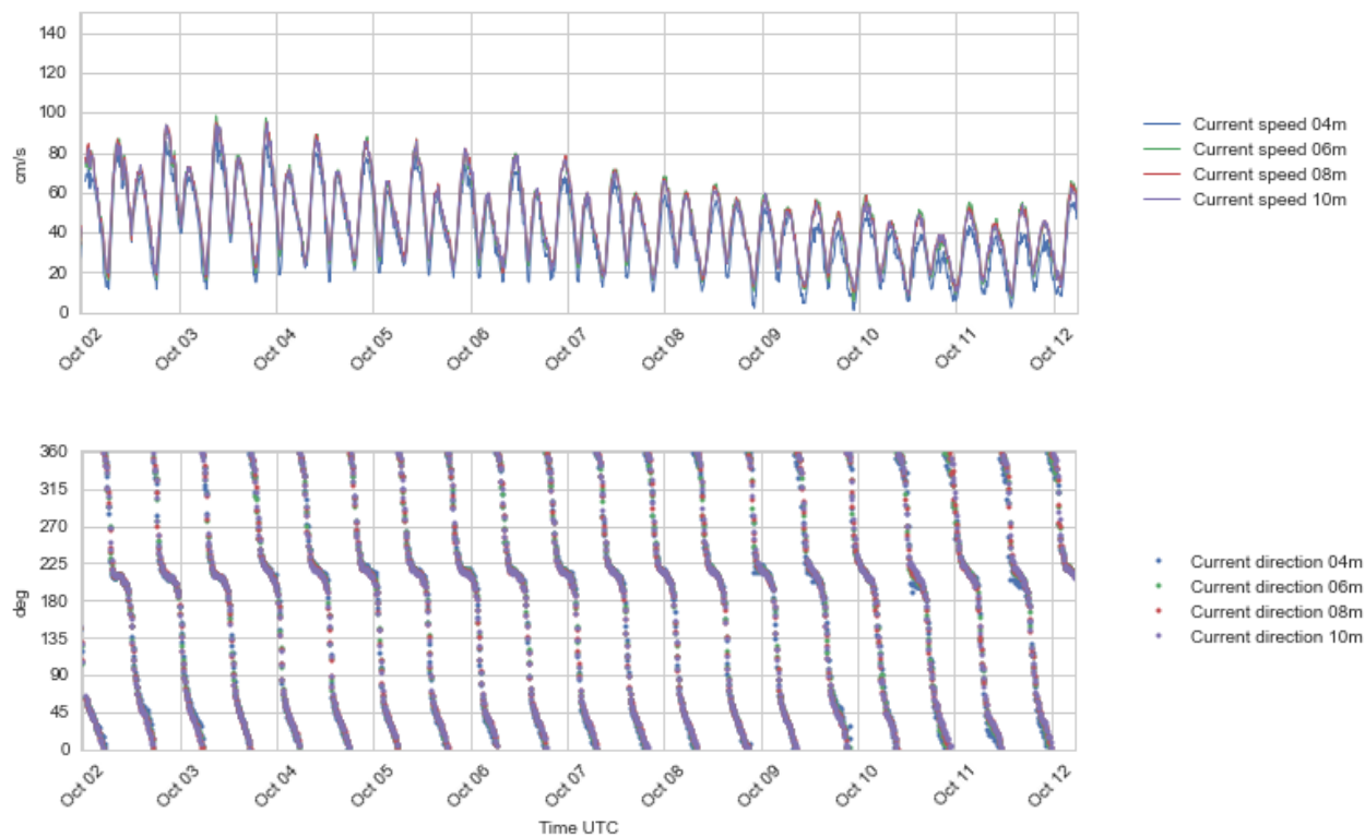
Figure 4.23 Time series plots of current speed (upper) and direction (lower panel), 4 - 10 m depth, 2 - 12 Oct 2016.
