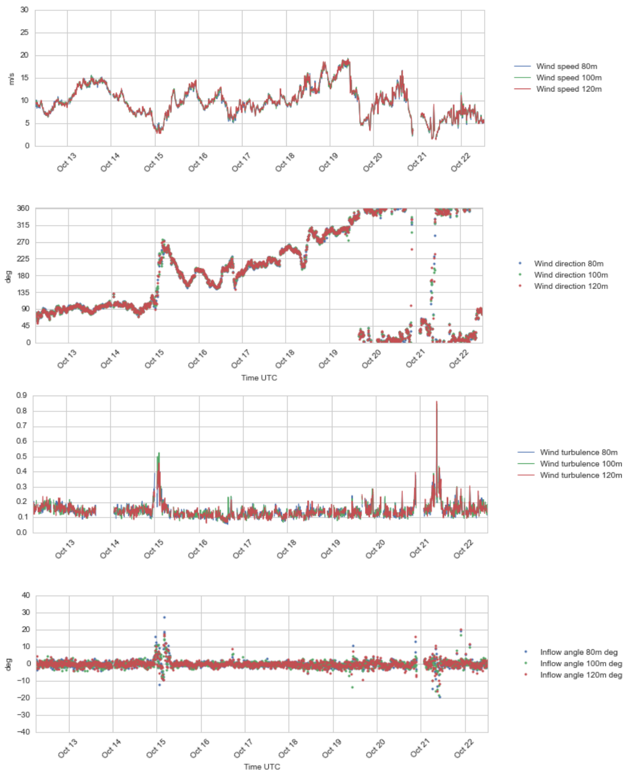
Figure 4.17 Plots of wind profile data, 80 – 120 m a.s.l., 12 - 22 Oct 2016.
