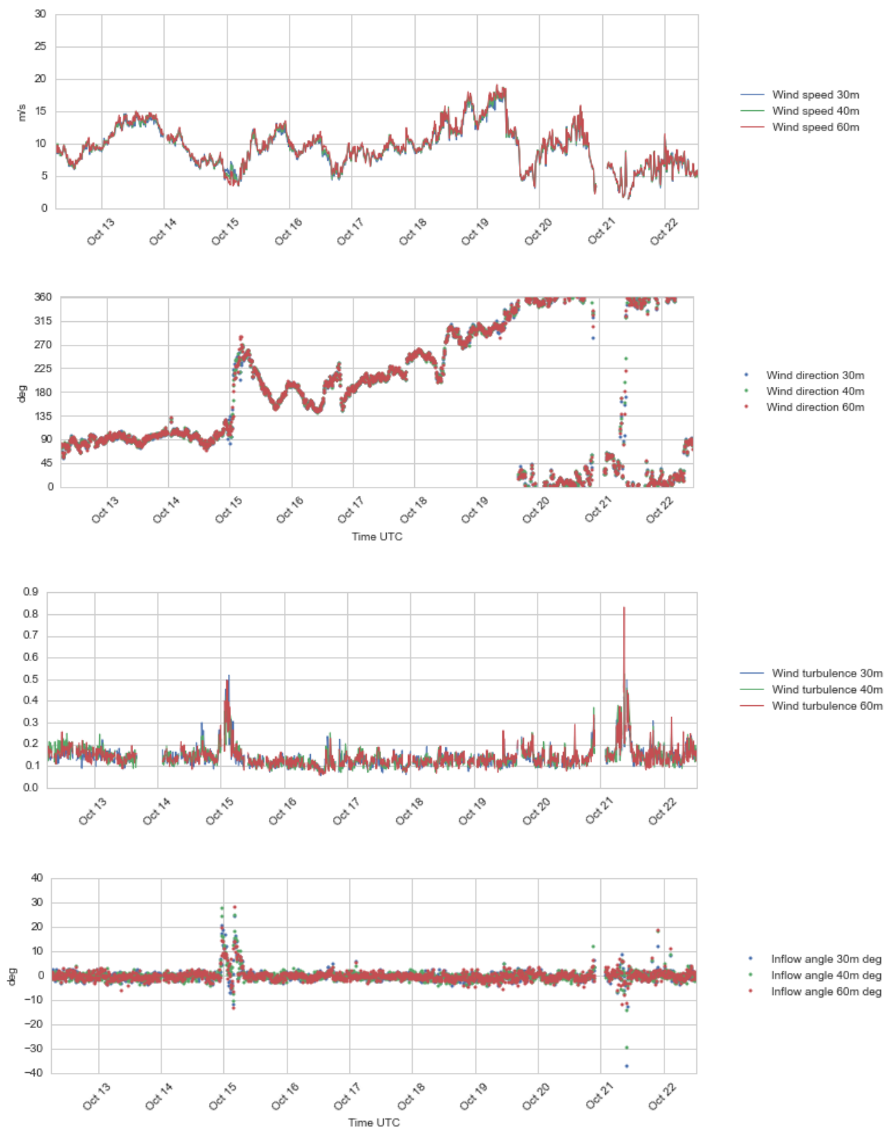
Figure 4.16 Plots of wind profile data, 30 – 60 m a.s.l., 12 - 22 Oct 2016.
