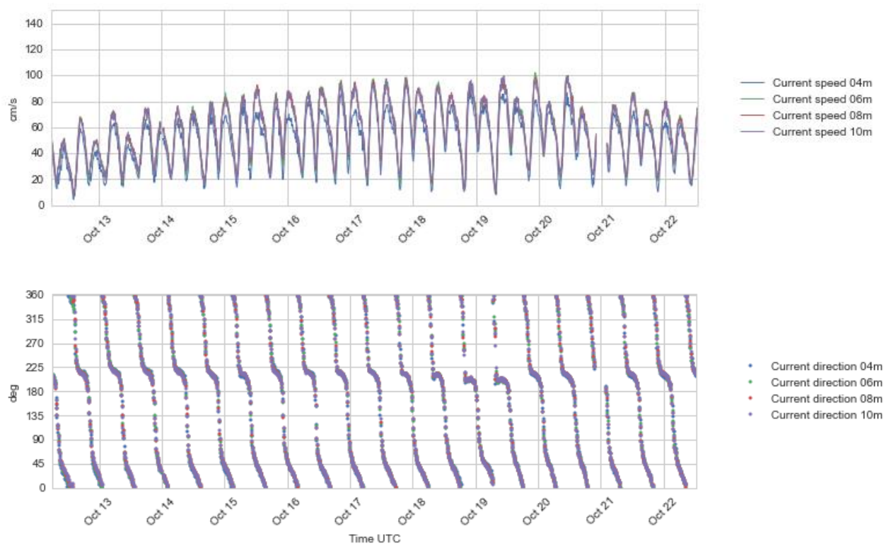
Figure 4.27 Time series plots of current speed (upper) and direction (lower panel), 4 - 10 m depth, 12 - 22 Oct 2016.
