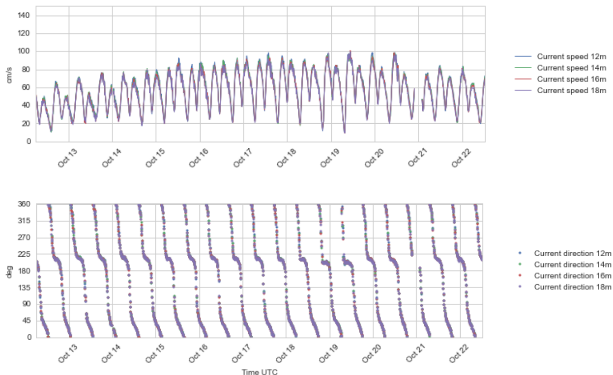
Figure 4.28 Time series plots of current speed (upper) and direction (lower panel), 12 - 18 m depth, 12 - 22 Oct 2016.
