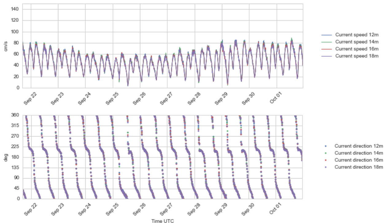
Figure 4.20 Time series plots of current speed (upper) and direction (lower panel), 12 - 18 m depth, 21 Sept - 1 Oct 2016.
