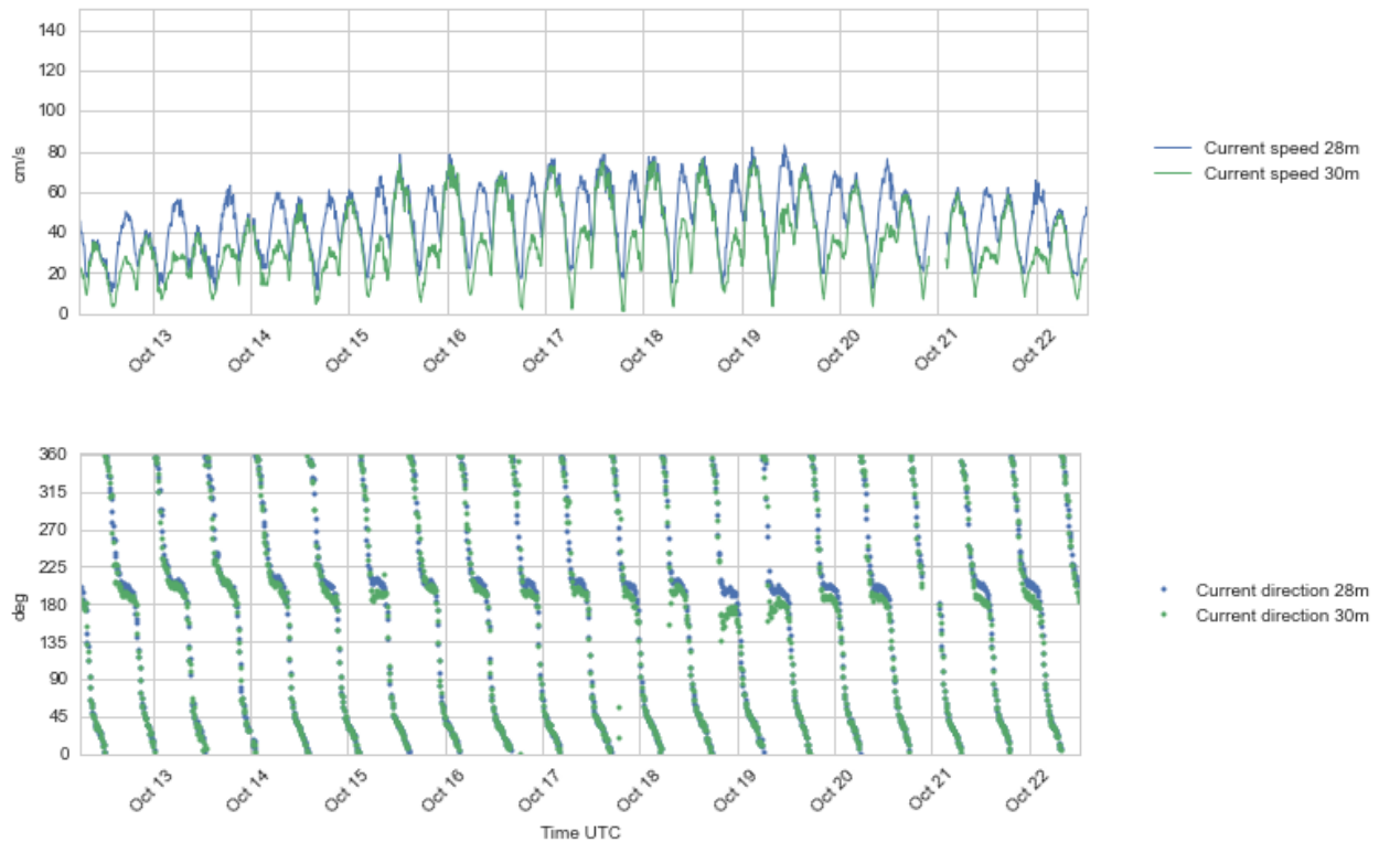
Figure 4.30 Time series plots of current speed (upper) and direction (lower panel), 28 - 30 m depth, 12 - 22 Oct 2016.
