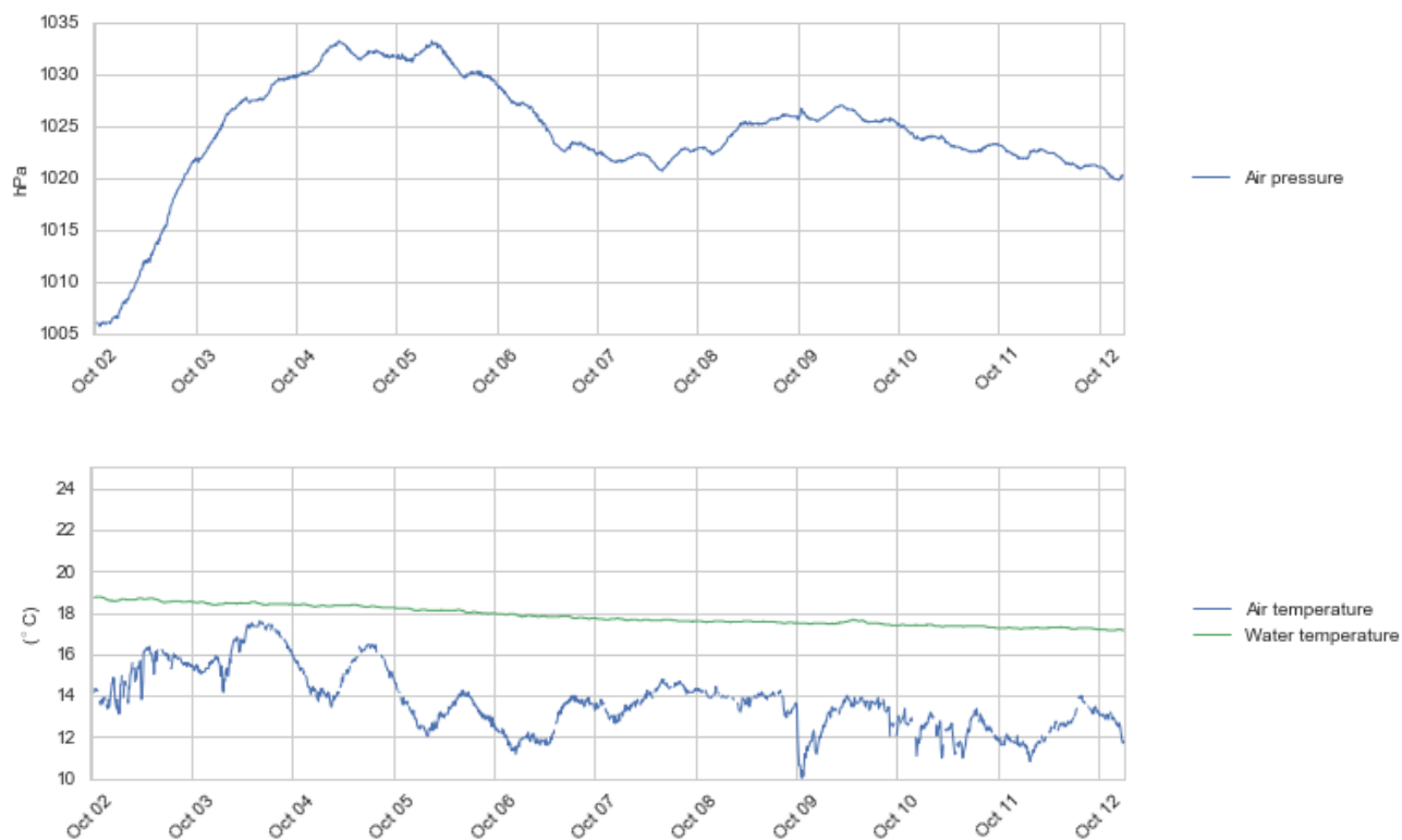
Figure 4.2 Time series plots of air pressure (upper panel), air and water temperature (lower panel), 2 - 12 Oct 2016.
