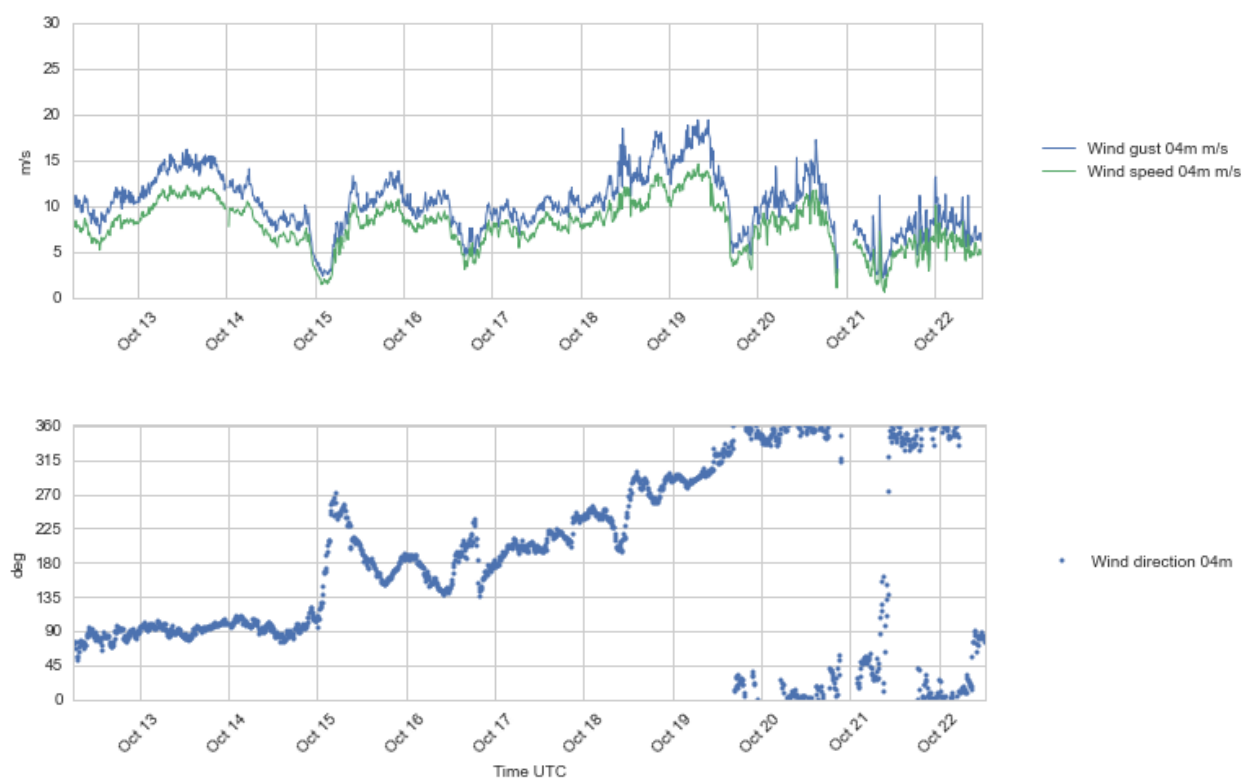
Figure 4.9 Plots of wind speed and gust (upper), and wind direction (lower) at 4 m a.s.l., 12 - 22 Oct 2016.
