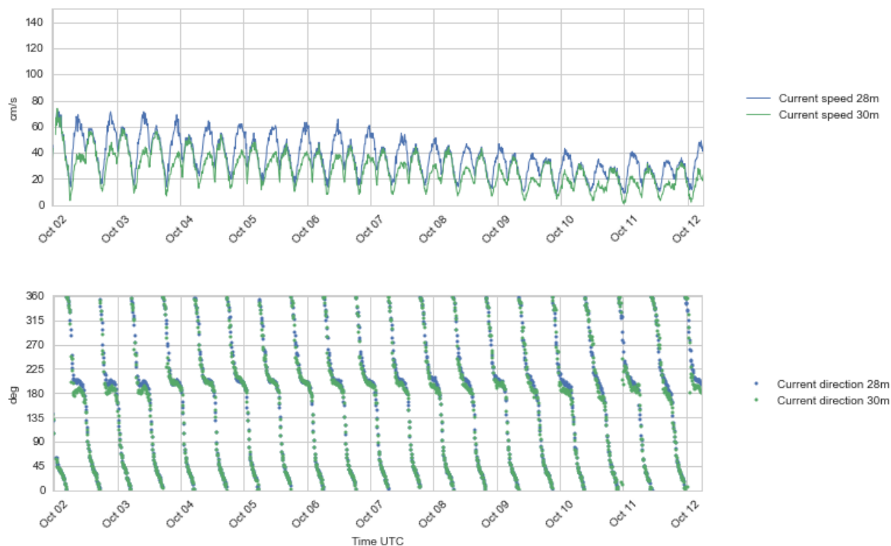
Figure 4.26 Time series plots of current speed (upper) and direction (lower panel), 28 – 30 m depth, 2 - 12 Oct 2016.
