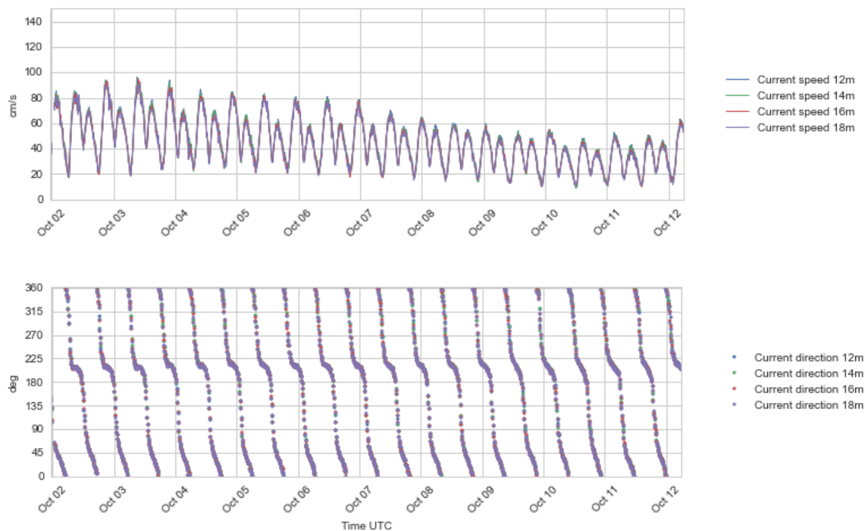
Figure 4.24 Time series plots of current speed (upper) and direction (lower panel), 12 -18 m depth, 2 - 12 Oct 2016.
