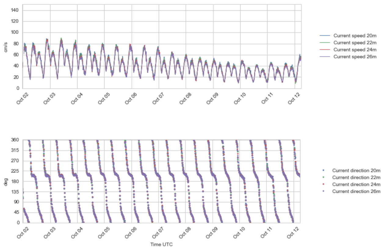
Figure 4.25 Time series plots of current speed (upper) and direction (lower panel), 20 – 26 m depth, 2 - 12 Oct 2016.
