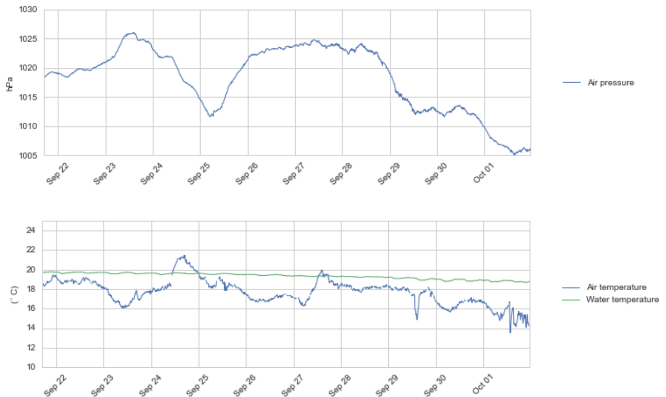
Figure 4.1 Time series plots of air pressure (upper panel), air and water temperature (lower panel), 21 Sept - 1 Oct 2016.
