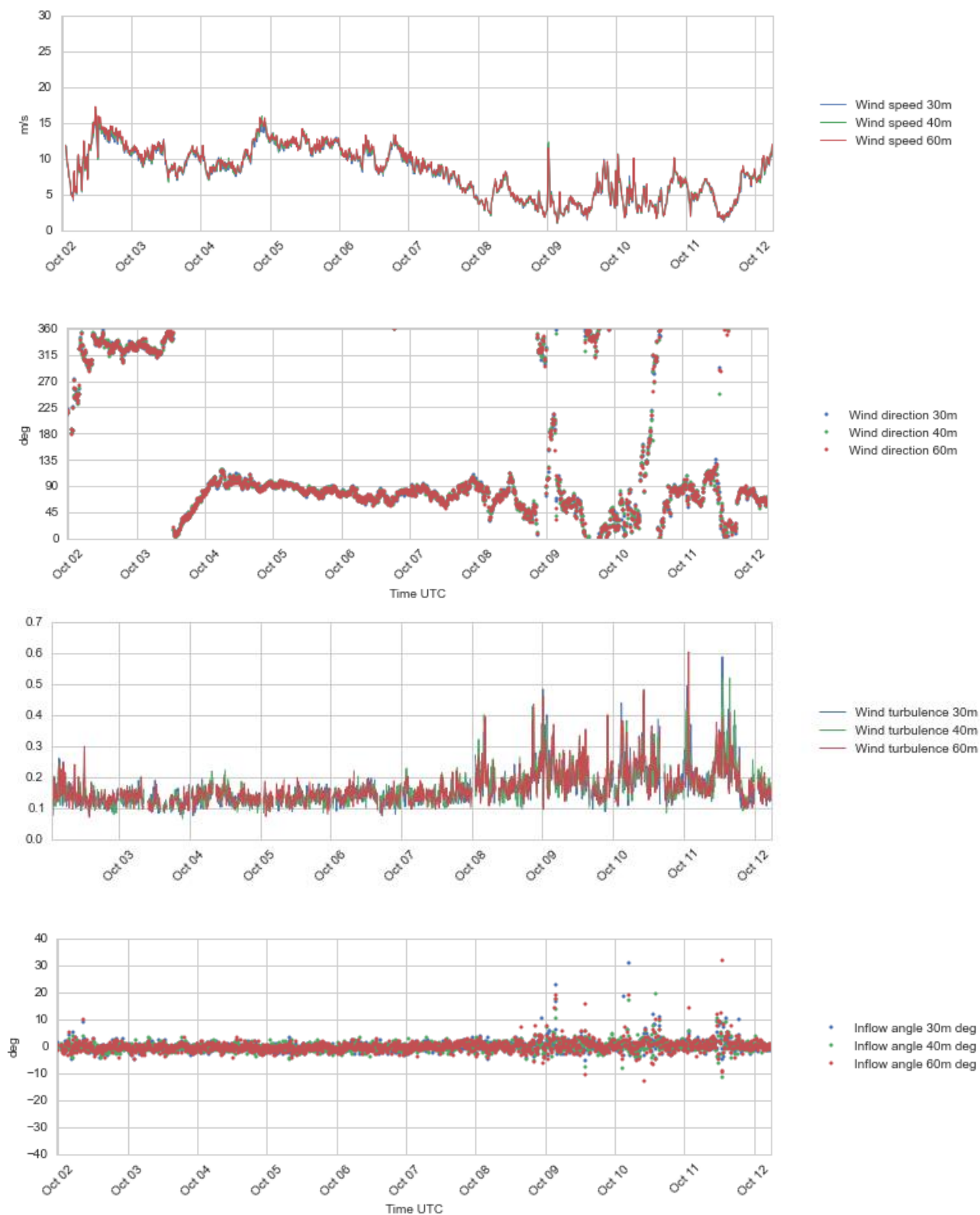
Figure 4.13 Plots of wind profile data, 30 – 60 m a.s.l., 2 - 12 Oct 2016.
