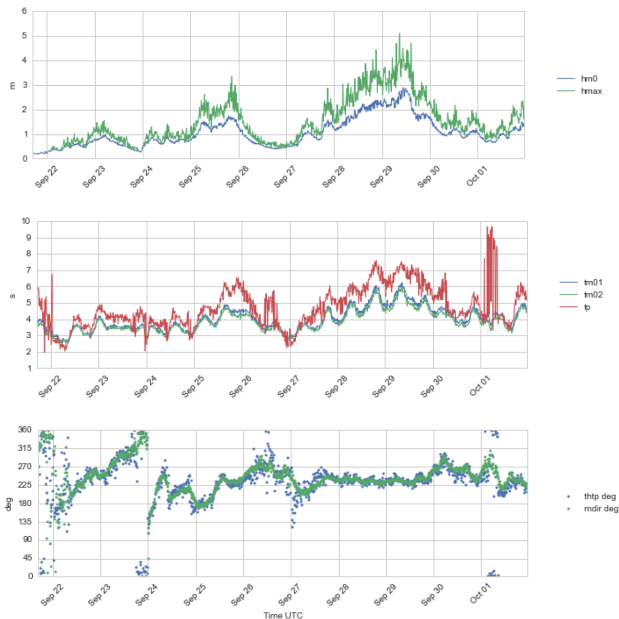
Figure 4.4 Time series plots of wave height ( Hm0 and Hmax ) (upper panel), wave period ( Tm01 , Tm02 and Tp ) (second panel), and wave direction ( ThTp and Mdir ) (lower panel), 21 Sept - 1 Oct 2016.
