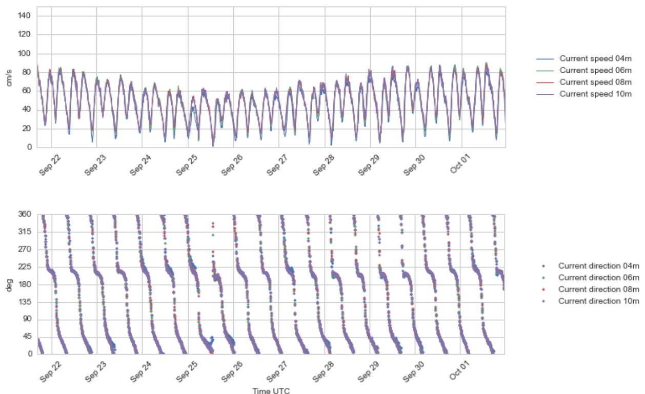
Figure 4.19 Time series plots of current speed (upper) and direction (lower panel), 4 - 10 m depth, 21 Sept - 1 Oct 2016.
