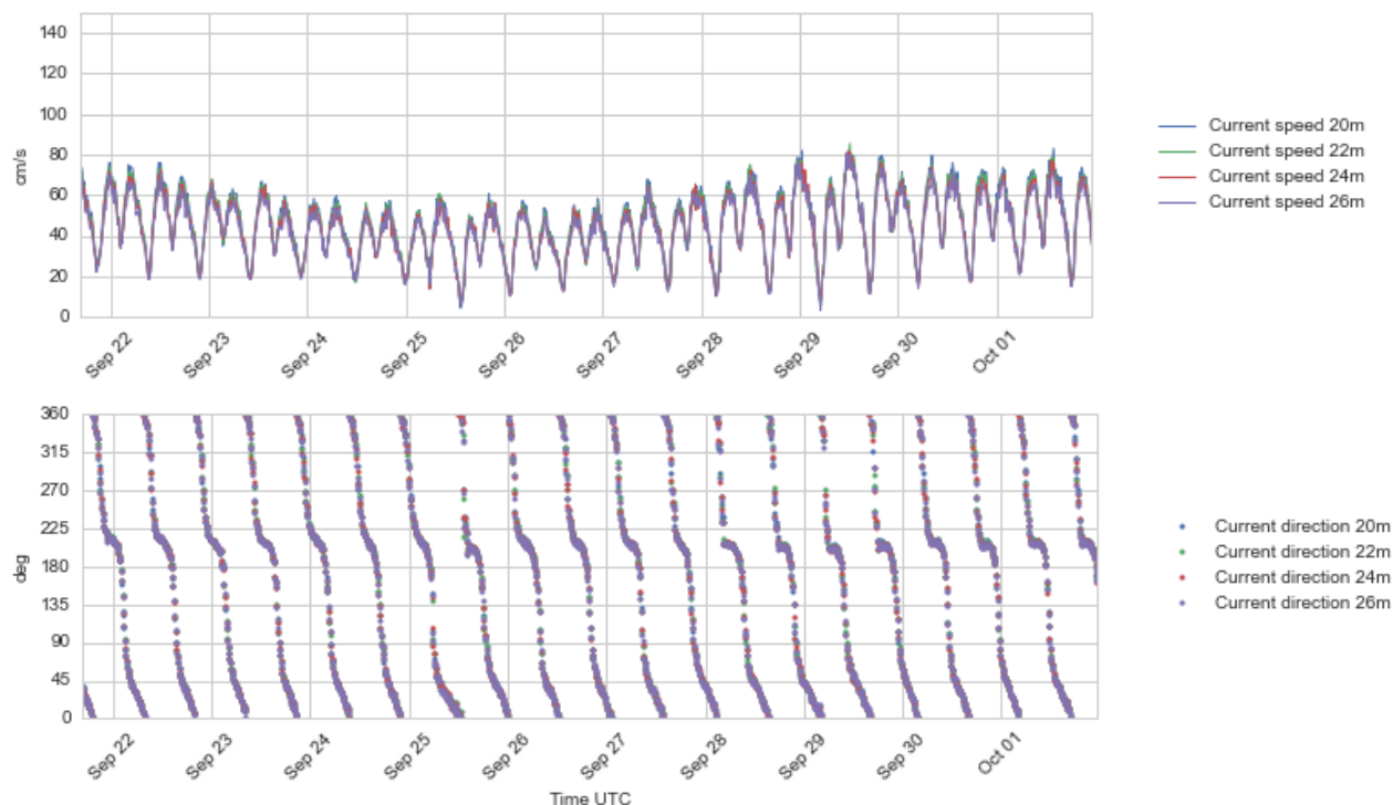
Figure 4.21 Time series plots of current speed (upper) and direction (lower panel), 20 - 26 m depth, 21 Sept - 1 Oct 2016.
