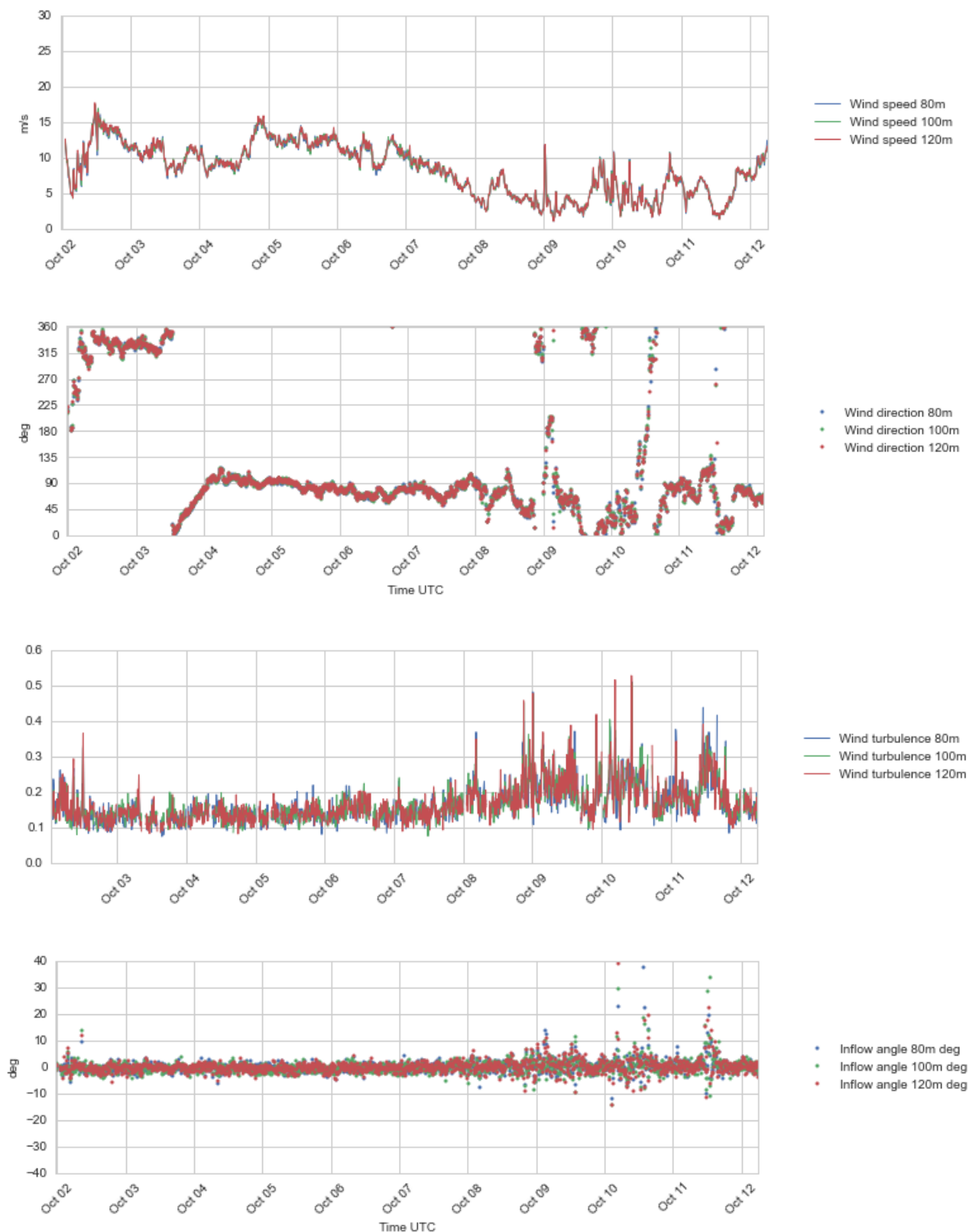
Figure 4.14 Plots of wind profile data, 80 – 120 m a.s.l., 2 - 12 Oct 2016.
