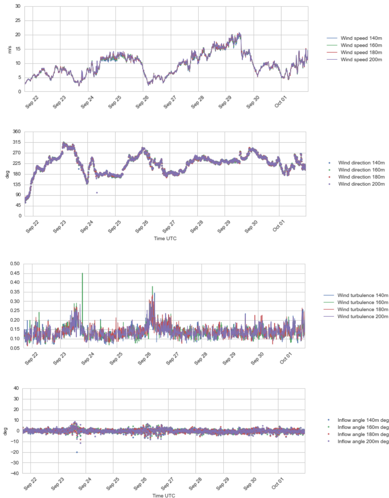
Figure 4.12 Plots of wind profile data, 140 – 200 m a.s.l., 21 Sept - 1 Oct 2016.
