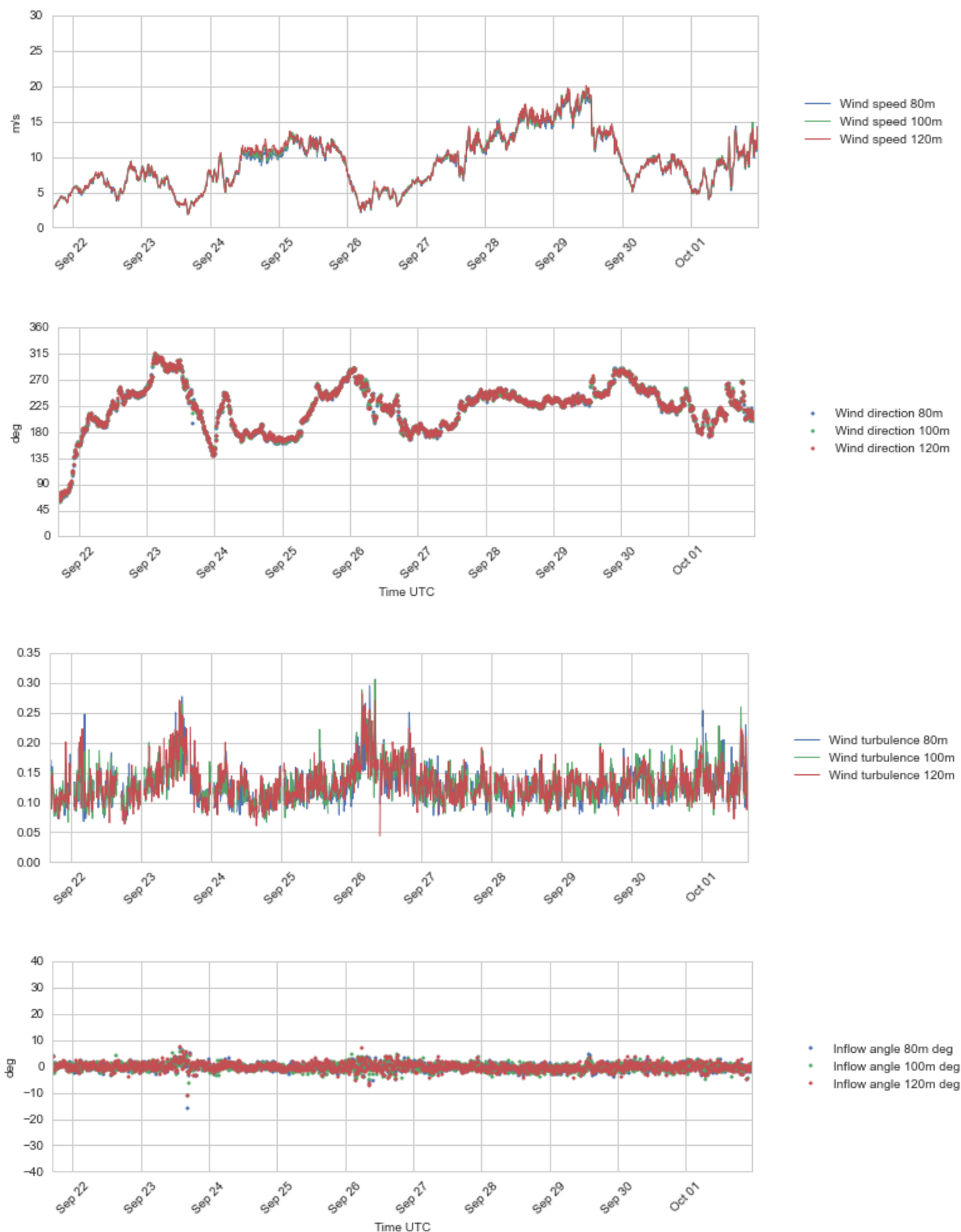
Figure 4.11 Plots of wind profile data, 80 – 120 m a.s.l., 21 Sept - 1 Oct 2016.
