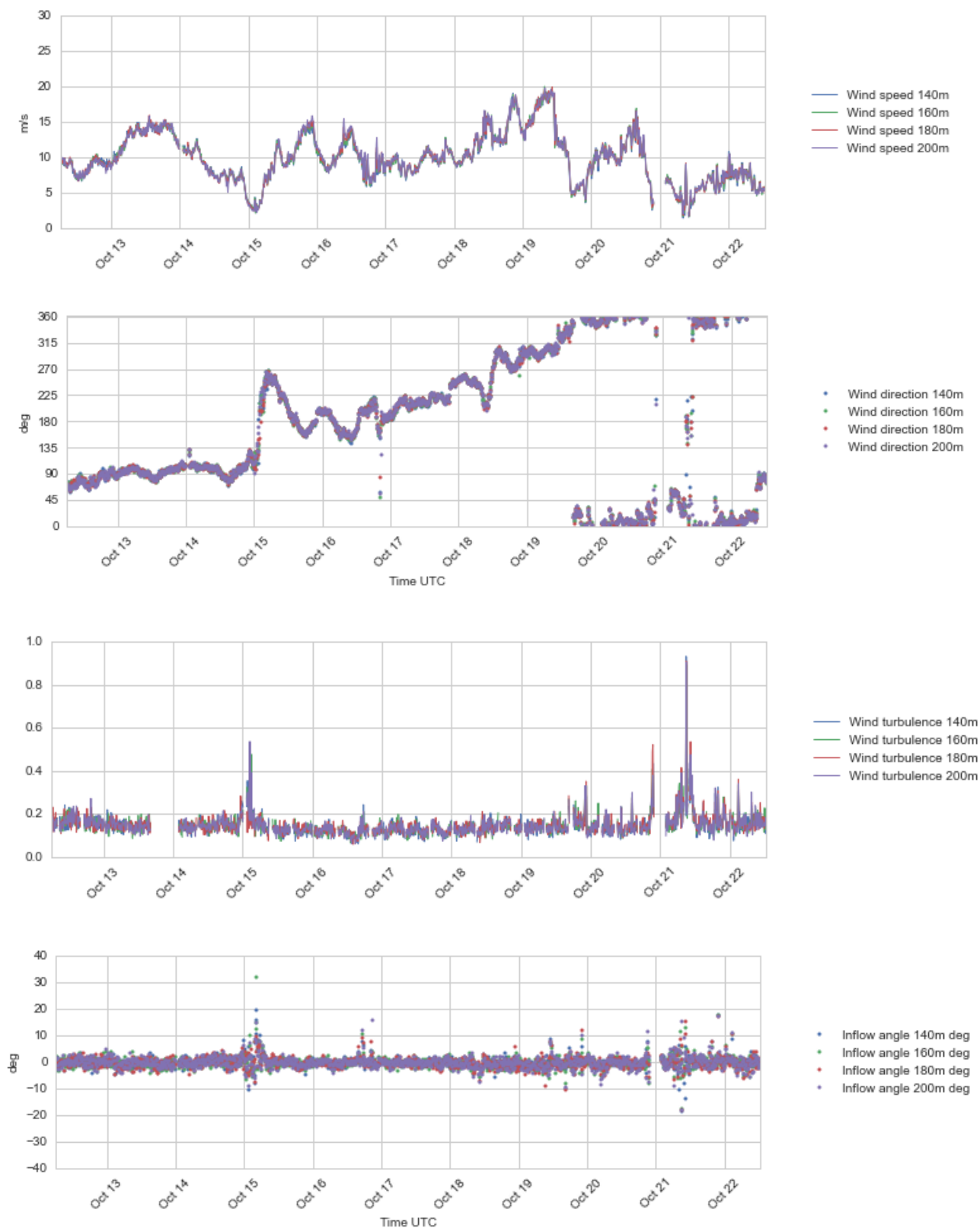
Figure 4.18 Plots of wind profile data, 140 – 200 m a.s.l., 12 - 22 Oct 2016.
