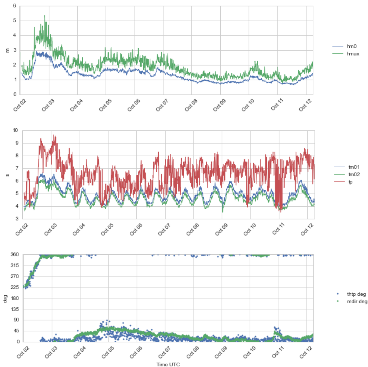
Figure 4.5 Time series plots of wave height (Hm0 and Hmax) (upper panel), wave period (Tm01, Tm02 and Tp) (second panel), and wave direction (ThTp and Mdir) (lower panel), 2 - 12 Oct 2016.
