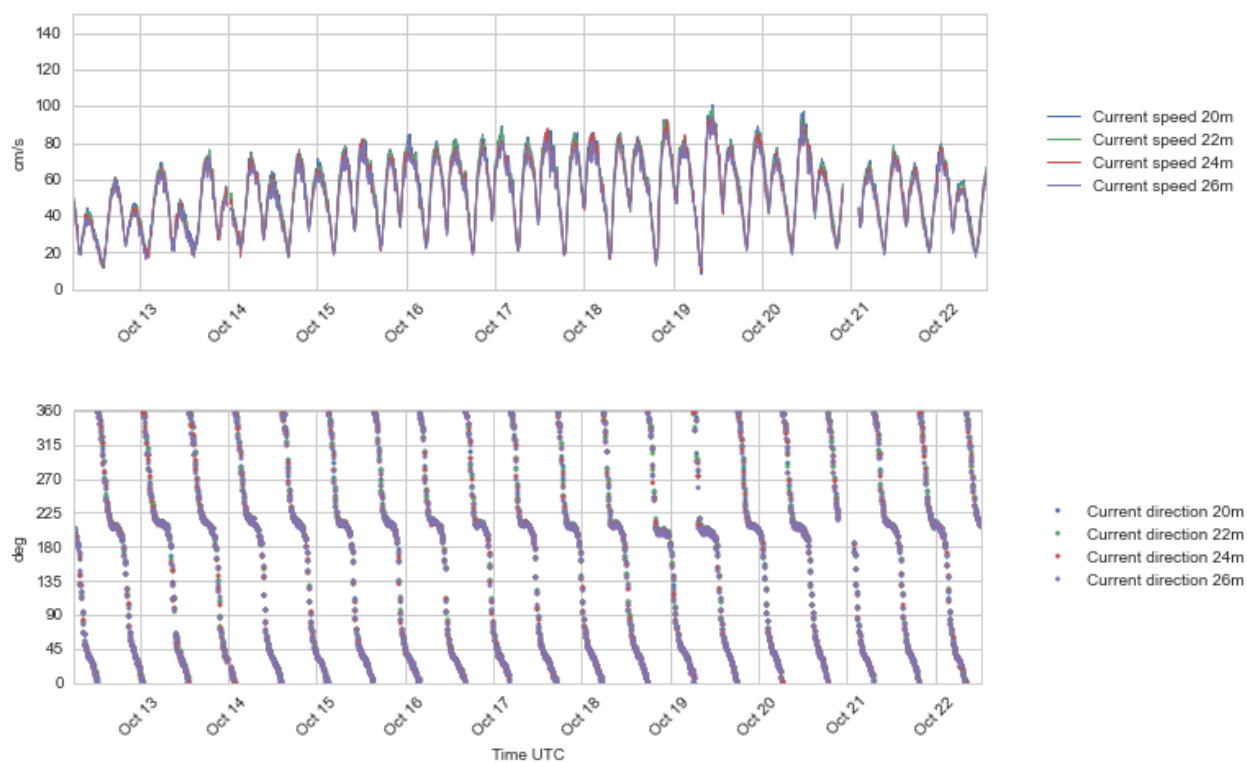
Figure 4.29 Time series plots of current speed (upper) and direction (lower panel), 20 - 26 m depth, 12 - 22 Oct 2016.
