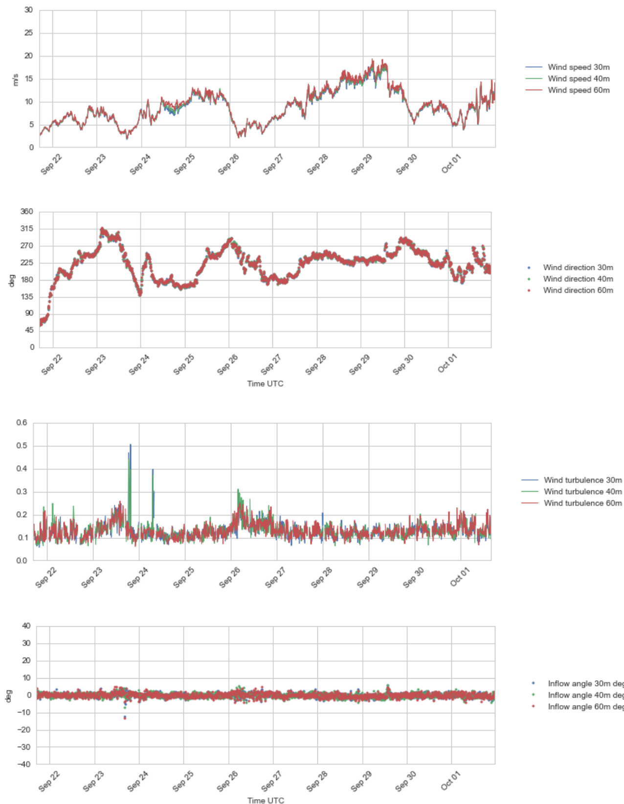
Figure 4.10 Plots of wind profile data, 30 – 60 m a.s.l., 21 Sept - 1 Oct 2016.
