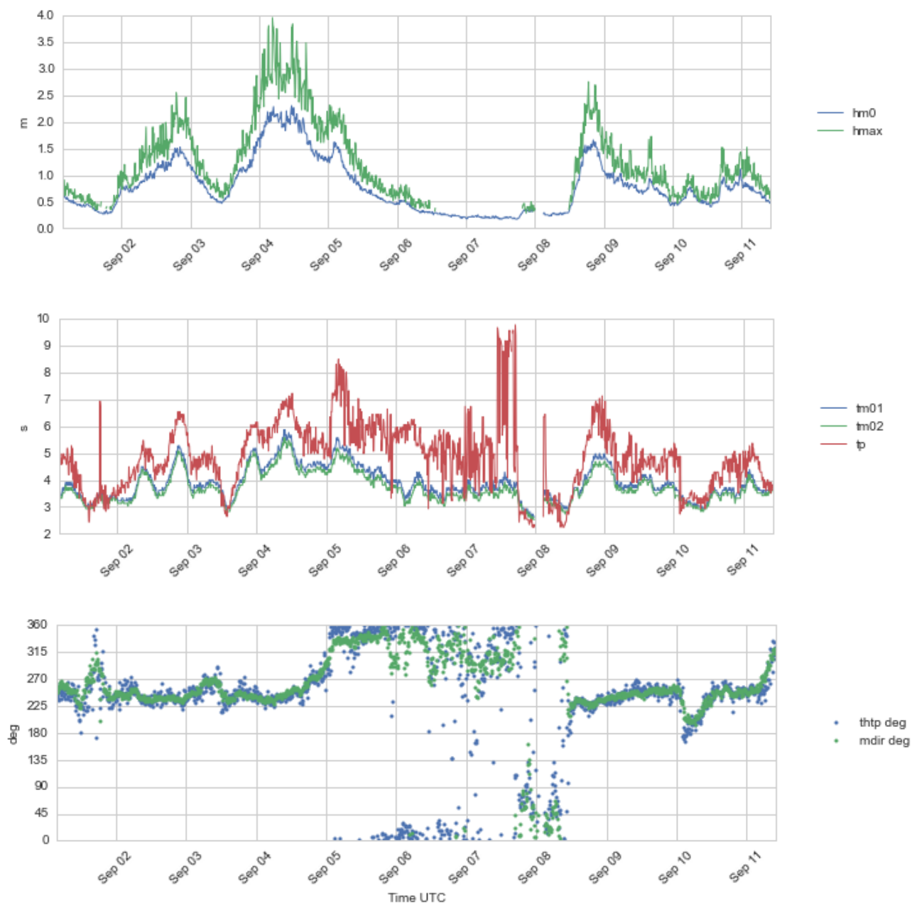
Figure 4.5 Time series plots of wave height (Hm0 and Hmax) (upper panel), wave period (Tm01, Tm02 and Tp) (second panel), and wave direction (ThTp and Mdir) (lower panel), 1 – 11 Sept 2016.
