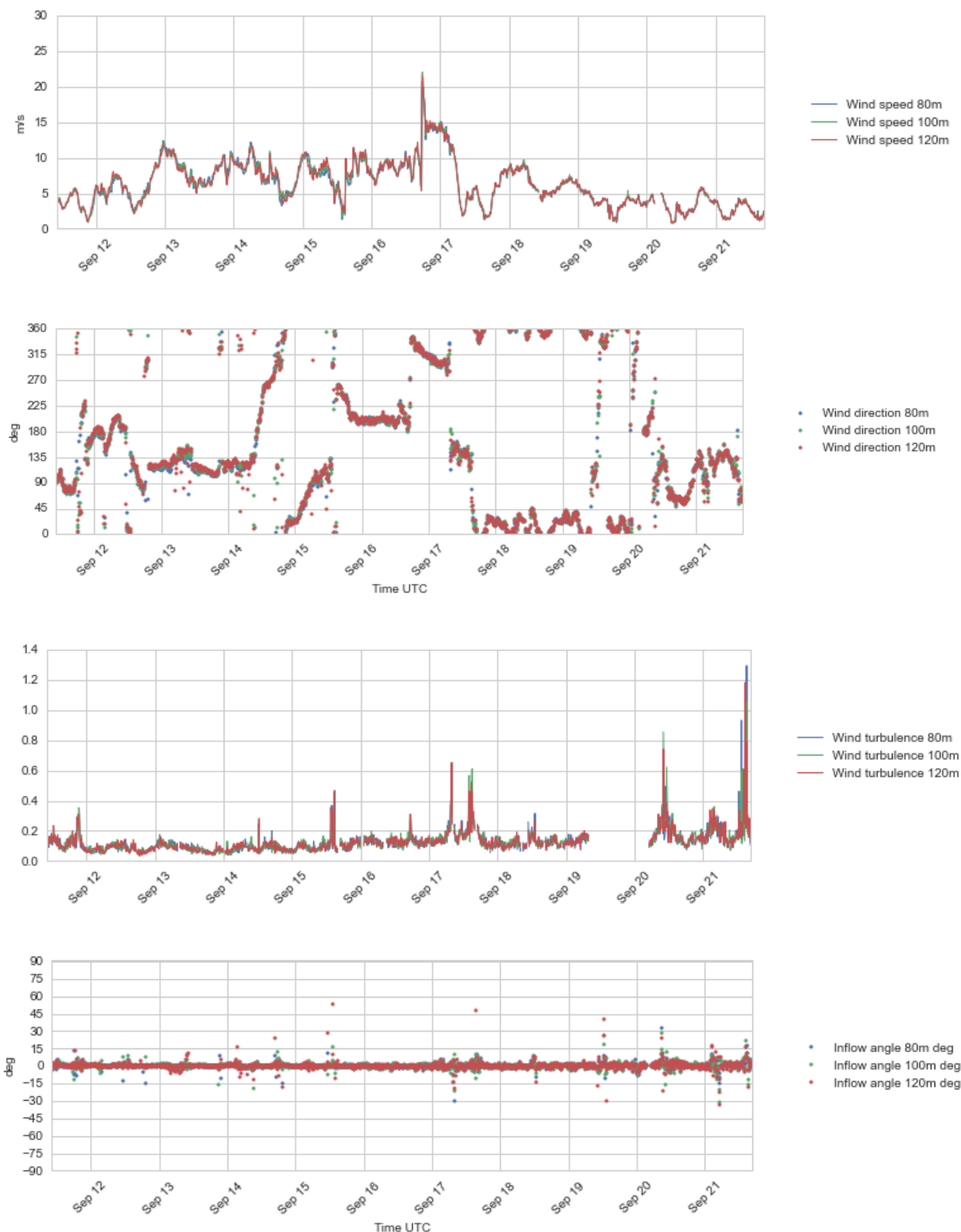
Figure 4.17 Plots of wind profile data, 80 – 120 m a.s.l., 11 - 21 Sept 2016.
