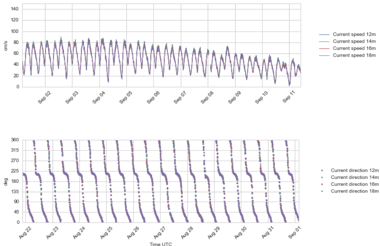
Figure 4.24 Time series plots of current speed (upper) and direction (lower panel), 12 -18 m depth, 1 – 11 Sept 2016.
