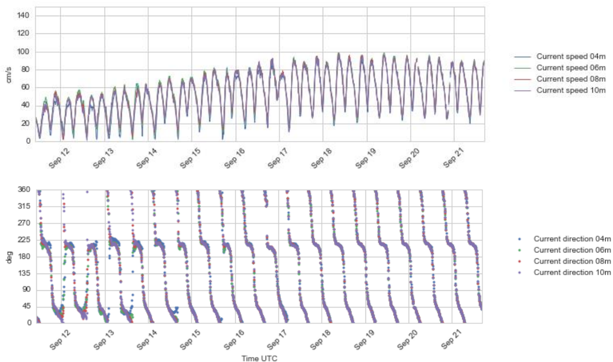
Figure 4.27 Time series plots of current speed (upper) and direction (lower panel), 4 - 10 m depth, 11 - 21 Sept 2016.
