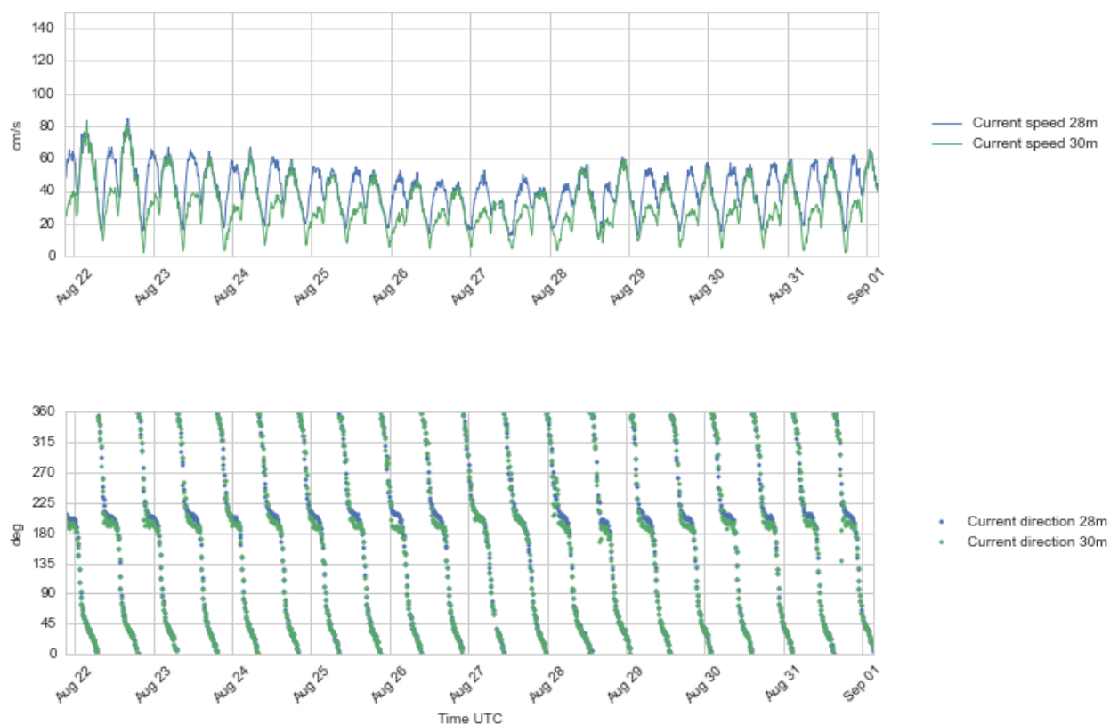
Figure 4.22 Time series plots of current speed (upper) and direction (lower panel), 28 - 30 m depth, 21 – 31 Aug 2016.
