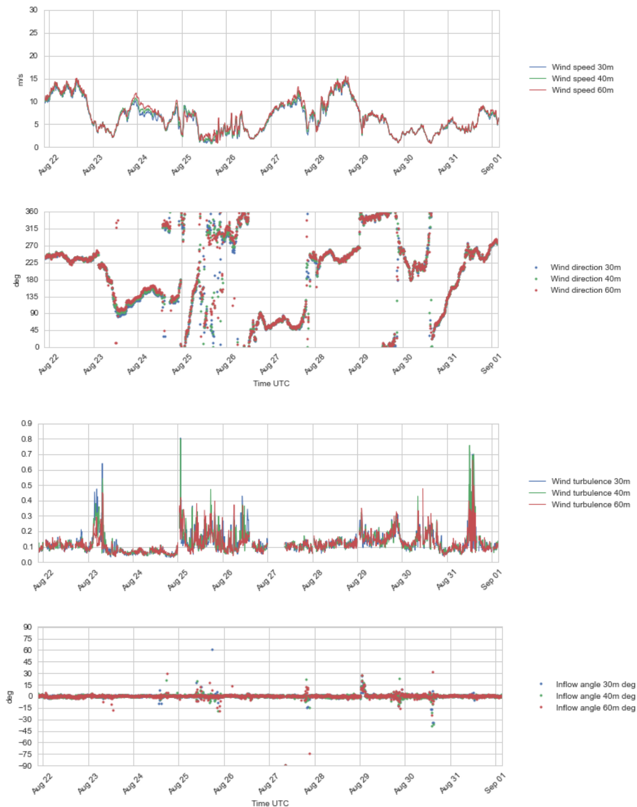
Figure 4.10 Plots of wind profile data, 30 – 60 m a.s.l., 21 – 31 Aug 2016.
