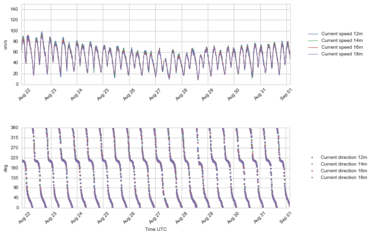
Figure 4.20 Time series plots of current speed (upper) and direction (lower panel), 12 - 18 m depth, 21 – 31 Aug 2016.
