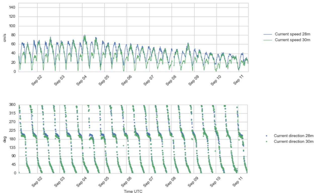
Figure 4.26 Time series plots of current speed (upper) and direction (lower panel), 28 – 30 m depth, 1 – 11 Sept 2016.
