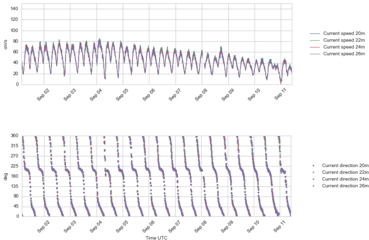
Figure 4.25 Time series plots of current speed (upper) and direction (lower panel), 20 – 26 m depth, 1 – 11 Sept 2016.
