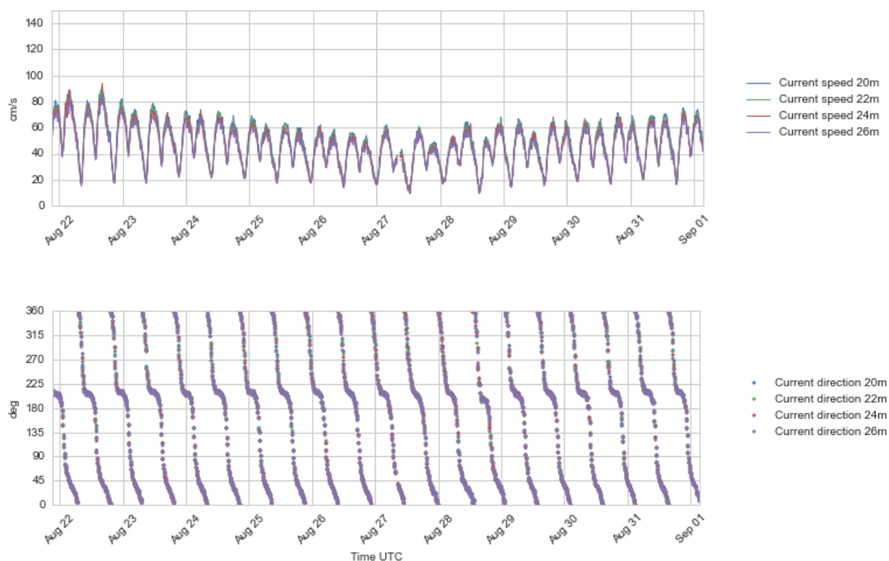
Figure 4.21 Time series plots of current speed (upper) and direction (lower panel), 20 - 26 m depth, 21 – 31 Aug 2016.
