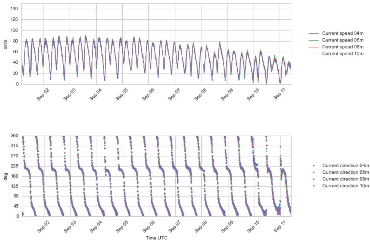
Figure 4.23 Time series plots of current speed (upper) and direction (lower panel), 4 - 10 m depth, 1 – 11 Sept 2016.
