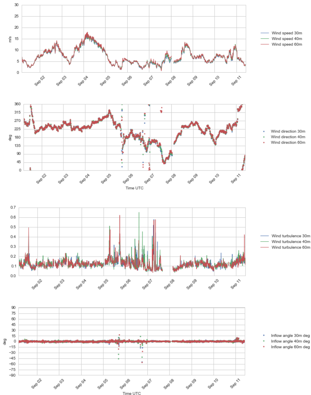
Figure 4.13 Plots of wind profile data, 30 – 60 m a.s.l., 1 – 11 Sept 2016.
