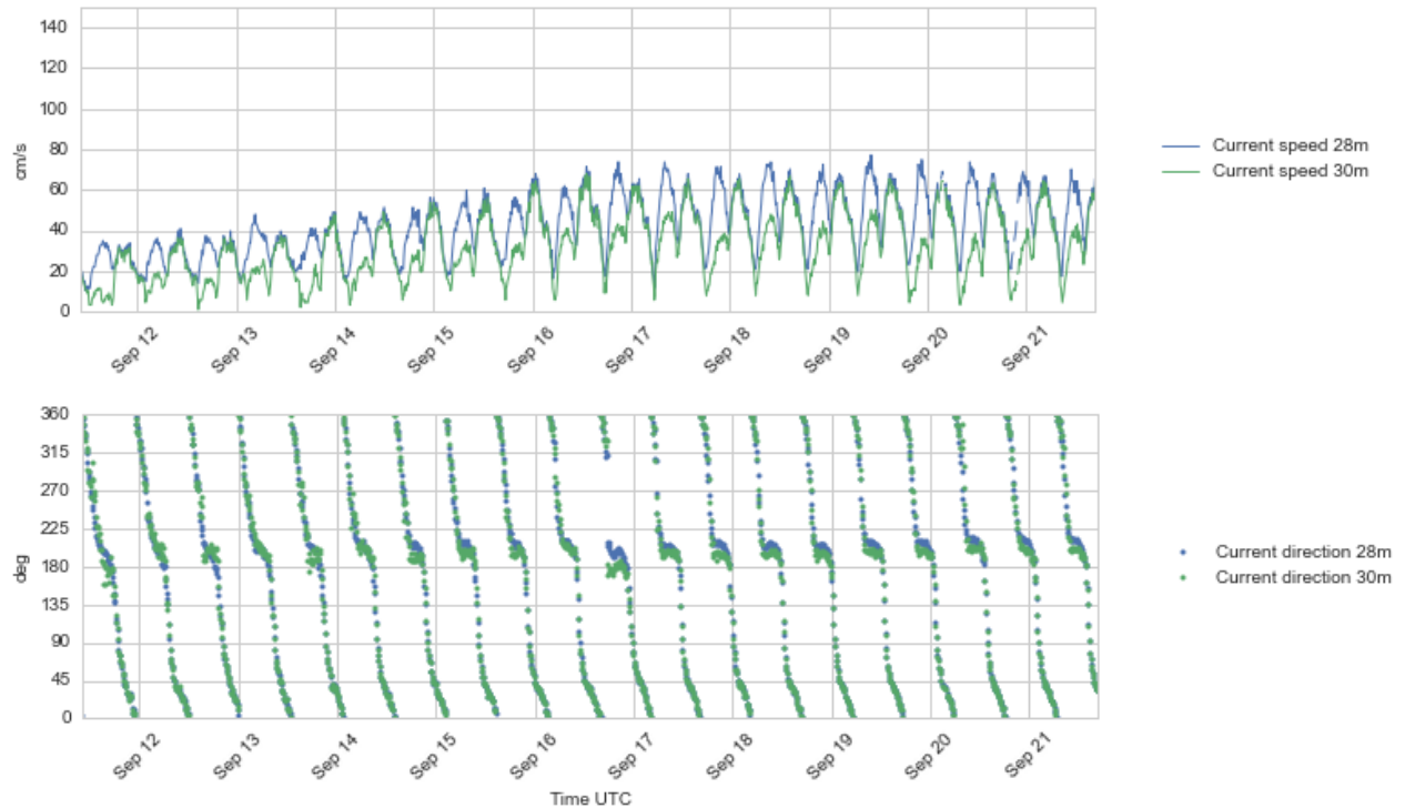
Figure 4.30 Time series plots of current speed (upper) and direction (lower panel), 28 - 30 m depth, 11 - 21 Sept 2016.
