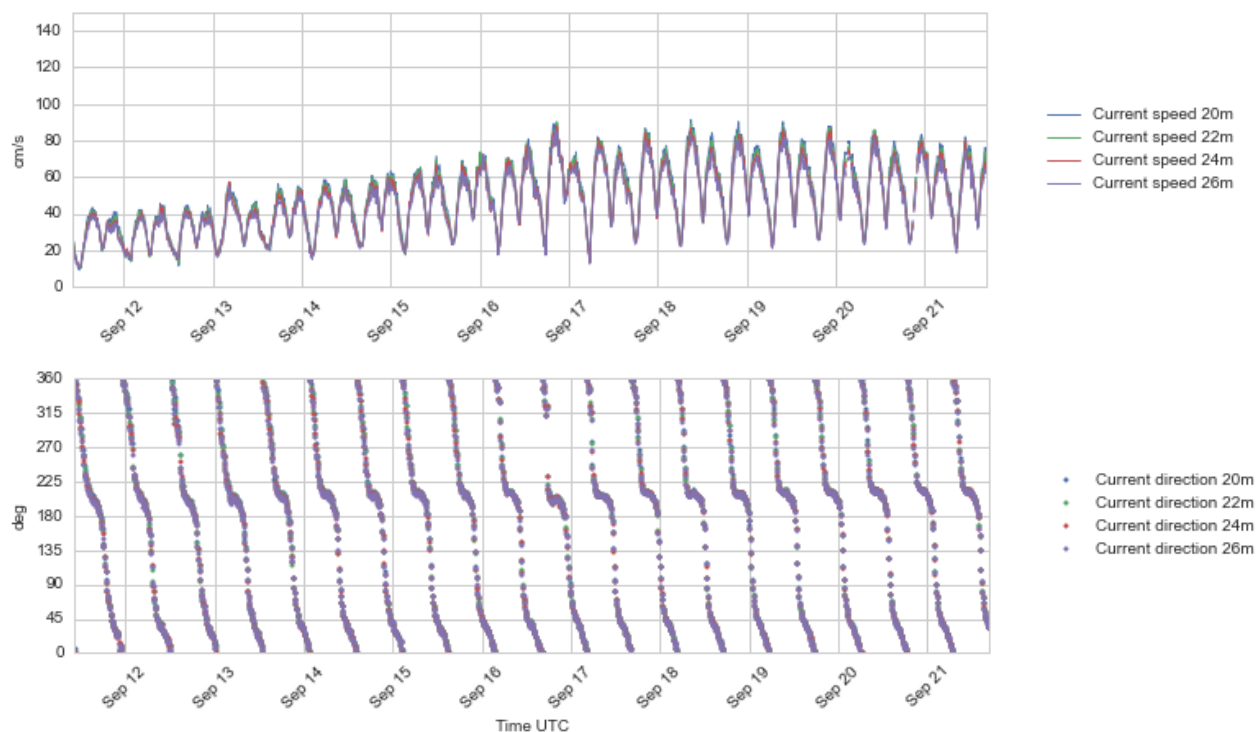
Figure 4.29 Time series plots of current speed (upper) and direction (lower panel), 20 - 26 m depth, 11 - 21 Sept 2016.
