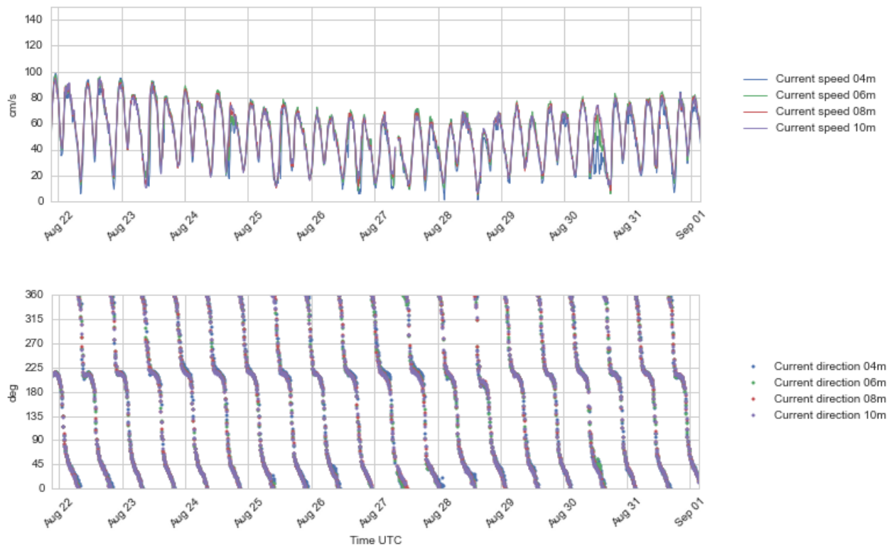
Figure 4.19 Time series plots of current speed (upper) and direction (lower panel), 4 - 10 m depth, 21 – 31 Aug 2016.
