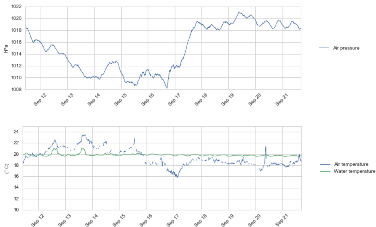
Figure 4.3 Time series plots of air pressure (upper panel), air and water temperature (lower panel), 11 - 21 Sept 2016.
