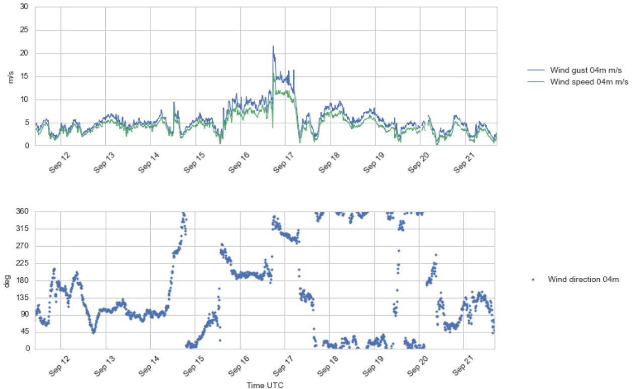
Figure 4.9 Plots of wind speed and gust (upper), and wind direction (lower) at 4 m a.s.l., 11 - 21 Sept 2016.
