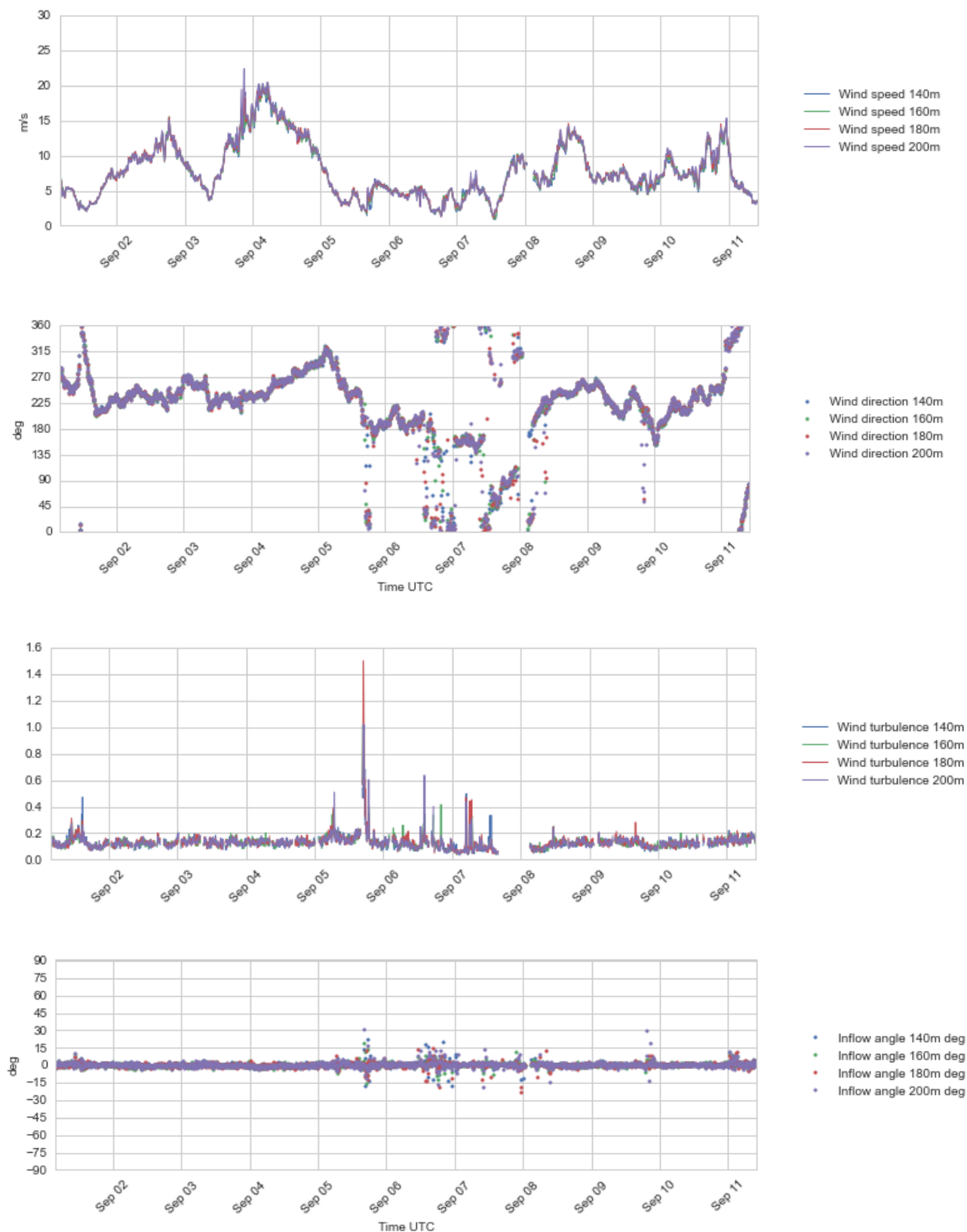
Figure 4.15 Plots of wind profile data, 140 – 200 m a.s.l., 1 – 11 Sept 2016.
