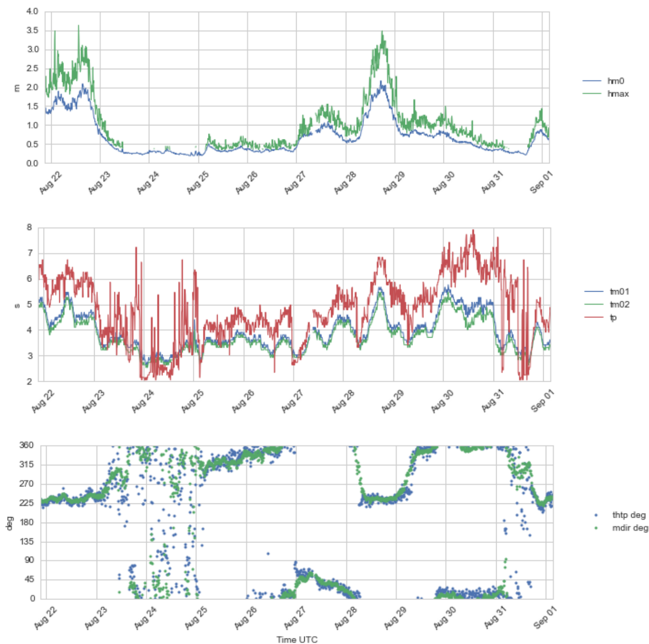
Figure 4.4 Time series plots of wave height (Hm0 and Hmax) (upper panel), wave period (Tm01, Tm02 and Tp) (second panel), and wave direction (ThTp and Mdir) (lower panel), 21 - 31 Aug 2016.
