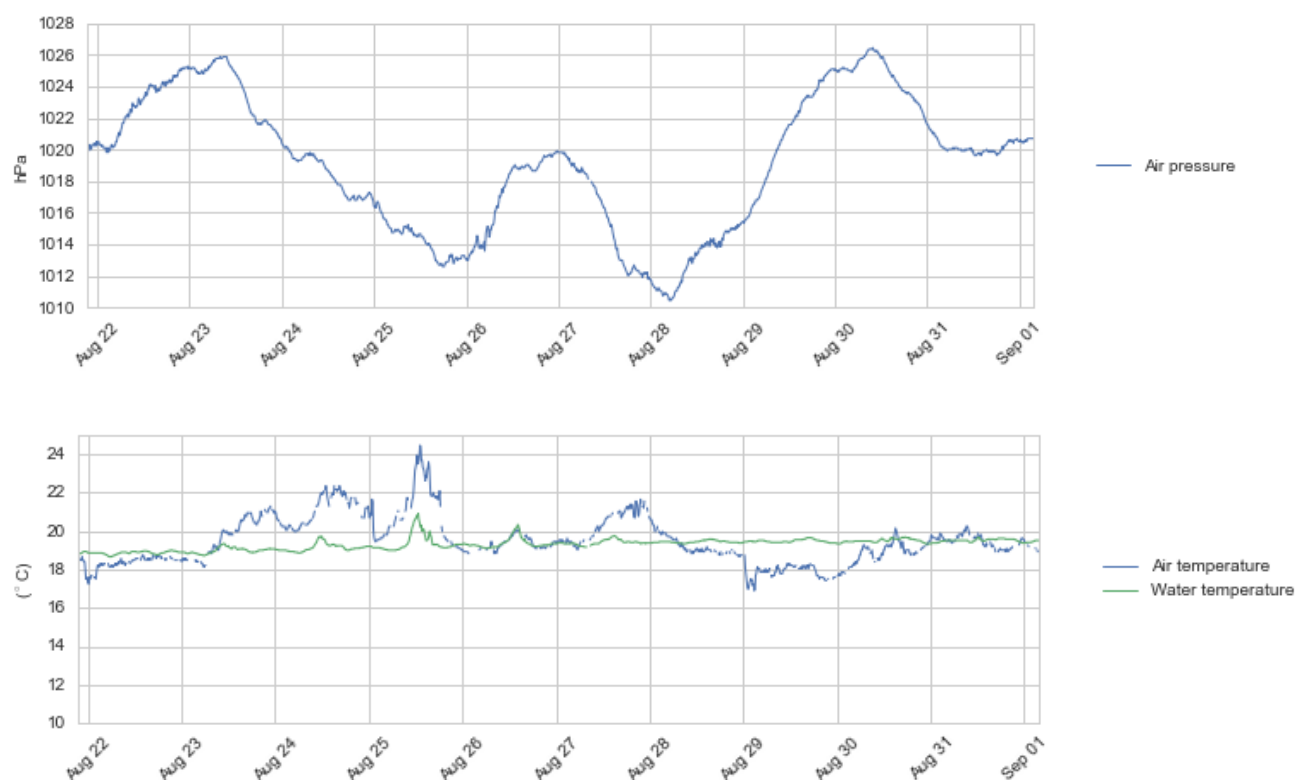
Figure 4.1 Time series plots of air pressure (upper panel), air and water temperature (lower panel), 21 - 31 August 2016.
