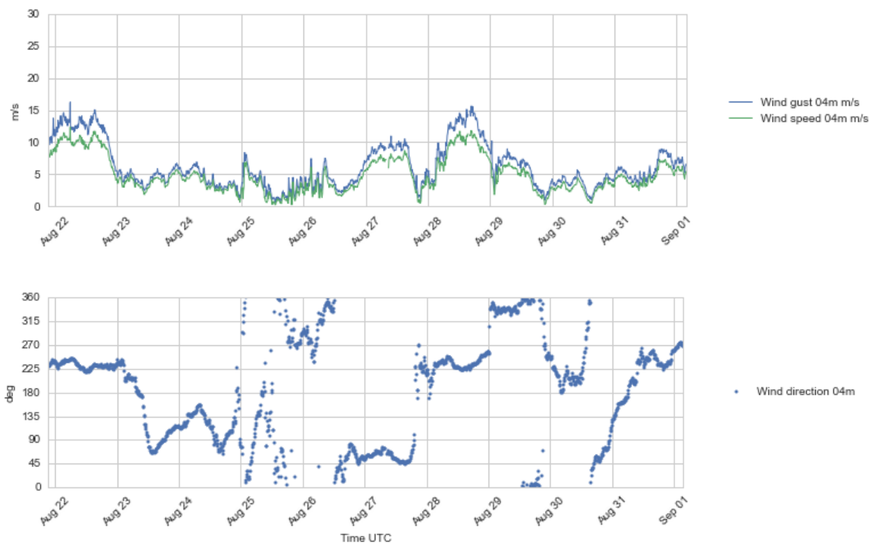
Figure 4.7 Plots of wind speed and gust (upper), and wind direction (lower) at 4 m a.s.l., 21 - 31 Aug 2016.
