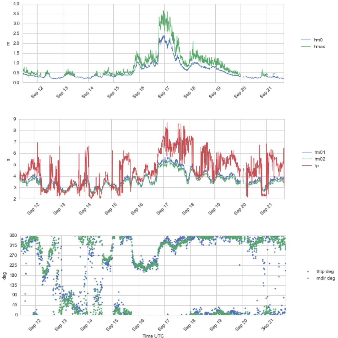
Figure 4.6 Time series plots of wave height ( H_{m0} and H_{max} ) (upper panel), wave period ( T_{m01} , T_{m02} and T_p ) (second panel), and wave direction ( ThTp and Mdir ) (lower panel), 11 - 21 Sept 2016.
