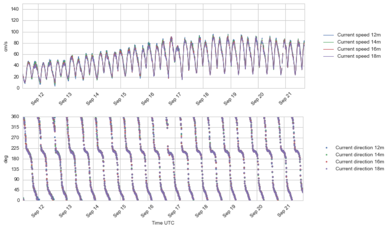
Figure 4.28 Time series plots of current speed (upper) and direction (lower panel), 12 - 18 m depth, 11 - 21 Sept 2016.
