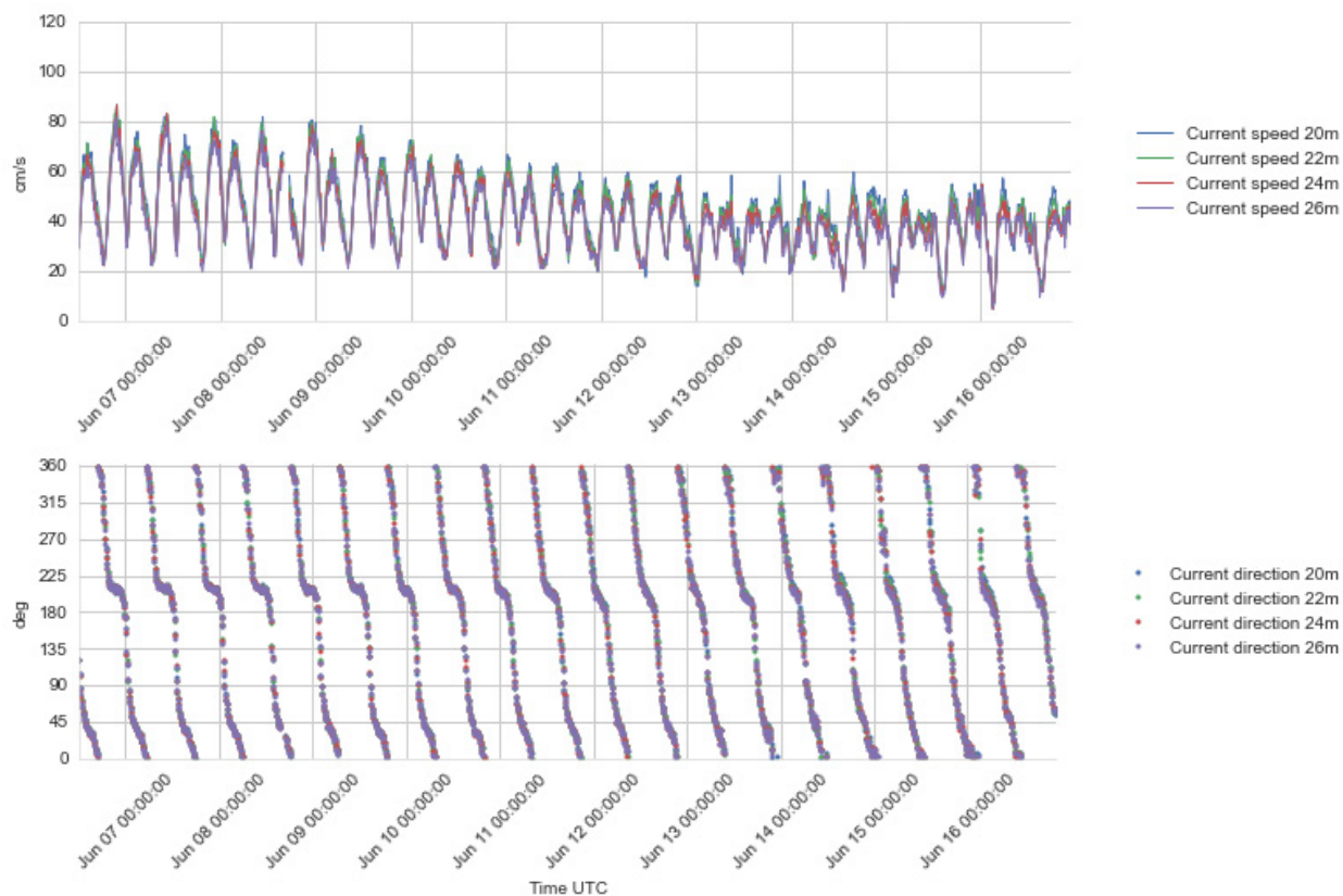
Figure 4.29 Time series plots of current speed (upper) and direction (lower panel), 20 - 26 m depth, 6 - 16 Jun 2016.
