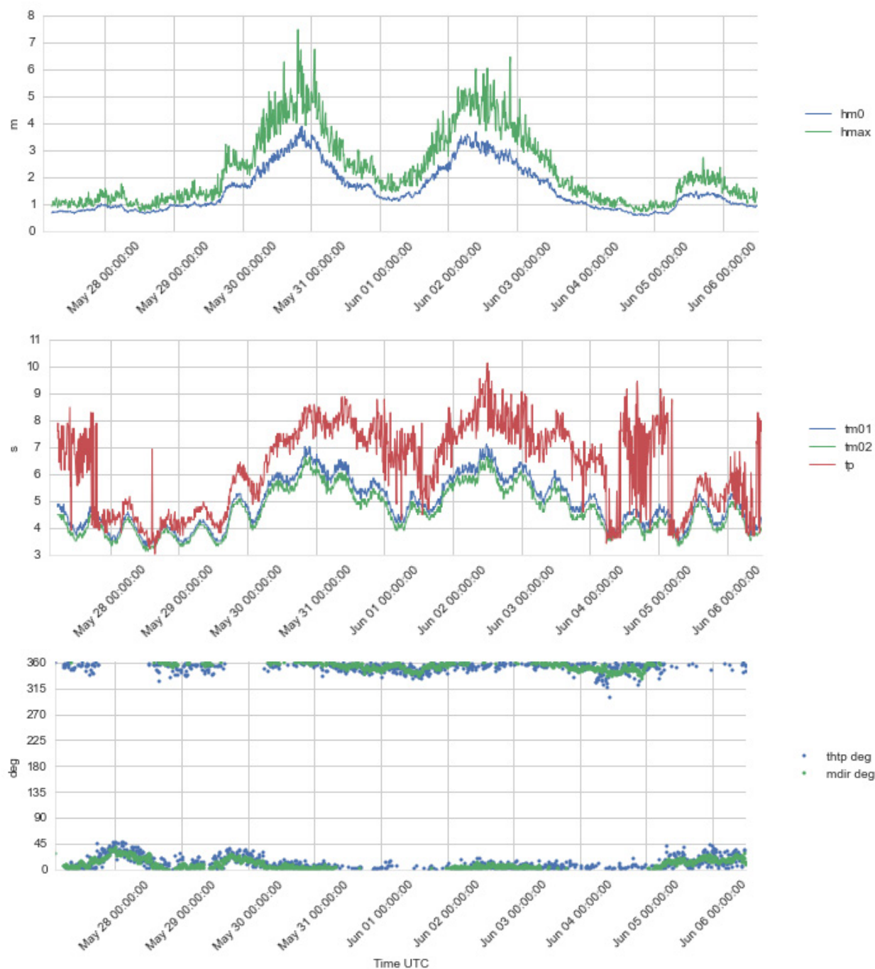
Figure 4.5 Time series plots of wave height ( H_{m0} and H_{max} ) (upper panel), wave period ( T_{m01} , T_{m02} and T_p ) (second panel), and wave direction ( ThTp and Mdir ) (lower panel), 27 May – 6 Jun 2016.
