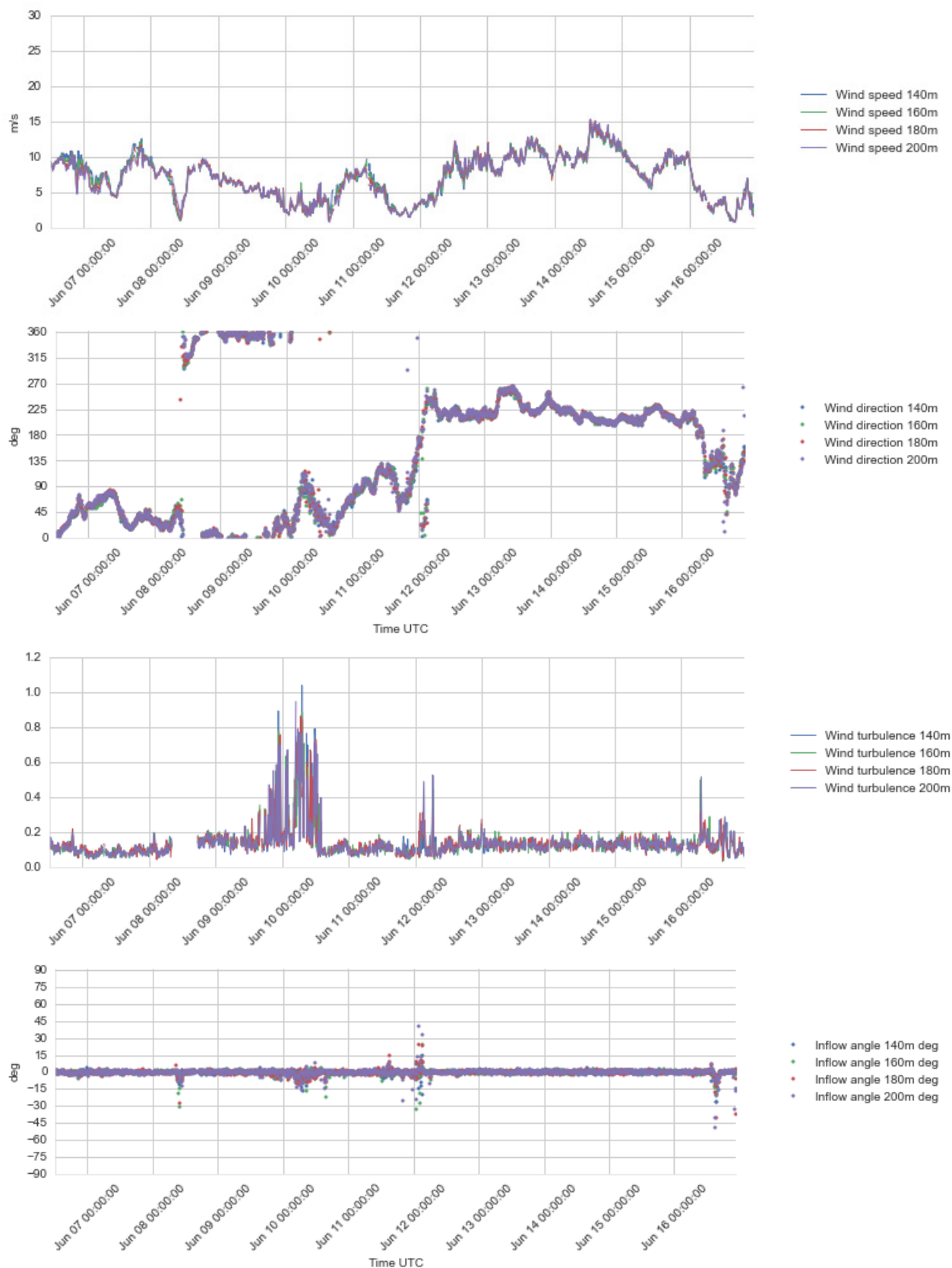
Figure 4.18 Plots of wind profile data, 140 – 200 m a.s.l., 6 - 16 Jun 2016.
