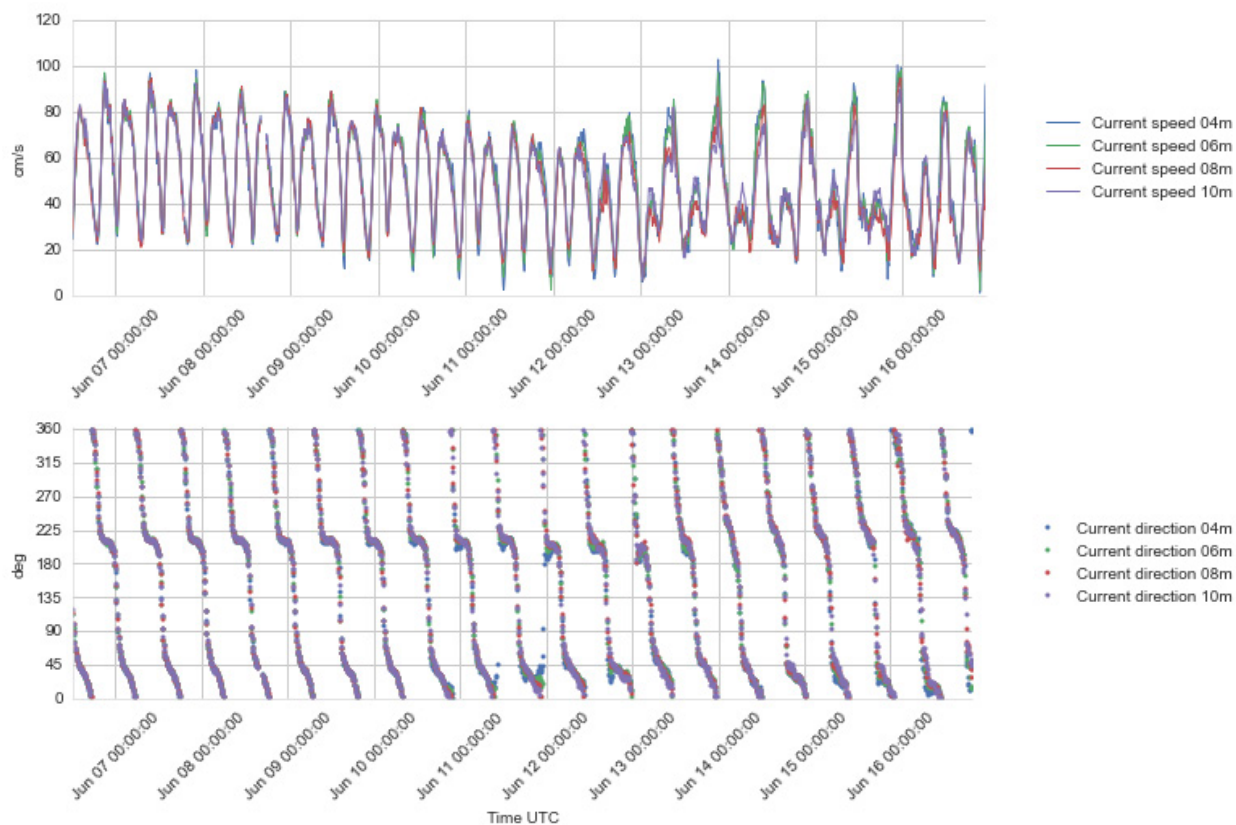
Figure 4.27 Time series plots of current speed (upper) and direction (lower panel), 4 - 10 m depth, 6 - 16 Jun 2016.
