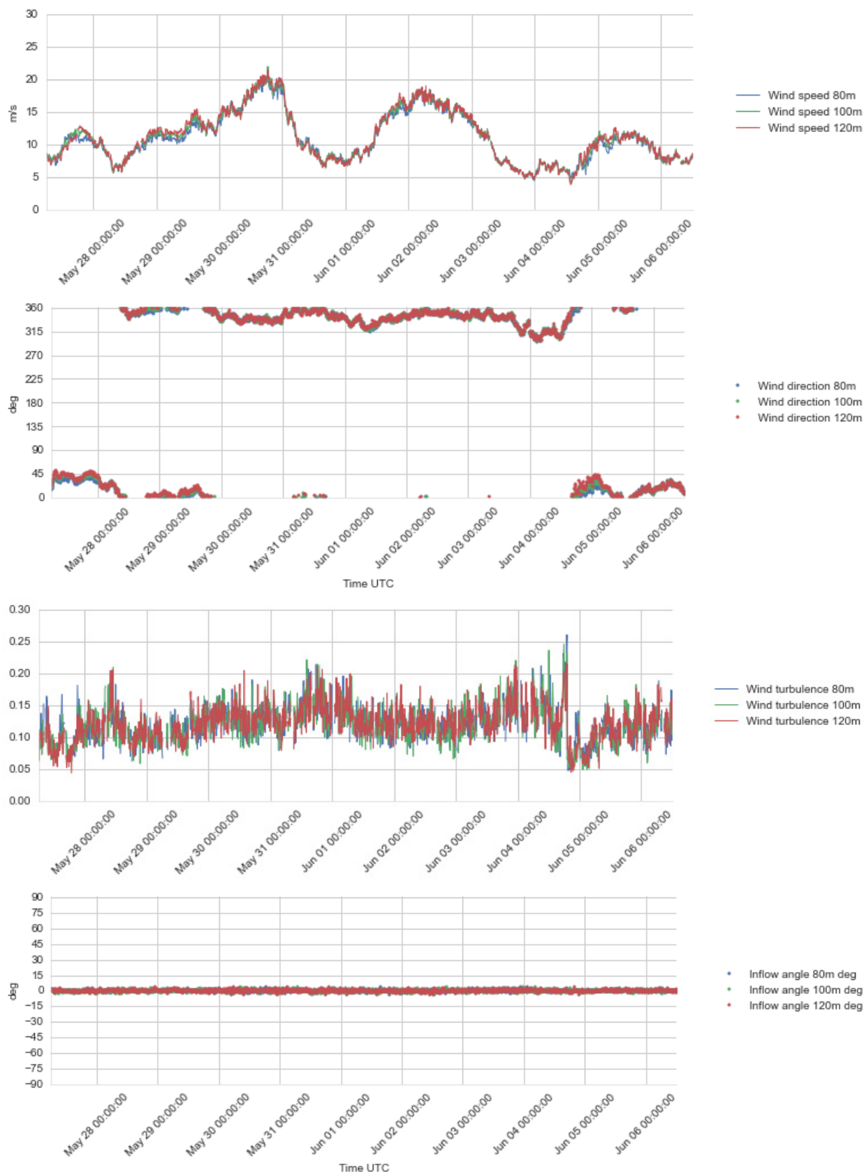
Figure 4.14 Plots of wind profile data, 80 – 120 m a.s.l., 27 May – 6 Jun 2016.
