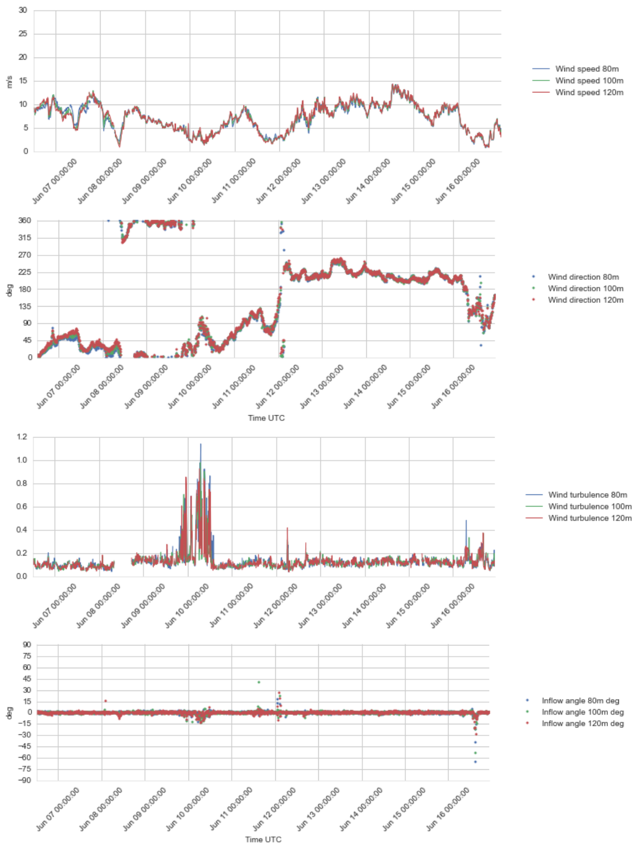
Figure 4.17 Plots of wind profile data, 80 – 120 m a.s.l., 6 - 16 Jun 2016.
