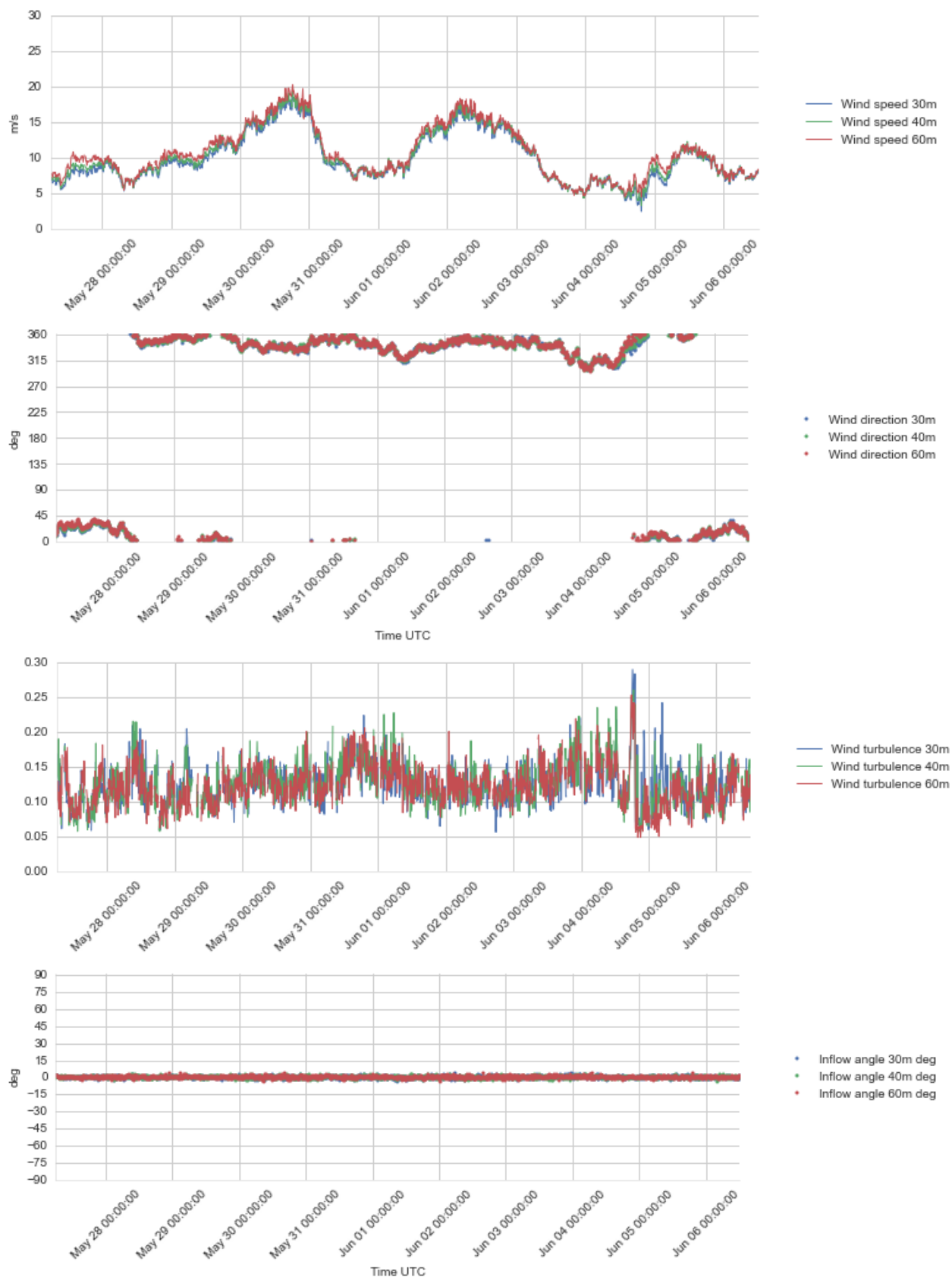
Figure 4.13 Plots of wind profile data, 30 – 60 m a.s.l., 27 May – 6 Jun 2016.
