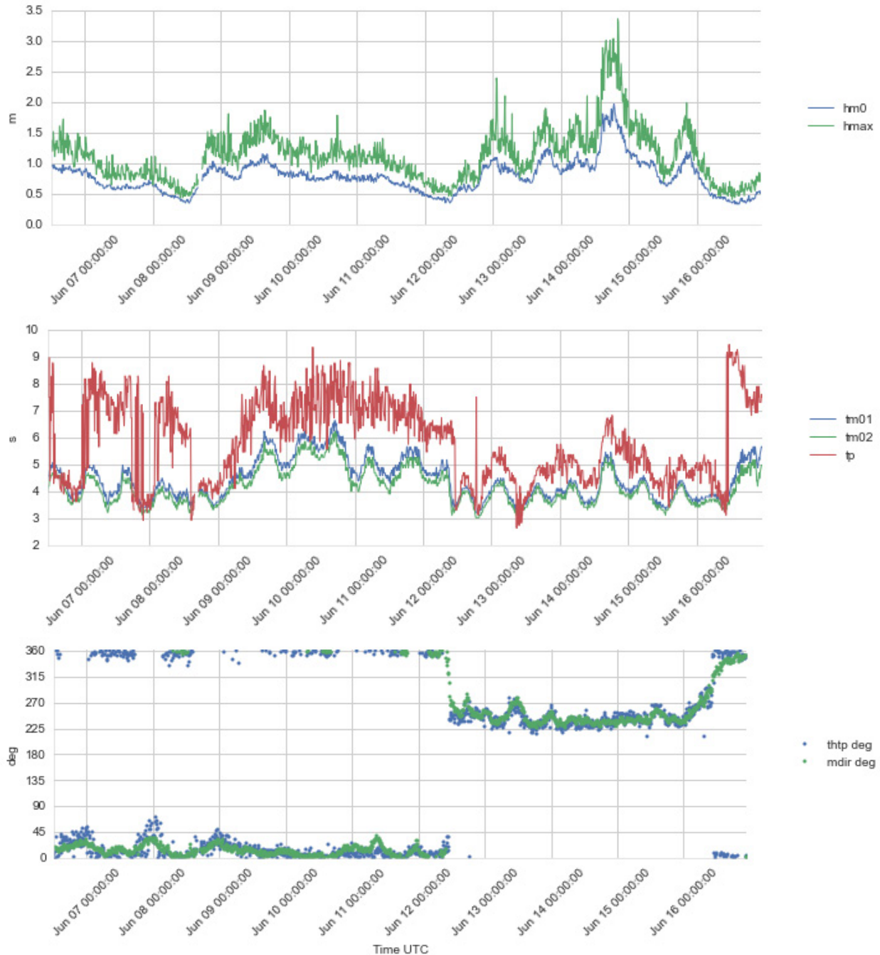
Figure 4.6 Time series plots of wave height ( Hm0 and Hmax ) (upper panel), wave period ( Tm01 , Tm02 and Tp ) (second panel), and wave direction ( ThTp and Mdir ) (lower panel), 6 - 16 Jun 2016.
