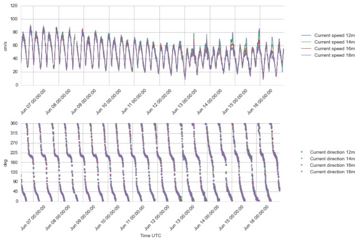
Figure 4.28 Time series plots of current speed (upper) and direction (lower panel), 12 - 18 m depth, 6 - 16 Jun 2016.
