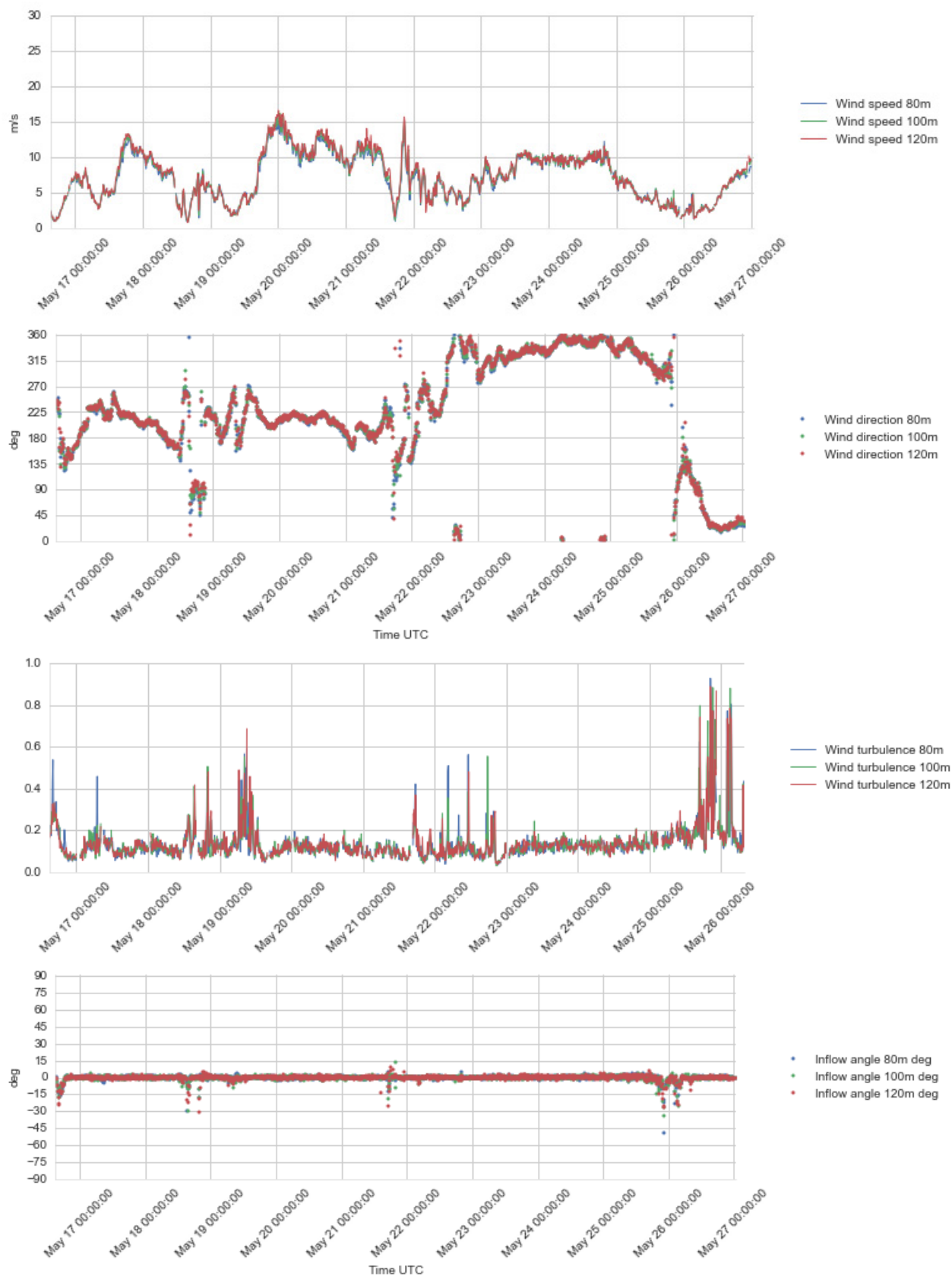
Figure 4.11 Plots of wind profile data, 80 – 120 m a.s.l., 16 – 26 May 2016.
