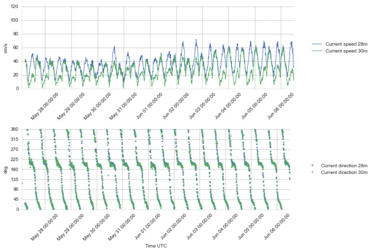
Figure 4.26 Time series plots of current speed (upper) and direction (lower panel), 28 – 30 m depth, 27 May – 6 Jun 2016.
