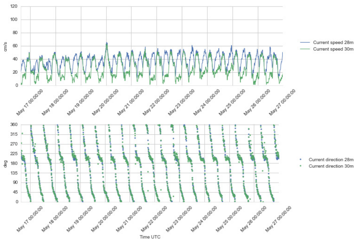
Figure 4.22 Time series plots of current speed (upper) and direction (lower panel), 28 - 30 m depth, 16 – 26 May 2016.
