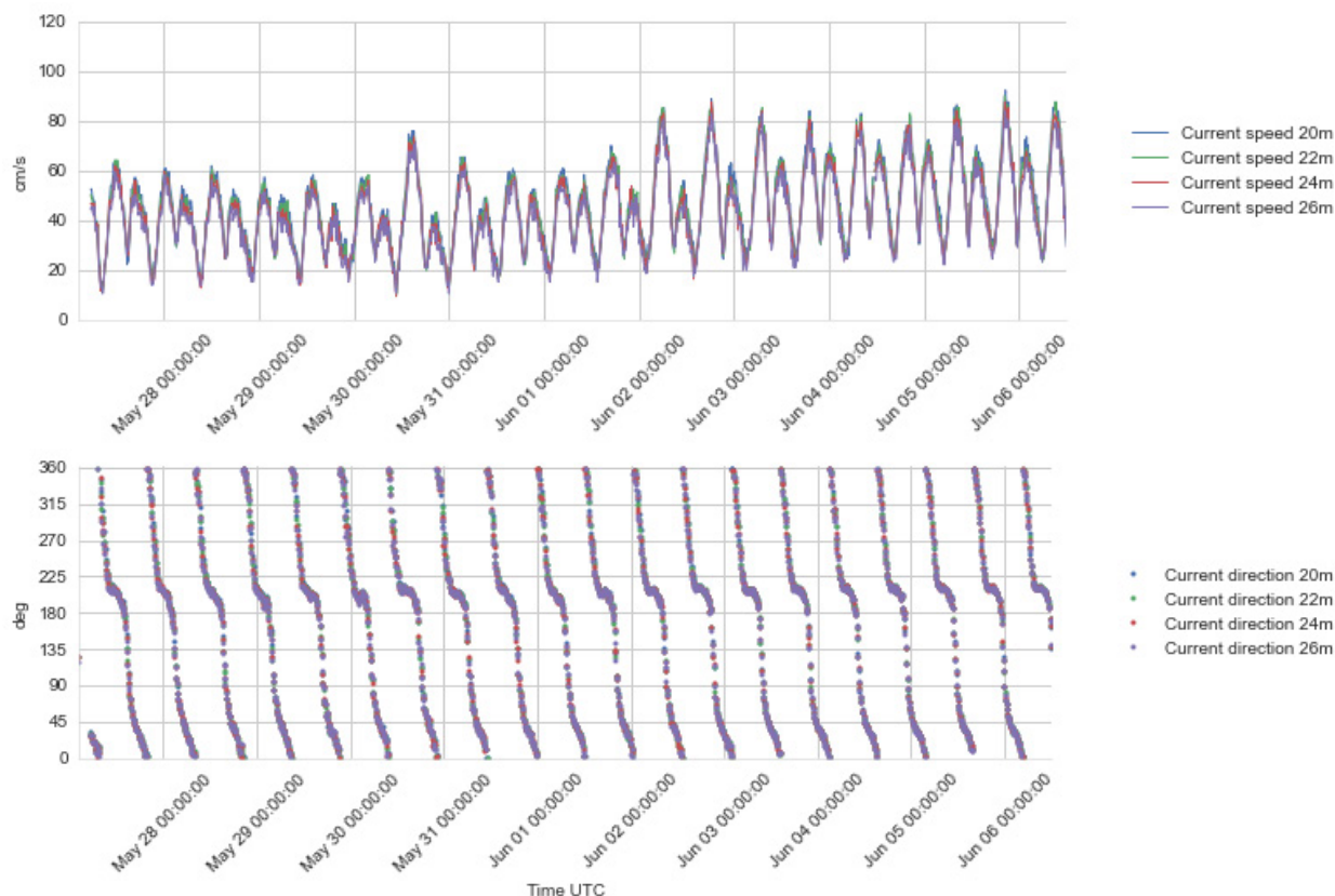
Figure 4.25 Time series plots of current speed (upper) and direction (lower panel), 20 – 26 m depth, 27 May – 6 Jun 2016.
