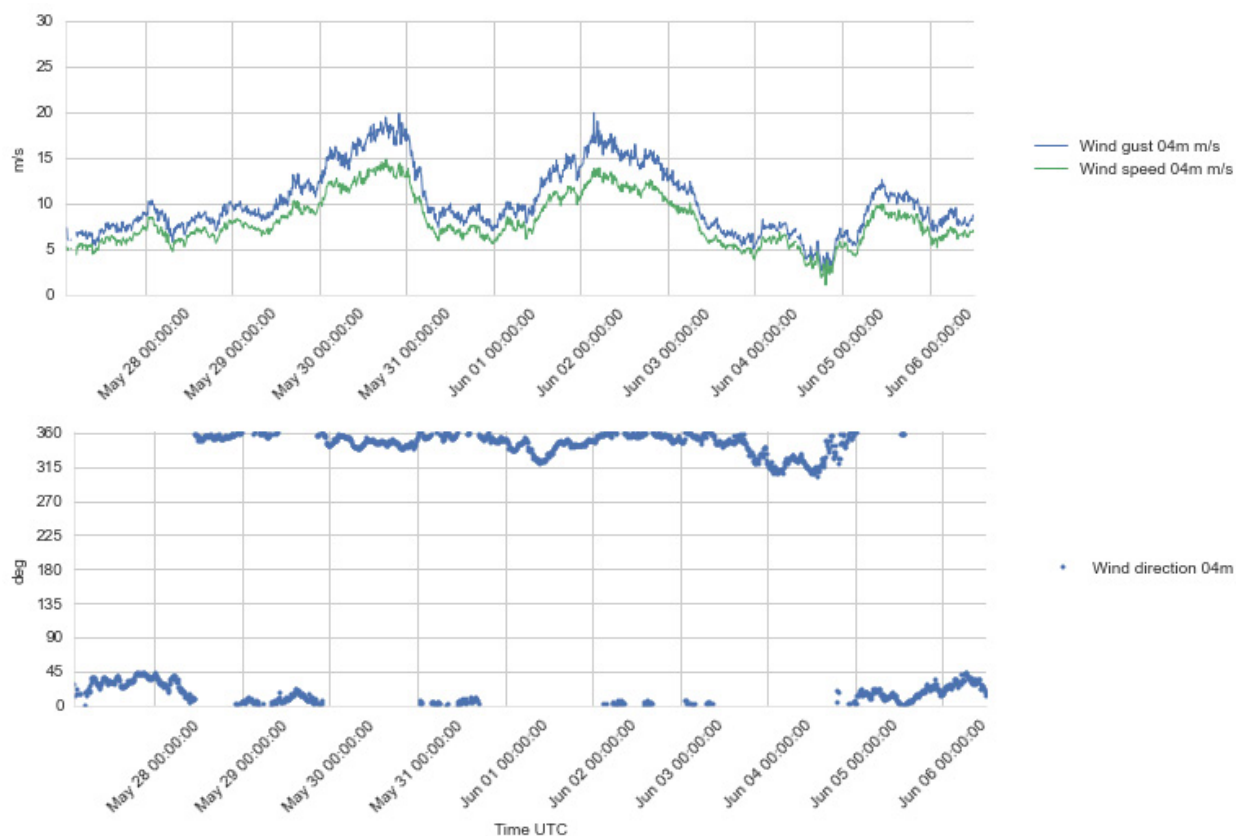
Figure 4.8 Plots of wind speed and gust (upper), and wind direction (lower) at 4 m a.s.l., 27 May – 6 Jun 2016.
