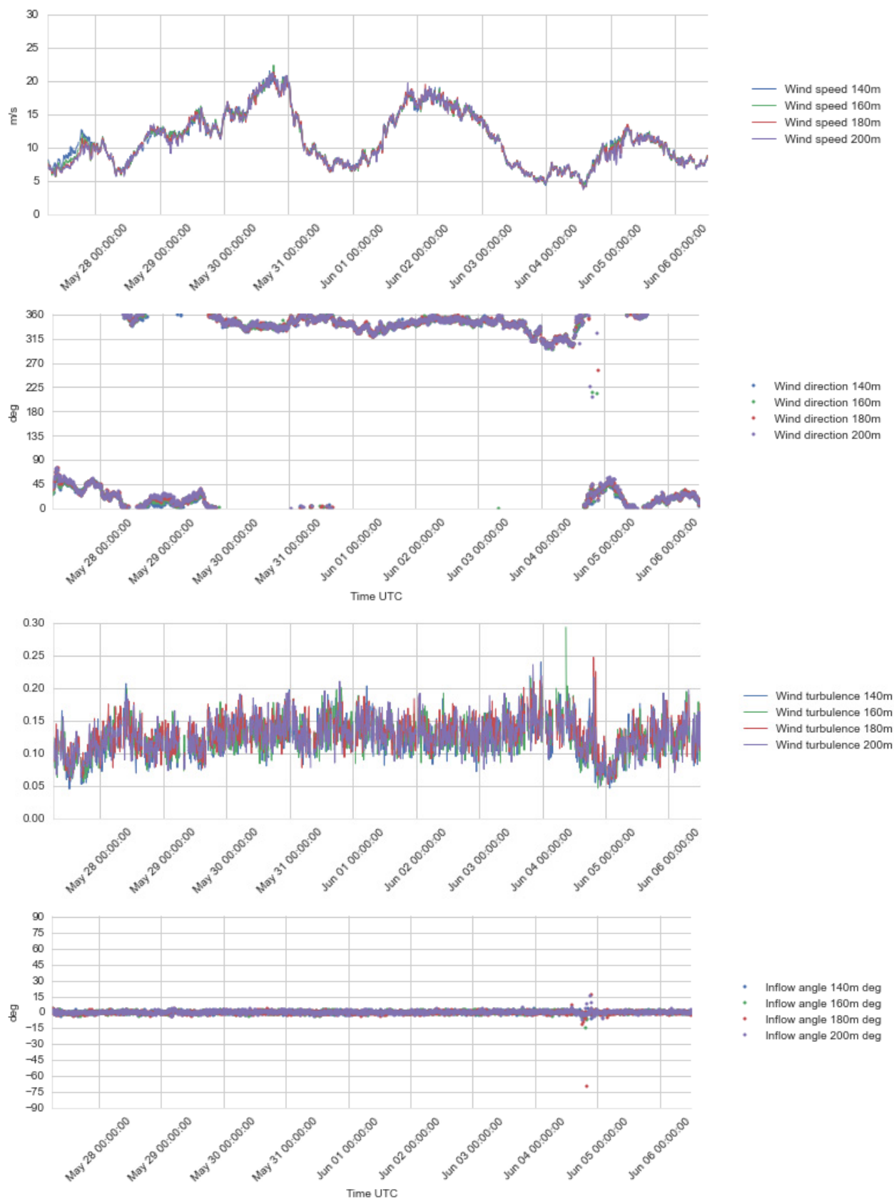
Figure 4.15 Plots of wind profile data, 140 – 200 m a.s.l., 27 May – 6 Jun 2016.
