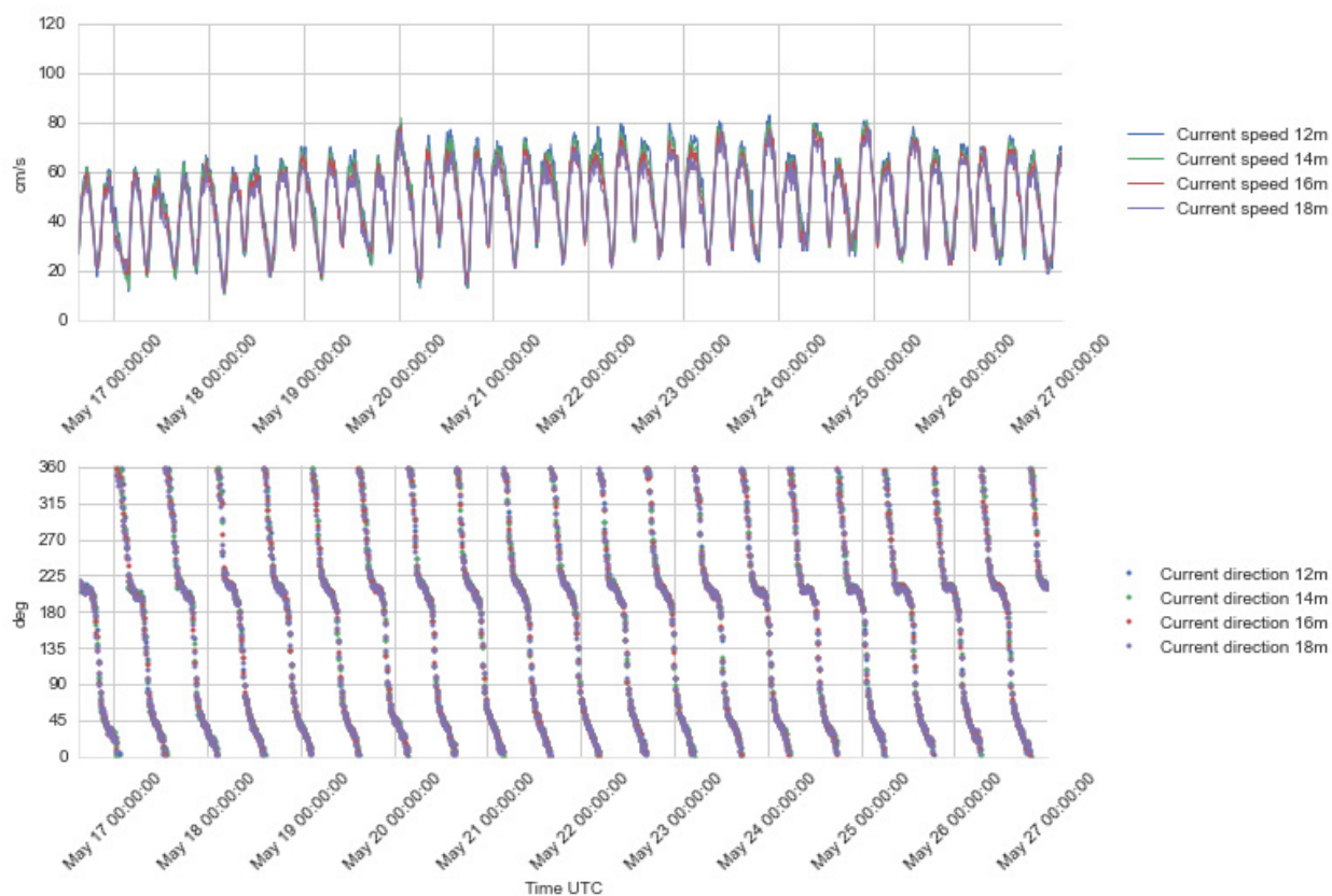
Figure 4.20 Time series plots of current speed (upper) and direction (lower panel), 12 - 18 m depth, 16 – 26 May 2016.
