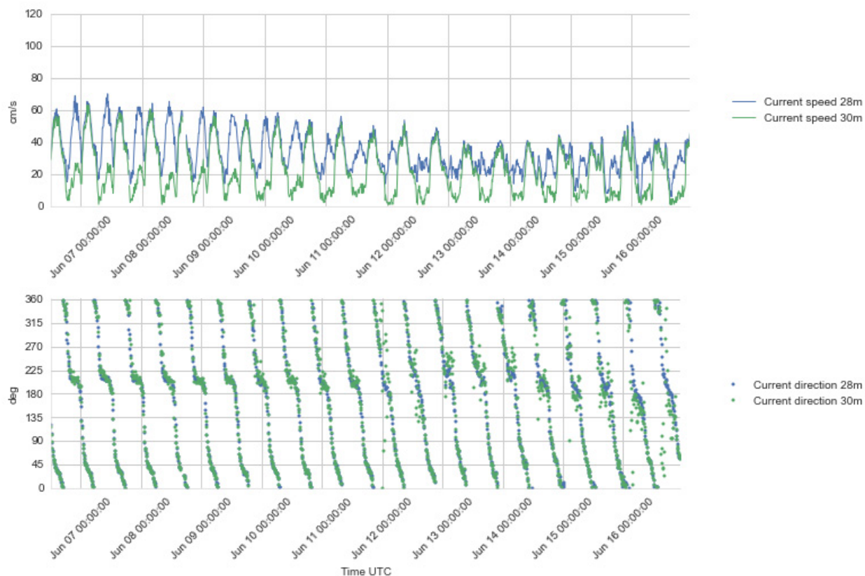
Figure 4.30 Time series plots of current speed (upper) and direction (lower panel), 28 - 30 m depth, 6 - 16 Jun 2016.
