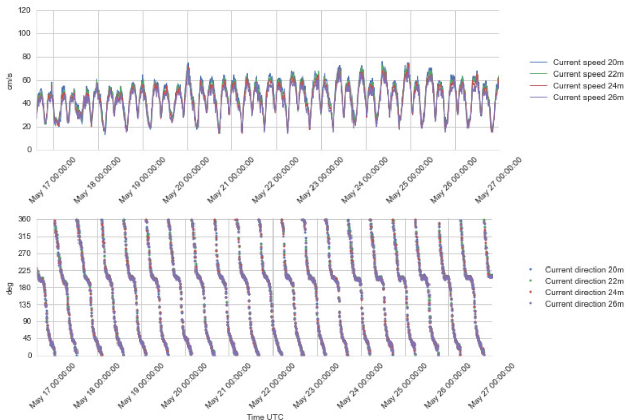
Figure 4.21 Time series plots of current speed (upper) and direction (lower panel), 20 - 26 m depth, 16 – 26 May 2016.
