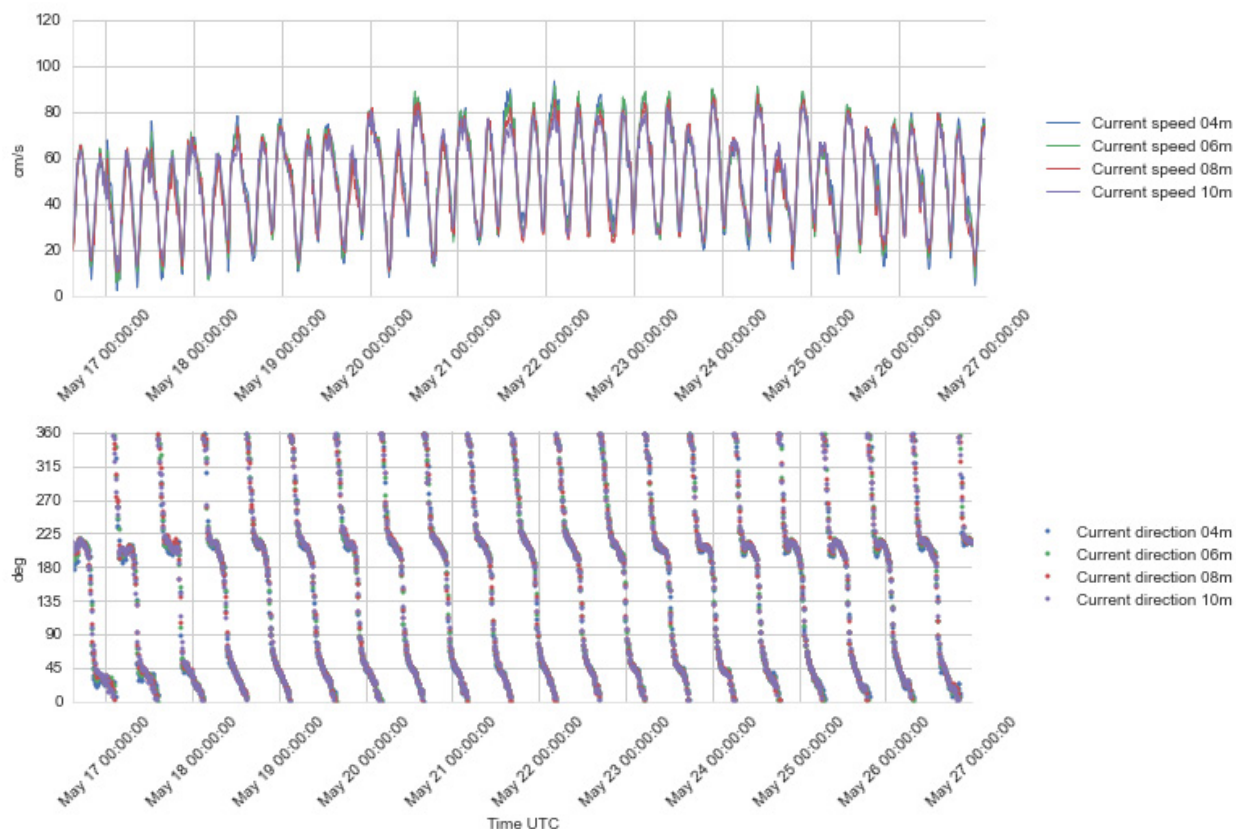
Figure 4.19 Time series plots of current speed (upper) and direction (lower panel), 4 - 10 m depth, 16 – 26 May 2016.
