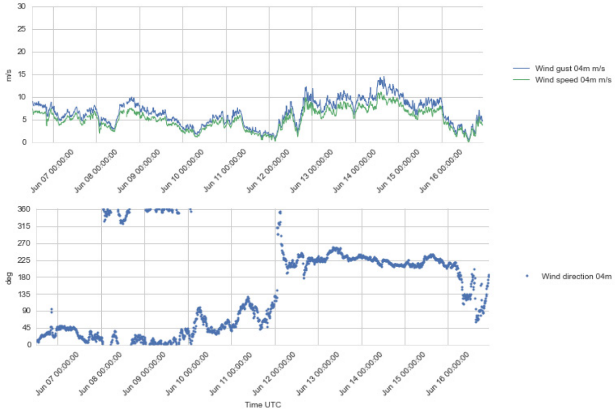
Figure 4.9 Plots of wind speed and gust (upper), and wind direction (lower) at 4 m a.s.l., 6 - 16 June 2016.
