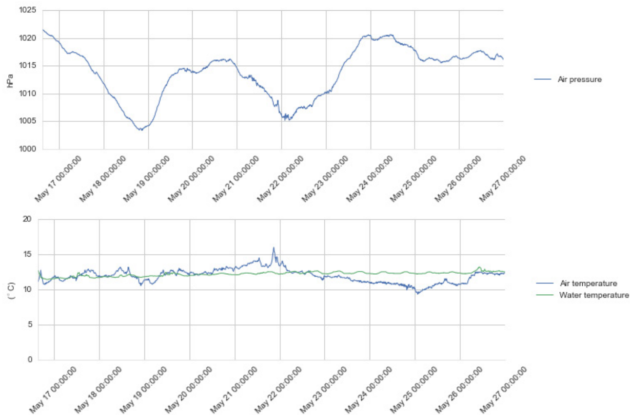
Figure 4.1 Time series plots of air pressure (upper panel), air and water temperature (lower panel), 16 - 26 May 2016.
