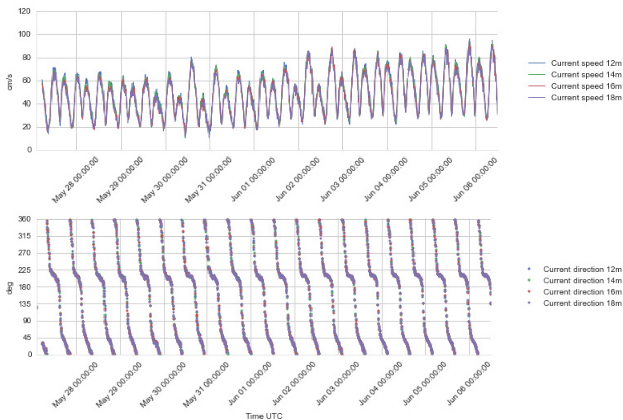
Figure 4.24 Time series plots of current speed (upper) and direction (lower panel), 12 -18 m depth, 27 May – 6 Jun 2016.
