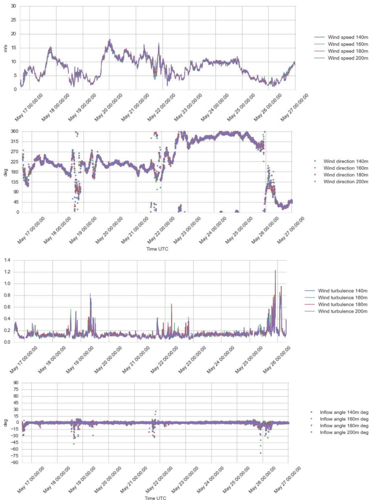
Figure 4.12 Plots of wind profile data, 140 – 200 m a.s.l., 16 – 26 May 2016.
