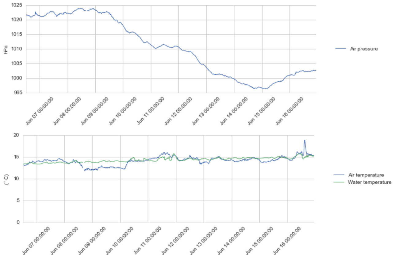
Figure 4.3 Time series plots of air pressure (upper panel), air and water temperature (lower panel), 6 - 16 Jun 2016.
