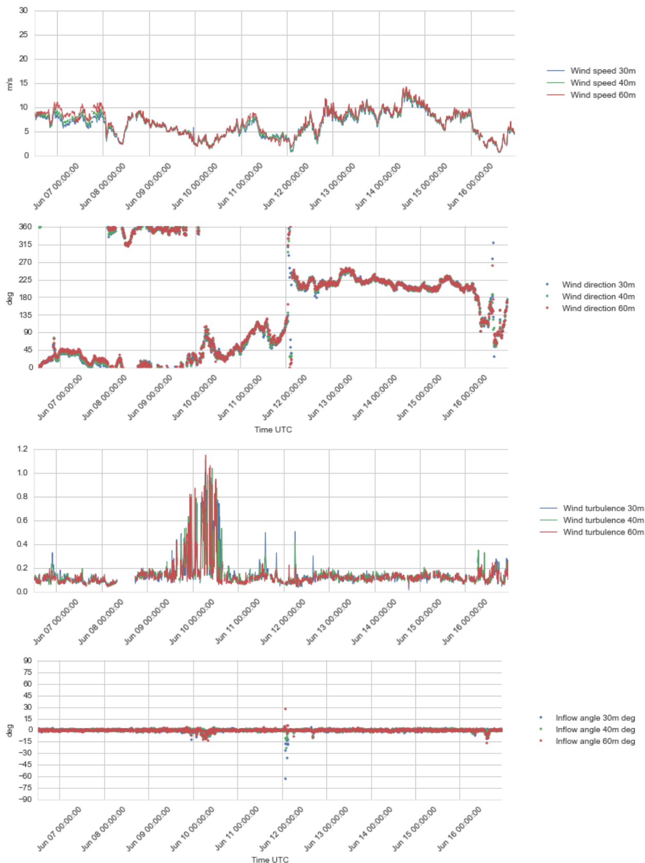
Figure 4.16 Plots of wind profile data, 30 – 60 m a.s.l., 6 - 16 Jun 2016.
