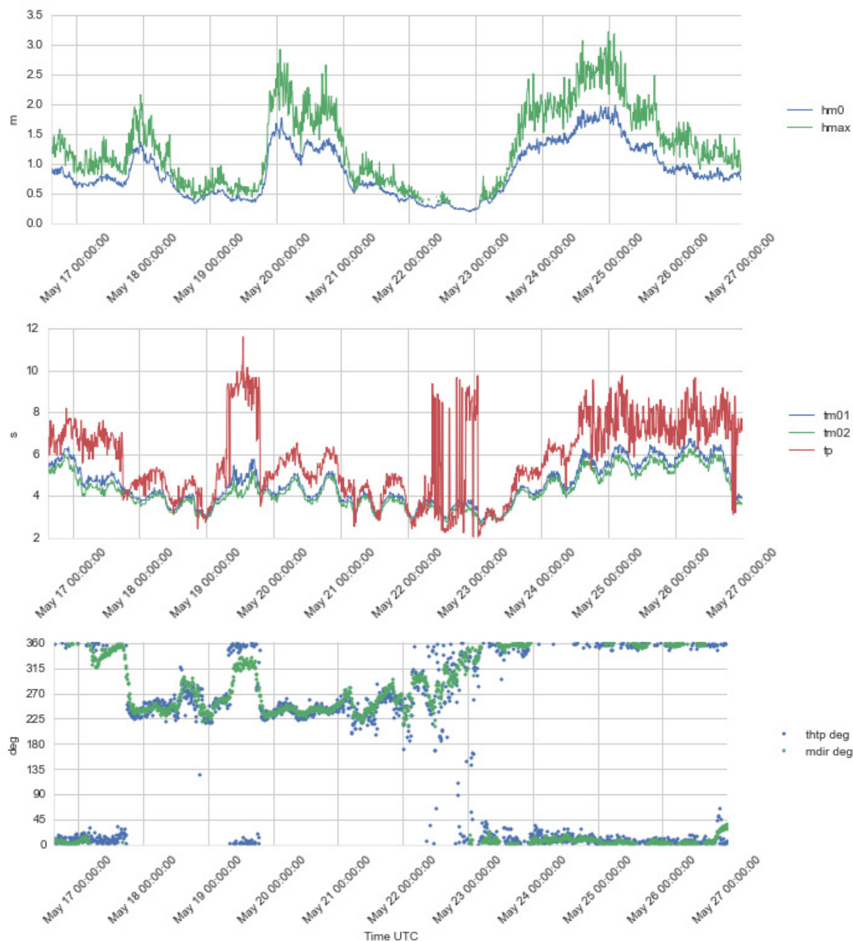
Figure 4.4 Time series plots of wave height ( Hm0 and Hmax ) (upper panel), wave period ( Tm01 , Tm02 and Tp ) (second panel), and wave direction ( ThTp and Mdir ) (lower panel), 16 - 26 May 2016.
