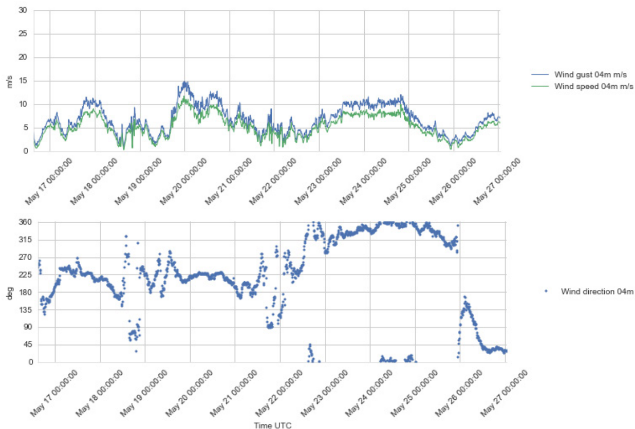
Figure 4.7 Plots of wind speed and gust (upper), and wind direction (lower) at 4 m a.s.l., 16 - 26 May 2016.
