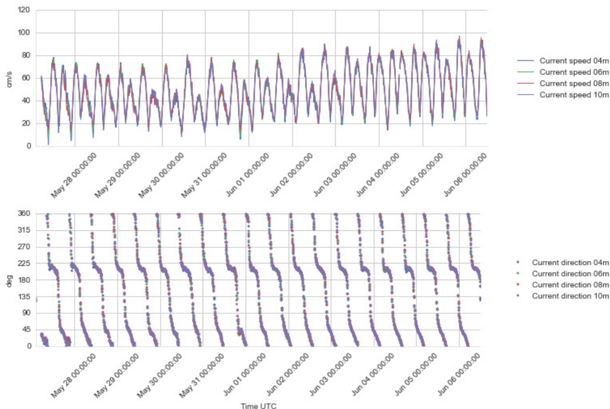
Figure 4.23 Time series plots of current speed (upper) and direction (lower panel), 4 - 10 m depth, 27 May – 6 Jun 2016.
