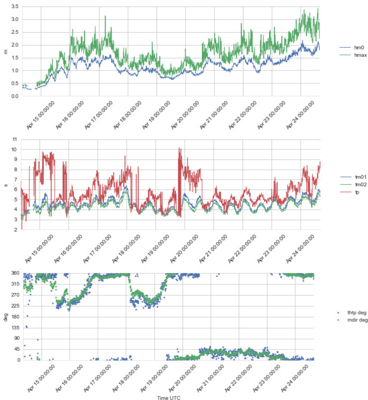
Figure 4.4 Time series plots of wave height (Hm0 and Hmax) (upper panel), wave period (Tm01, Tm02 and Tp) (second panel), and wave direction (ThTp and Mdir) (lower panel), 14 - 24 Apr 2016.
