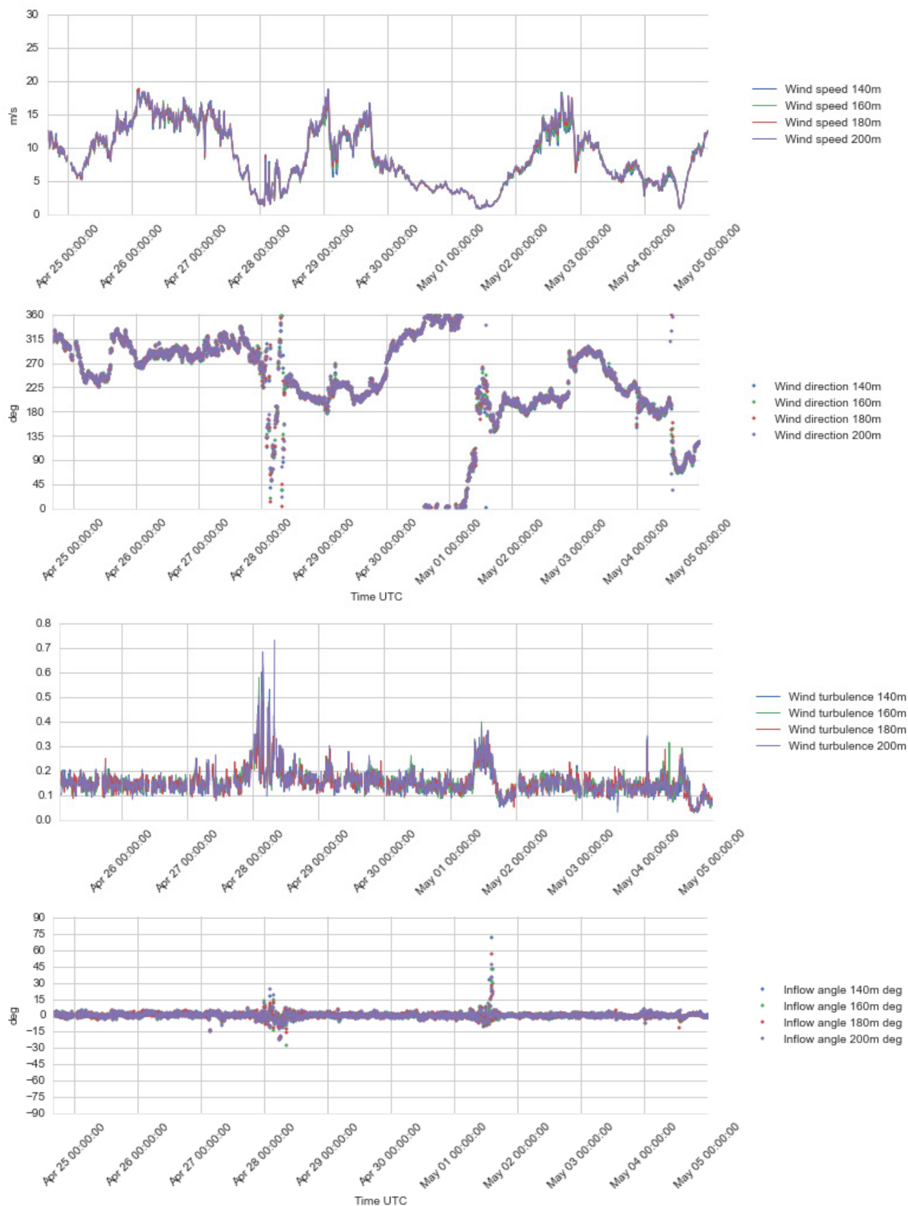
Figure 4.15 Plots of wind profile data, 140 – 200 m a.s.l., 24 Apr – 4 May 2016.
