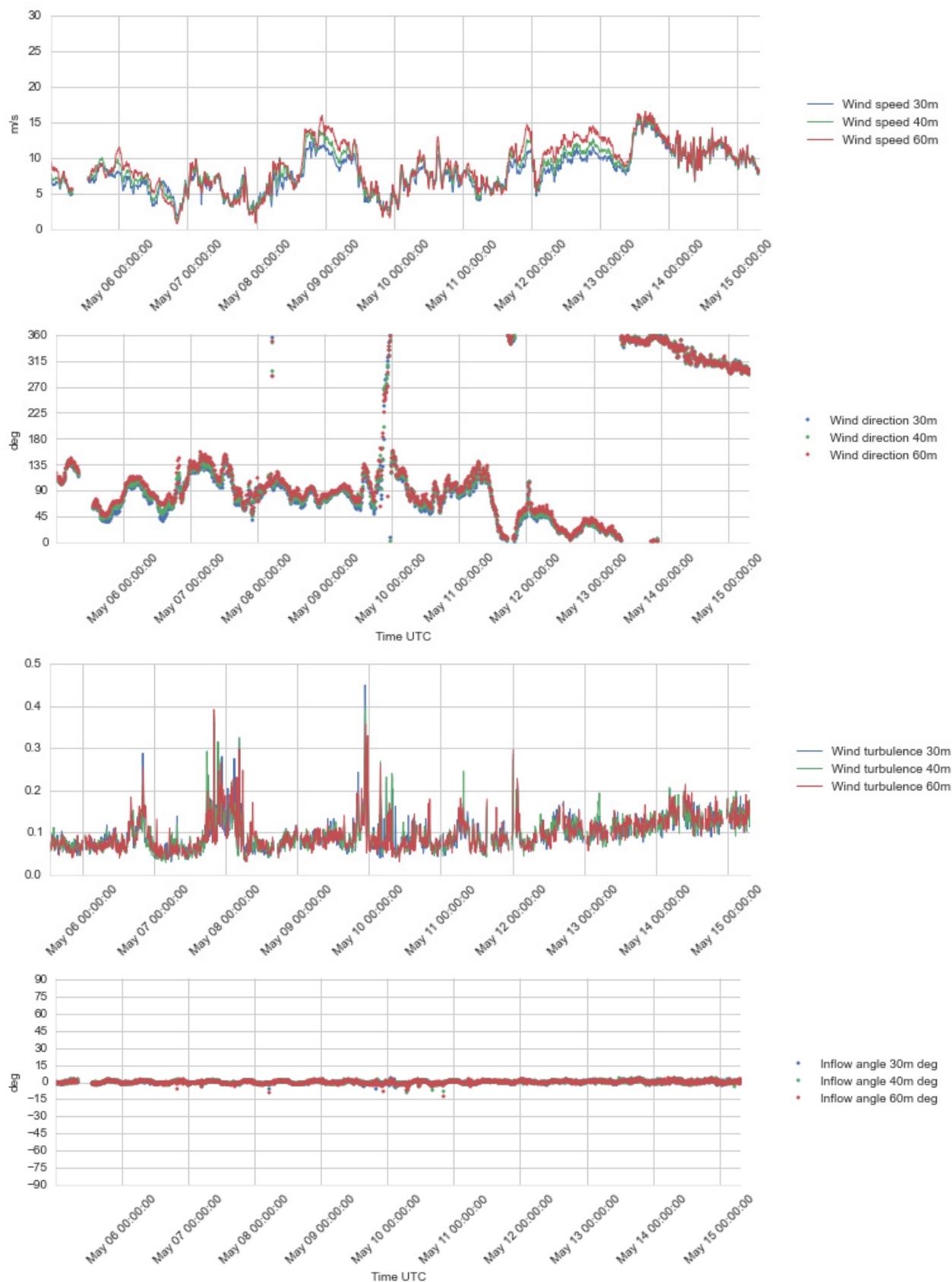
Figure 4.16 Plots of wind profile data, 30 – 60 m a.s.l., 5 – 15 May 2016.
