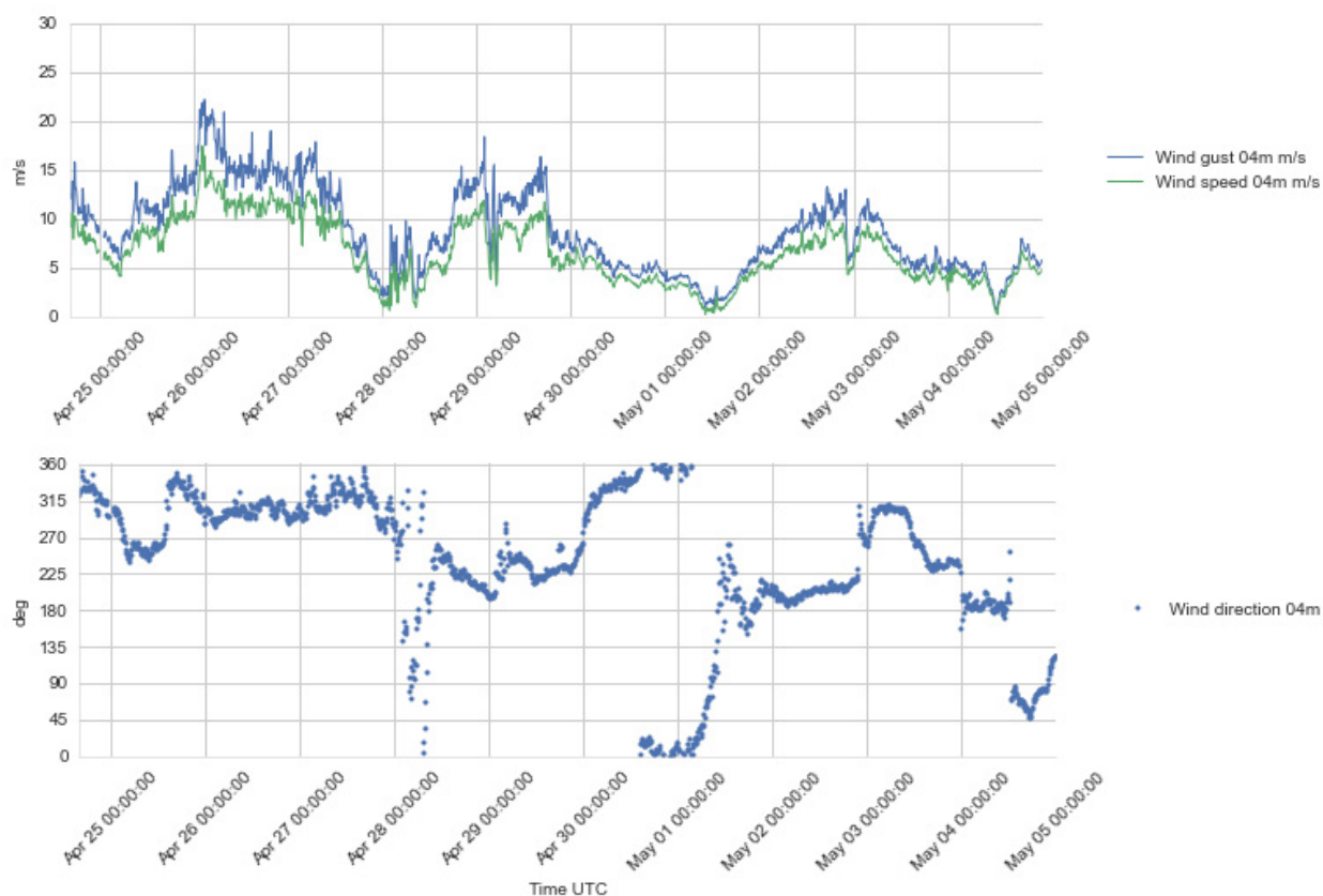
Figure 4.8 Plots of wind speed and gust (upper), and wind direction (lower) at 4 m a.s.l., 24 Apr – 4 May 2016.
