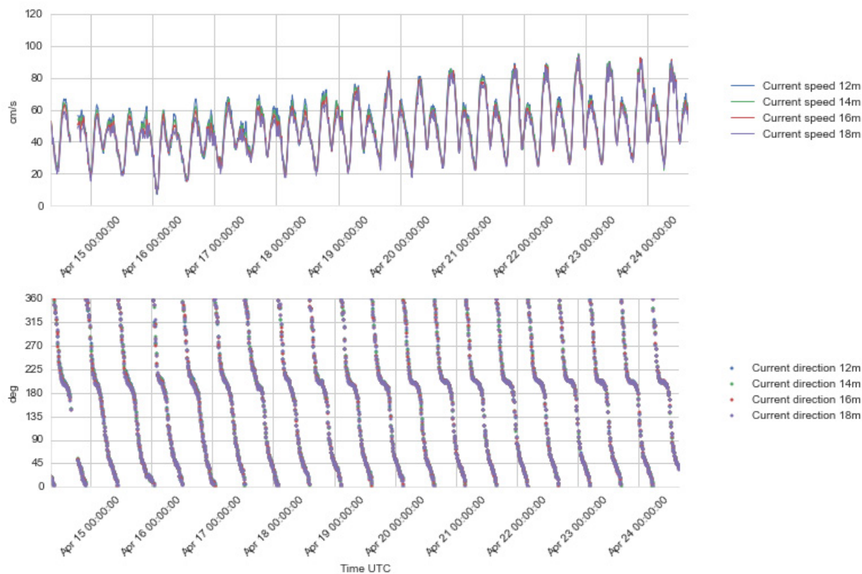
Figure 4.20 Time series plots of current speed (upper) and direction (lower panel), 12 - 18 m depth, 14 -24 Apr 2016.
