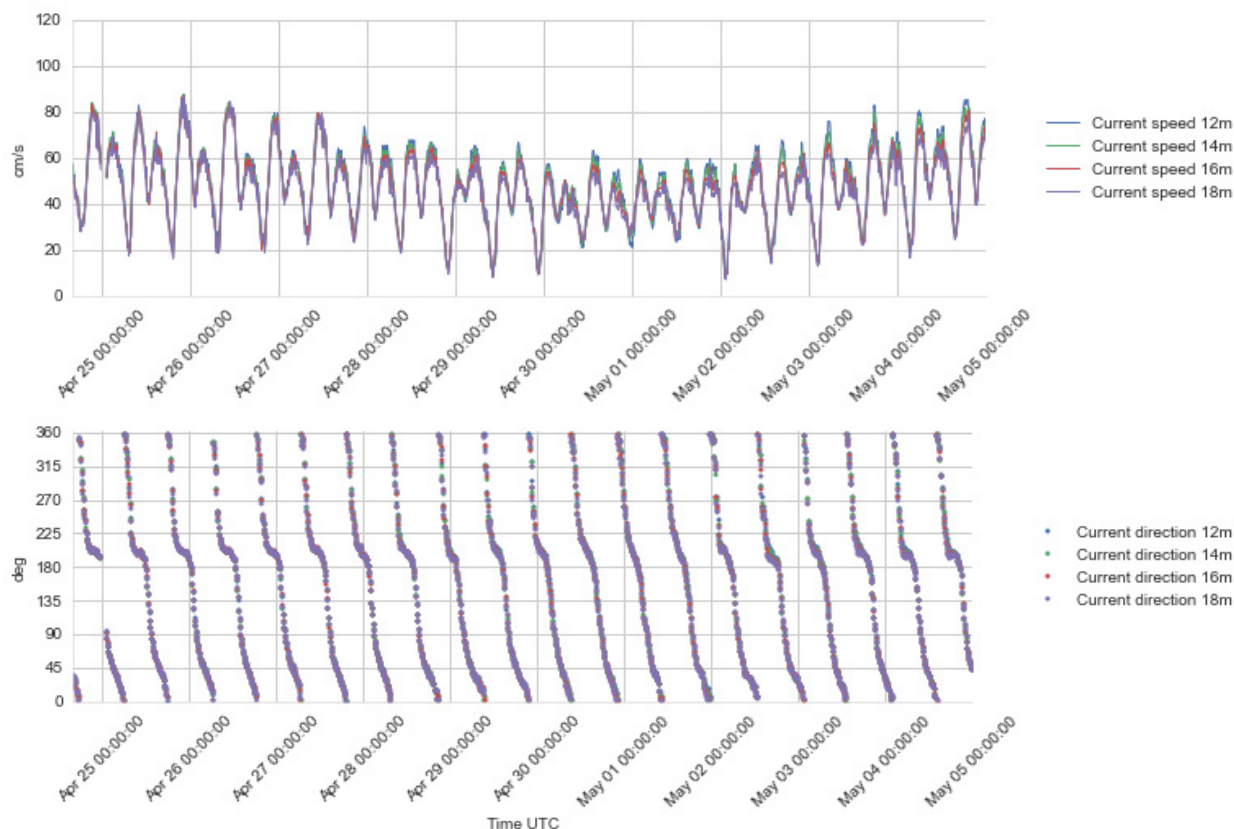
Figure 4.23 Time series plots of current speed (upper) and direction (lower panel), 12 -18 m depth, 24 Apr – 4 May 2016.
