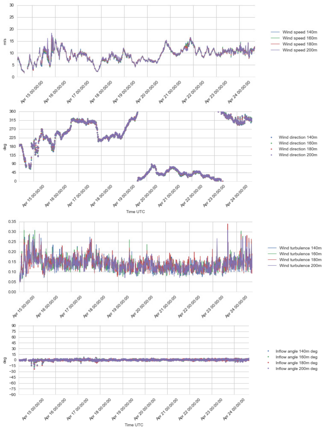
Figure 4.12 Plots of wind profile data, 140 – 200 m a.s.l., 14 - 24 Apr 2016.
