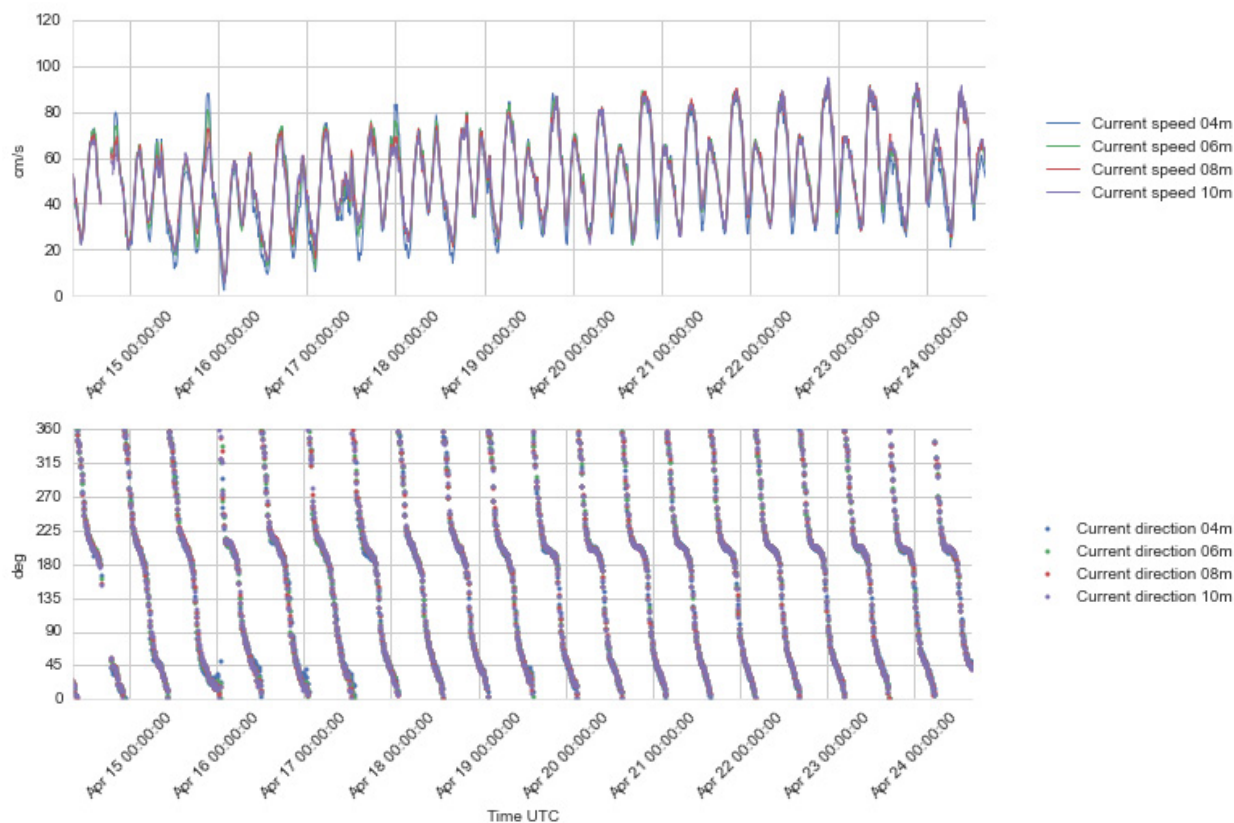
Figure 4.19 Time series plots of current speed (upper) and direction (lower panel), 4 - 10 m depth, 14 -24 Apr 2016
