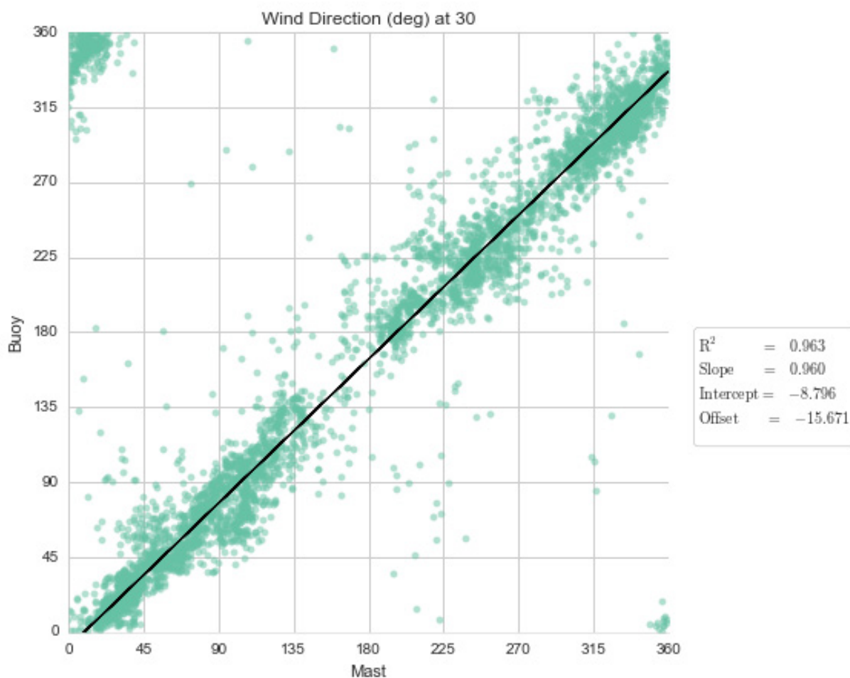
Figure 3.10 Wind direction at 30 m above sea level measured by the Lidar buoy compared to wind direction at Vlake van de Raan. (Samples with VR wind speed less than 2 m/s are excluded.) ("Offset" is the average difference of directions.)
