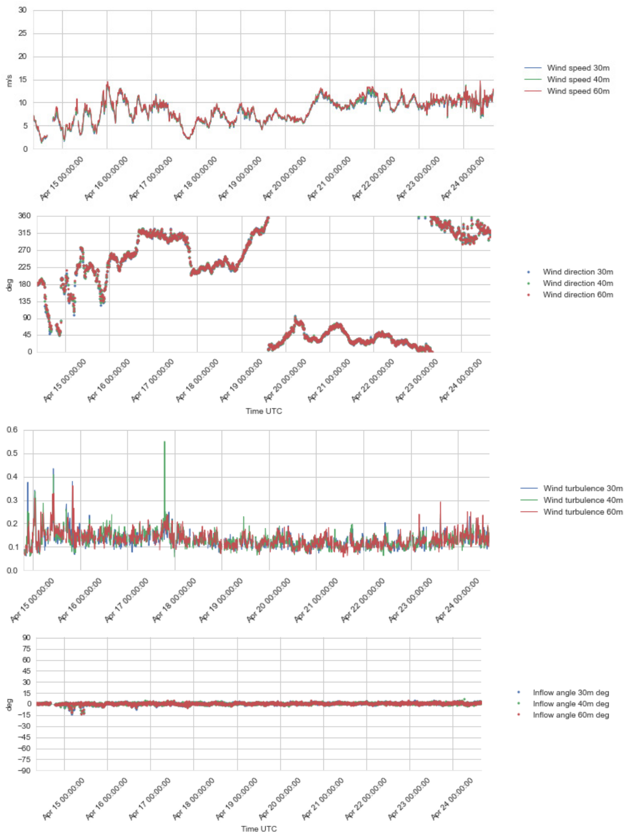
Figure 4.10 Plots of wind profile data, 30 – 60 m a.s.l., 14 - 24 Apr 2016.
