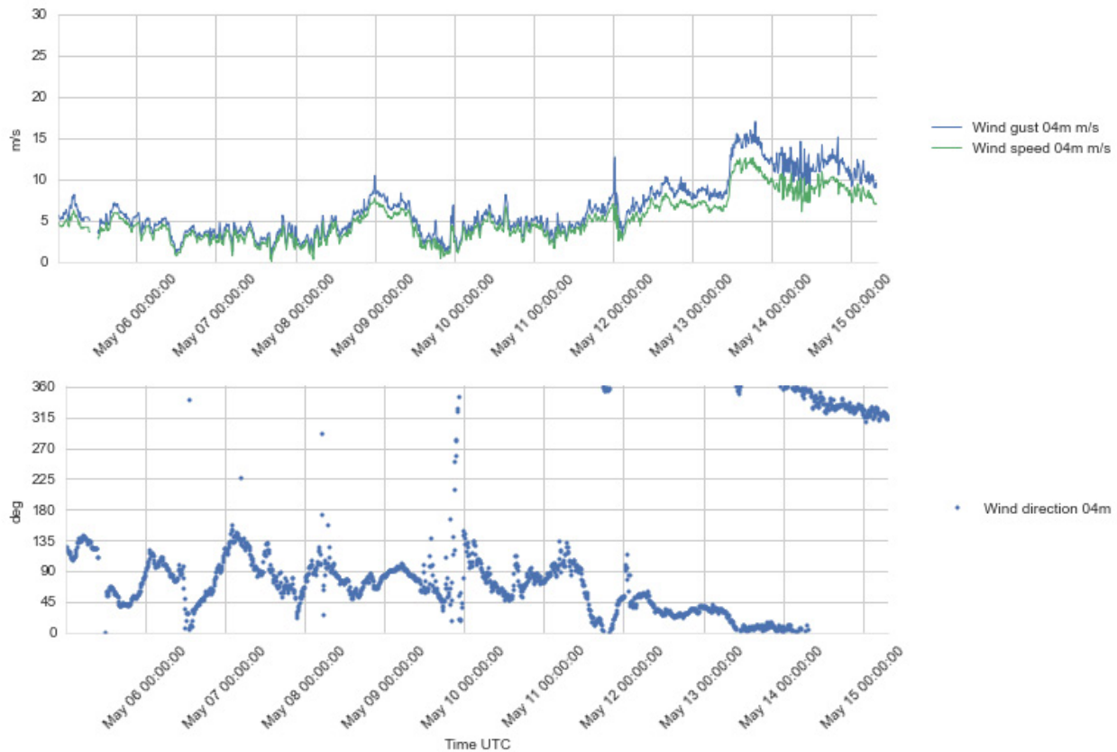
Figure 4.9 Plots of wind speed and gust (upper), and wind direction (lower) at 4 m a.s.l., 5 - 15 May 2016.
