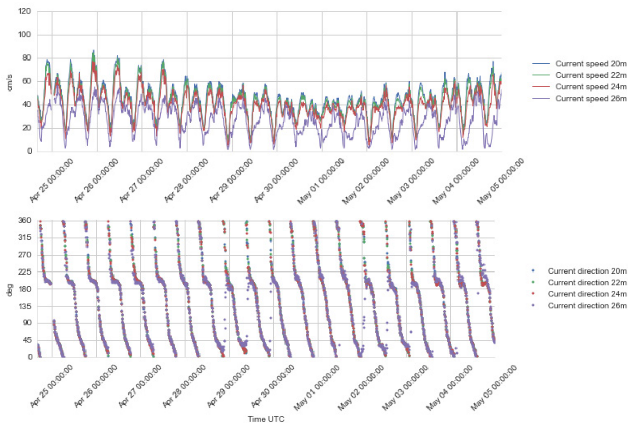
Figure 4.24 Time series plots of current speed (upper) and direction (lower panel), 20 – 26 m depth, 24 Apr – 4 May 2016.
