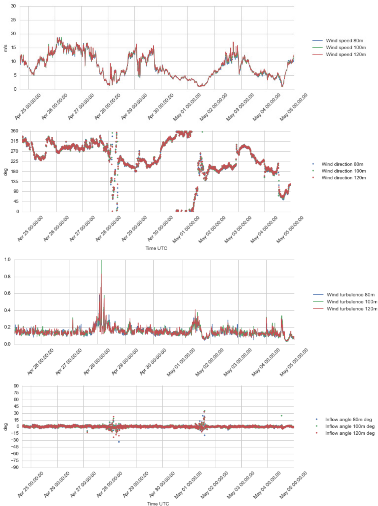
Figure 4.14 Plots of wind profile data, 80 – 120 m a.s.l., 24 Apr – 4 May 2016.
