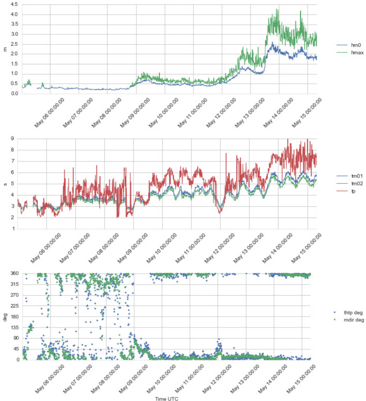
Figure 4.6 Time series plots of wave height ( Hm0 and Hmax ) (upper panel), wave period ( Tm01 , Tm02 and Tp ) (second panel), and wave direction ( ThTp and Mdir ) (lower panel), 5 - 15 May 2016.
