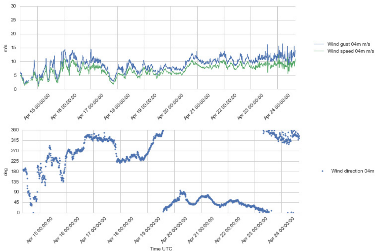
Figure 4.7 Plots of wind speed and gust (upper), and wind direction (lower) at 4 m a.s.l., 14 - 24 Apr 2016.
