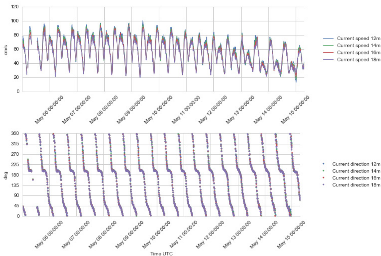
Figure 4.26 Time series plots of current speed (upper) and direction (lower panel), 12 - 18 m depth, 5 – 15 May 2016.
