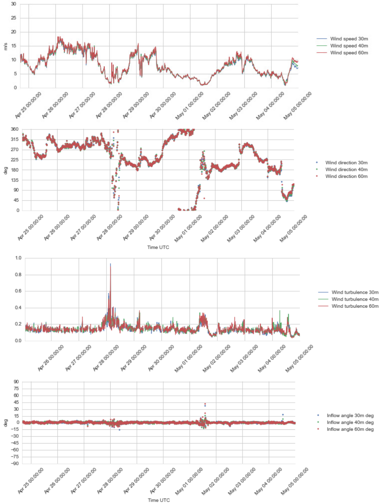
Figure 4.13 Plots of wind profile data, 30 – 60 m a.s.l., 24 Apr – 4 May 2016.
