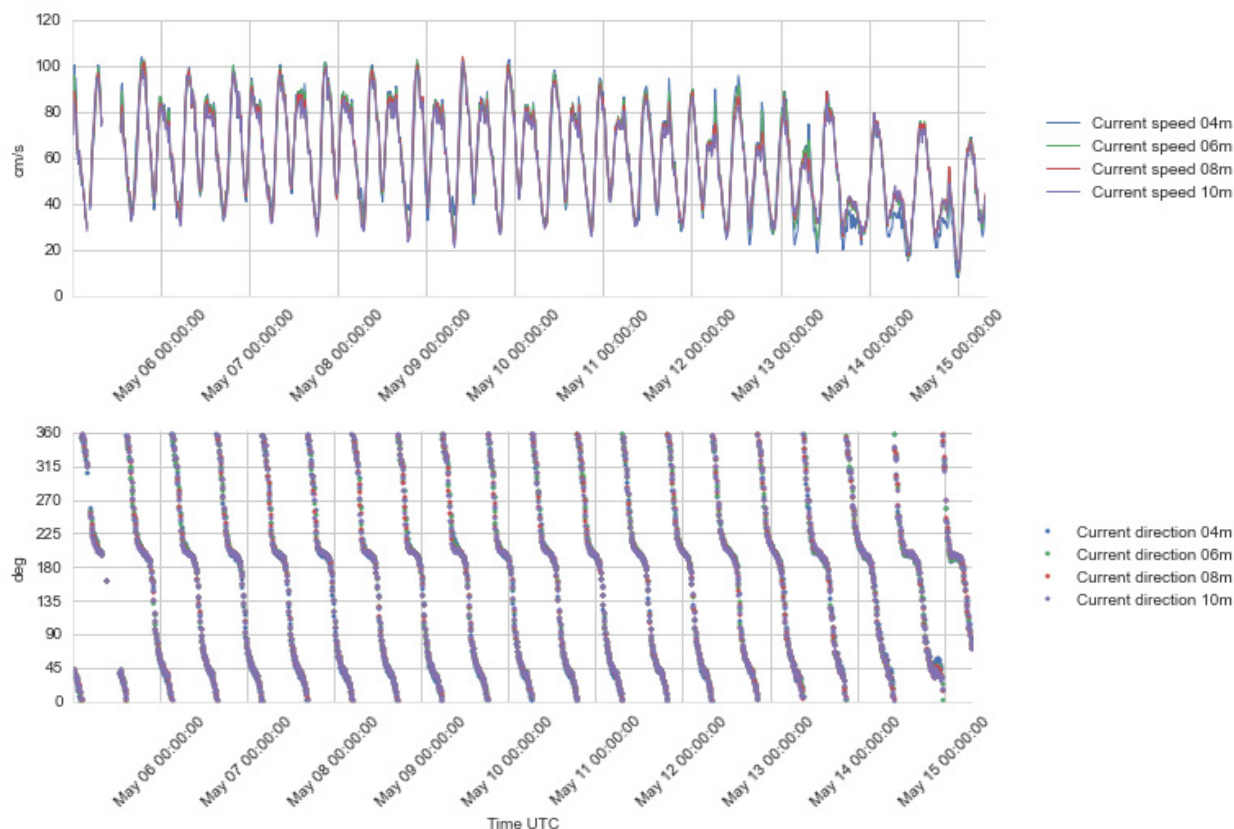
Figure 4.25 Time series plots of current speed (upper) and direction (lower panel), 4 - 10 m depth, 5 – 15 May 2016.
