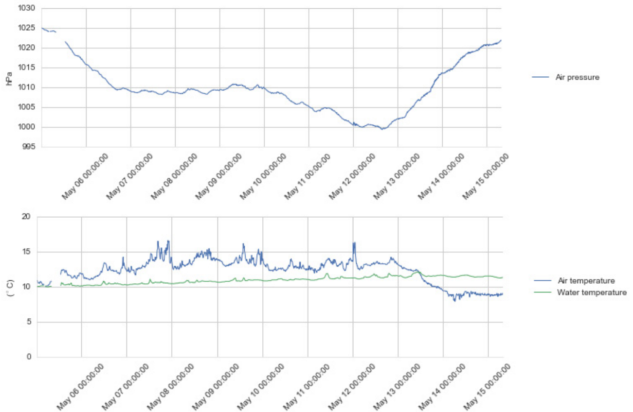
Figure 4.3 Time series plots of air pressure (upper panel), air and water temperature (lower panel), 5 - 15 May 2016.
