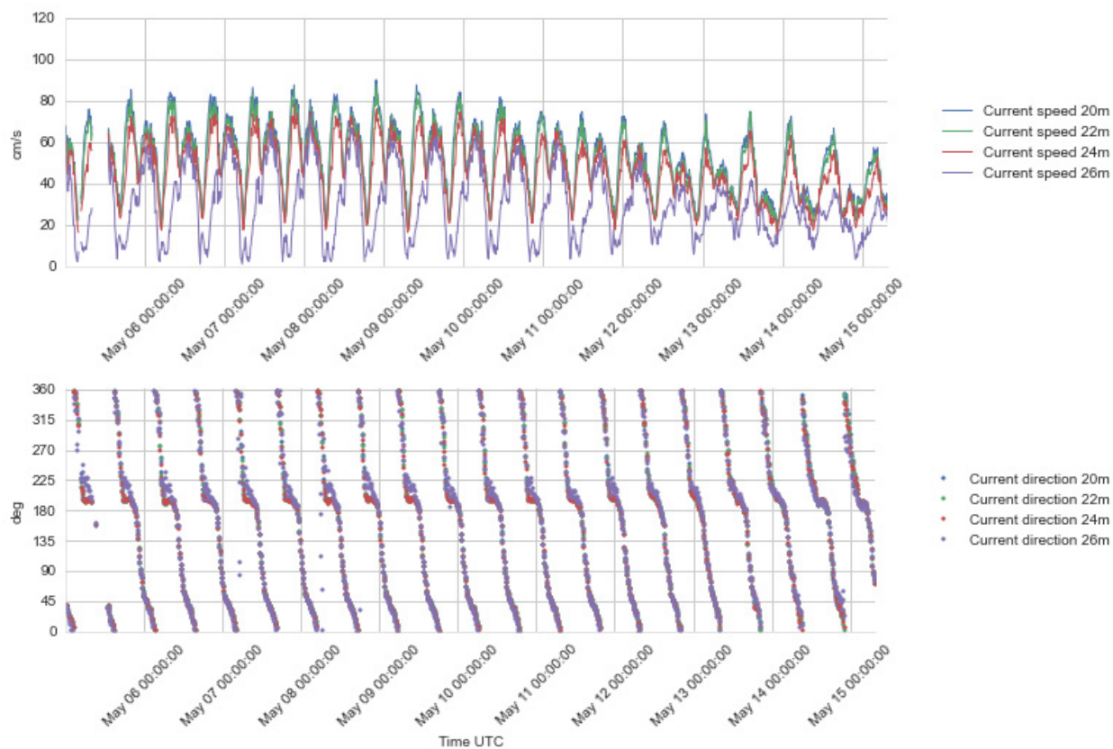
Figure 4.27 Time series plots of current speed (upper) and direction (lower panel), 20 - 26 m depth, 5 – 15 May 2016.
