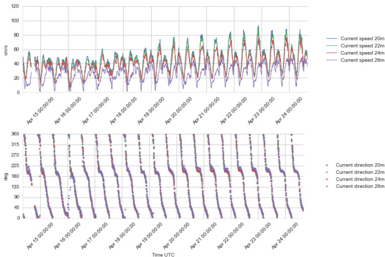
Figure 4.21 Time series plots of current speed (upper) and direction (lower panel), 20 - 26 m depth, 14 -24 Apr 2016.
