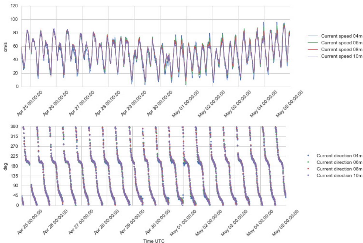
Figure 4.22 Time series plots of current speed (upper) and direction (lower panel), 4 - 10 m depth, 24 Apr – 4 May 2016.
