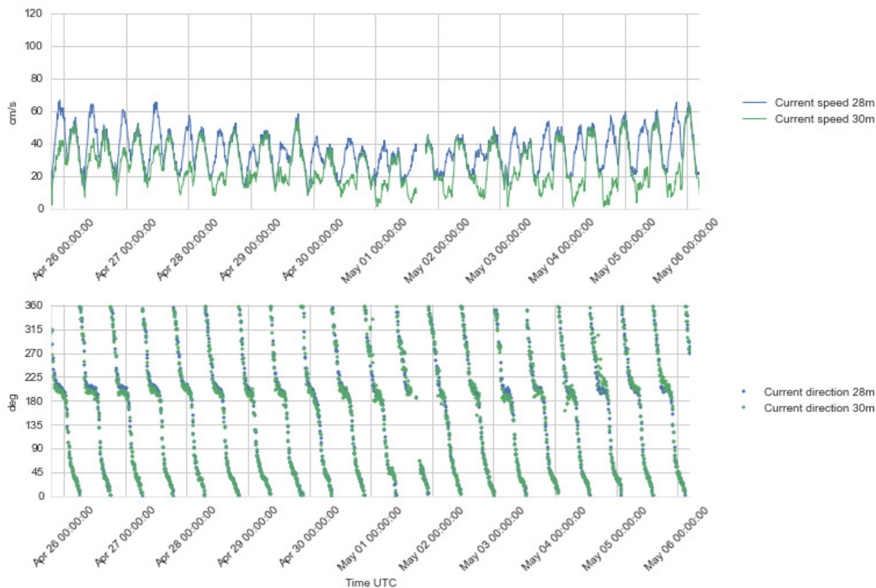
Figure 4.26 Time series plots of current speed (upper) and direction (lower panel), 28 – 30 m depth, 25 Apr – 6 May 2016.
