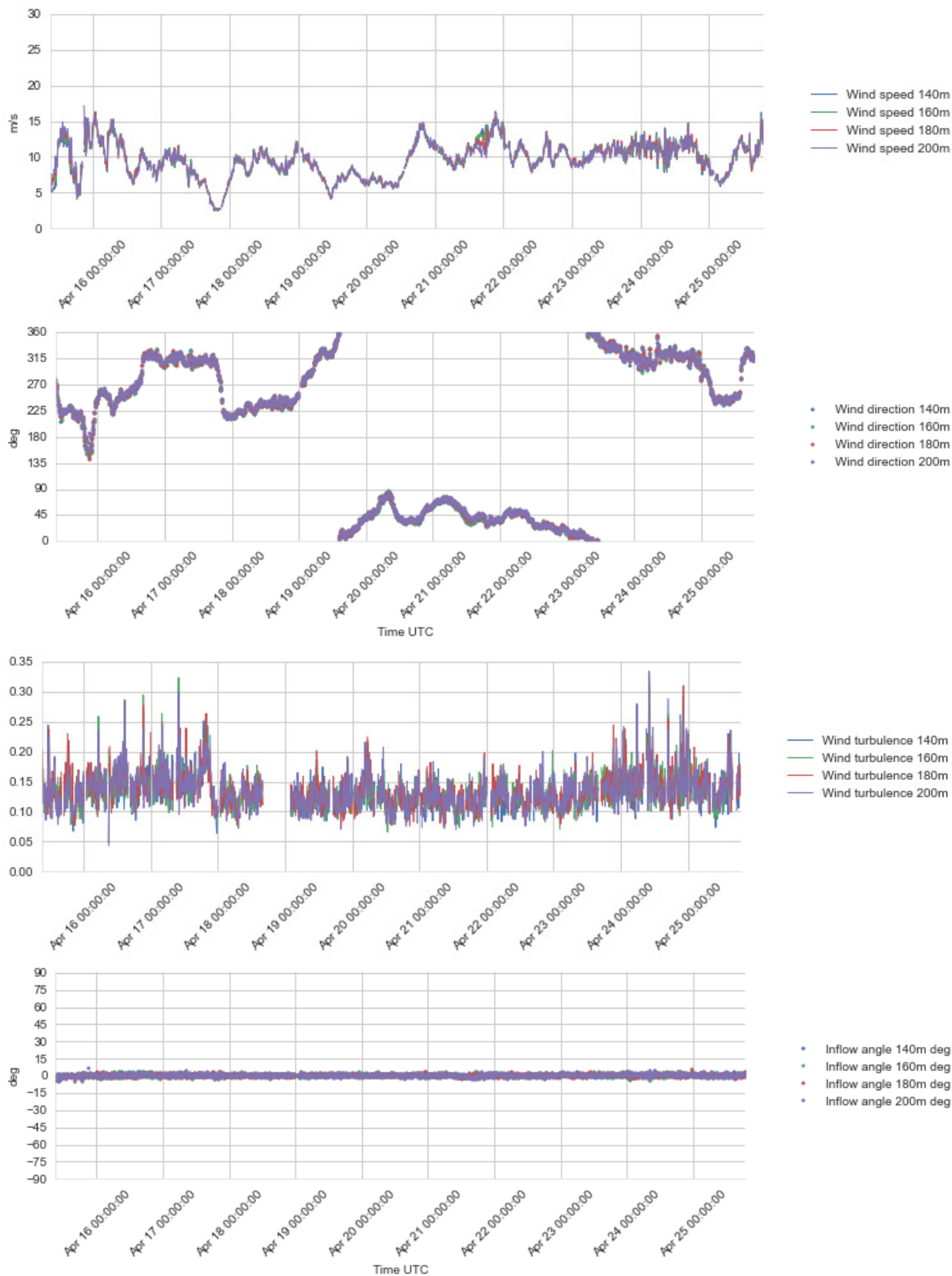
Figure 4.12 Plots of wind profile data, 140 – 200 m a.s.l., 15 – 25 Apr 2016.
