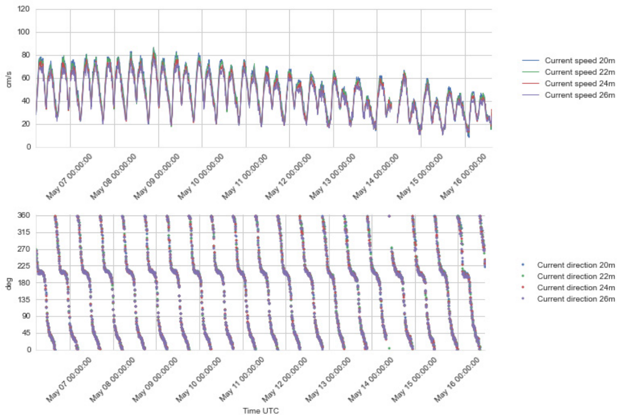
Figure 4.29 Time series plots of current speed (upper) and direction (lower panel), 20 - 26 m depth, 6 - 16 May 2016.
