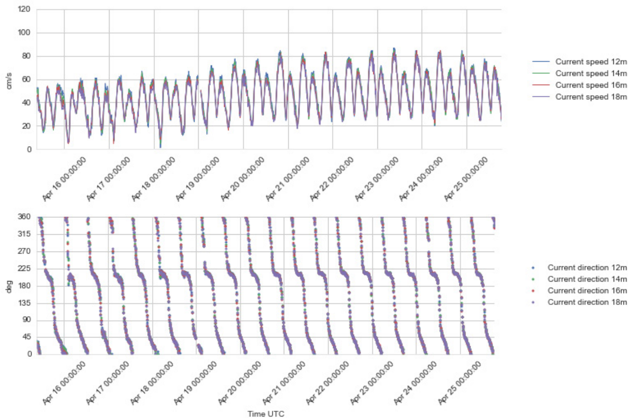
Figure 4.20 Time series plots of current speed (upper) and direction (lower panel), 12 - 18 m depth, 15 – 25 Apr 2016.
