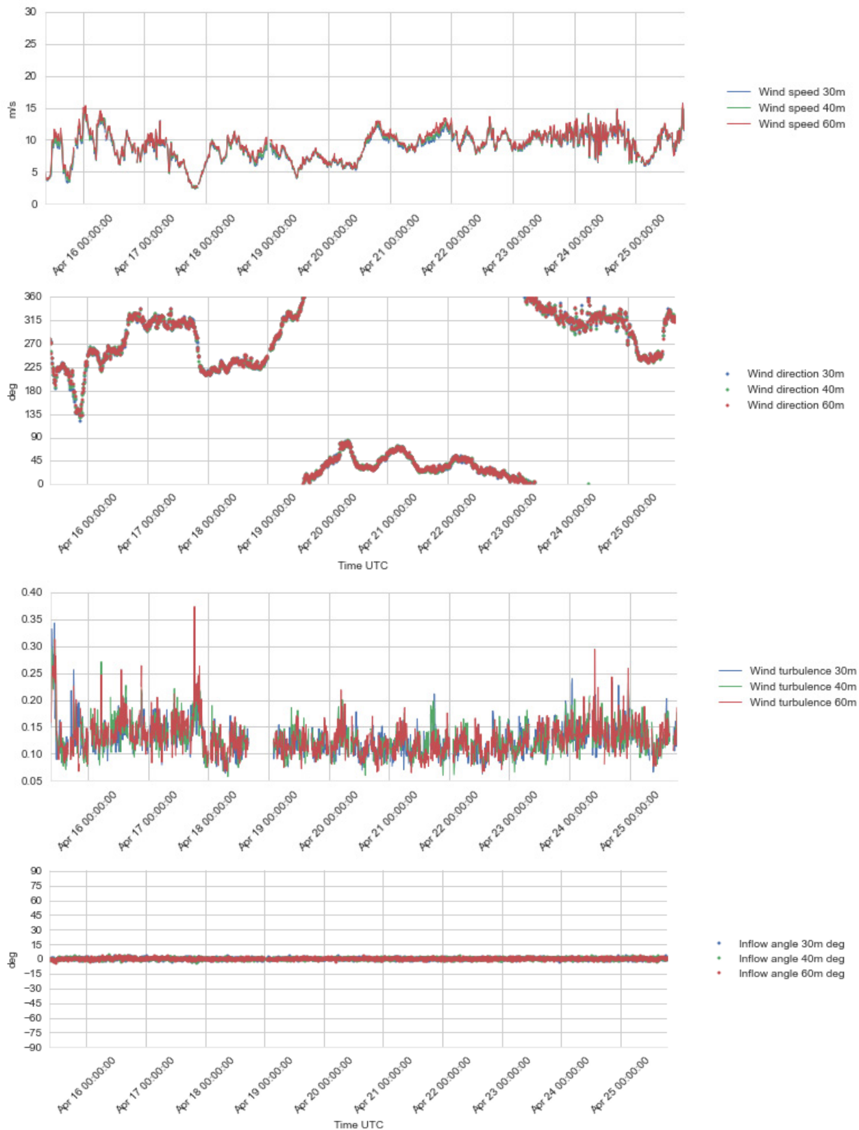
Figure 4.10 Plots of wind profile data, 30 – 60 m a.s.l., 15 – 25 Apr 2016.
