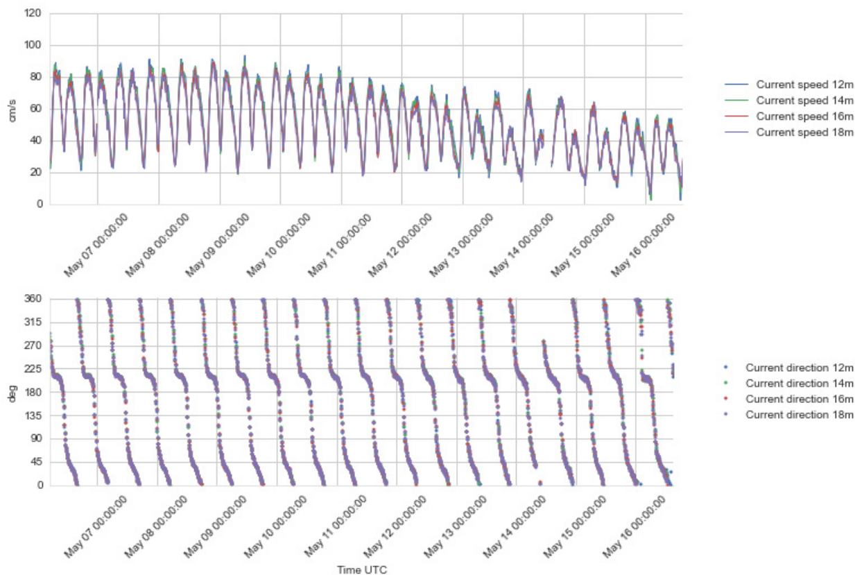
Figure 4.28 Time series plots of current speed (upper) and direction (lower panel), 12 - 18 m depth, 6 - 16 May 2016.
