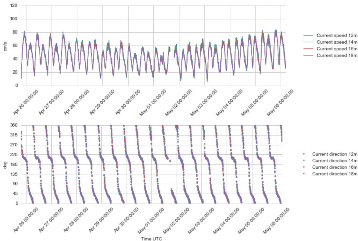
Figure 4.24 Time series plots of current speed (upper) and direction (lower panel), 12 -18 m depth, 25 Apr – 6 May 2016.
