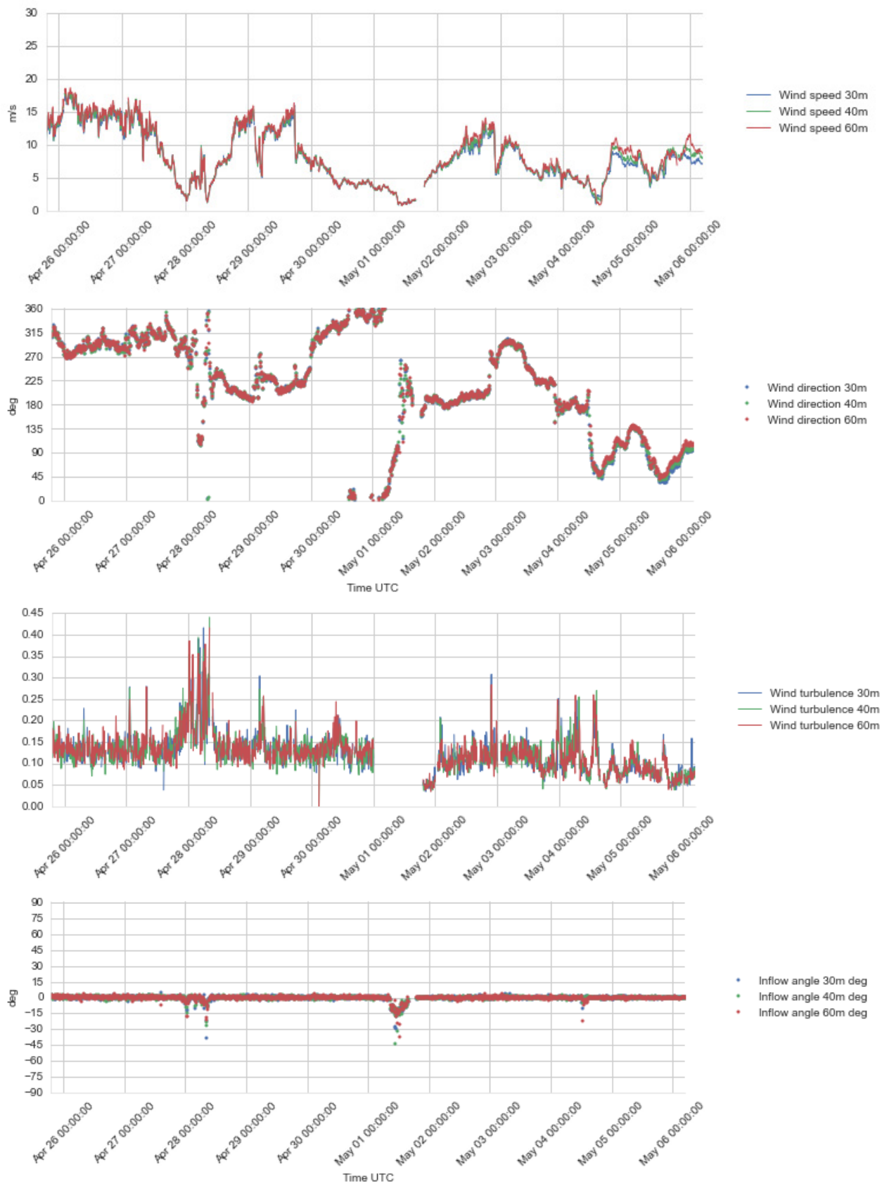
Figure 4.13 Plots of wind profile data, 30 – 60 m a.s.l., 25 Apr – 6 May 2016. From top to bottom: Wind speed, Wind direction, Turbulence Intensity, and Inflow Angle.
