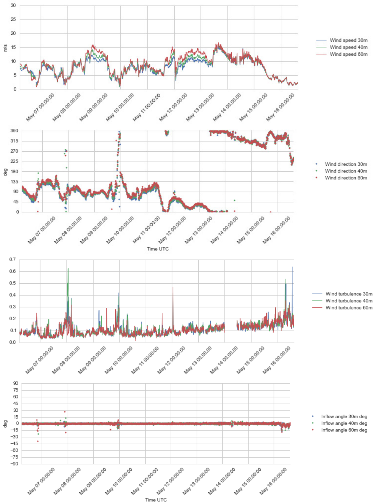
Figure 4.16 Plots of wind profile data, 30 – 60 m a.s.l., 6 - 16 May 2016.
