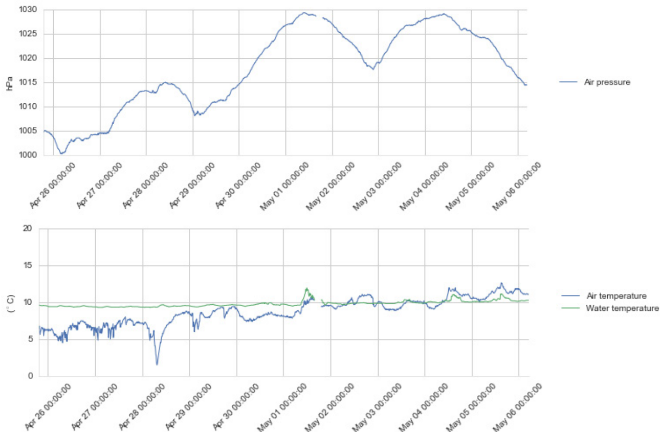
Figure 4.2 Time series plots of air pressure (upper panel), air and water temperature (lower panel), 25 Apr – 6 May 2016.
