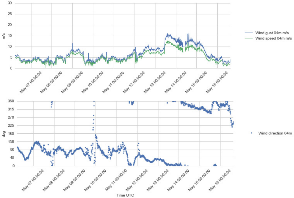
Figure 4.9 Plots of wind speed and gust (upper), and wind direction (lower) at 4 m a.s.l., 6 - 16 May 2016.
