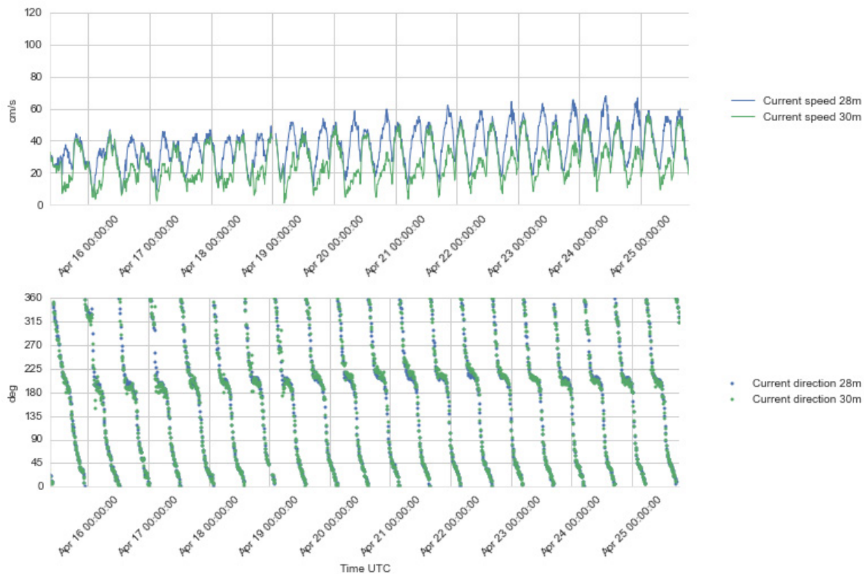
Figure 4.22 Time series plots of current speed (upper) and direction (lower panel), 28 - 30 m depth, 15 – 25 Apr 2016.
