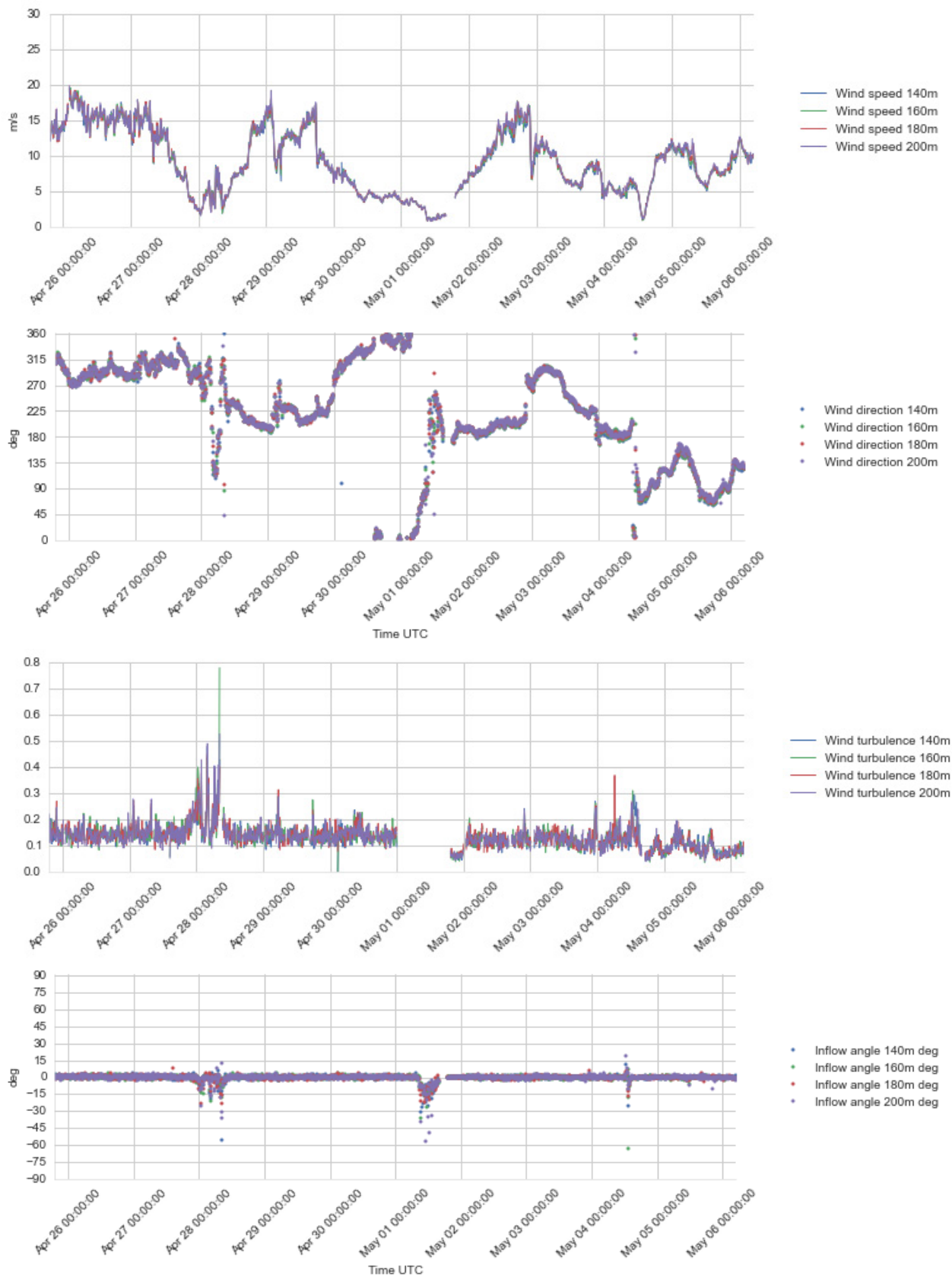
Figure 4.15 Plots of wind profile data, 140 – 200 m a.s.l., 25 Apr – 6 May 2016.
