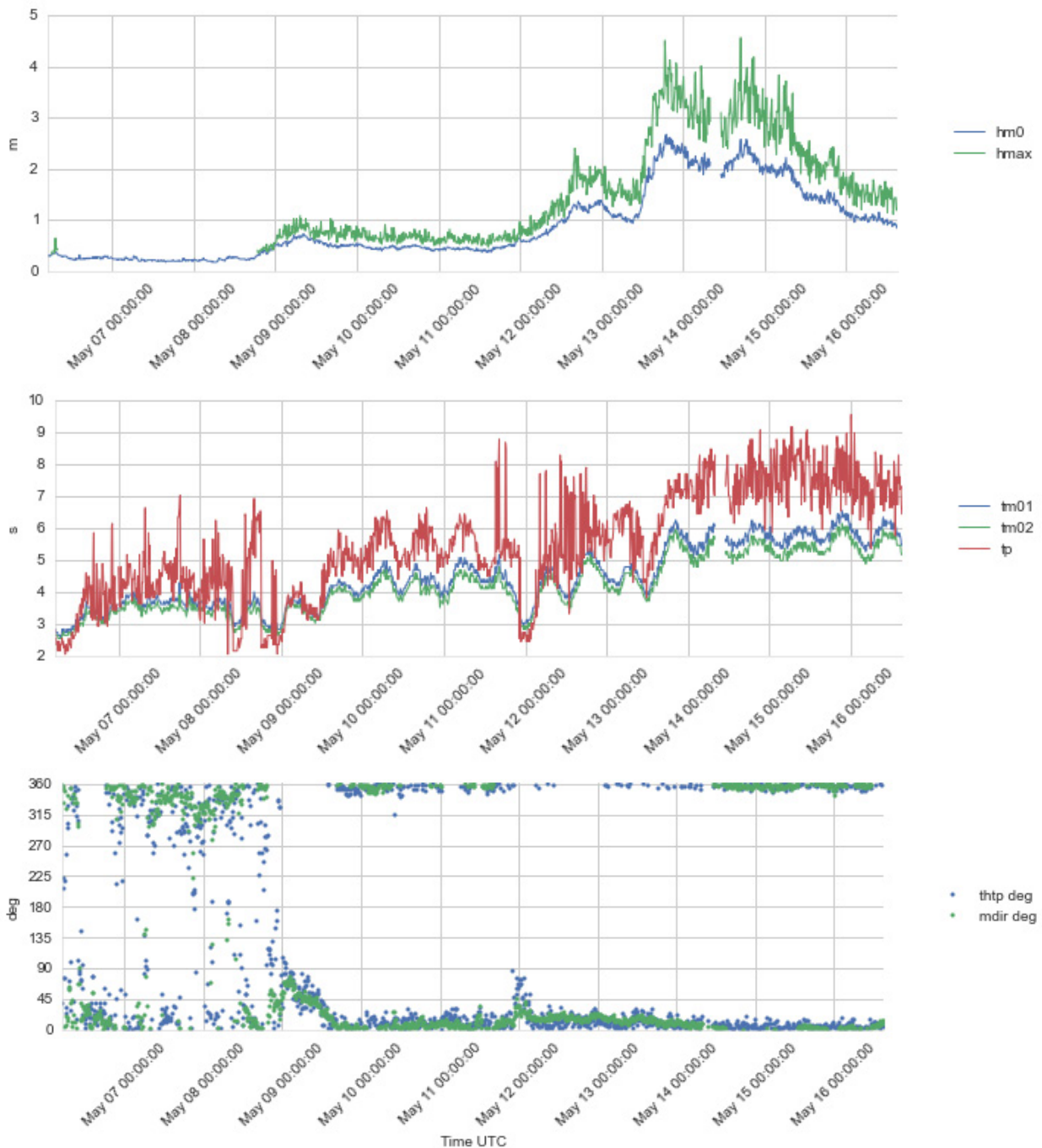
Figure 4.6 Time series plots of wave height ( H_{m0} and H_{max} ) (upper panel), wave period ( T_{m01} , T_{m02} and T_p ) (second panel), and wave direction ( ThTp and Mdir ) (lower panel), 6 - 16 May 2016.
