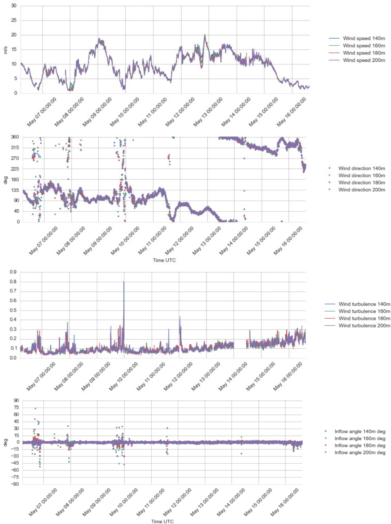
Figure 4.18 Plots of wind profile data, 140 – 200 m a.s.l., 6 - 16 May 2016.
