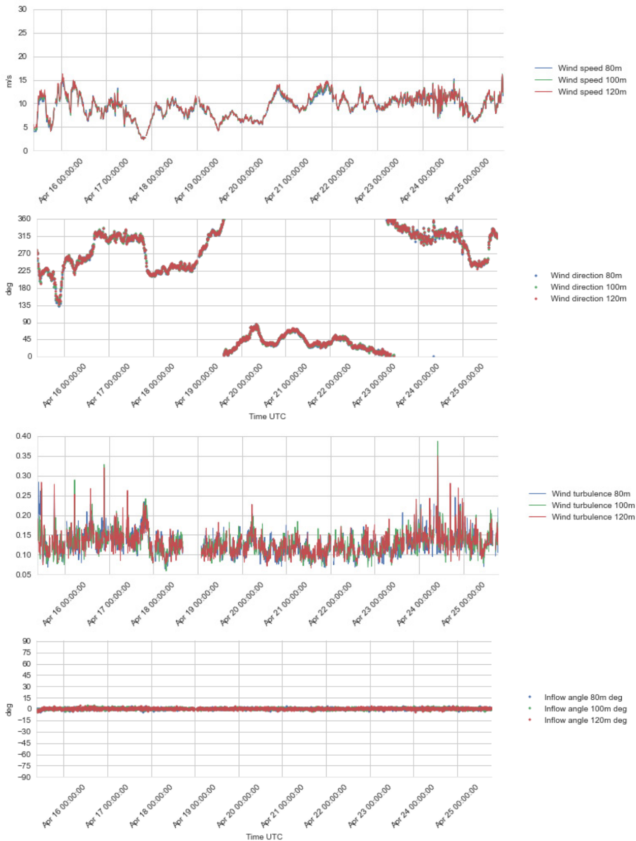
Figure 4.11 Plots of wind profile data, 80 – 120 m a.s.l., 15 – 25 Apr 2016.
