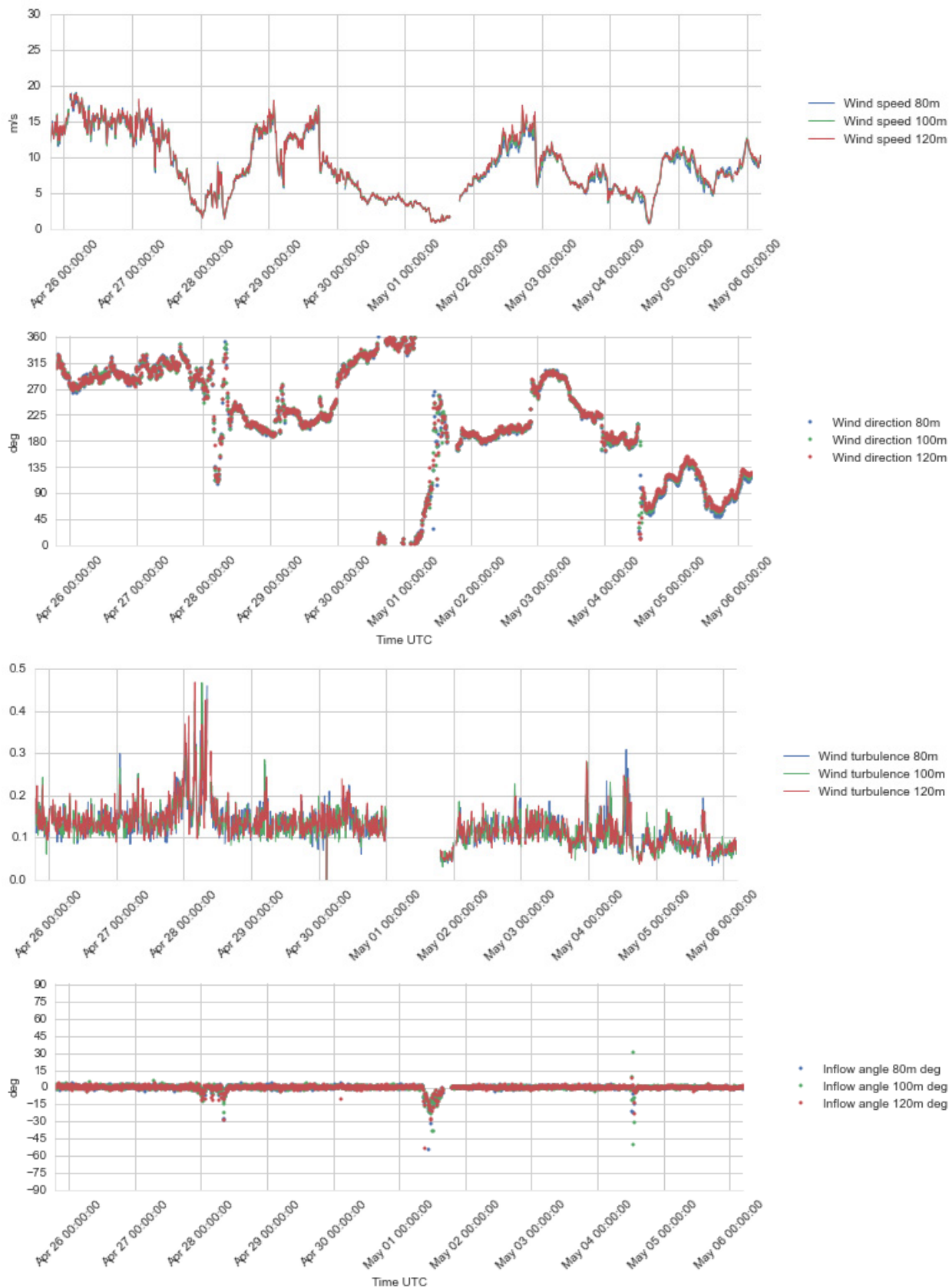
Figure 4.14 Plots of wind profile data, 80 – 120 m a.s.l., 25 Apr – 6 May 2016.
