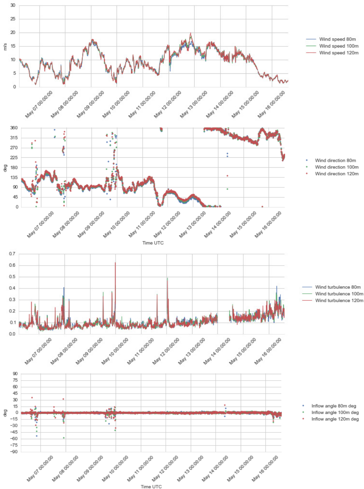
Figure 4.17 Plots of wind profile data, 80 – 120 m a.s.l., 6 - 16 May 2016.
