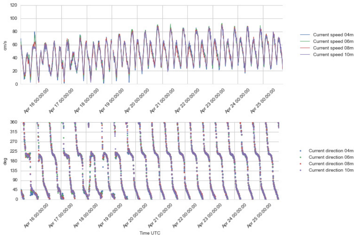
Figure 4.19 Time series plots of current speed (upper) and direction (lower panel), 4 - 10 m depth, 15 – 25 Apr 2016.
