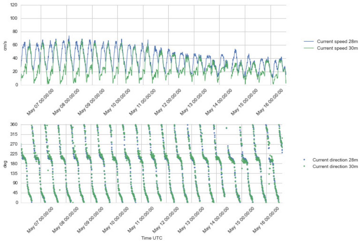
Figure 4.30 Time series plots of current speed (upper) and direction (lower panel), 28 - 30 m depth, 6 - 16 May 2016.
