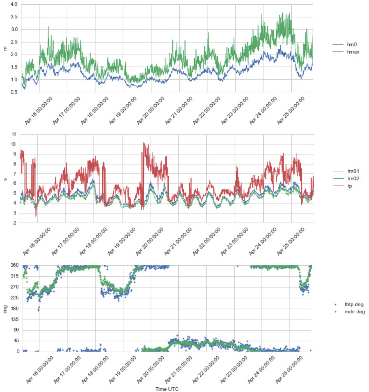
Figure 4.4 Time series plots of wave height ( H_{m0} and H_{max} ) (upper panel), wave period ( T_{m01} , T_{m02} and T_p ) (second panel), and wave direction ( \theta_{Htp} and M_{dir} ) (lower panel), 15 - 25 Apr 2016.
