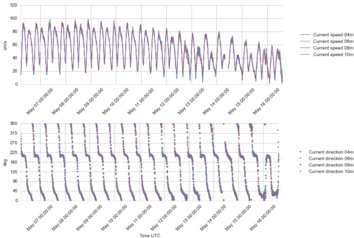
Figure 4.27 Time series plots of current speed (upper) and direction (lower panel), 4 - 10 m depth, 6 - 16 May 2016.
