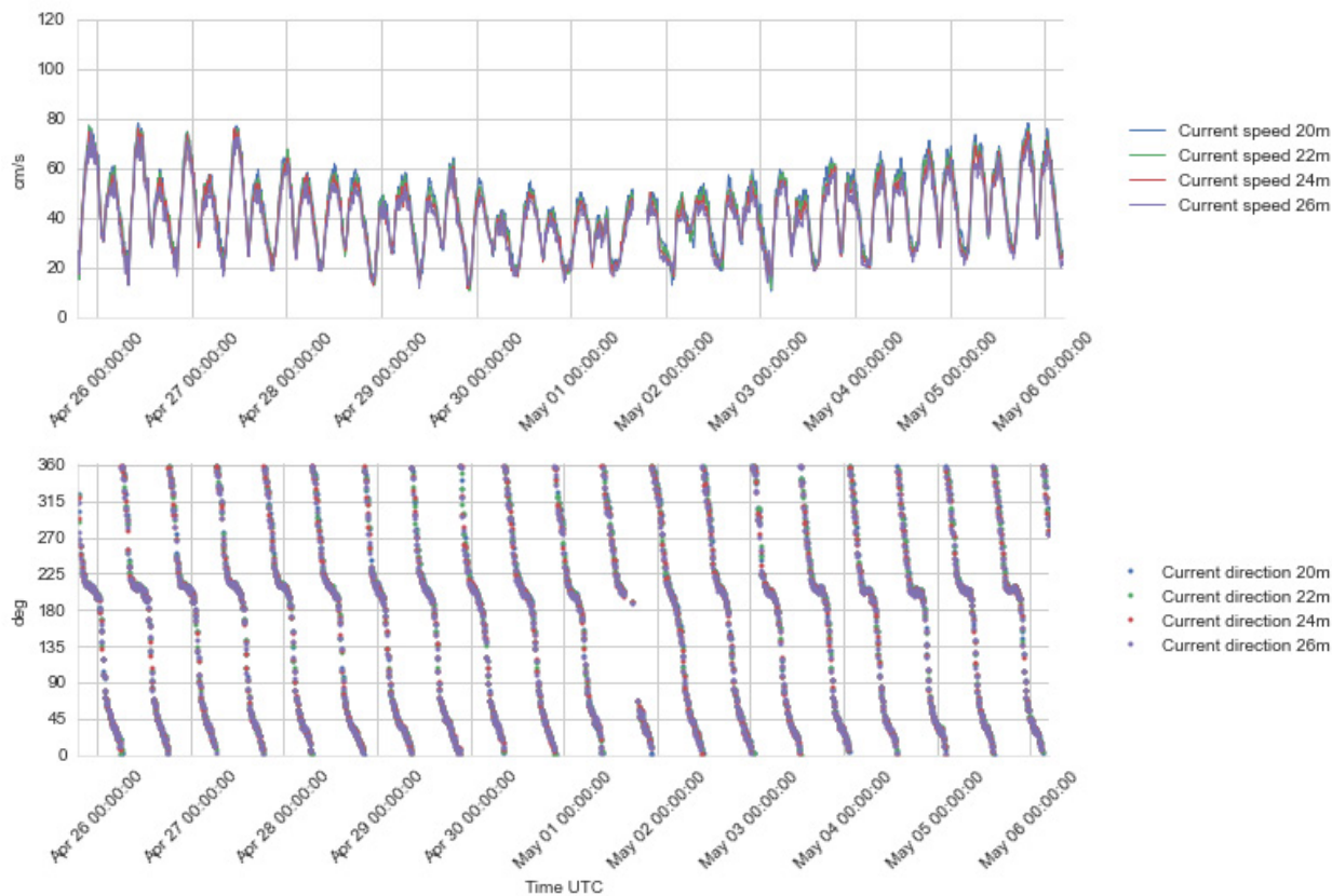
Figure 4.25 Time series plots of current speed (upper) and direction (lower panel), 20 – 26 m depth, 25 Apr – 6 May 2016.
