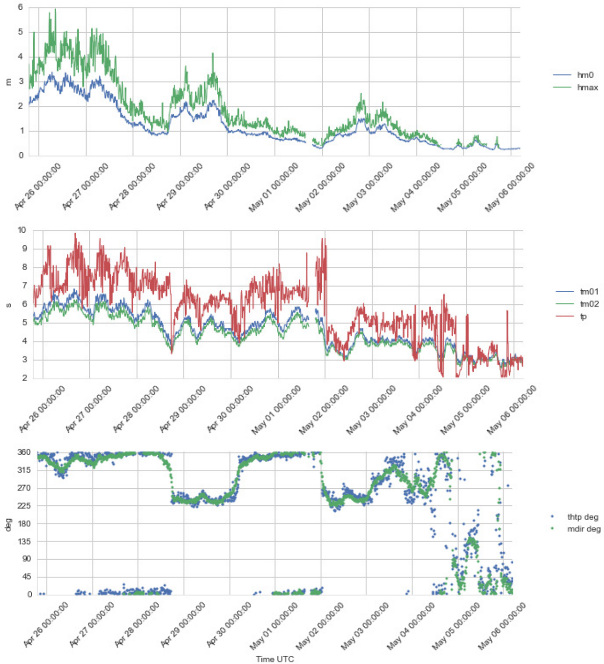
Figure 4.5 Time series plots of wave height ( H_{m0} and H_{max} ) (upper panel), wave period ( T_{m01} , T_{m02} and T_p ) (second panel), and wave direction ( ThTp and Mdir ) (lower panel), 25 Apr – 6 May 2016.
