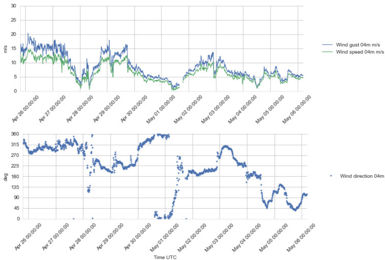
Figure 4.8 Plots of wind speed and gust (upper), and wind direction (lower) at 4 m a.s.l., 25 Apr – 6 May 2016.
