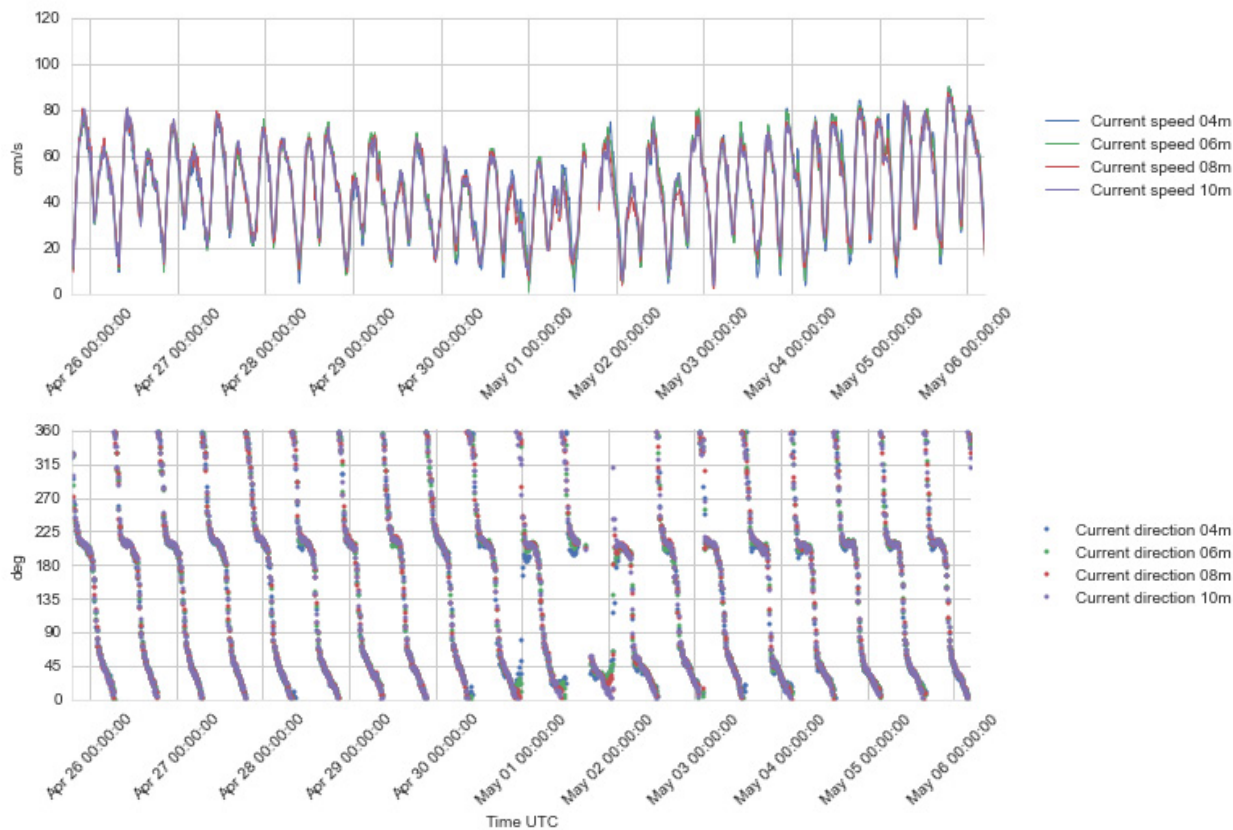
Figure 4.23 Time series plots of current speed (upper) and direction (lower panel), 4 - 10 m depth, 25 Apr – 6 May 2016.
