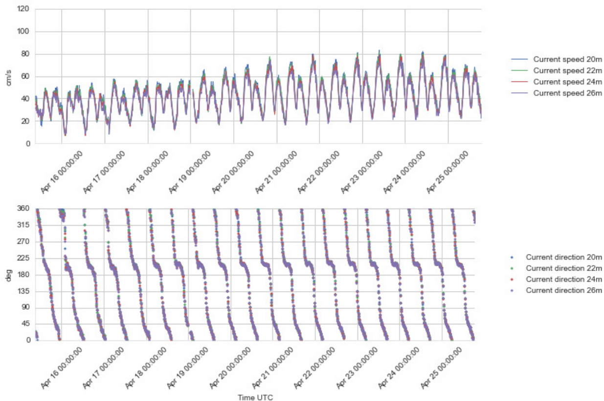
Figure 4.21 Time series plots of current speed (upper) and direction (lower panel), 20 - 26 m depth, 15 – 25 Apr 2016.
