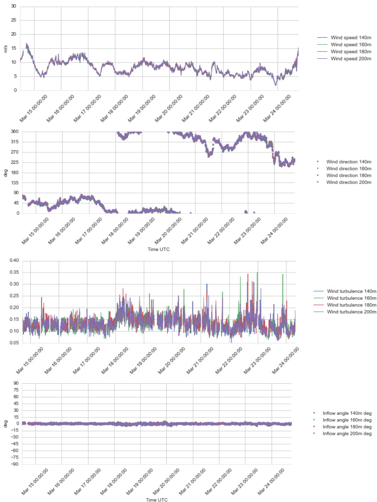
Figure 4.12 Plots of wind profile data, 140 – 200 m a.s.l., 14 - 24 Mar 2016.
