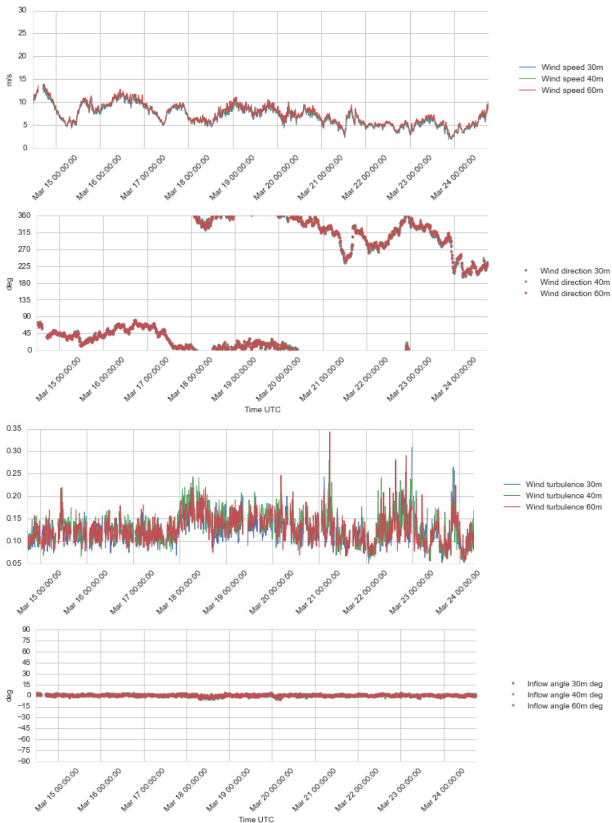
Figure 4.10 Plots of wind profile data, 30 – 60 m a.s.l., 14 - 24 Mar 2016.
