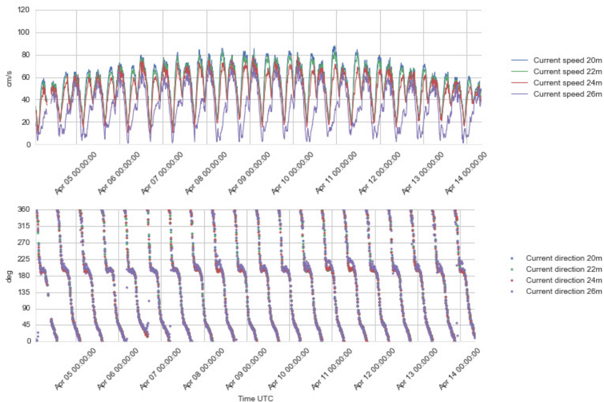
Figure 4.27 Time series plots of current speed (upper) and direction (lower panel), 20 - 26 m depth, 4 – 14 Apr 2016.
