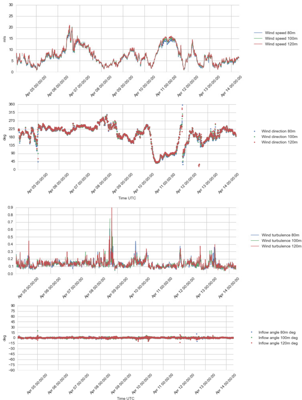
Figure 4.17 Plots of wind profile data, 80 – 120 m a.s.l., 4 – 14 Apr 2016.
