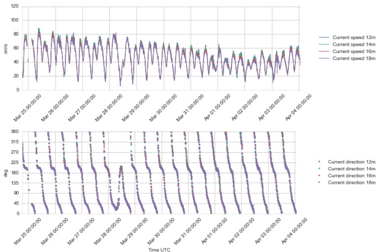
Figure 4.23 Time series plots of current speed (upper) and direction (lower panel), 12 -18 m depth, 24 Mar – 4 Apr 2016.
