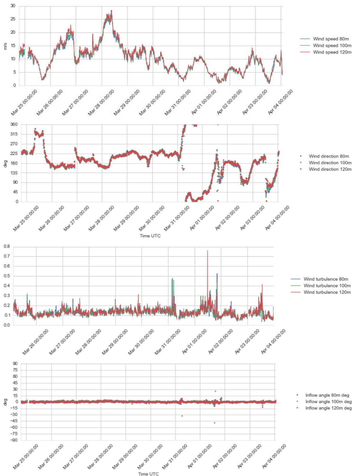
Figure 4.14 Plots of wind profile data, 80 – 120 m a.s.l., 24 Mar – 4 Apr 2016.
