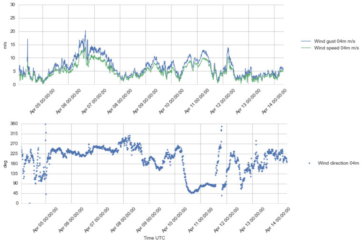
Figure 4.9 Plots of wind speed and gust (upper), and wind direction (lower) at 4 m a.s.l., 4 - 14 Apr 2016.
