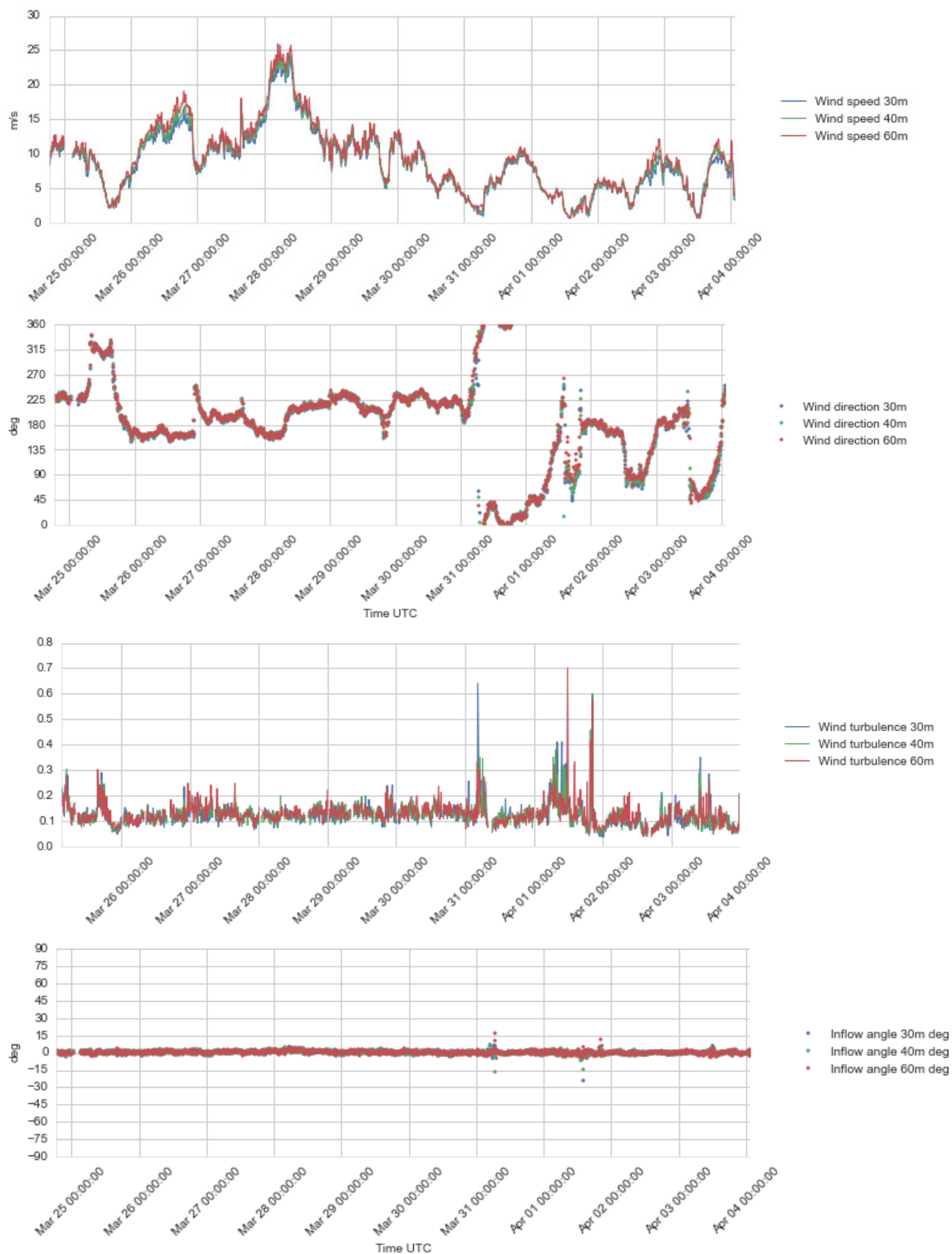
Figure 4.13 Plots of wind profile data, 30 – 60 m a.s.l., 24 Mar – 4 Apr 2016.
