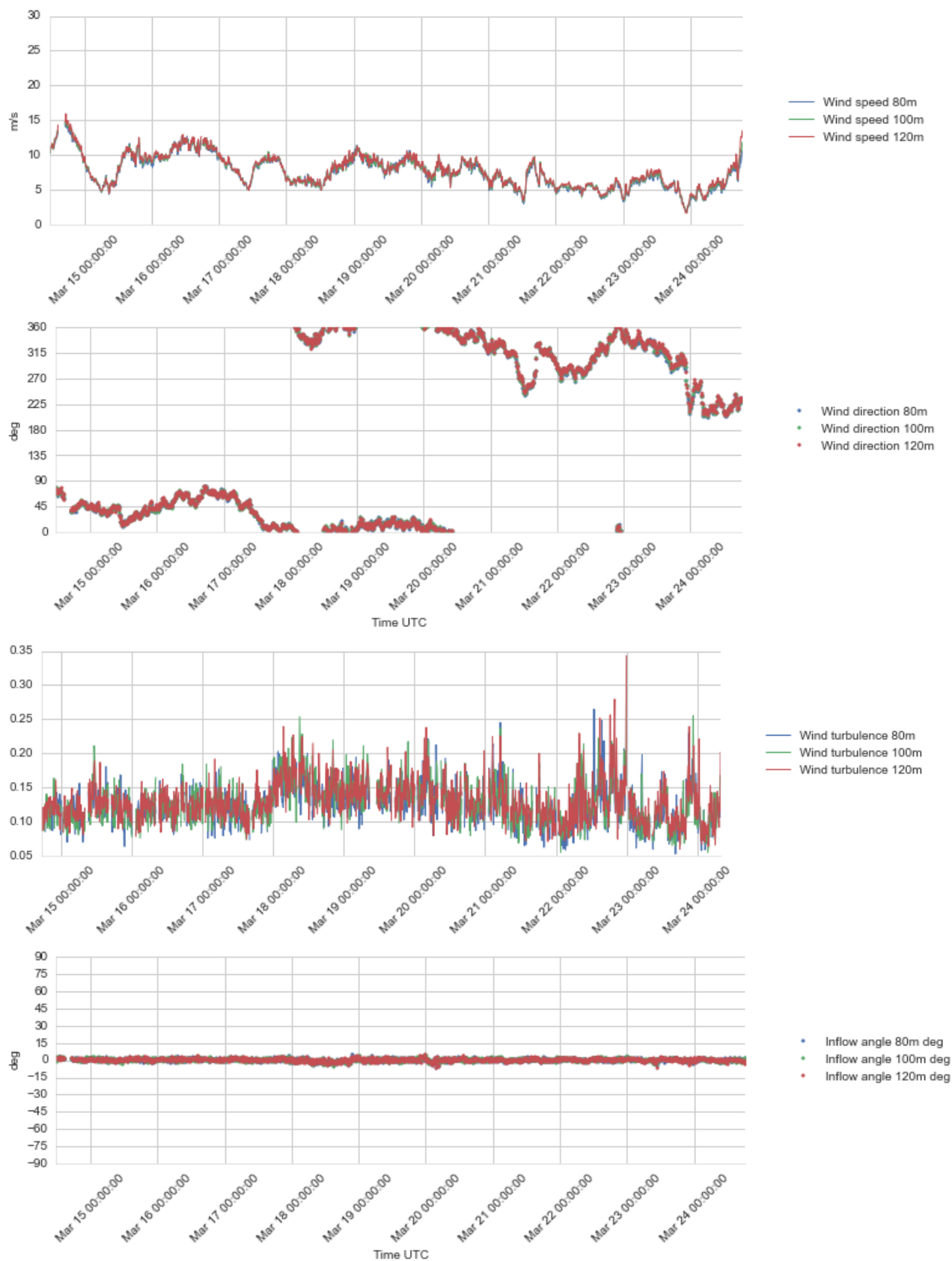
Figure 4.11 Plots of wind profile data, 80 – 120 m a.s.l., 14 - 24 Mar 2016.
