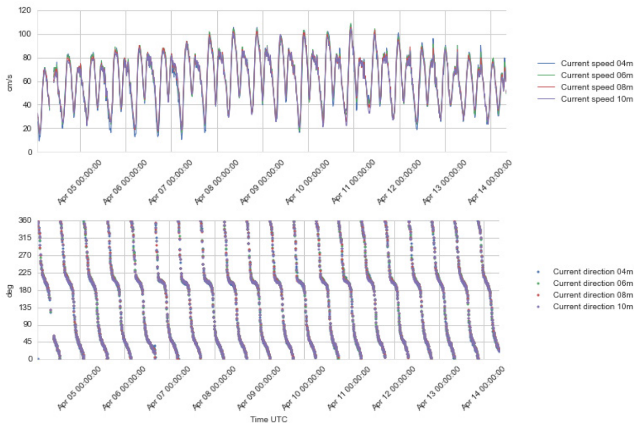
Figure 4.25 Time series plots of current speed (upper) and direction (lower panel), 4 – 10 m depth, 4 – 14 Apr 2016.
