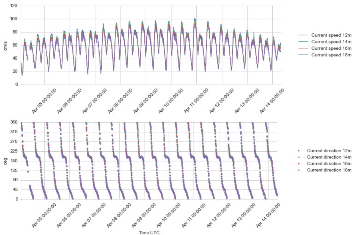
Figure 4.26 Time series plots of current speed (upper) and direction (lower panel), 12 - 18 m depth, 4 – 14 Apr 2016.
