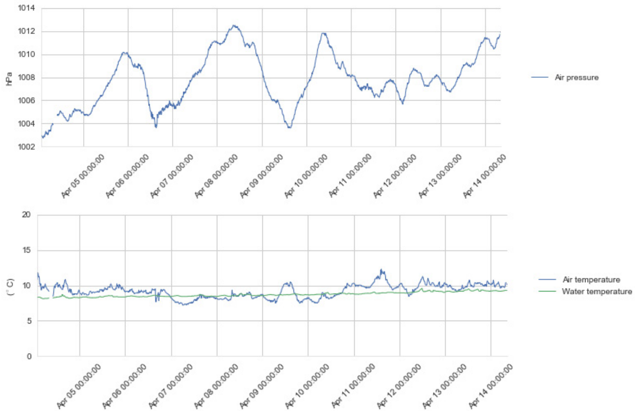
Figure 4.3 Time series plots of air pressure (upper panel), air and water temperature (lower panel), 4 - 14 Apr 2016.
