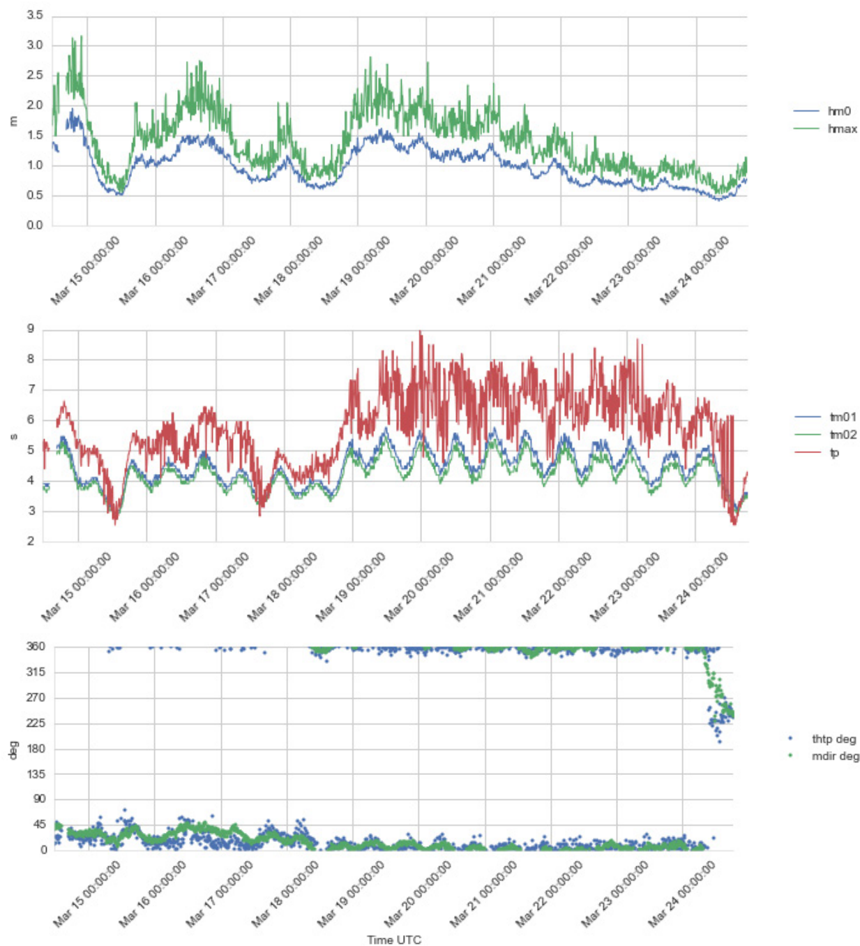
Figure 4.4 Time series plots of wave height ( H_{m0} and H_{max} ) (upper panel), wave period ( T_{m01} , T_{m02} and T_p ) (second panel), and wave direction ( ThTp and Mdir ) (lower panel), 14 - 24 Mar 2016.
