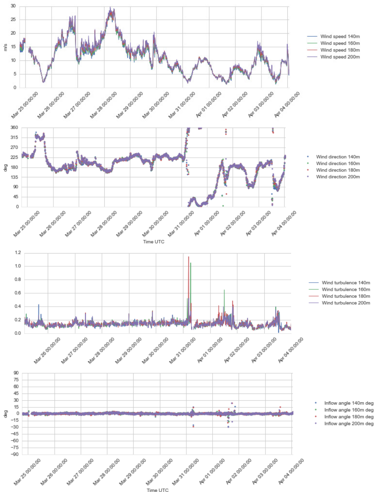
Figure 4.15 Plots of wind profile data, 140 – 200 m a.s.l., 24 Mar – 4 Apr 2016.
