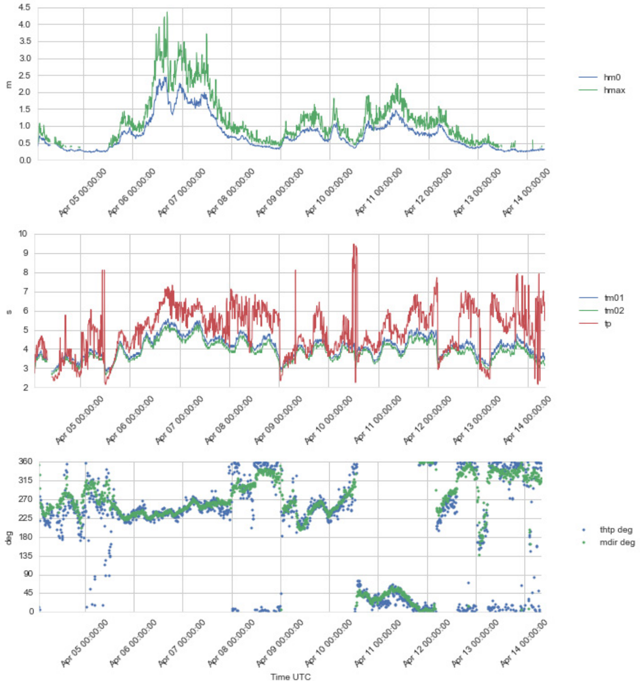
Figure 4.6 Time series plots of wave height (Hm0 and Hmax) (upper panel), wave period (Tm01, Tm02 and Tp) (second panel), and wave direction (ThTp and Mdir) (lower panel), 4 - 14 Apr 2016.
