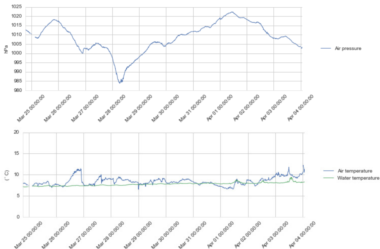
Figure 4.2 Time series plots of air pressure (upper panel), air and water temperature (lower panel), 24 Mar – 4 Apr 2016.
