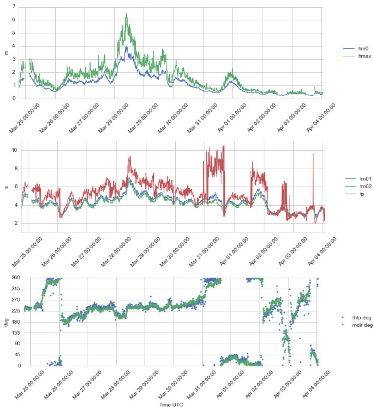
Figure 4.5 Time series plots of wave height ( H_{m0} and H_{max} ) (upper panel), wave period ( T_{m01} , T_{m02} and T_p ) (second panel), and wave direction ( ThTp and Mdir ) (lower panel), 24 Mar – 4 Apr 2016.
