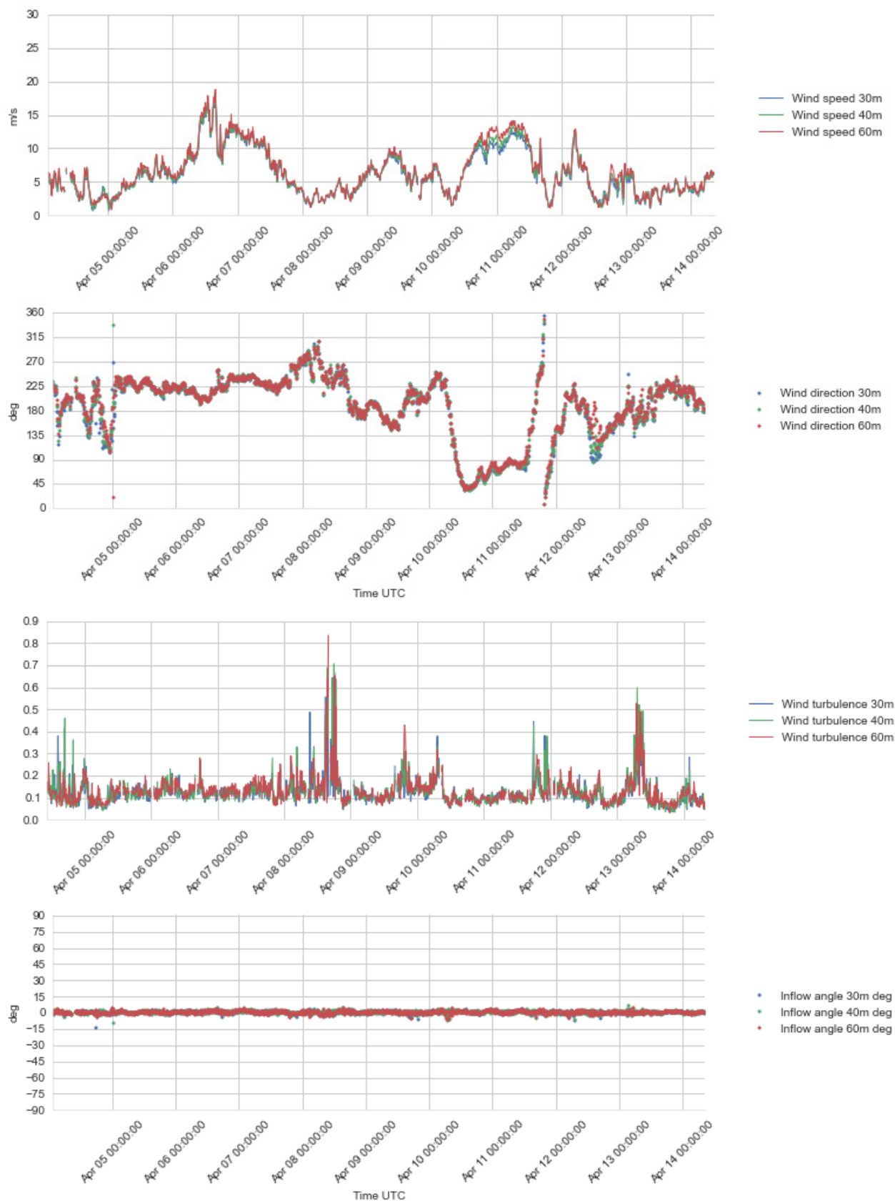
Figure 4.16 Plots of wind profile data, 30 – 60 m a.s.l., 4 – 14 Apr 2016.
