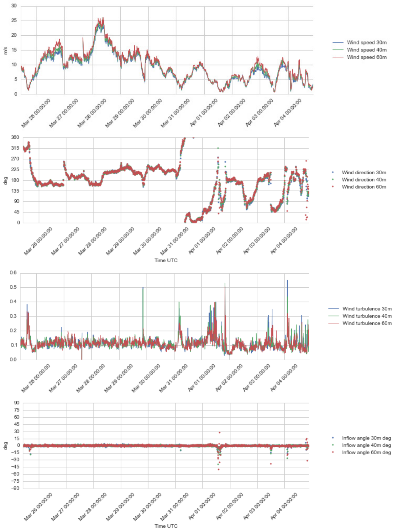
Figure 4.13 Plots of wind profile data, 30 – 60 m a.s.l., 25 Mar – 4 Apr 2016.
