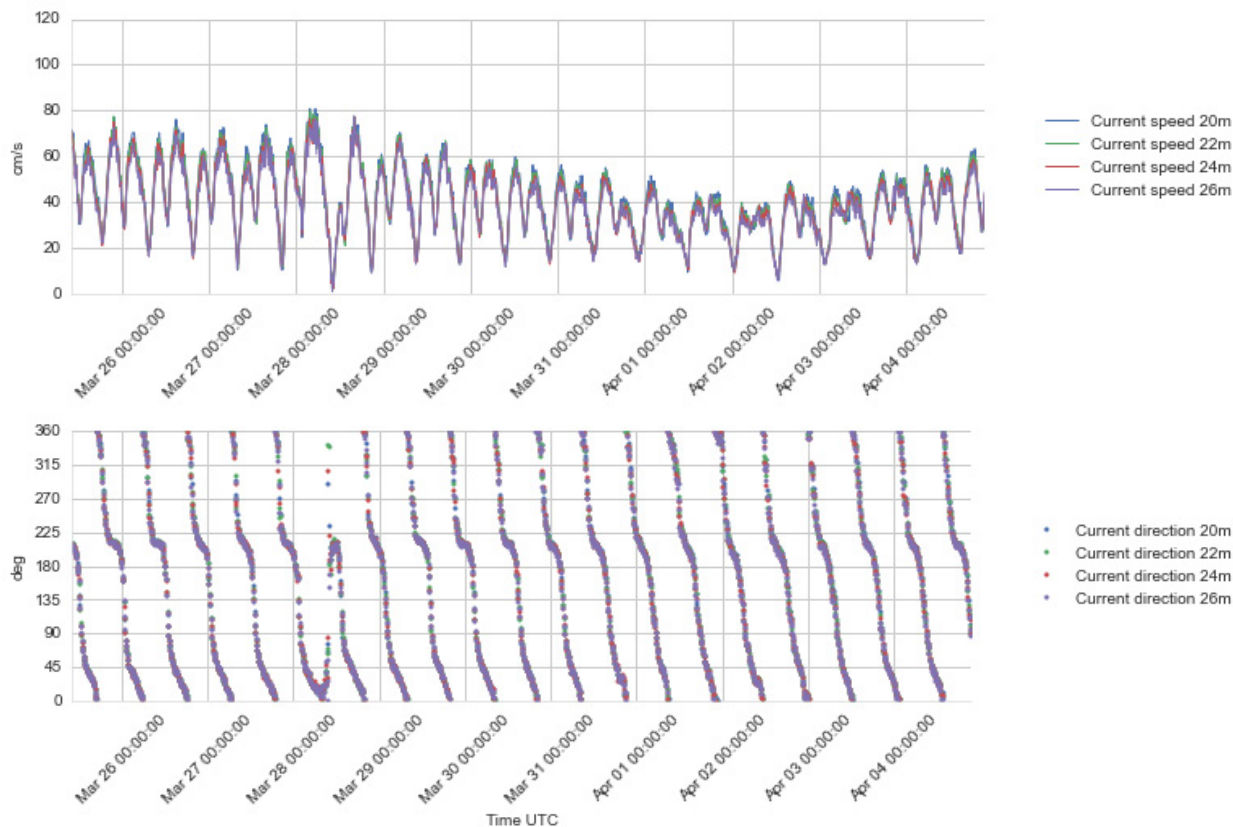
Figure 4.25 Time series plots of current speed (upper) and direction (lower panel), 20 – 26 m depth, 25 Mar – 4 Apr 2016.
