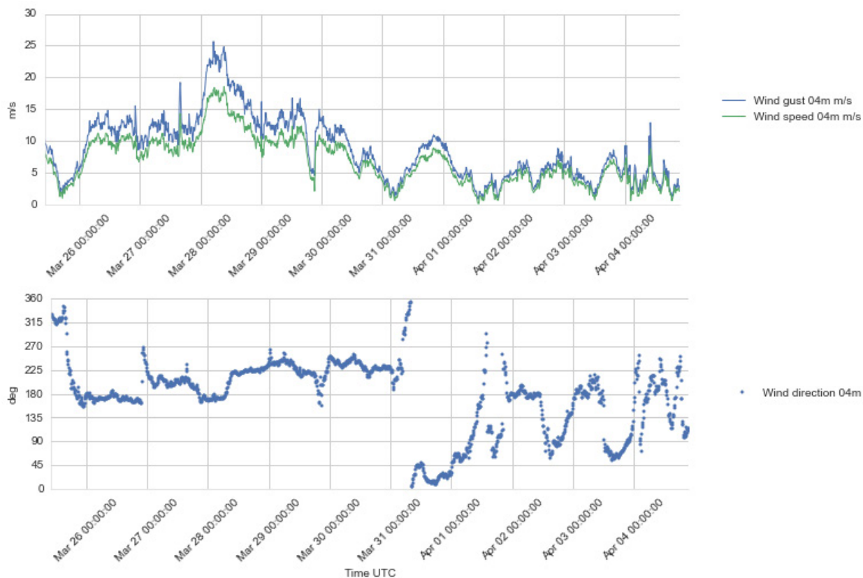
Figure 4.8 Plots of wind speed and gust (upper), and wind direction (lower) at 4 m a.s.l., 25 Mar – 4 Apr 2016.
