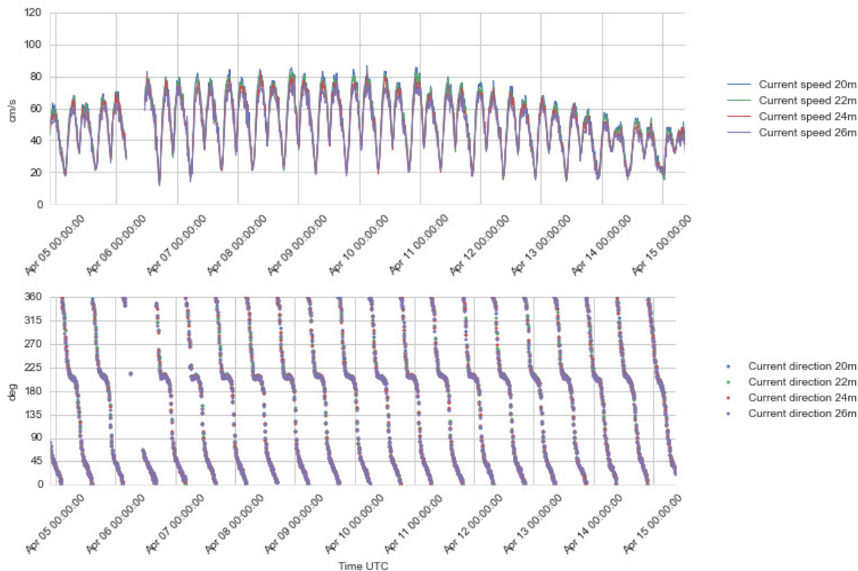
Figure 4.29 Time series plots of current speed (upper) and direction (lower panel), 20 - 26 m depth, 4 - 15 Apr 2016.
