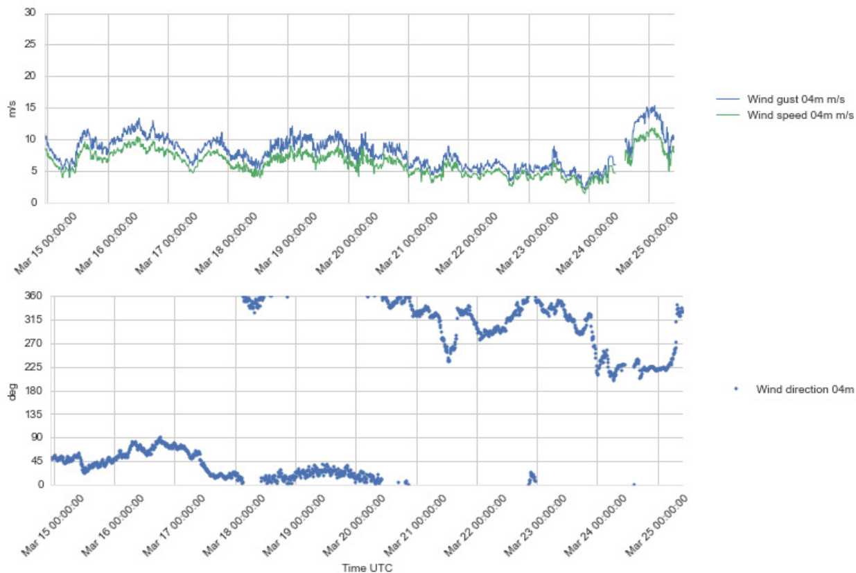
Figure 4.7 Plots of wind speed and gust (upper), and wind direction (lower) at 4 m a.s.l., 14 – 25 Mar 2016.
