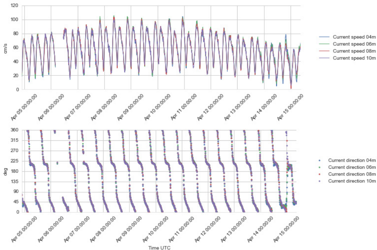
Figure 4.27 Time series plots of current speed (upper) and direction (lower panel), 4 - 10 m depth, 4 - 15 Apr 2016.
