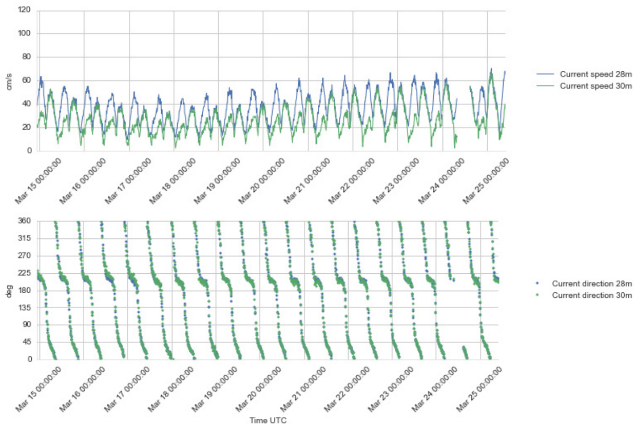
Figure 4.22 Time series plots of current speed (upper) and direction (lower panel), 28 - 30 m depth, 14 – 25 Mar 2016.
