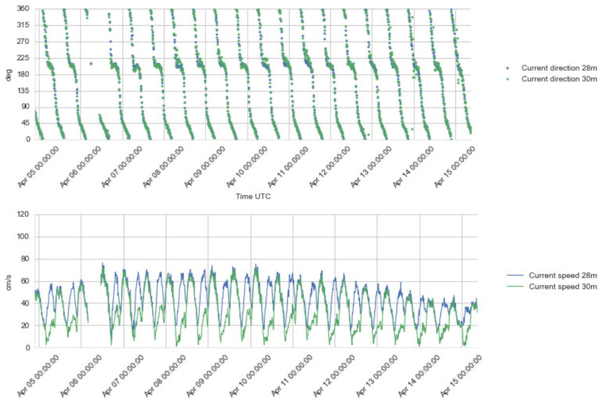
Figure 4.30 Time series plots of current speed (upper) and direction (lower panel), 28 - 30 m depth, 4 - 15 Apr 2016.
