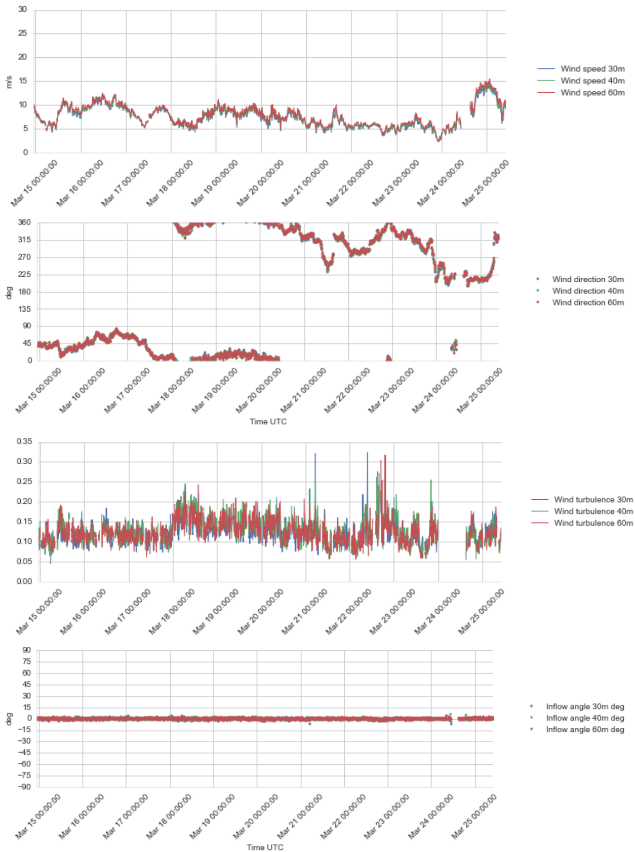
Figure 4.10 Plots of wind profile data, 30 – 60 m a.s.l., 14 – 25 Mar 2016. From top to bottom: Wind speed, Wind direction, Turbulence Intensity, and Inflow Angle.
