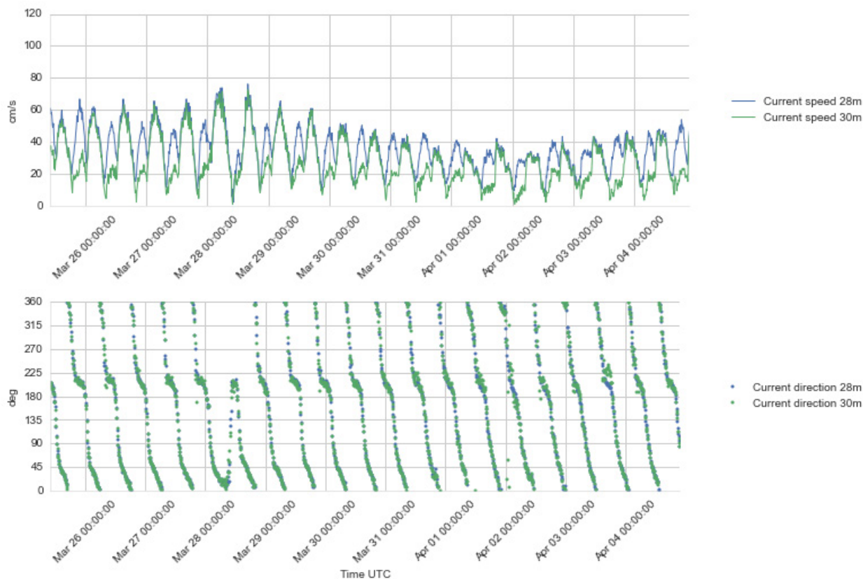
Figure 4.26 Time series plots of current speed (upper) and direction (lower panel), 28 – 30 m depth, 25 Mar – 4 Apr 2016.
