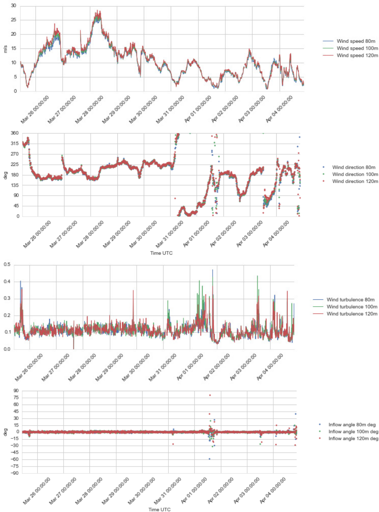
Figure 4.14 Plots of wind profile data, 80 – 120 m a.s.l., 25 Mar – 4 Apr 2016.
