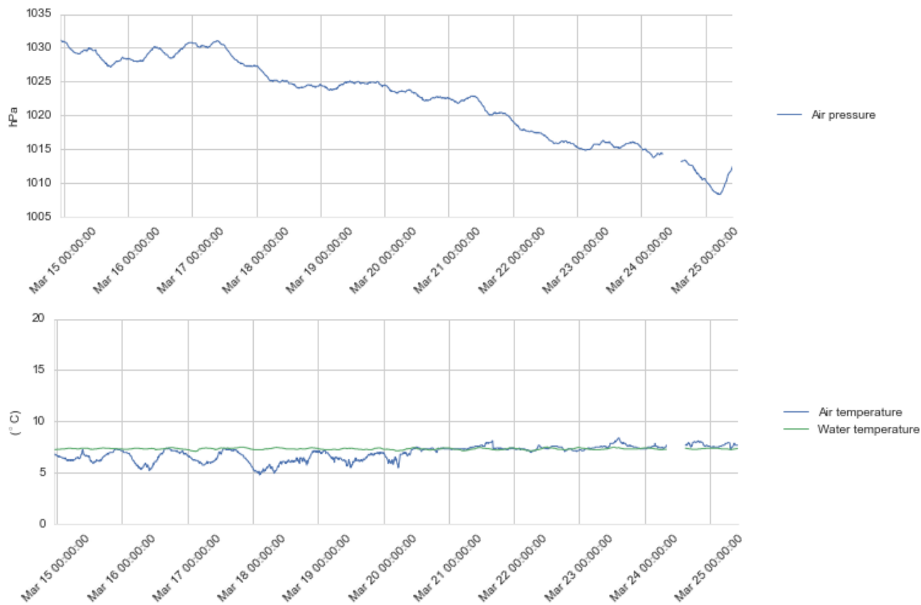
Figure 4.1 Time series plots of air pressure (upper panel), air and water temperature (lower panel), 14 - 25 Mar 2016.
