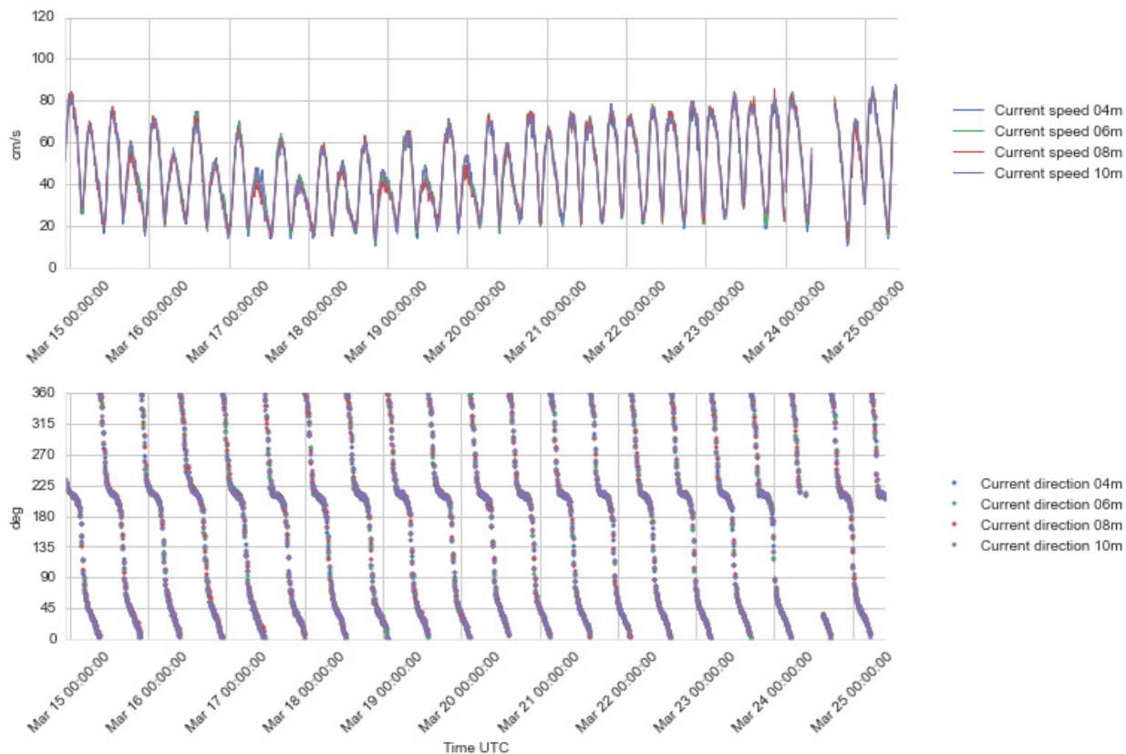
Figure 4.19 Time series plots of current speed (upper) and direction (lower panel), 4 - 10 m depth, 14 – 25 Mar 2016.
