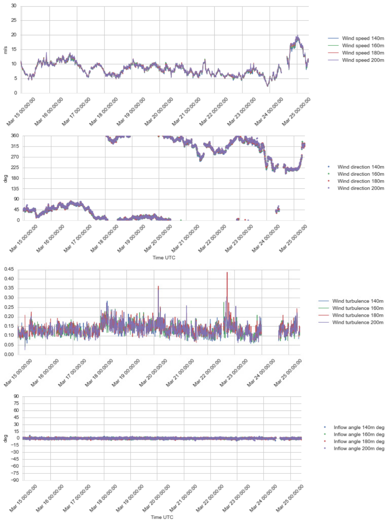
Figure 4.12 Plots of wind profile data, 140 – 200 m a.s.l., 14 – 25 Mar 2016.
