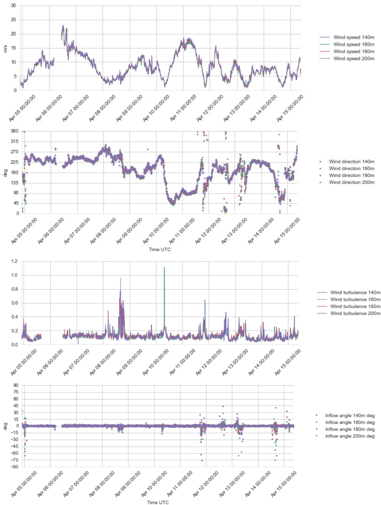
Figure 4.18 Plots of wind profile data, 140 – 200 m a.s.l., 4 - 15 Apr 2016.
