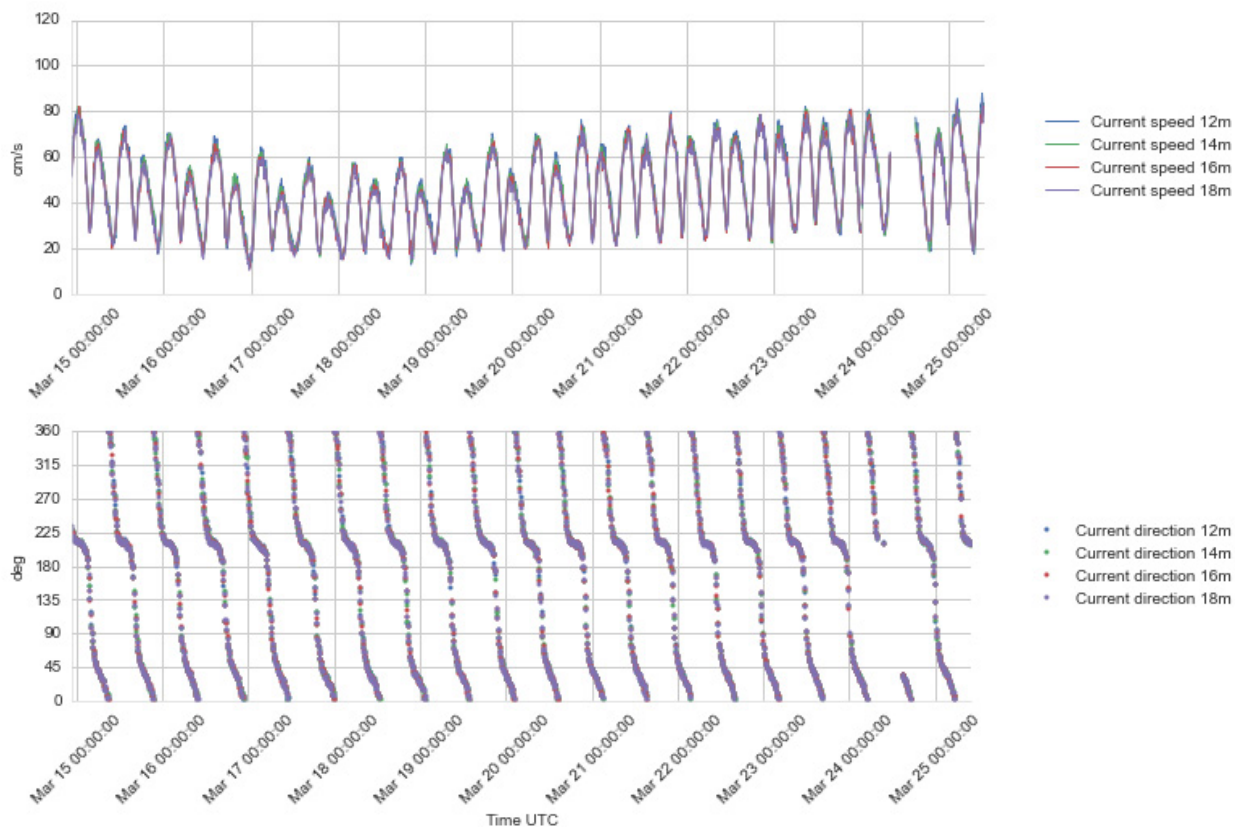
Figure 4.20 Time series plots of current speed (upper) and direction (lower panel), 12 - 18 m depth, 14 – 25 Mar 2016.
