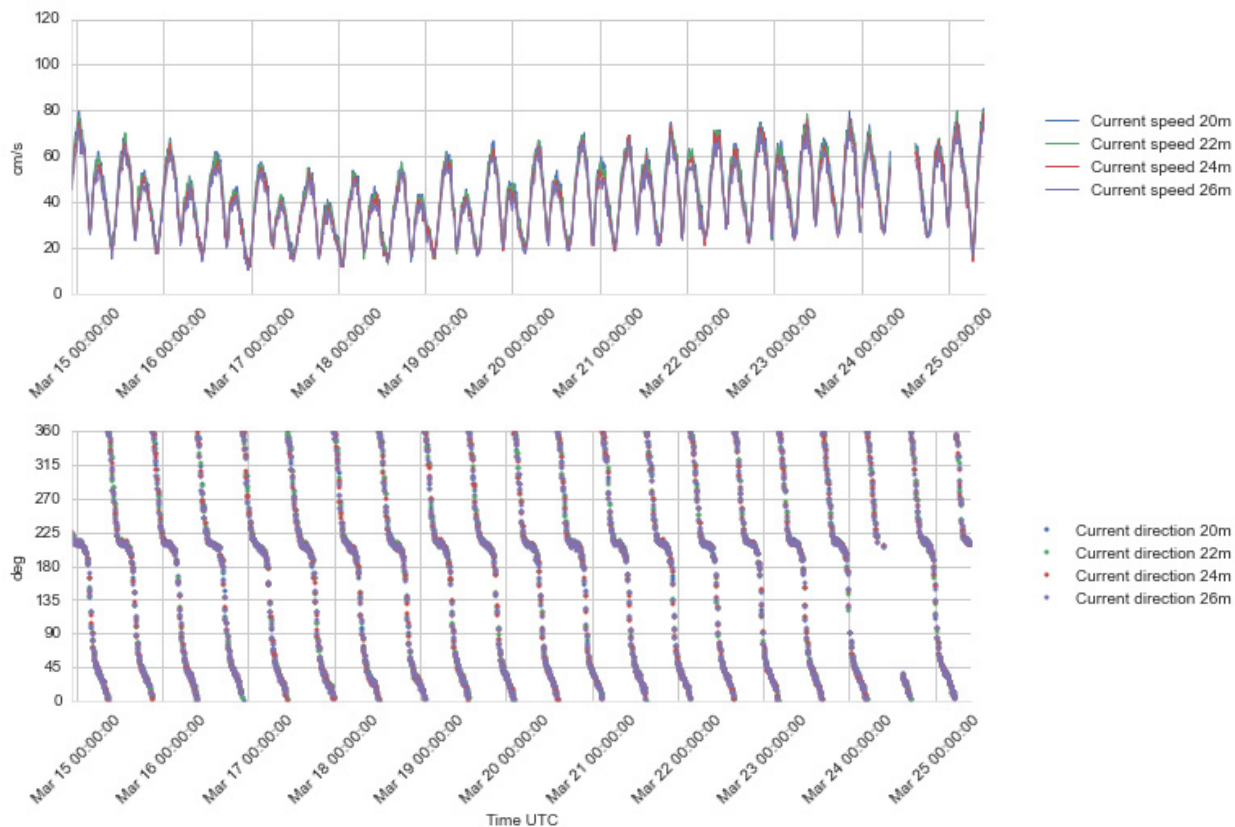
Figure 4.21 Time series plots of current speed (upper) and direction (lower panel), 20 - 26 m depth, 14 – 25 Mar 2016.
