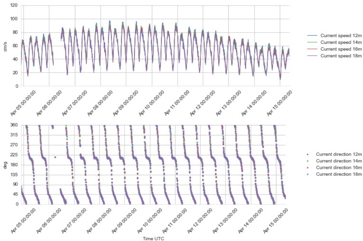
Figure 4.28 Time series plots of current speed (upper) and direction (lower panel), 12 - 18 m depth, 4 - 15 Apr 2016.
