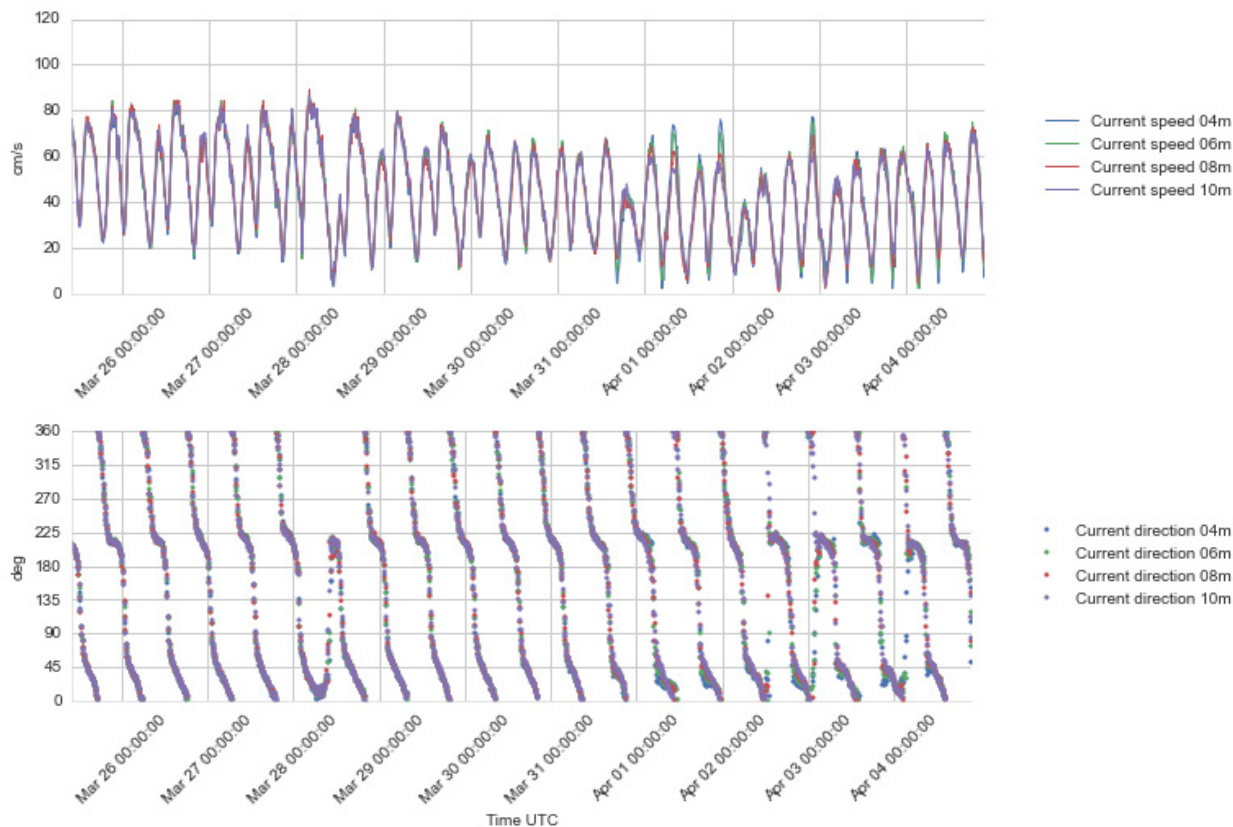
Figure 4.23 Time series plots of current speed (upper) and direction (lower panel), 4 - 10 m depth, 25 Mar – 4 Apr 2016.
