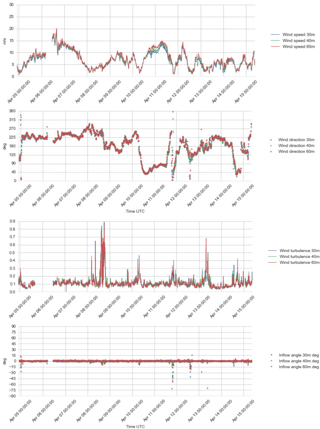
Figure 4.16 Plots of wind profile data, 30 – 60 m a.s.l., 4 - 15 Apr 2016.
