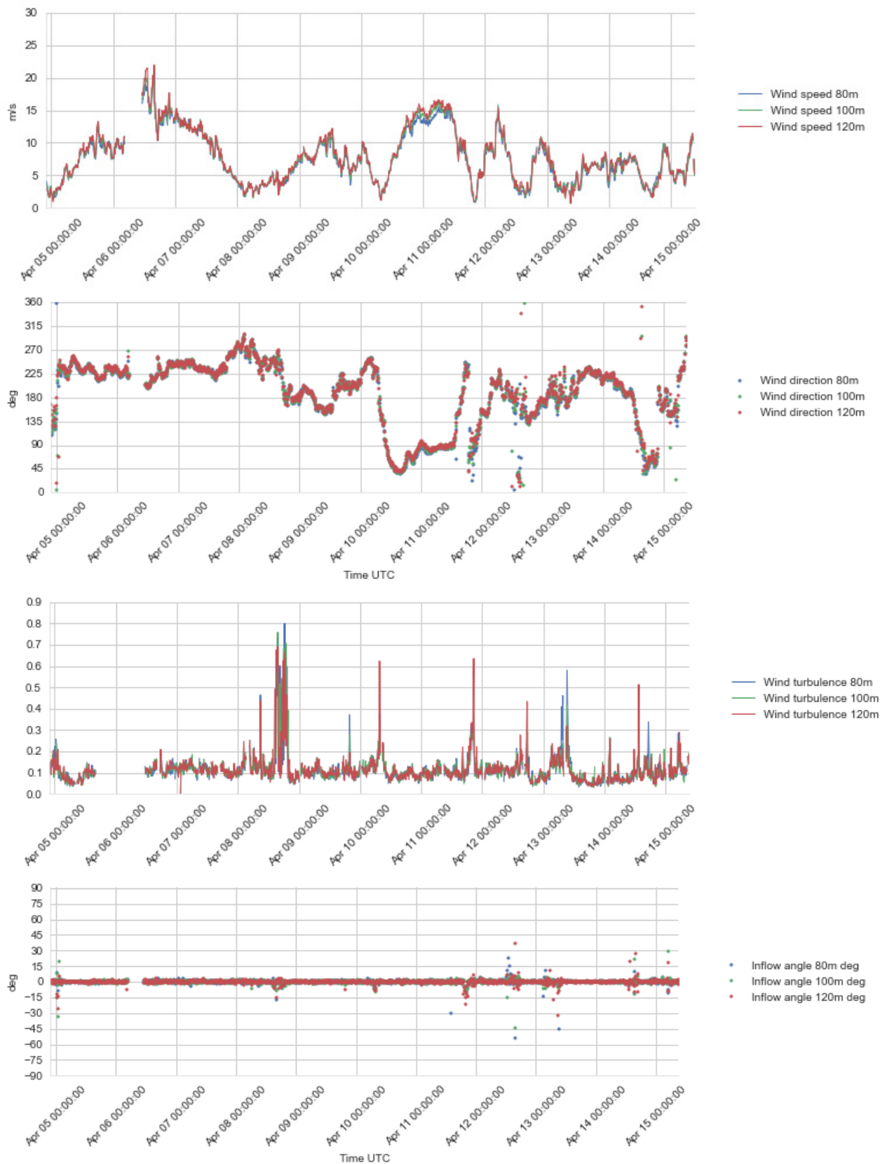
Figure 4.17 Plots of wind profile data, 80 – 120 m a.s.l., 4 - 15 Apr 2016.
