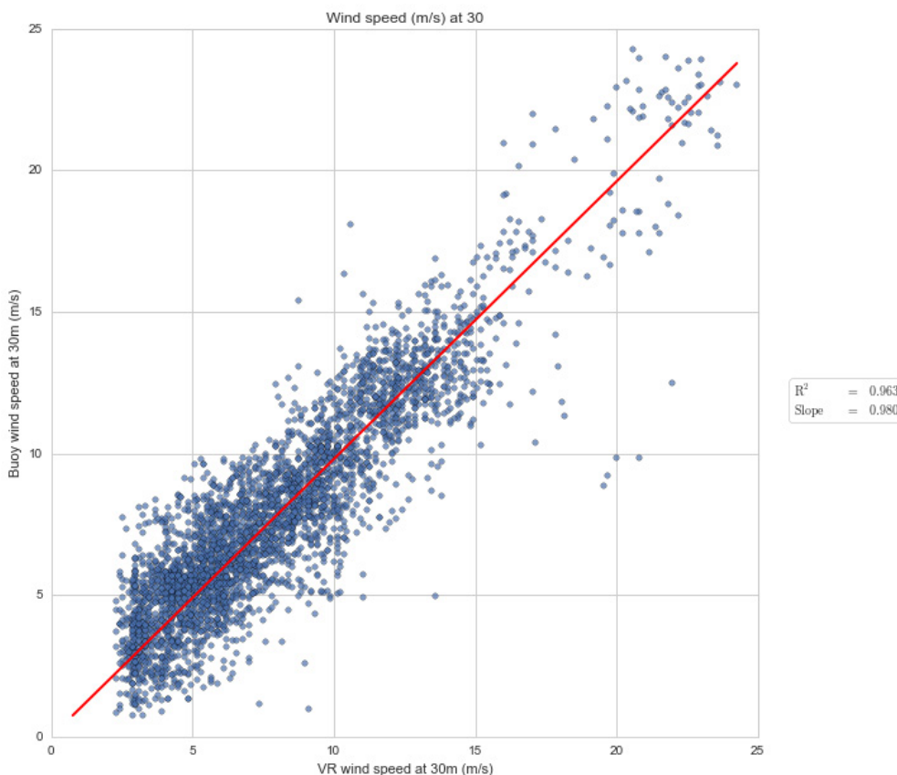
Figure 3.8 Scatter plot comparing the wind speed at 30 m above sea level measured by the Lidar buoy compared to the wind speed at Vlake van de Raan adjusted to 30 m a.s.l. (Regression formula: y = \text{Slope} * x )
