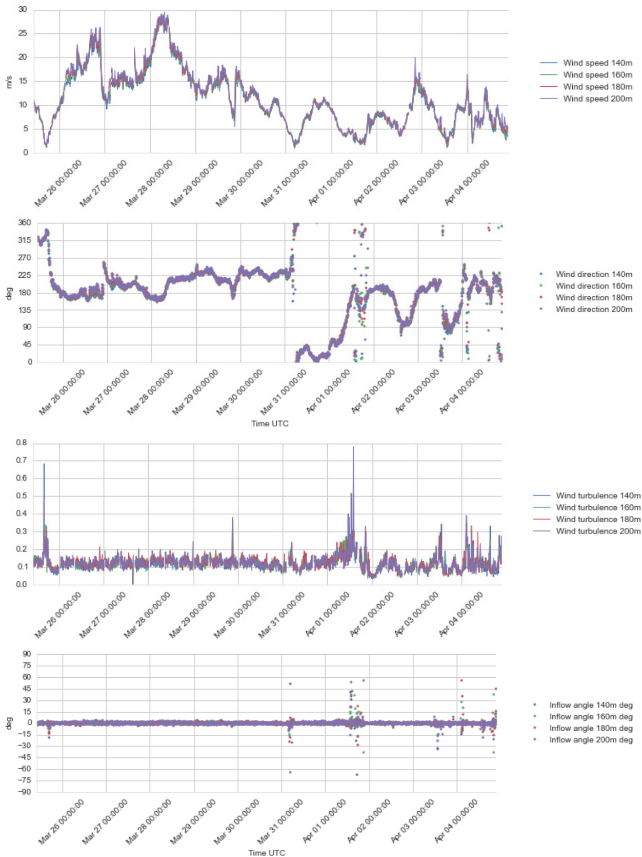
Figure 4.15 Plots of wind profile data, 140 – 200 m a.s.l., 25 Mar – 4 Apr 2016.
