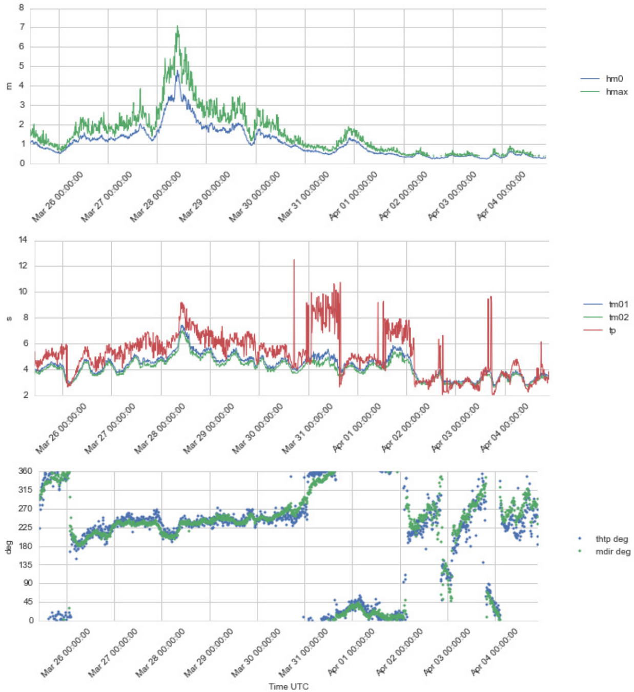
Figure 4.5 Time series plots of wave height ( H_{m0} and H_{max} ) (upper panel), wave period ( T_{m01} , T_{m02} and T_p ) (second panel), and wave direction ( ThTp and Mdir ) (lower panel), 25 Mar – 4 Apr 2016.
