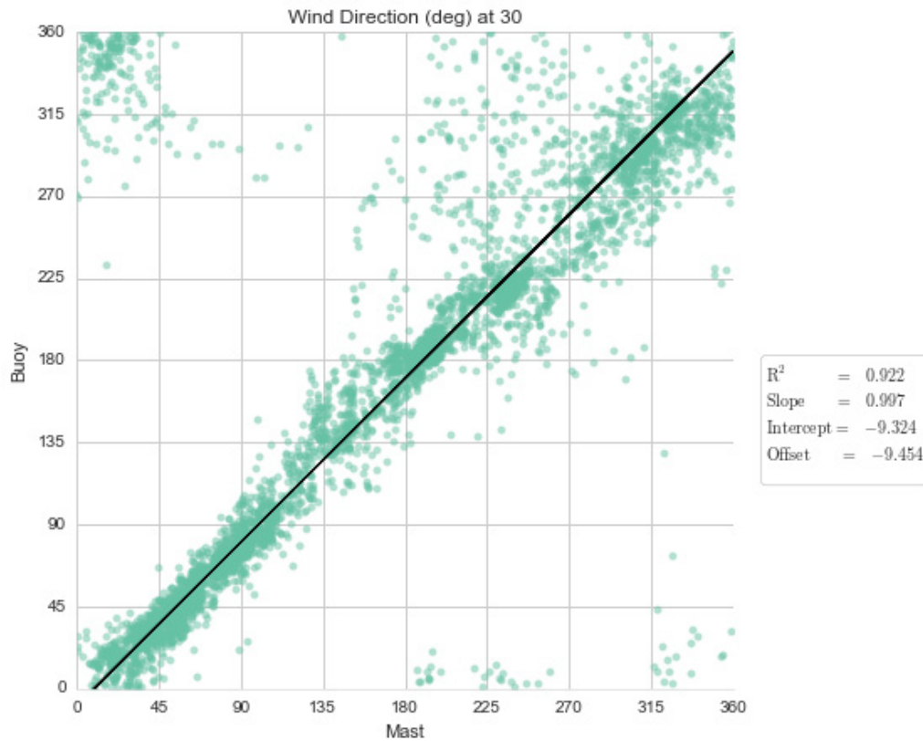
Figure 3.10 Wind direction at 30 m above sea level measured by the Lidar buoy compared to wind direction at Vlakte van de Raan.. (Samples with VR wind speed less than 2 m/s are excluded.) (“Offset” is the average difference of directions.)
