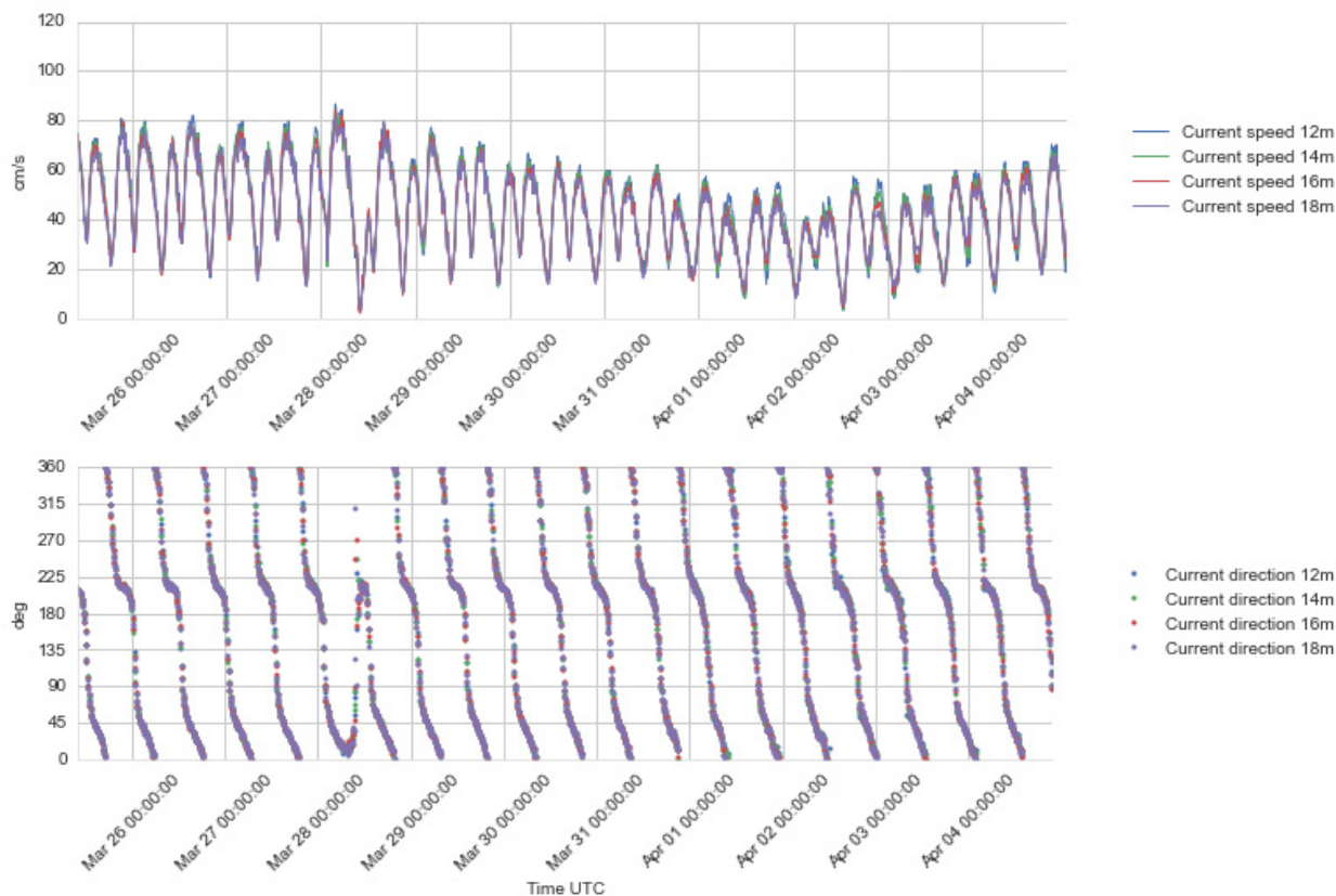
Figure 4.24 Time series plots of current speed (upper) and direction (lower panel), 12 -18 m depth, 25 Mar – 4 Apr 2016.
