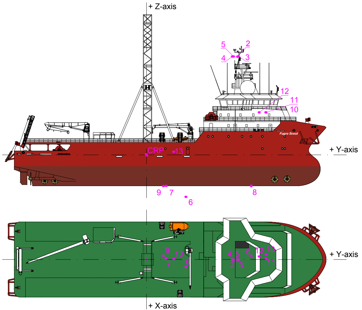
Figure 3.1: MV Fugro Scout Offsets Diagram
