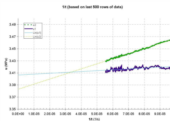
Figure 3, geometric data fitting of piezoprobe test data
