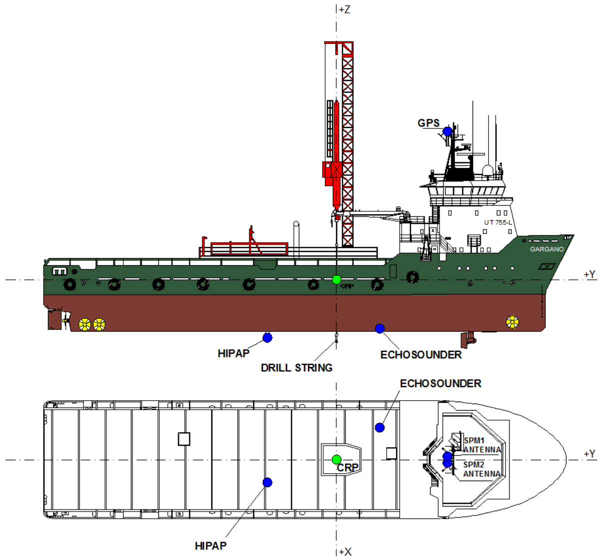
Figure 3.1: MV Gargano Vessel Diagram
