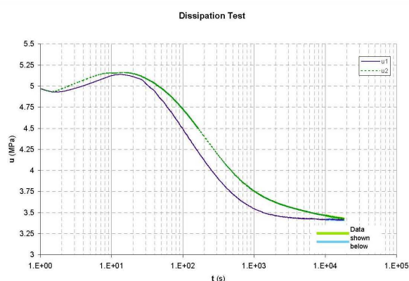
Figure 2, piezoprobe dissipation test results
