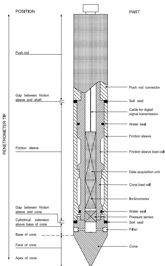
Figure 1 – Piezo-cone Penetrometer
