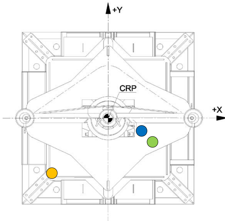
Figure 3.2: Seabed Frame Plan View
