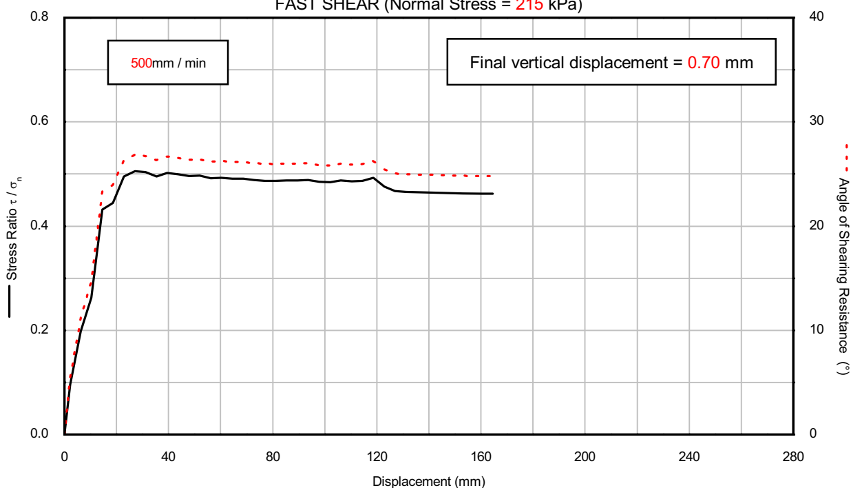
FAST SHEAR (Normal Stress = 215 kPa)
