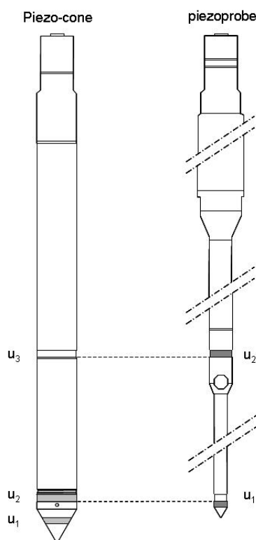
Figure 1, designations for pore pressure filter positions
