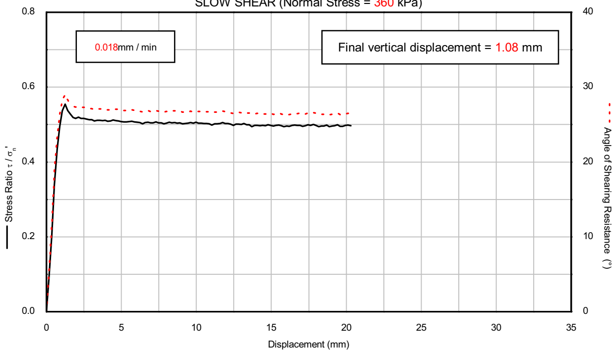
SLOW SHEAR (Normal Stress = 360 kPa)
