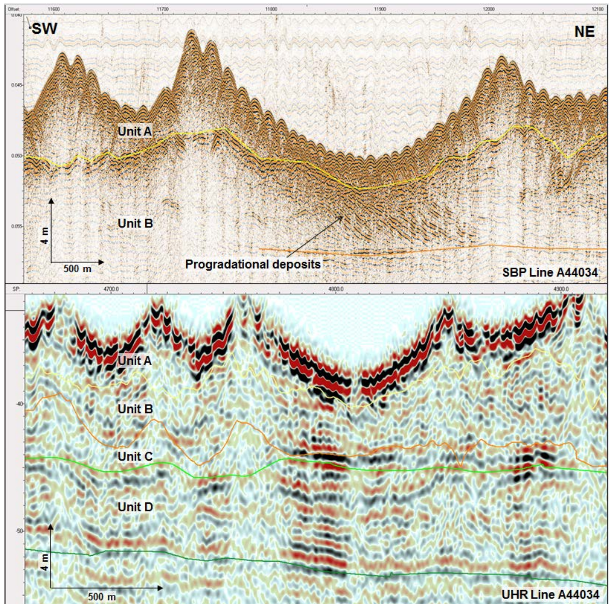
Figure 2.17: Examples of SBP (above) and UHR data (below) on Line A44034.
