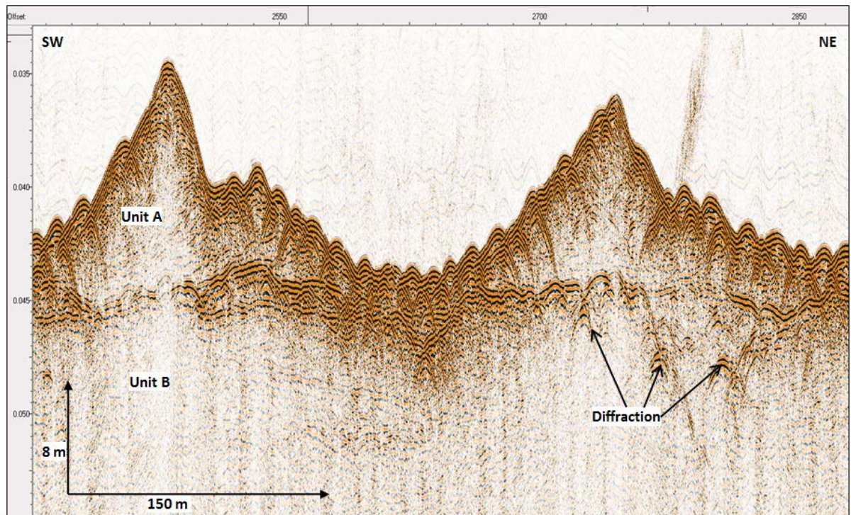
Figure 2.22: SBP Example showing Seismic Anomaly (A41146)
