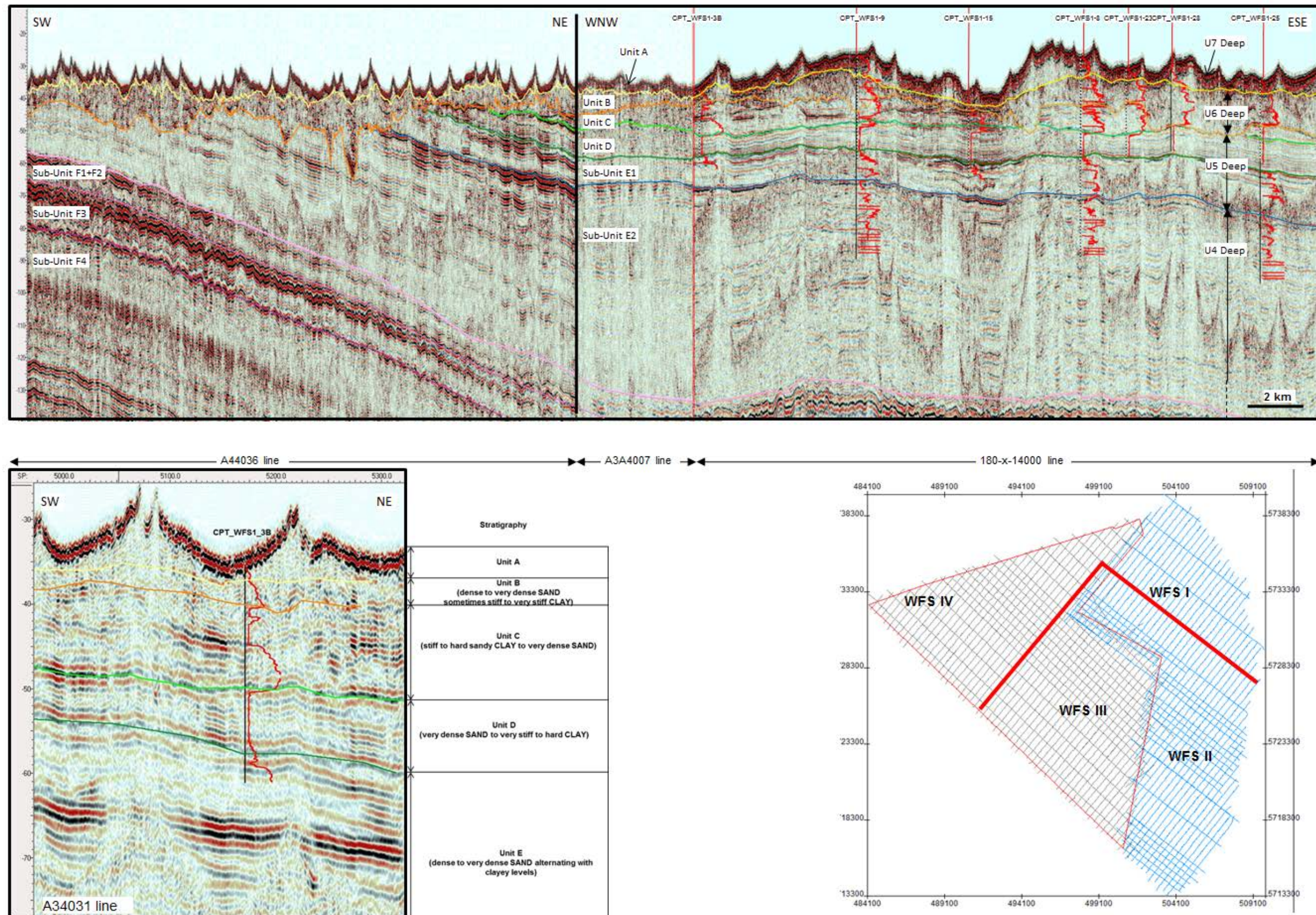
Figure 2.16: Correlation between UHR seismic data and CPT data
