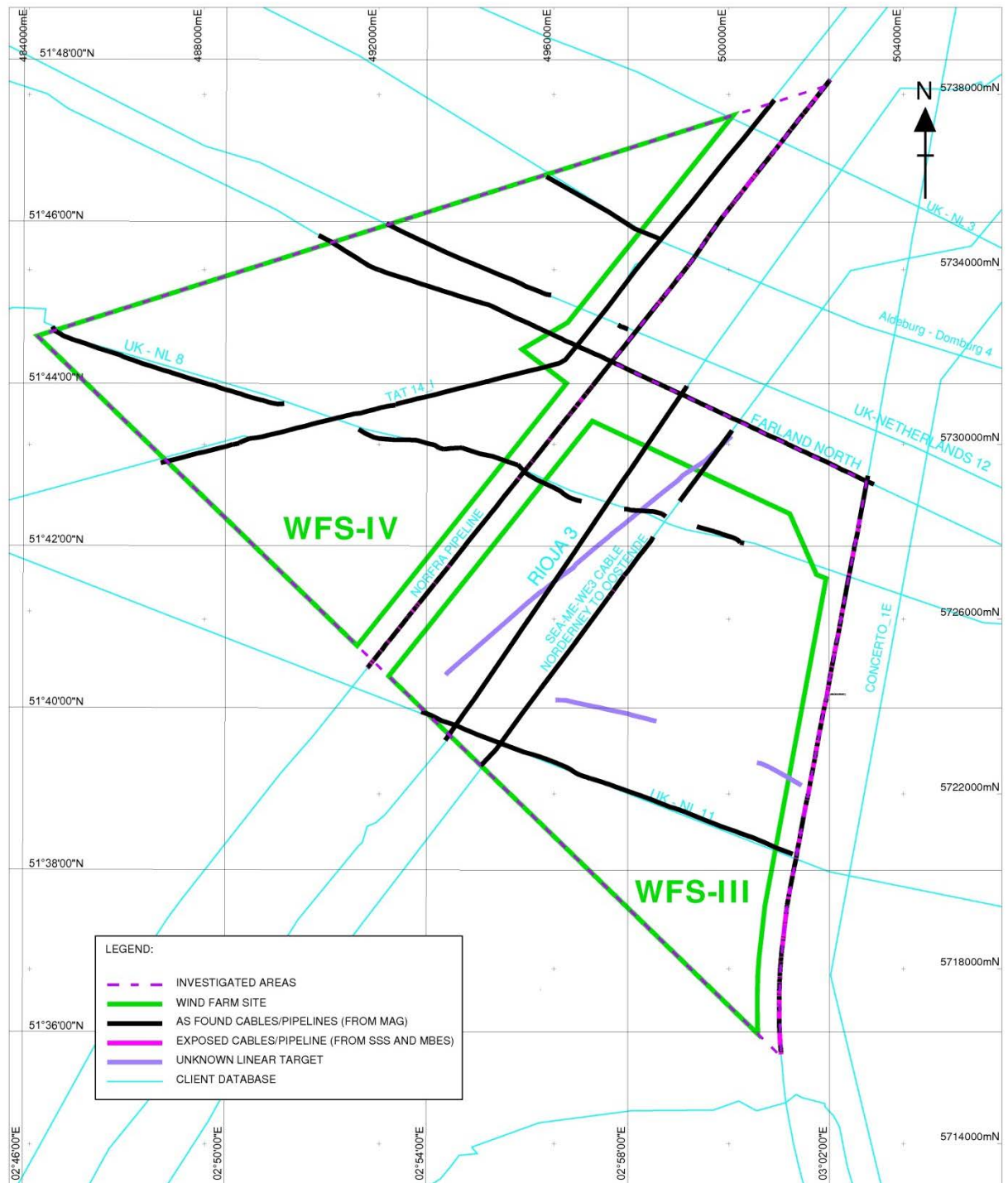
Figure 2.7: Overview map of cables and pipelines in the Investigated area
