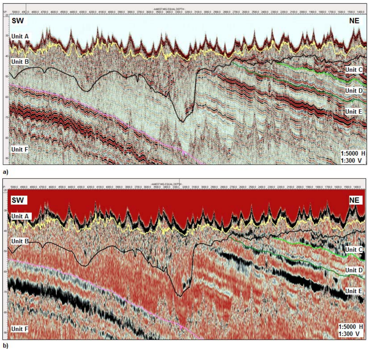
Figure 2.18: Examples of UHR data.
