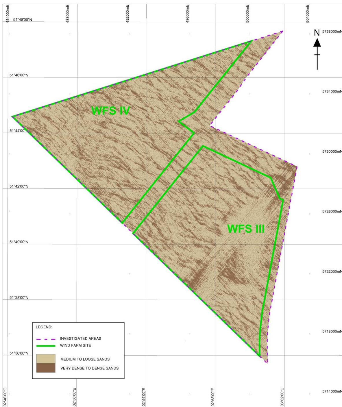
Figure 2.4: Sediment Classification map
