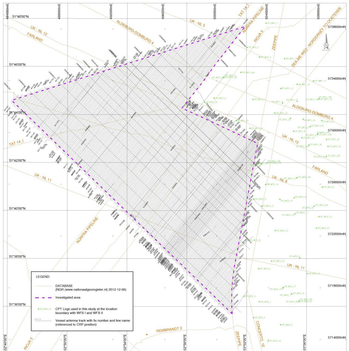
Figure 1.3: CRP track plot.
