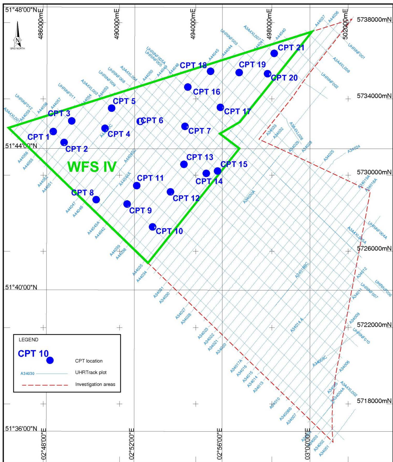
Figure 2.27: Proposed CPT locations within WFS IV
