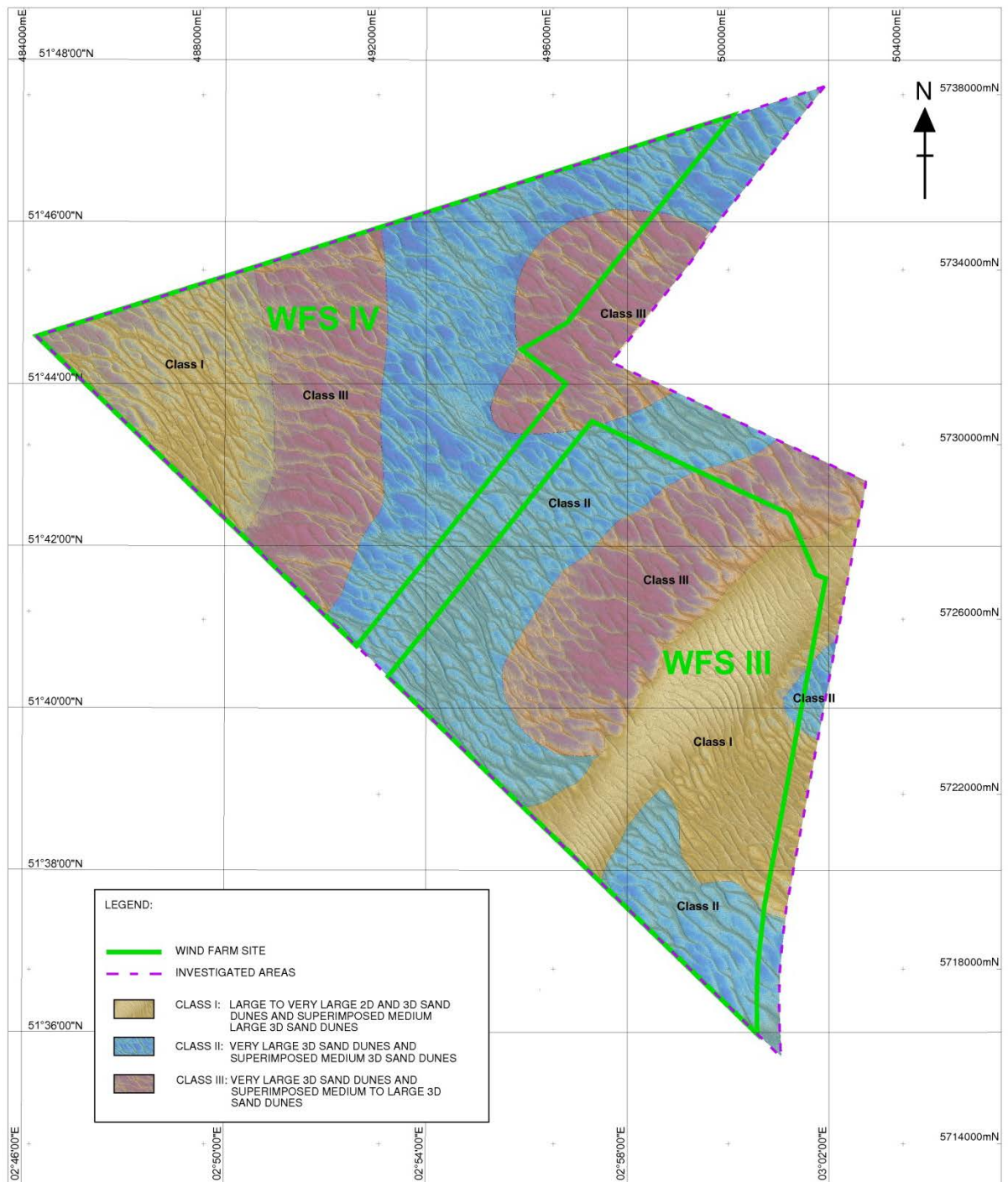
Figure 2.3: Seabed Classification map
