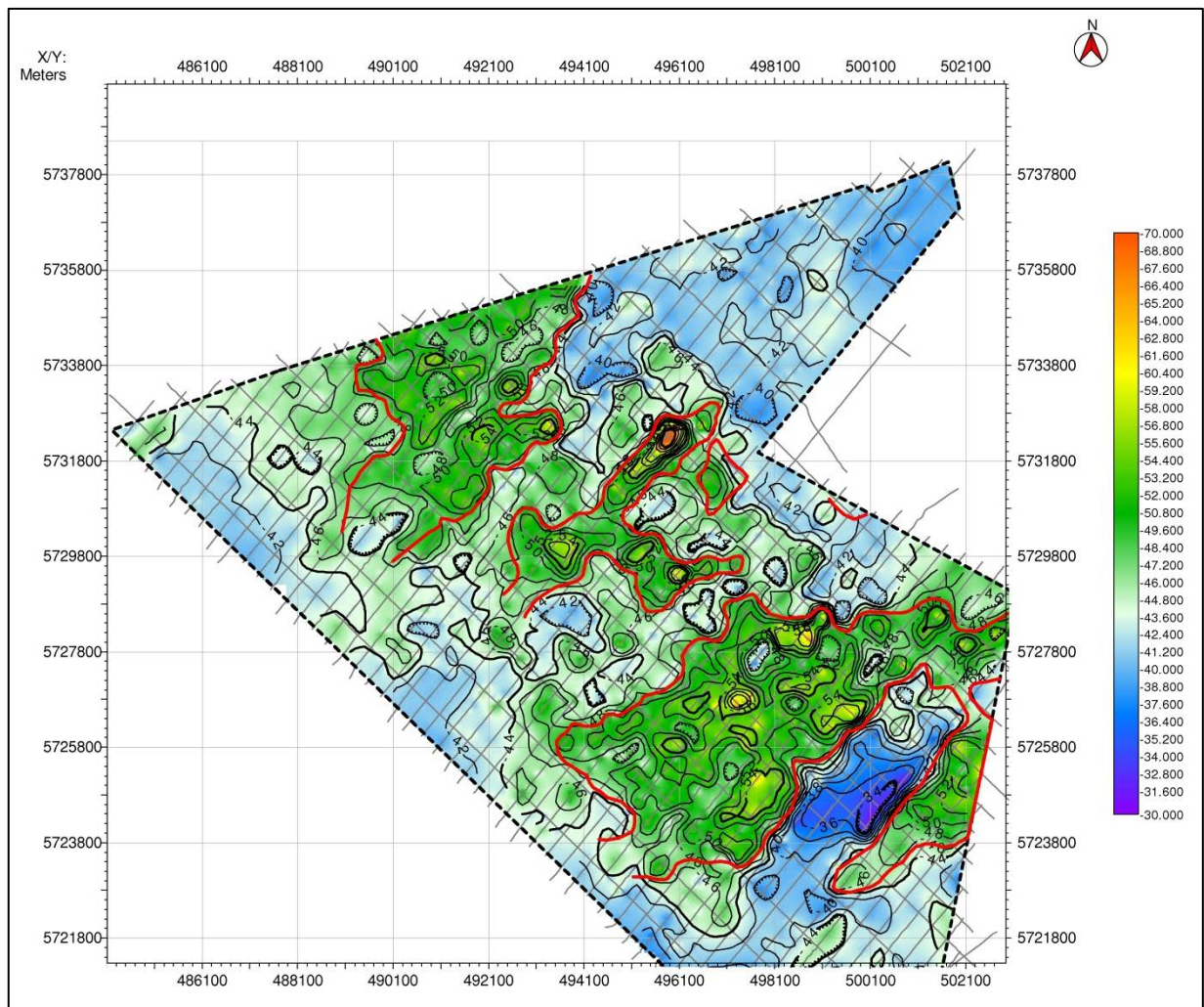
Figure 2.24: Base map of Unit B highlights the palaeochannel areas
