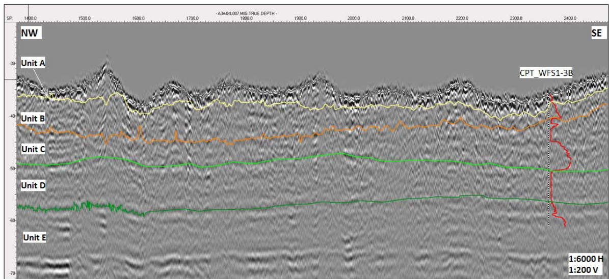
Figure 2.19: Correlation between UHR seismic data and CPT data
