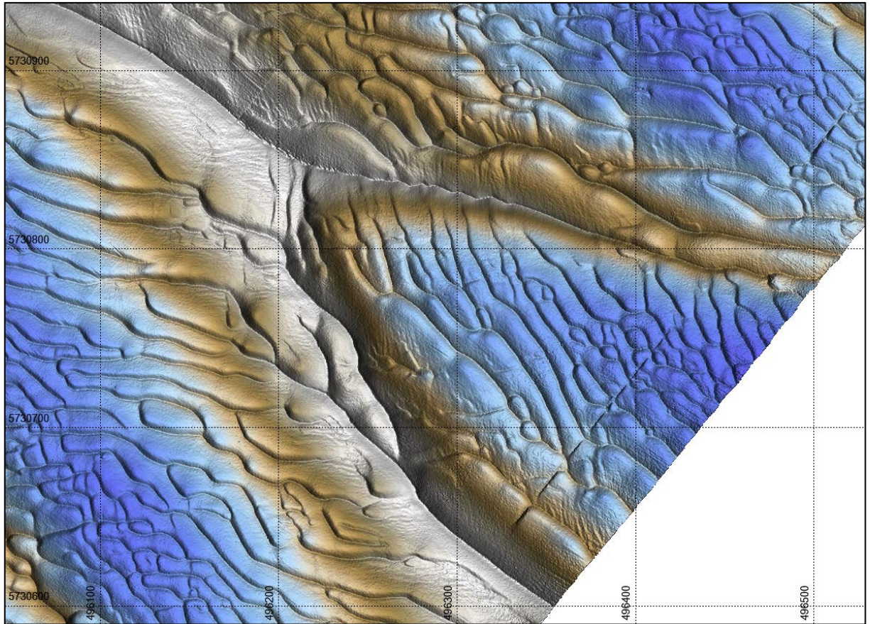
Figure 2.6: MBES data showing NORFRA Pipeline exposure between sand dunes
