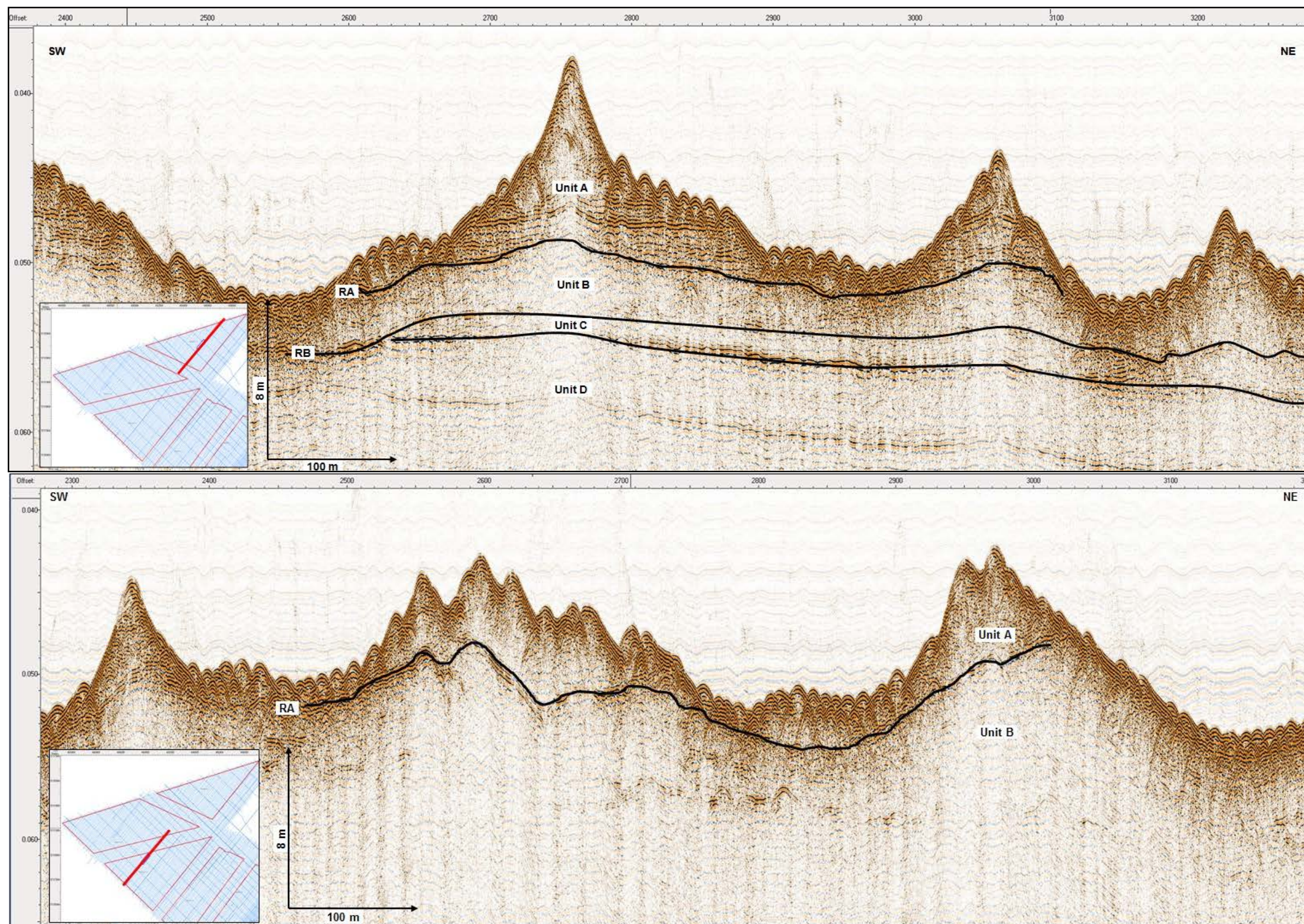
Figure 2.15: SBP data examples: Line A41106 (above) and Line A41112 (below)
