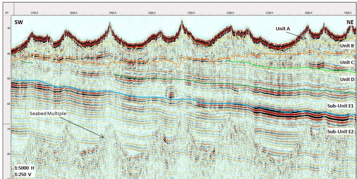
Figure 2.20: Example of Stratigraphy in UHR seismic data (A44037)
