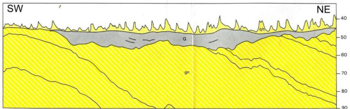
Figure 2.10: Schematic cross-section.
