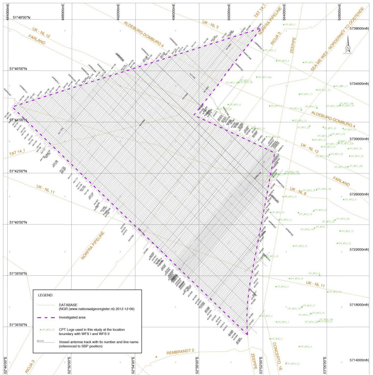
Figure 1.6:SBP track plot
