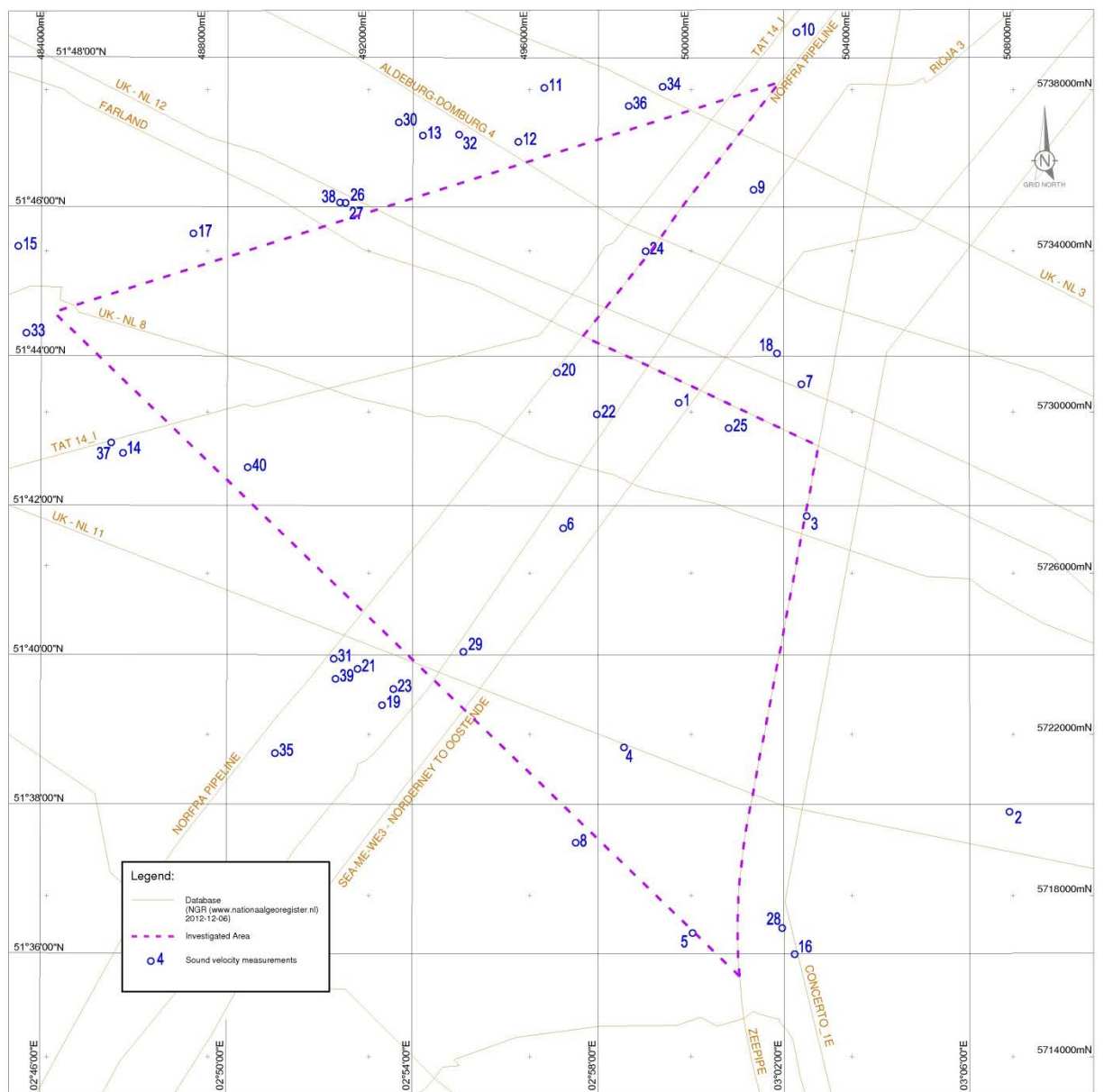
Figure 5.1: Overview of SVP locations.
