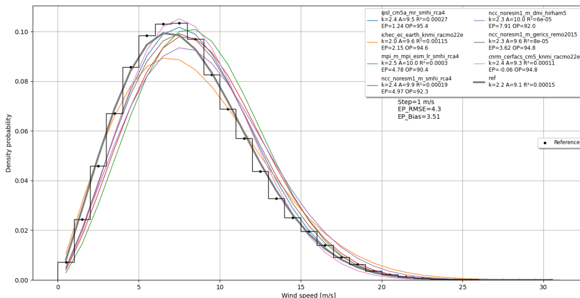
Figure 7.5 Weibull distributions of 7 RCM simulations and WRF (reference) for the IJWVFZ location
