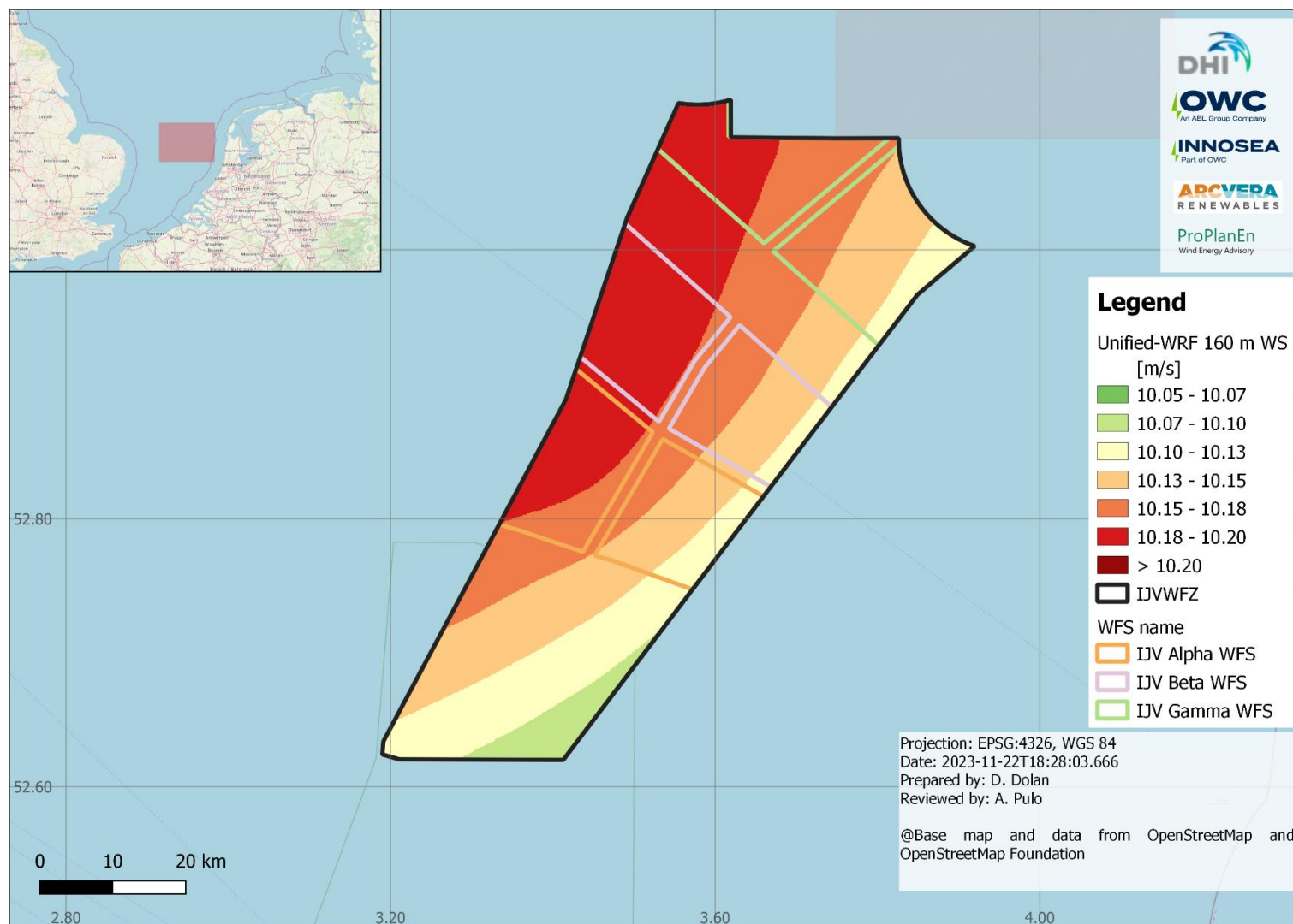
Figure 6.1 IJVWFZ wind speed gradient map at 160 m
