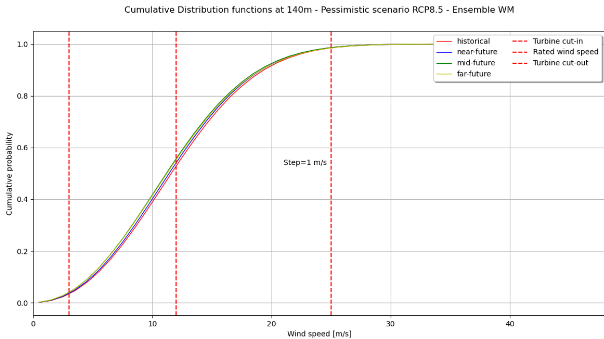
Figure 7.14 CDF at hub height for the ensemble WM under RCP8.5
