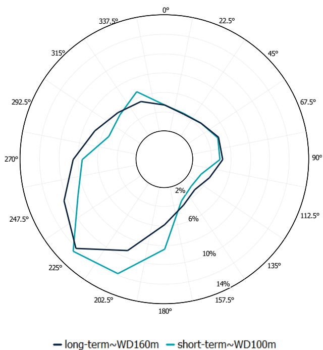
Figure 3.6 FLS IJV 160 m short-term and long-term wind roses
