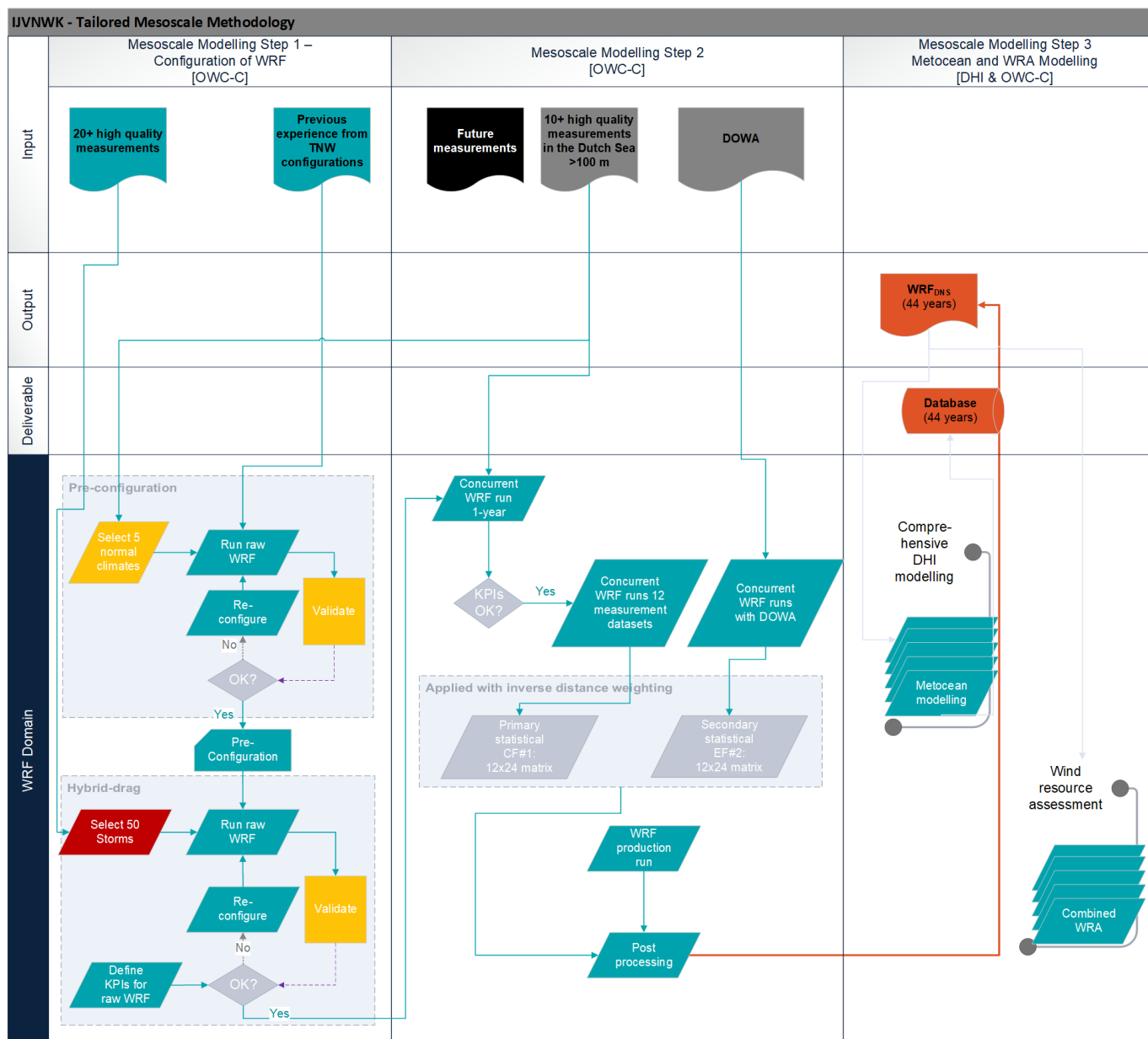
Figure 4.1 Mesoscale modelling methodology
