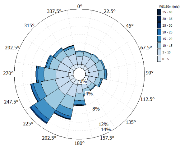
N6_Gamma2 160 m frequency wind rose (Copy from /1/ figure 6.28)
