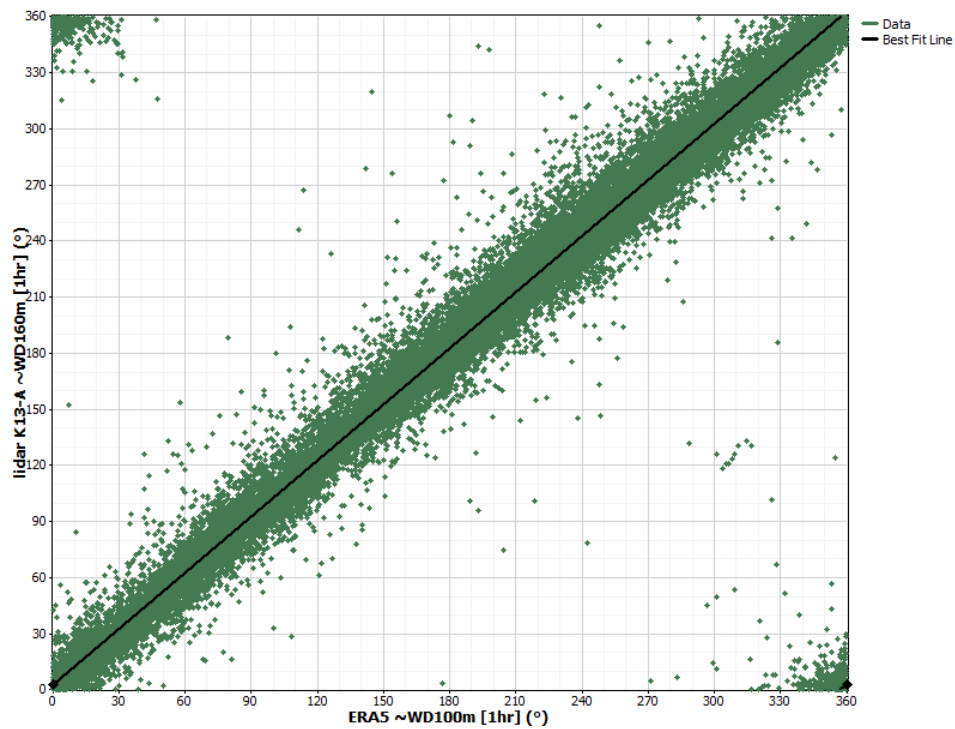
Figure F.8 Lidar K13-A: long-term correction wind direction scatter plots
