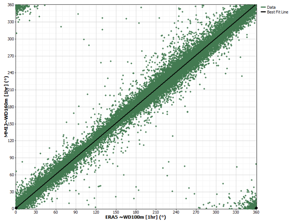
Figure F.6 MMIJ: long-term correction wind direction scatter plots
