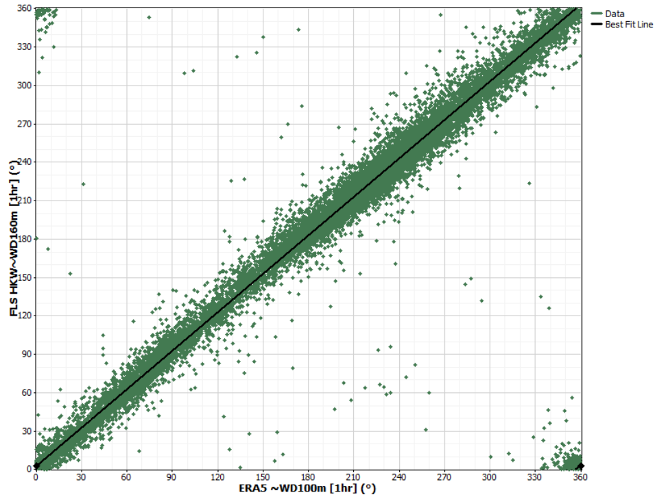
Figure F.7 FLS HKW: long-term correction wind direction scatter plots
