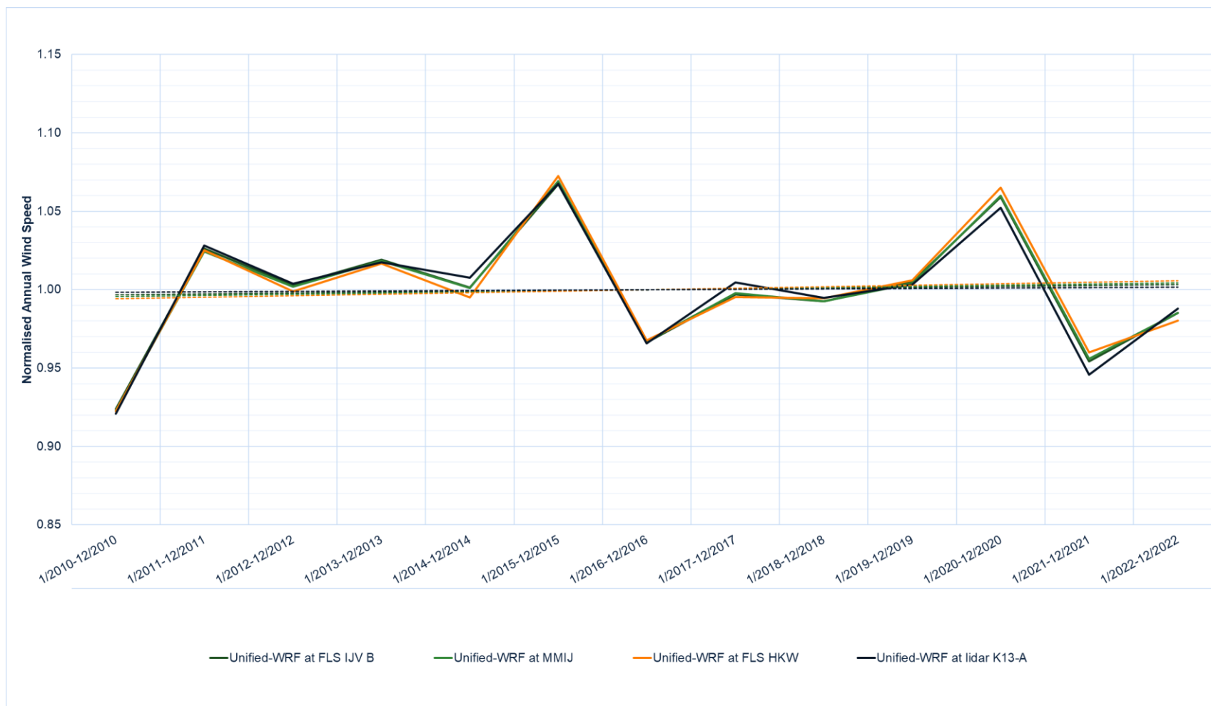
Figure I.1 Unified-WRF long-term trend analysis
