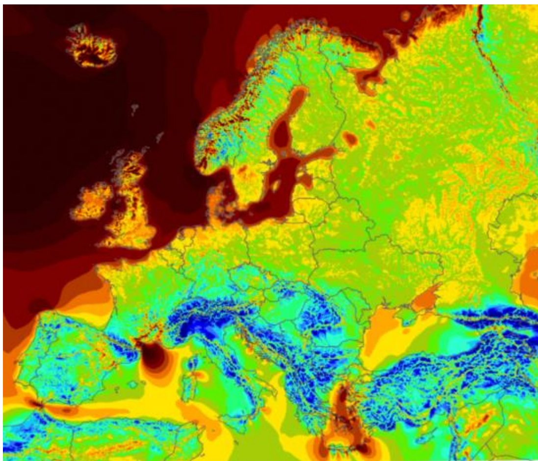
Figure G.1 EMD-WRF Europe+ Model Domain [48]
