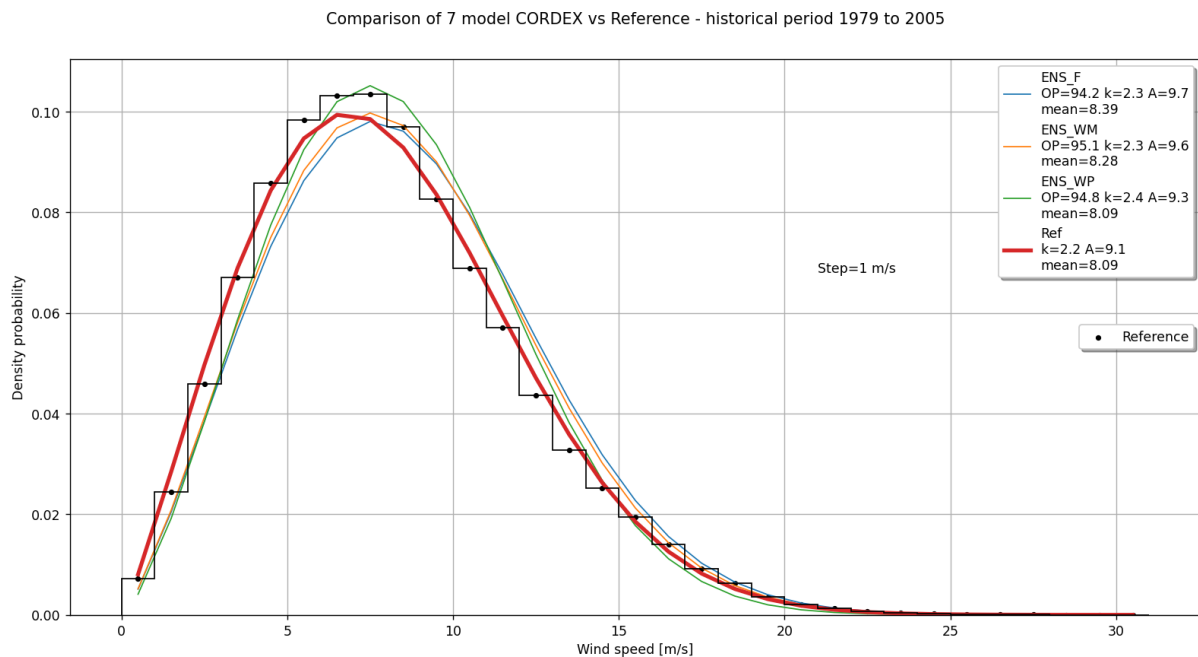
Figure 7.6 Weibull distribution of three ensembles at 10 m height
