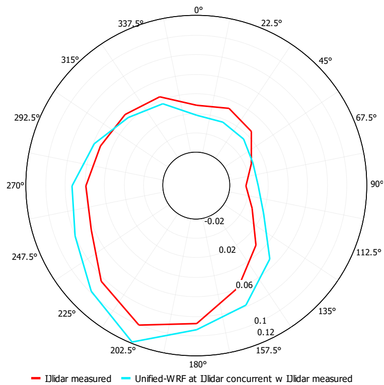
Figure 6.4 Concurrent measured and modelled wind shear rose at IJlilar
