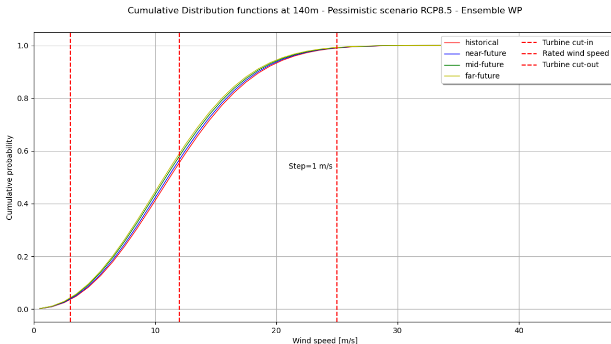
Figure 7.15 CDF at hub height for the ensemble WP under RCP8.5
