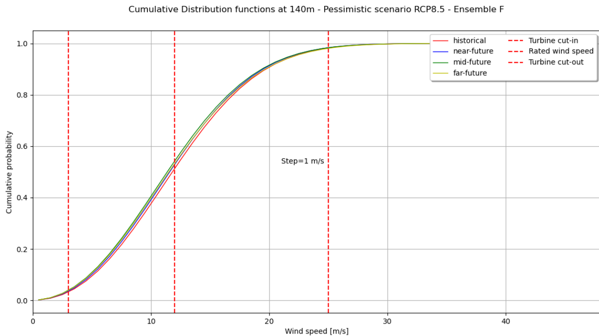
Figure 7.13 CDF at hub height for the ensemble F under RCP8.5
