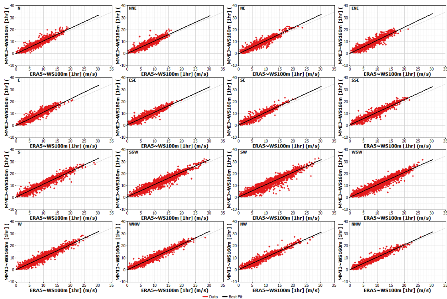
Figure F.2 MM1J: long-term correction wind speed scatter plots
