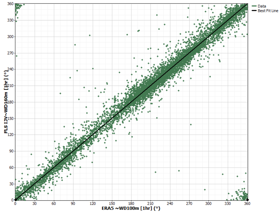
Figure F.5 FLS HKW: long-term correction wind direction scatter plots
