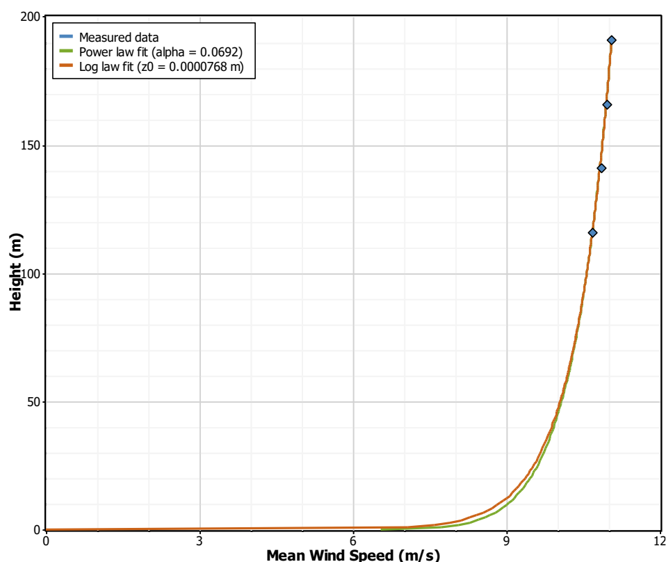
Figure 3.4 Lidar K13-A vertical wind profile
