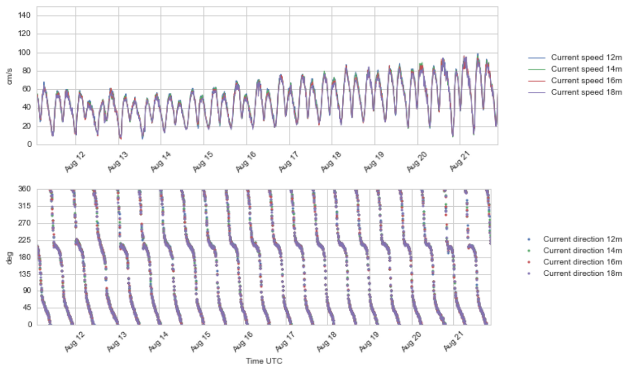
Figure 4.28 Time series plots of current speed (upper) and direction (lower panel), 12 - 18 m depth, 11- 21 Aug 2016.
