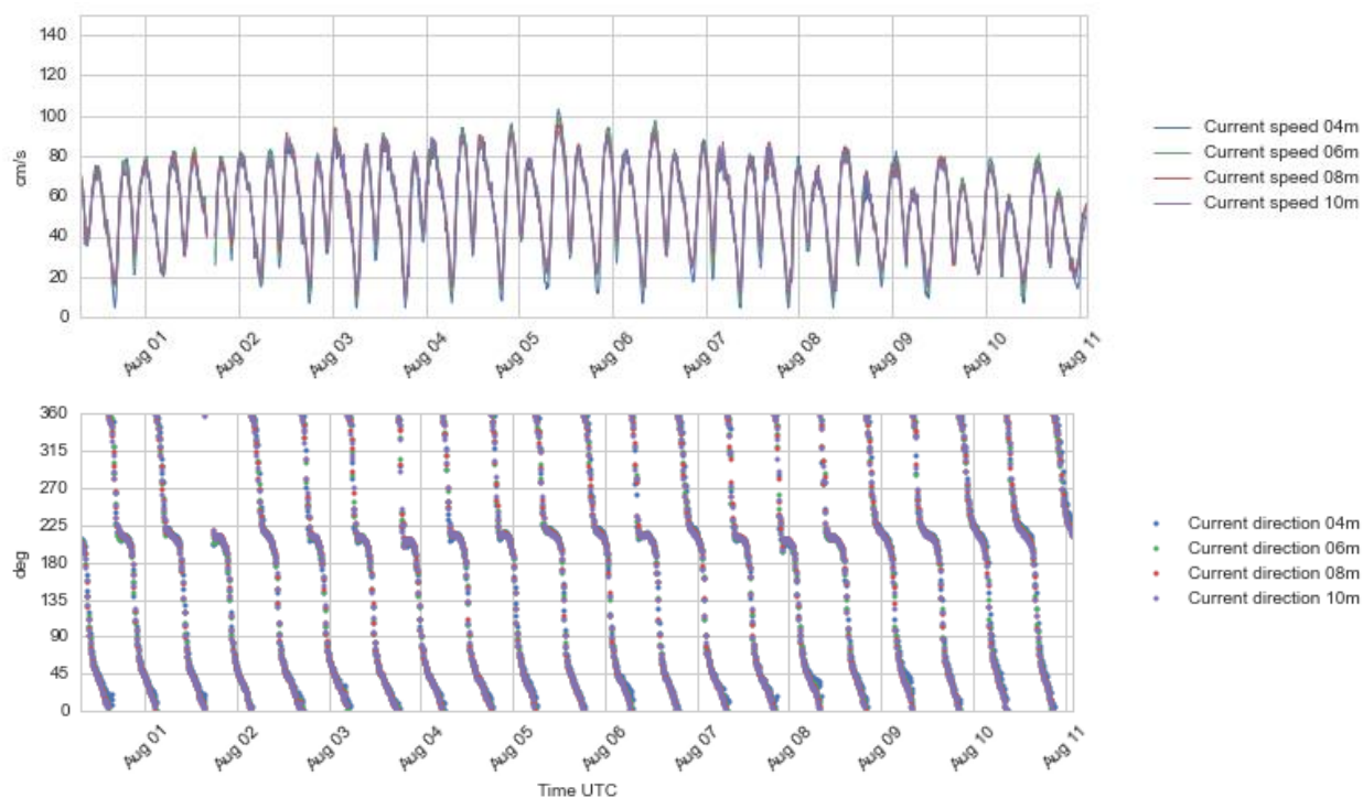
Figure 4.23 Time series plots of current speed (upper) and direction (lower panel), 4 - 10 m depth, 31 Jul – 11 Aug 2016.
