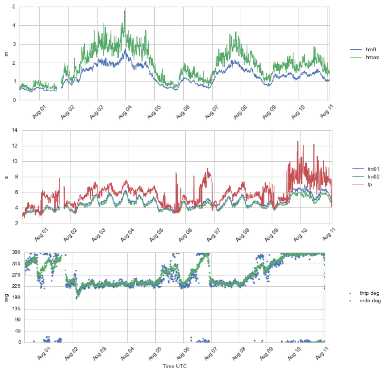
Figure 4.5 Time series plots of wave height ( H_{m0} and H_{max} ) (upper panel), wave period ( T_{m01} , T_{m02} and T_p ) (second panel), and wave direction ( ThTp and Mdir ) (lower panel), 31 Jul – 11 Aug 2016.
