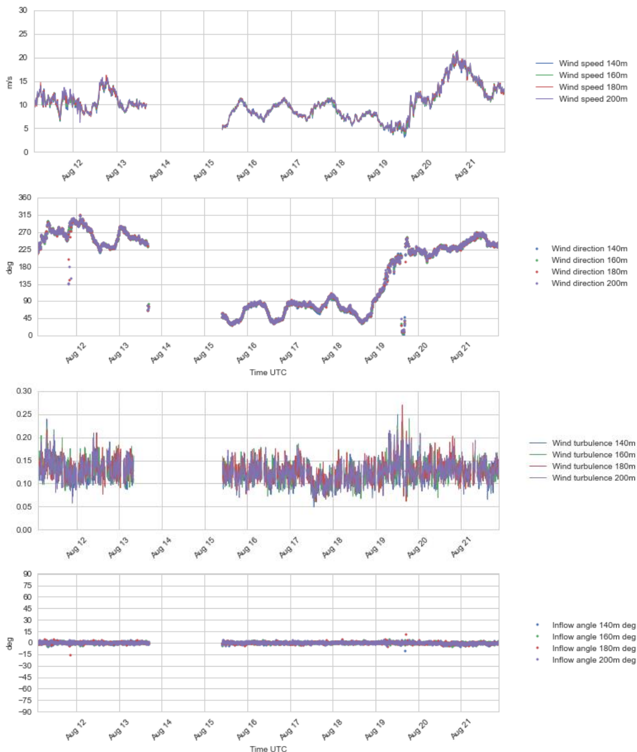
Figure 4.18 Plots of wind profile data, 140 – 200 m a.s.l., 11 - 21 Aug 2016.
