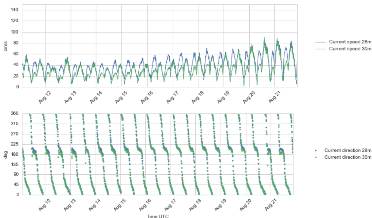
Figure 4.30 Time series plots of current speed (upper) and direction (lower panel), 28 - 30 m depth, 11 - 21 Aug 2016.
