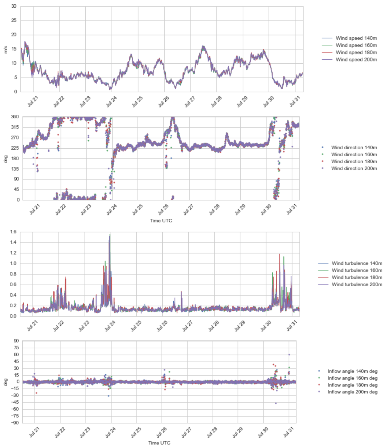
Figure 4.12 Plots of wind profile data, 140 – 200 m a.s.l., 21 – 31 Jul 2016.
