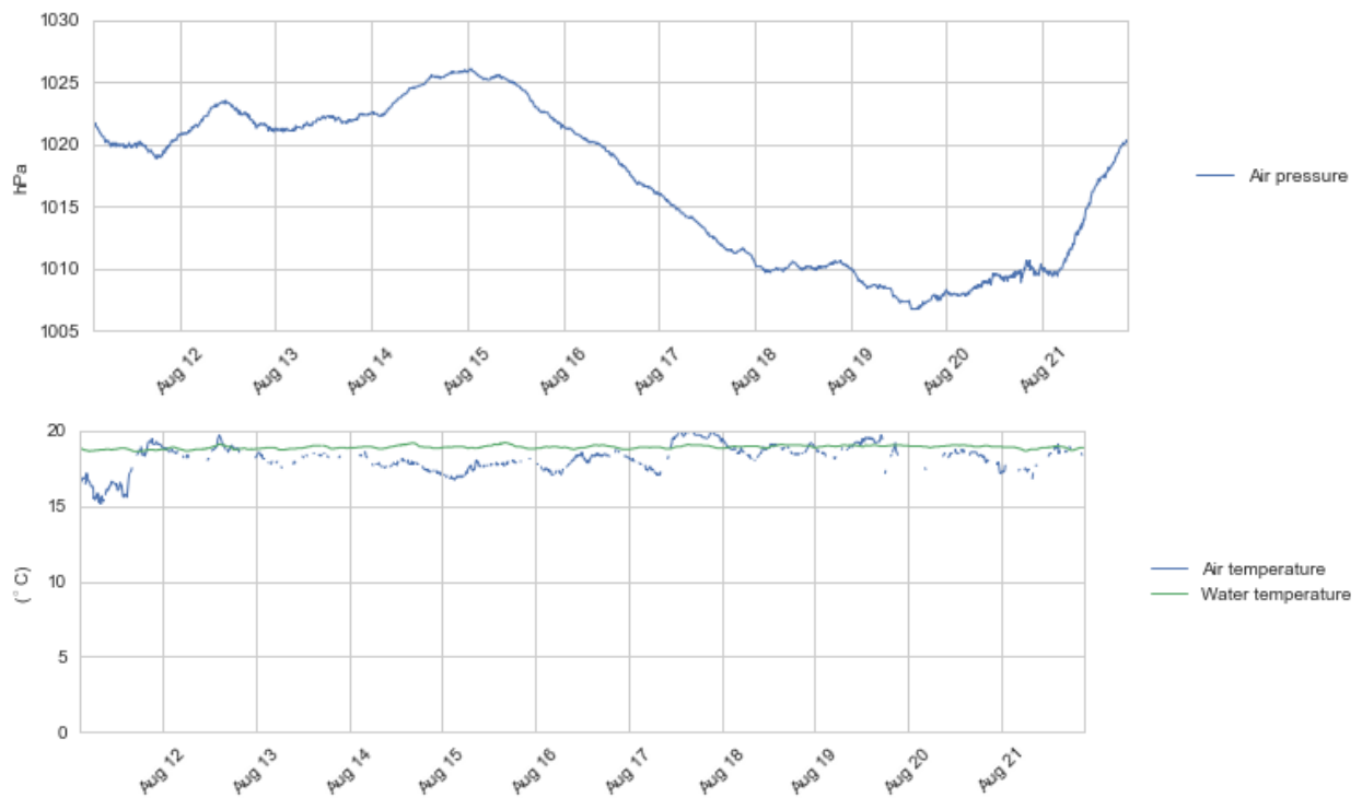
Figure 4.3 Time series plots of air pressure (upper panel), air and water temperature (lower panel), 11 - 21 Aug 2016.
