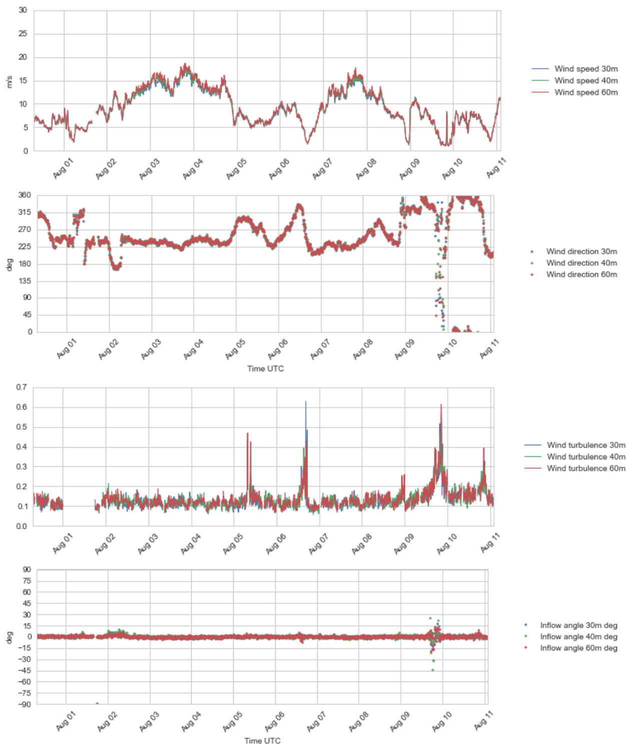
Figure 4.13 Plots of wind profile data, 30 – 60 m a.s.l., 31 Jul – 11 Aug 2016.
