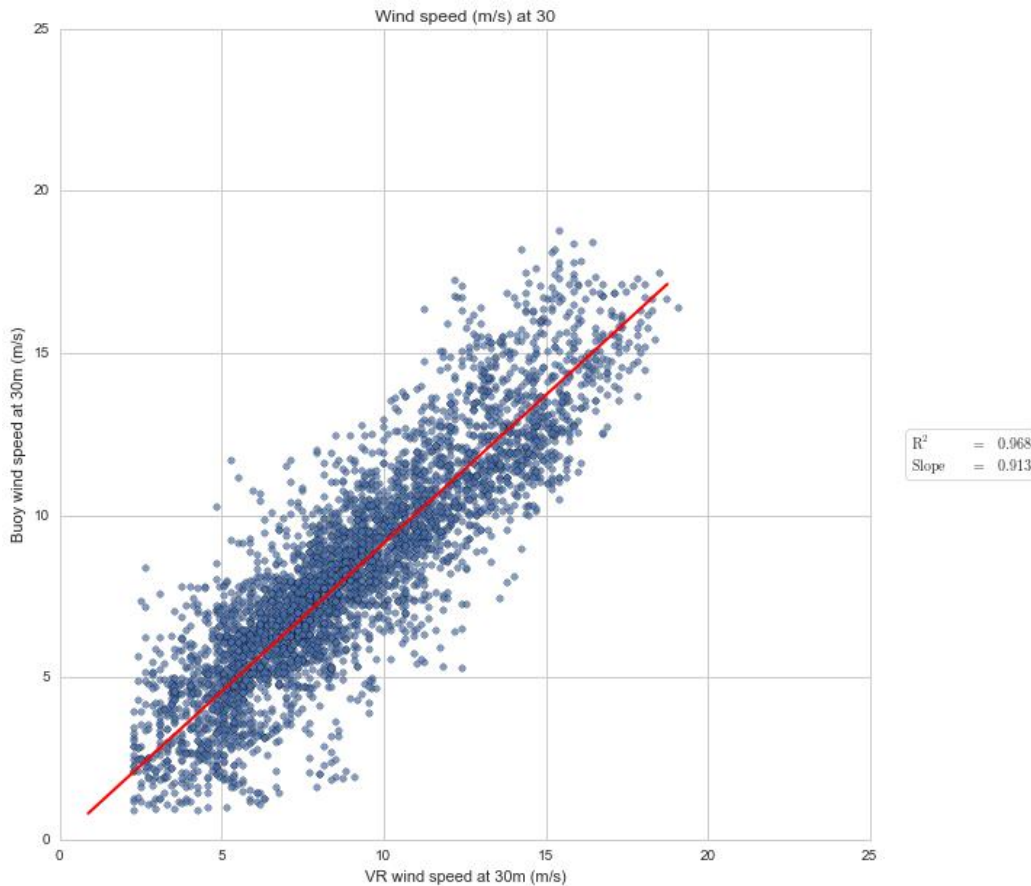
Figure 3.8 Scatter plot comparing the wind speed at 30 m above sea level measured by the Lidar buoy to the wind speed at Vlake van de Raan adjusted to 30 m a.s.l. (Regression formula: y = \text{Slope} * x )
