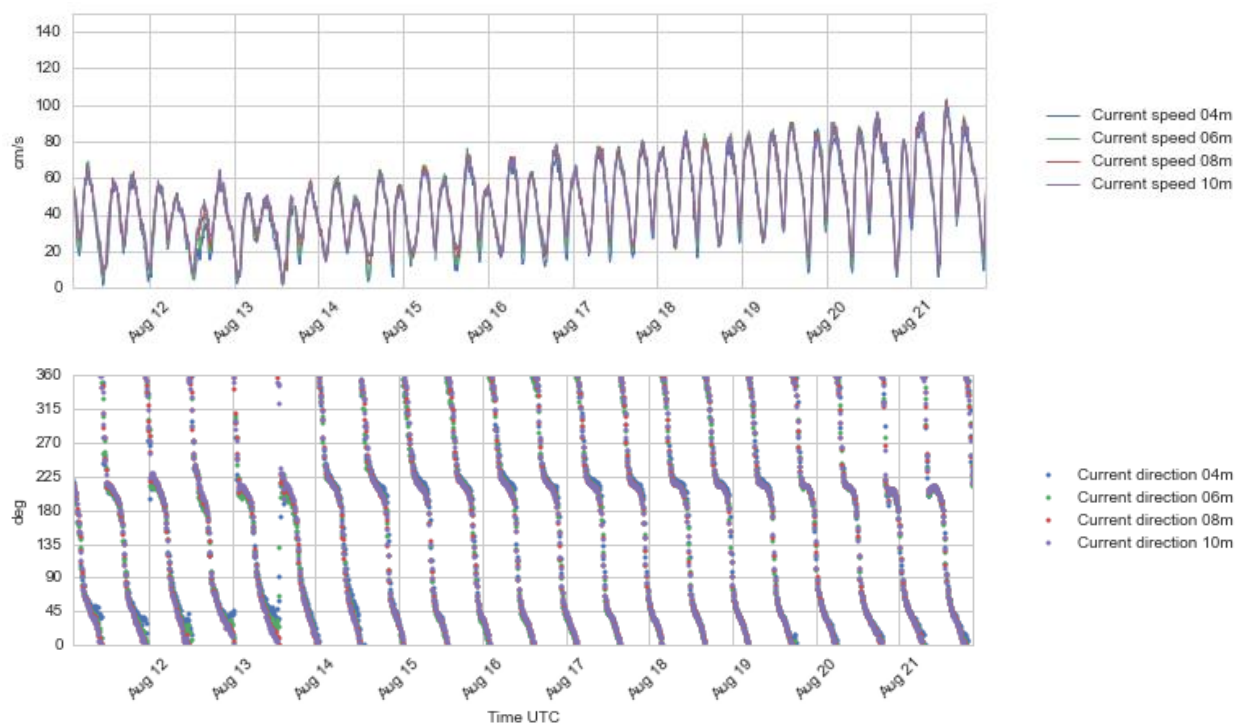
Figure 4.27 Time series plots of current speed (upper) and direction (lower panel), 4 - 10 m depth, 11 - 21 Aug 2016.
