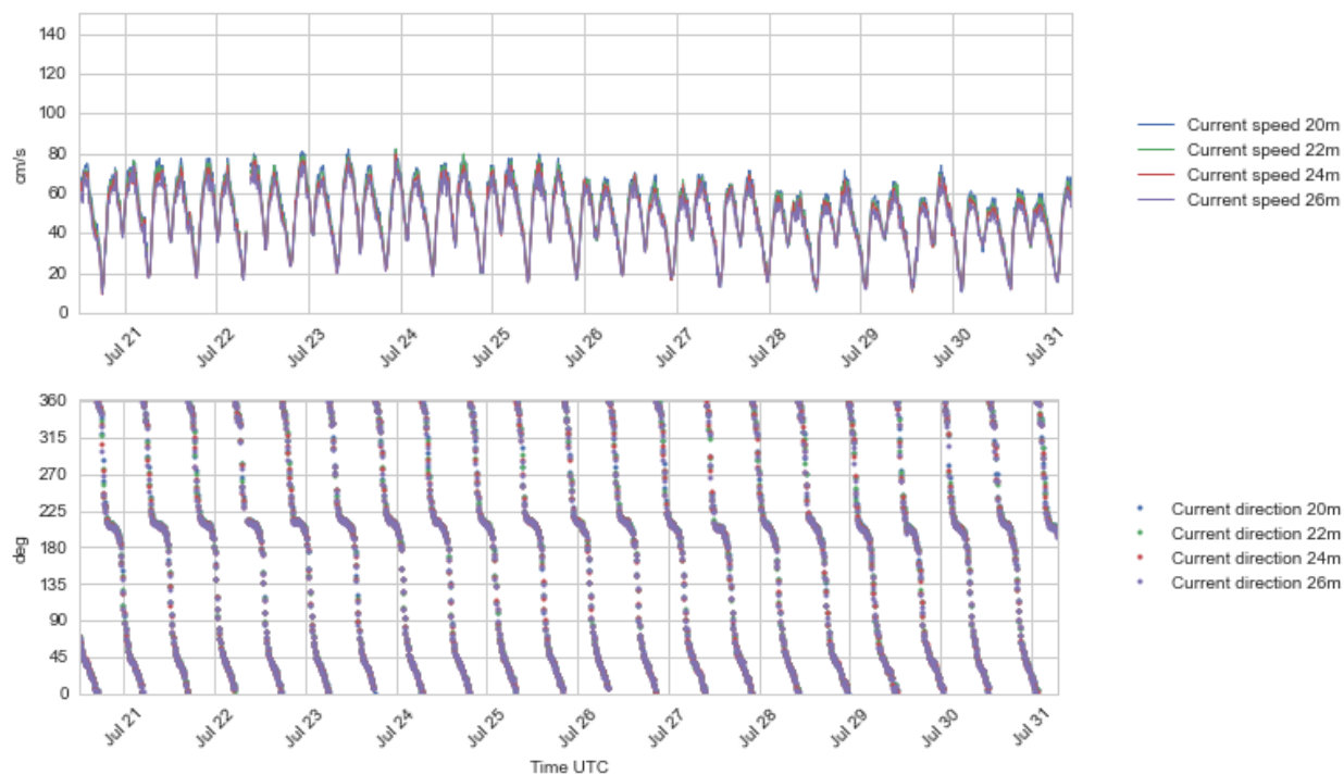
Figure 4.21 Time series plots of current speed (upper) and direction (lower panel), 20 - 26 m depth, 20 – 31 Jul 2016.
