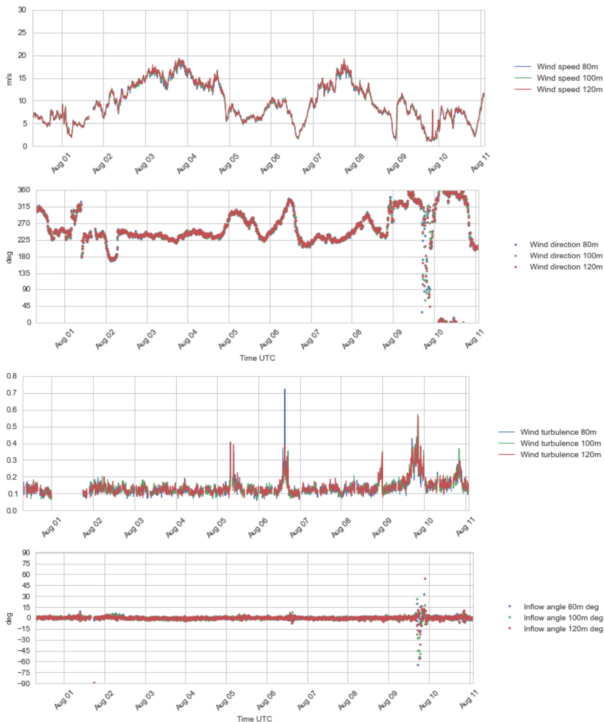
Figure 4.14 Plots of wind profile data, 80 – 120 m a.s.l., 31 Jul – 11 Aug 2016.
