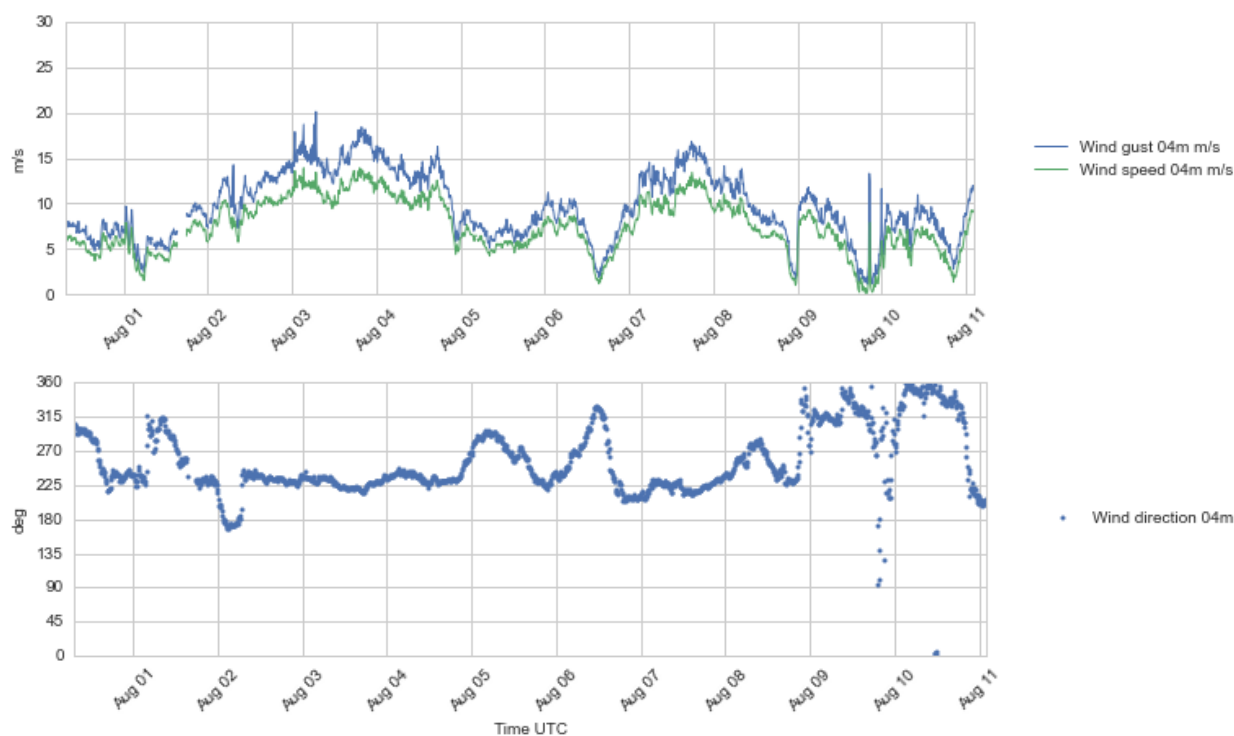
Figure 4.8 Plots of wind speed and gust (upper), and wind direction (lower) at 4 m a.s.l., 31 Jul – 11 Aug 2016.
