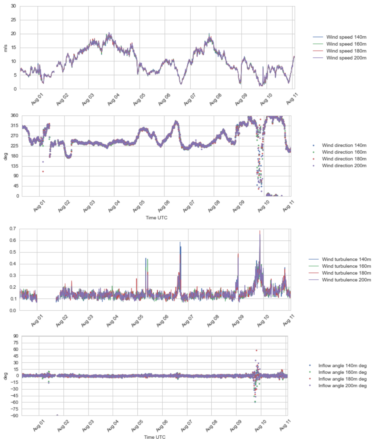
Figure 4.15 Plots of wind profile data, 140 – 200 m a.s.l., 31 Jul – 11 Aug 2016.
