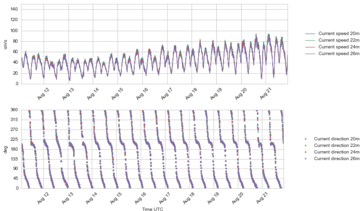
Figure 4.29 Time series plots of current speed (upper) and direction (lower panel), 20 - 26 m depth, 11 - 21 Aug 2016.
