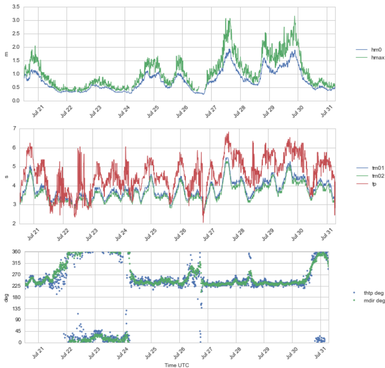
Figure 4.4 Time series plots of wave height ( Hm0 and Hmax ) (upper panel), wave period ( Tm01 , Tm02 and Tp ) (second panel), and wave direction ( ThTp and Mdir ) (lower panel), 21 - 31 Jul 2016.
