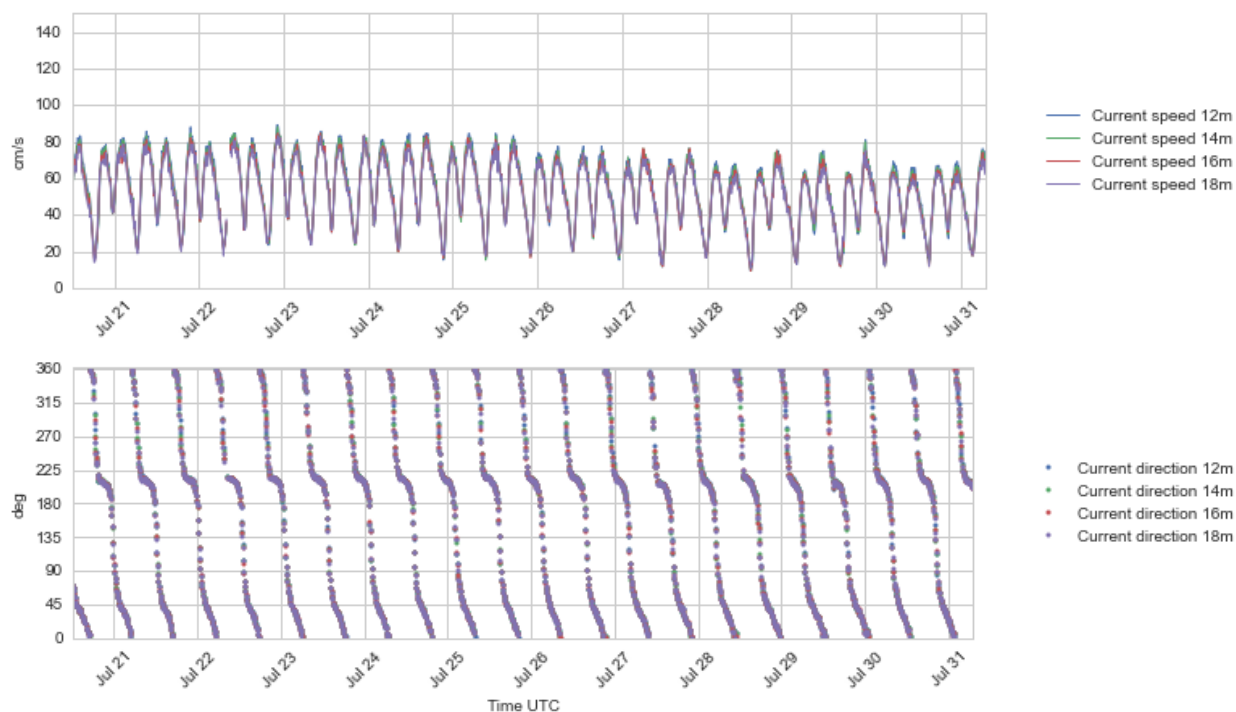
Figure 4.20 Time series plots of current speed (upper) and direction (lower panel), 12 - 18 m depth, 20 – 31 Jul 2016.
