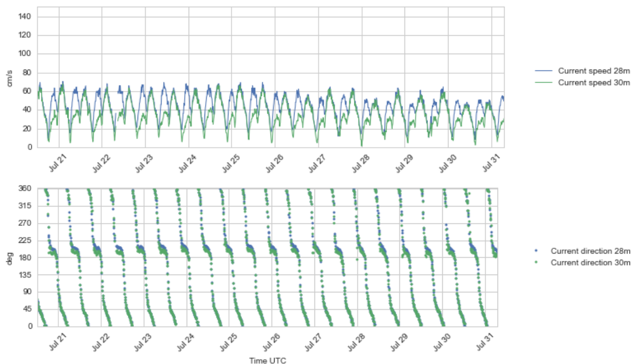
Figure 4.22 Time series plots of current speed (upper) and direction (lower panel), 28 - 30 m depth, 20 – 31 Jun 2016.
