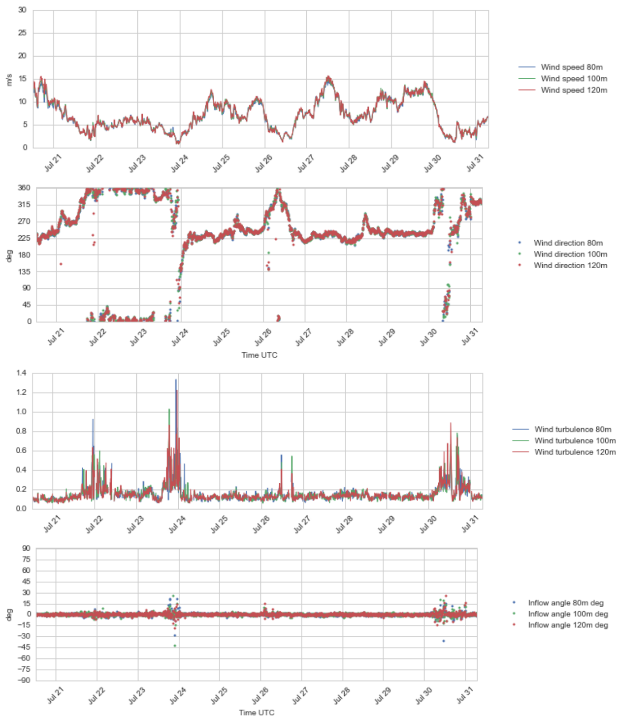
Figure 4.11 Plots of wind profile data, 80 – 120 m a.s.l., 21 – 31 Jul 2016.
