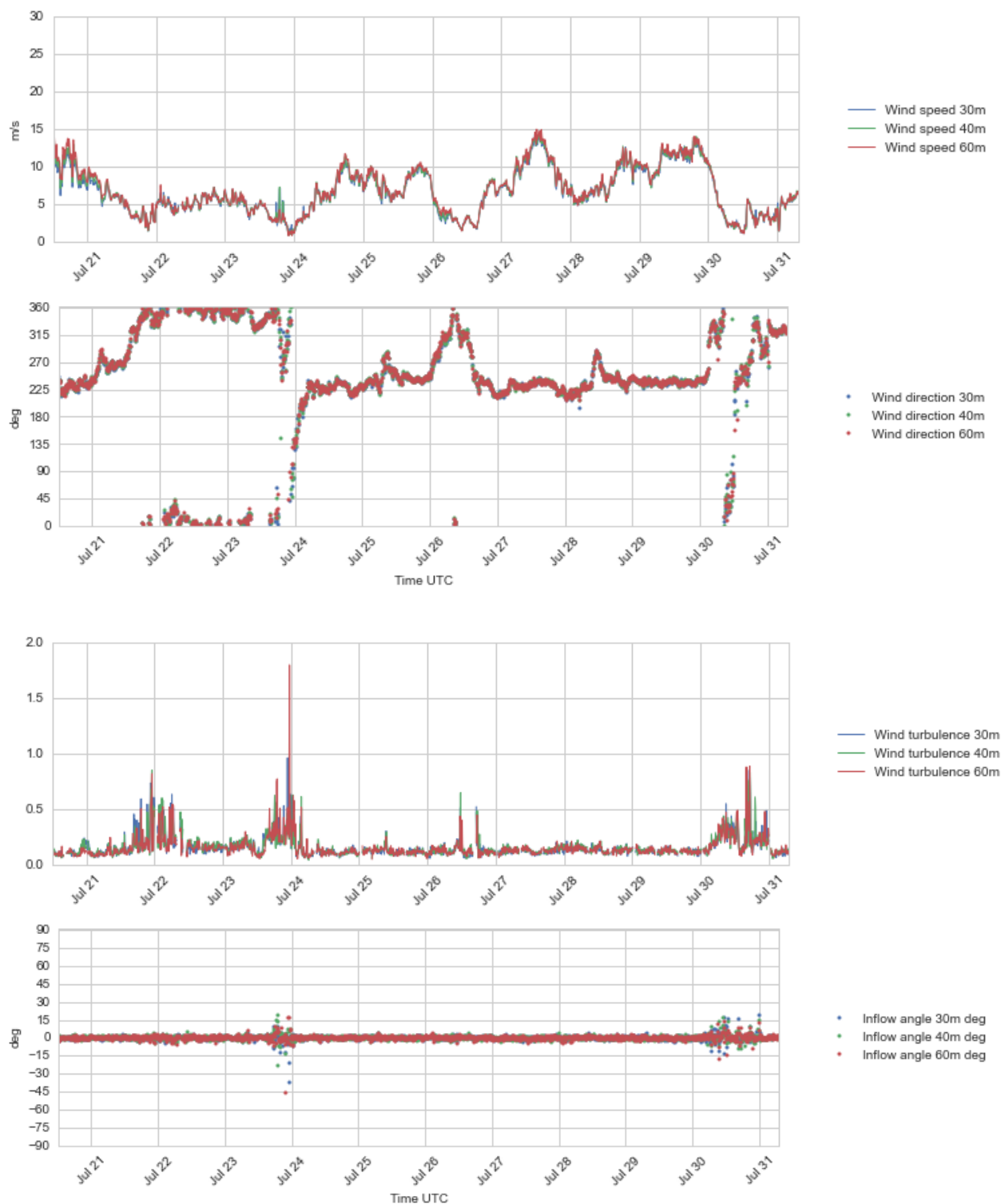
Figure 4.10 Plots of wind profile data, 30 – 60 m a.s.l., 21 – 31 Jul 2016.
