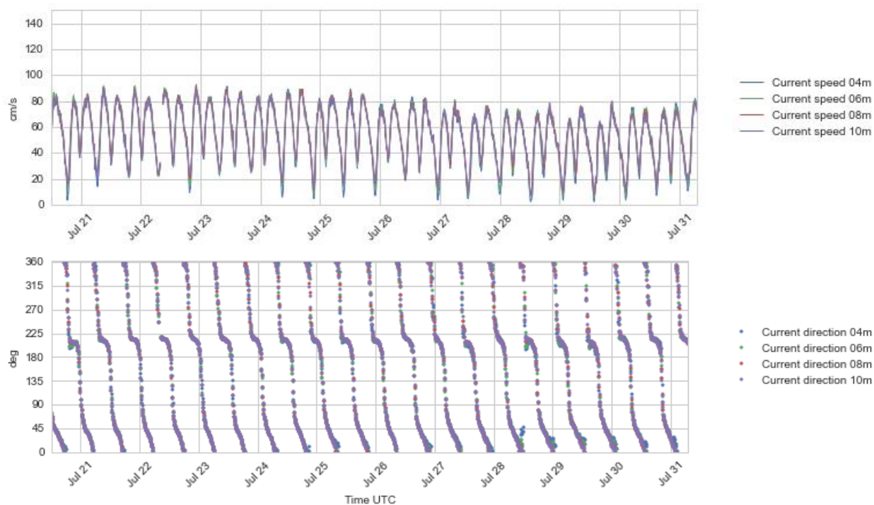
Figure 4.19 Time series plots of current speed (upper) and direction (lower panel), 4 - 10 m depth, 20 – 31 Jul 2016.
