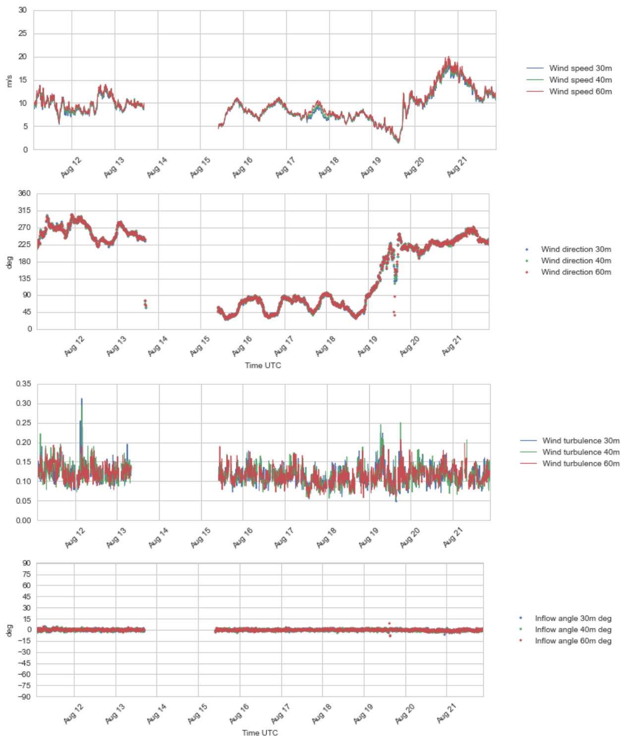
Figure 4.16 Plots of wind profile data, 30 – 60 m a.s.l., 11 - 21 Aug 2016.
