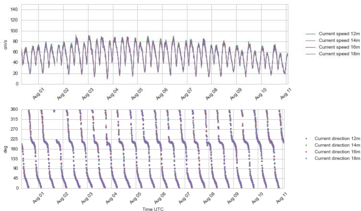
Figure 4.24 Time series plots of current speed (upper) and direction (lower panel), 12 -18 m depth, 31 Jul – 11 Aug 2016.
